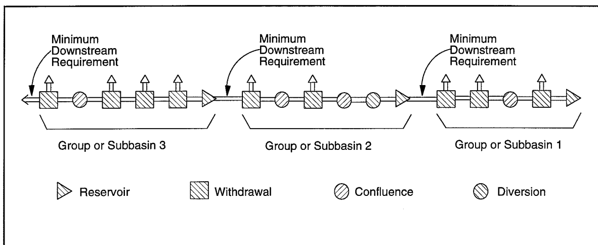
Figure 13: Grouping Nodes into Subbasins
