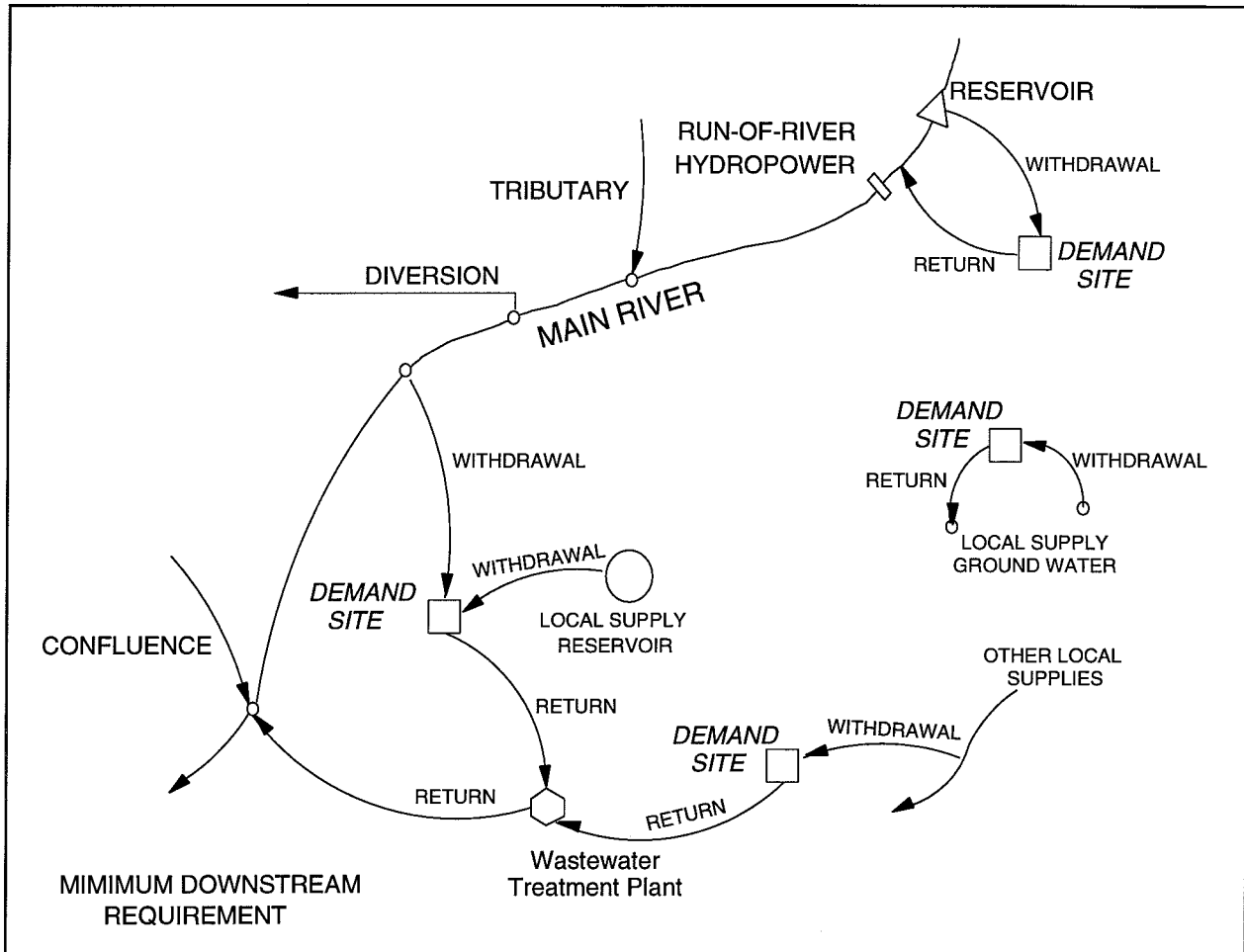
Figure 7: Supply and Demand Features Modeled by WEAP
