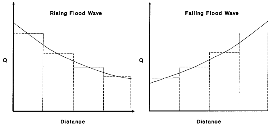
Figure 6 Modified Puls Application to Rising and Falling Flood Waves
