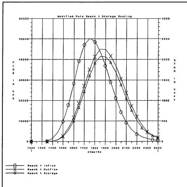
Figure 11 HEC-1 Storage Routing for Reach 1
