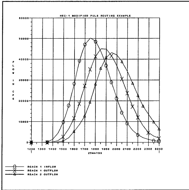
Figure 10 HEC-1 Routed Hydrographs
