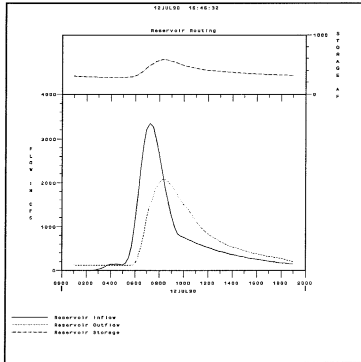
Figure 3 Reservoir Routing
