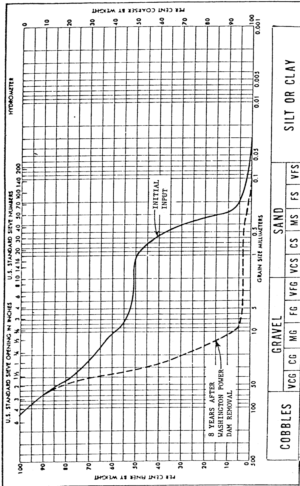
FIGURE 15 PARTICLE SIZE DISTRIBUTION OF BED MATERIAL RIVER MILE 4.62, CLEARWATER RIVER, IDAHO
