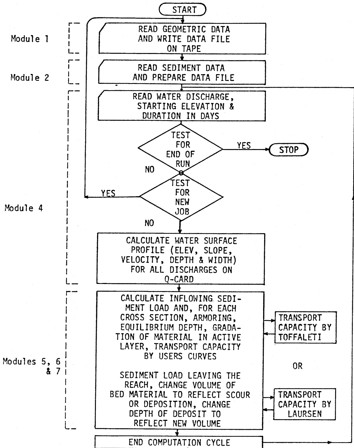
Figure 2 FUNCTIONAL FLOW CHART OF HEC-6
