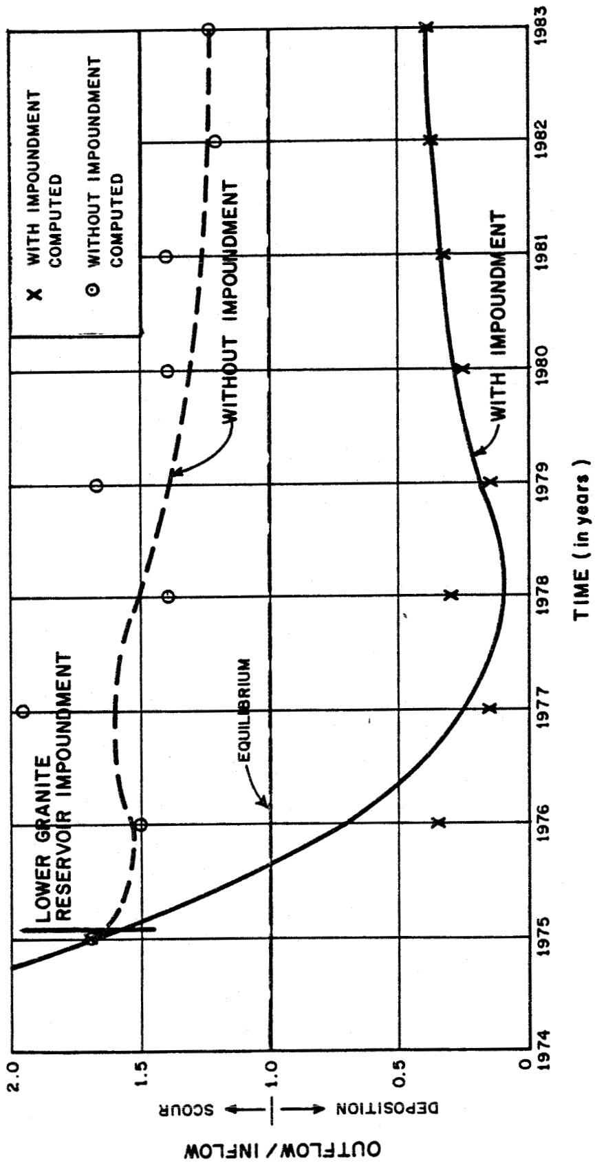
FIGURE 11 CALCULATED RATIO OF SEDIMENT OUTFLOW TO INFLOW WASHINGTON POWER DAM REMOVED
