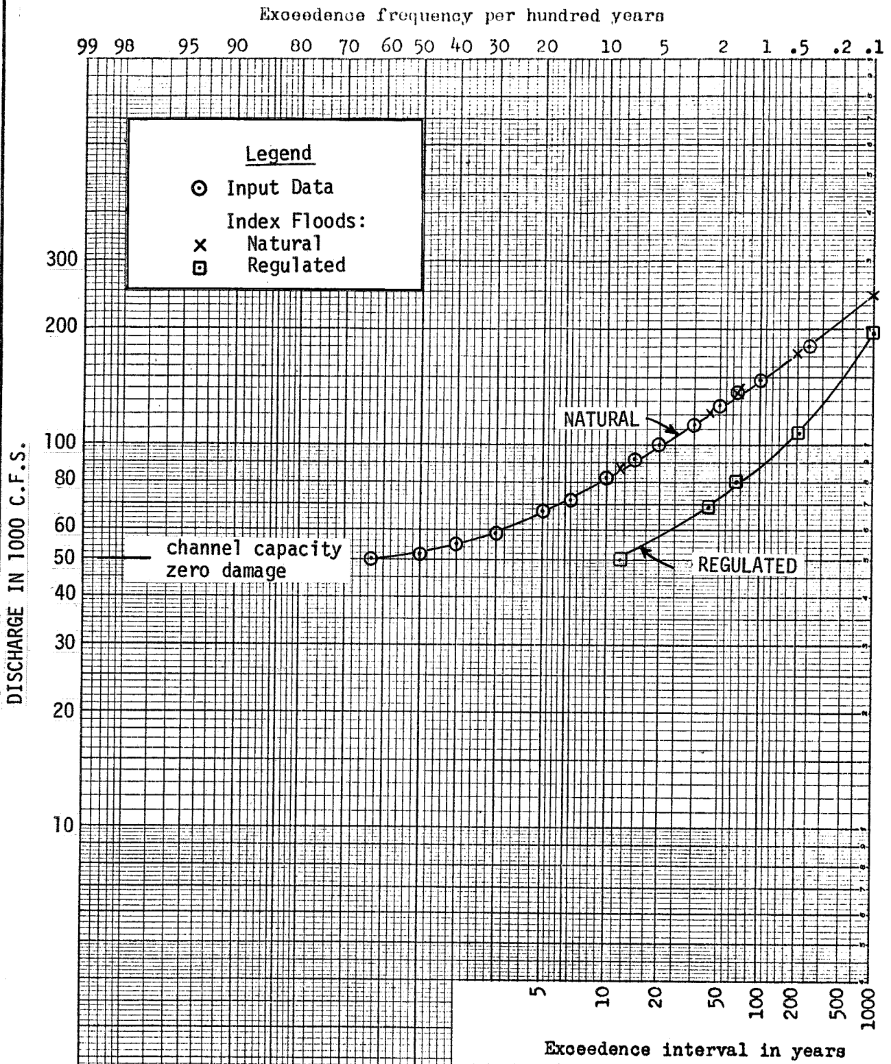
NATURAL AND REGULATED DISCHARGE-FREQUENCY CURVES C.P. #11 Lowell, Mass. Run J
