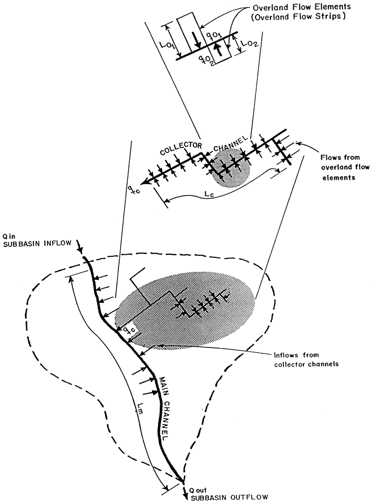
Figure 2. Subbasin Collector System
