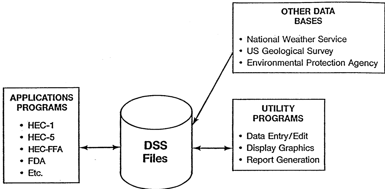
Figure 4. HEC-DSS Data Storage System
