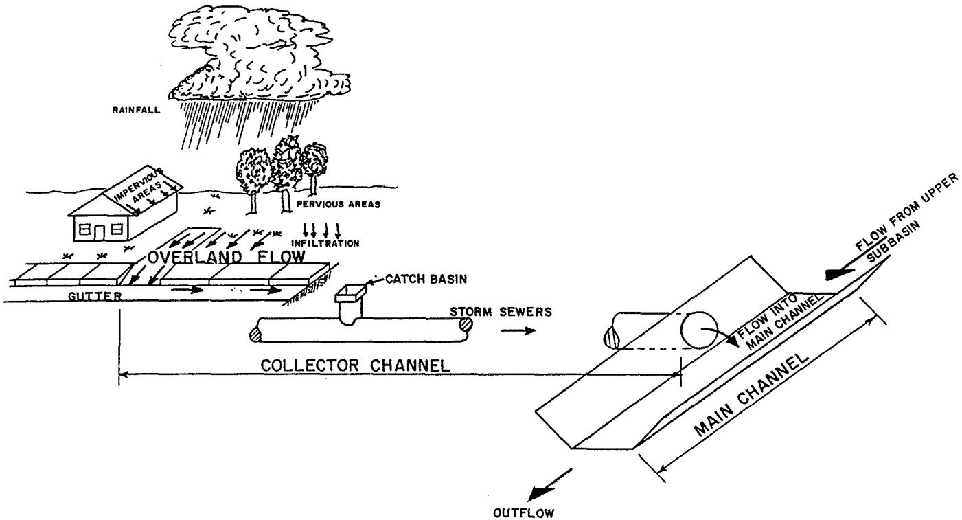
Figure 1. Elements Used in Urban-Runoff Calculations
