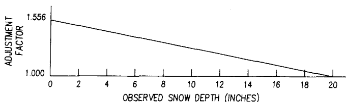
Figure 3. Snow Depth Adjustment Curve.
