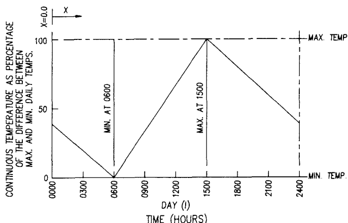
Figure 2. Diurnal Temperature Curve.
