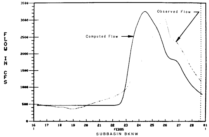
Figure 5. Observed and Computed Flow for Subbasin BKNW.
