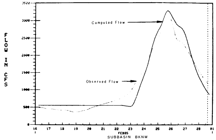
Figure 6. Observed and Computed (with weighting and lag adjustment) Flows for Subbasin BKNW.
