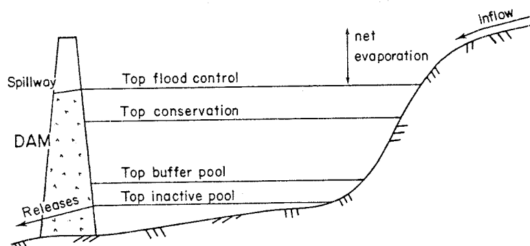
Fig. 1 Reservoir Operating Levels
