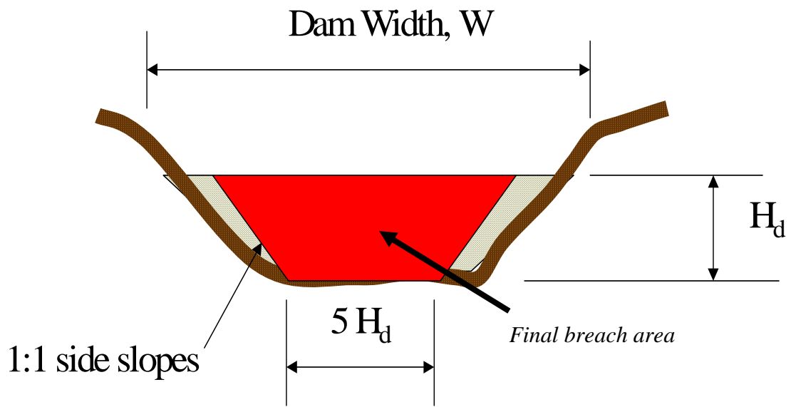
Figure 1. Breach geometry for earthen dams
