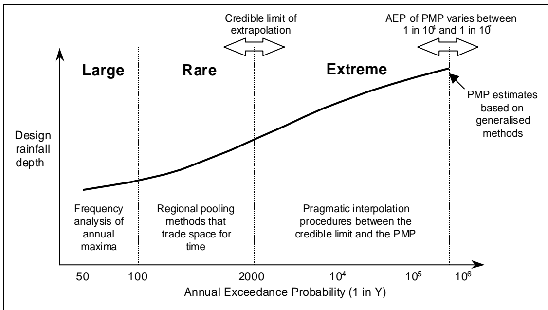
Figure 2: Summary of procedures used to derive design rainfall depths.
