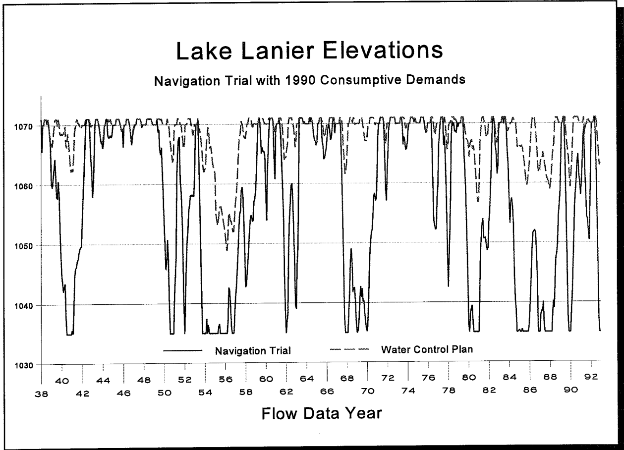
Figure 3. Lanier Elevations Under Two Different Operating Rule Sets
