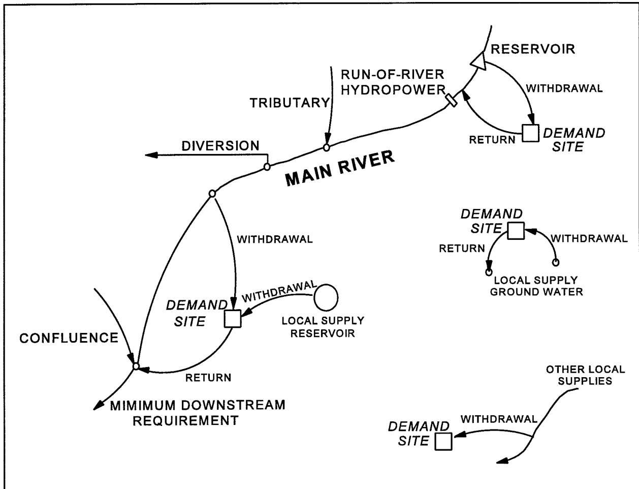
Figure 2: Supply and Demand Featuresn Modeled by WEAP
