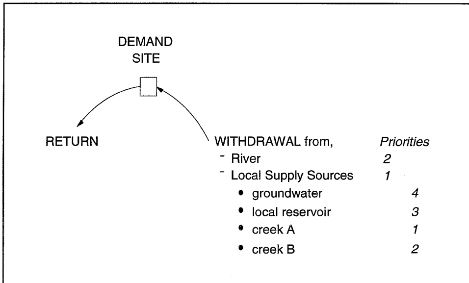
Figure 6: Priority Between Local Supply Sources
