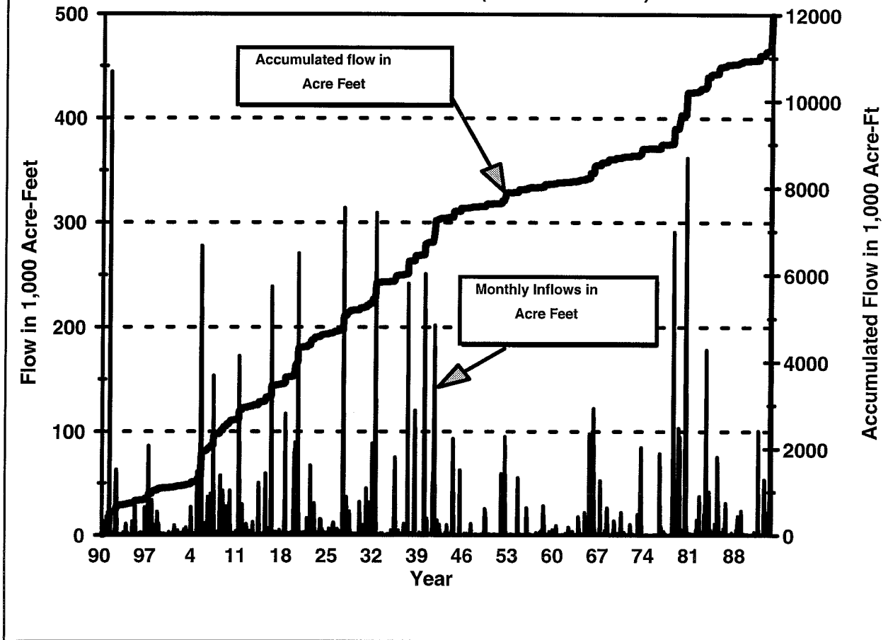
Figure 4- Alamo Dam Monthly Flows Period of Record (1890-1993)
