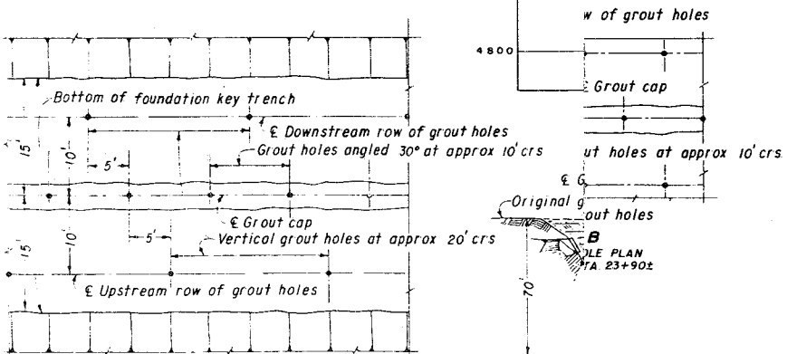
DETAIL A TYPICAL GROUT HOLE PLAN ABOVE EL 5100
