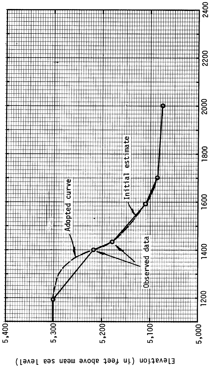
TETON DAM ELEVATION HYDROGRAPH FOR RESERVOIR
