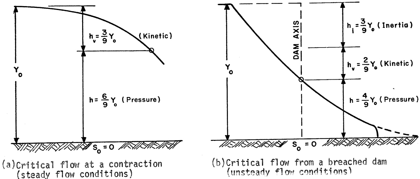
Figure 1. Components of Specific Energy Head.
