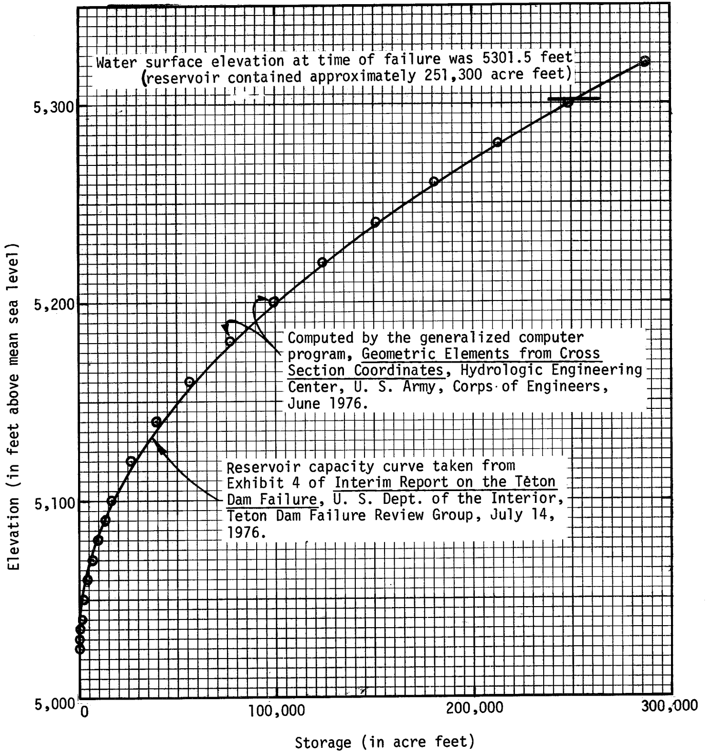
TETON DAM RESERVOIR CAPACITY Storage versus Elevation
