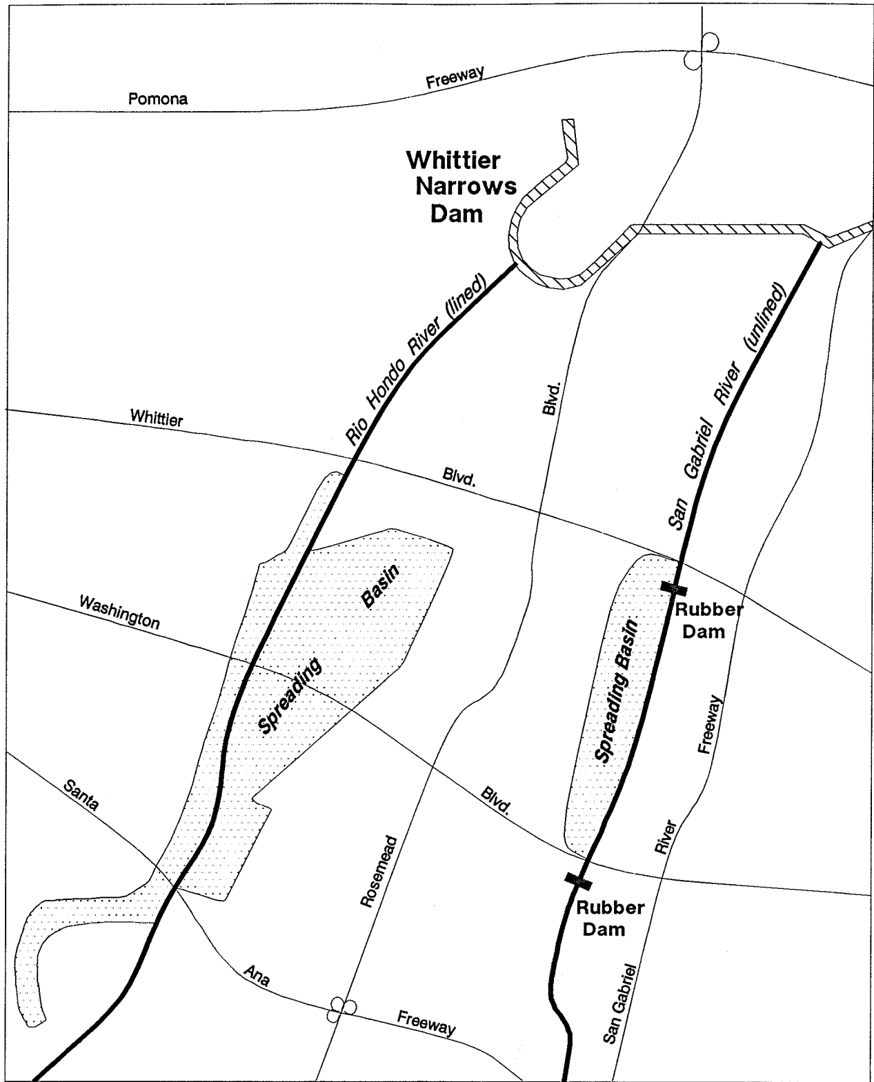
Figure 3: Whittier Narrows Dam and downstream recharge basins
