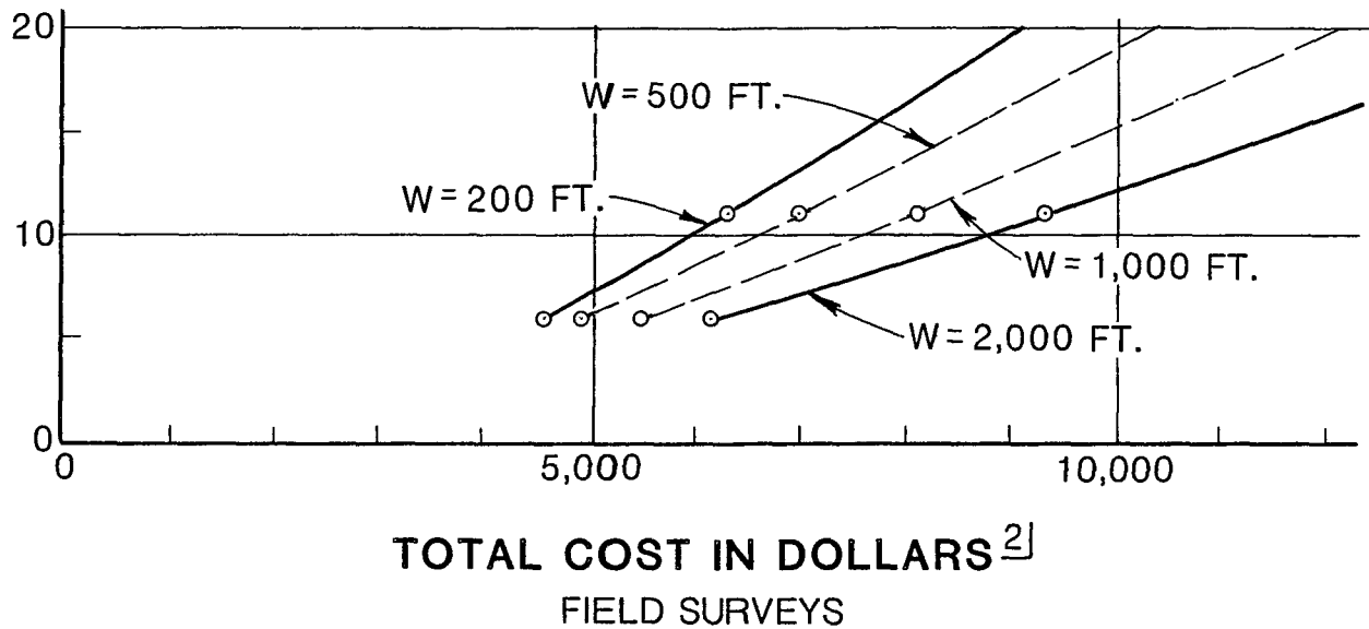
FIELD AND AERIAL SURVEYS COST INFORMATION - CROSS SECTIONS ONLY STEEP, HEAVY-COVER CASE
