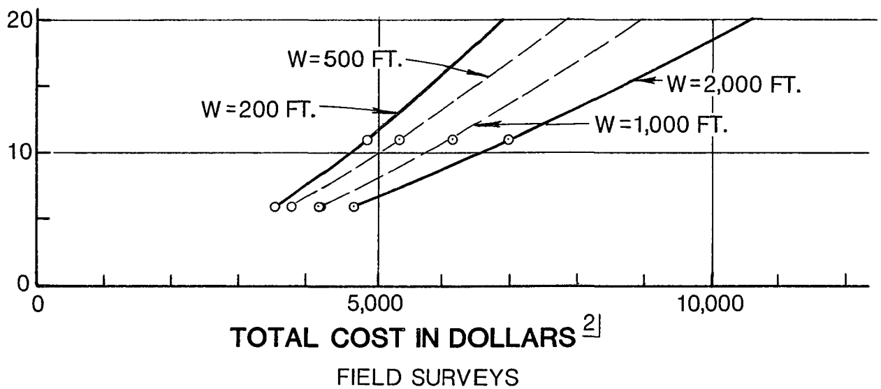
FIELD AND AERIAL SURVEYS COST INFORMATION - CROSS SECTIONS ONLY FLAT, LIGHT-COVER CASE
