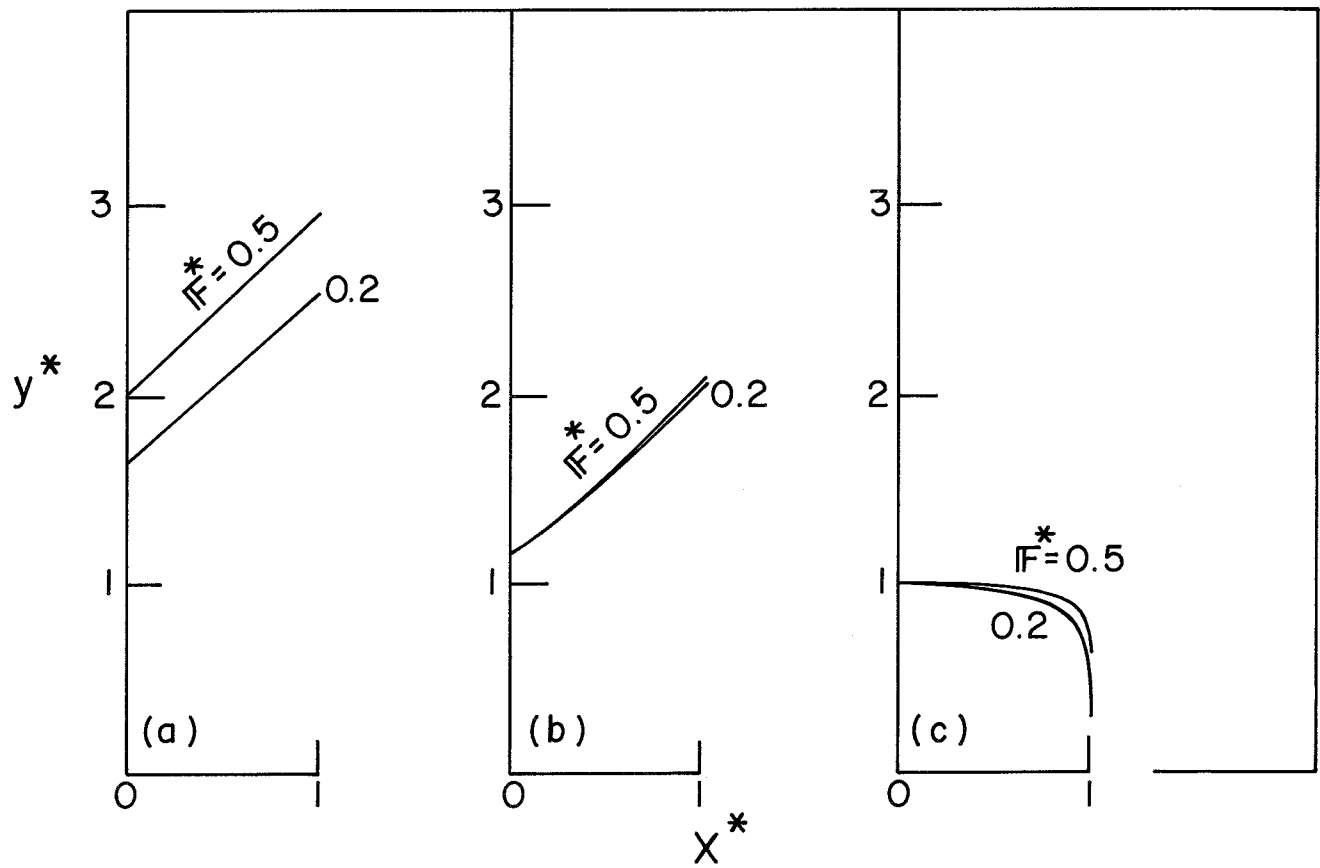
Fig. 1. Initial conditions. Base-flow depth profiles.
