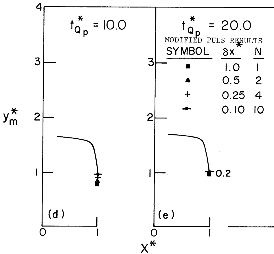
Fig. 21 d-e Attenuation of stage hydrograph peaks, channel with floodplain, overfall downstream boundary condition.
