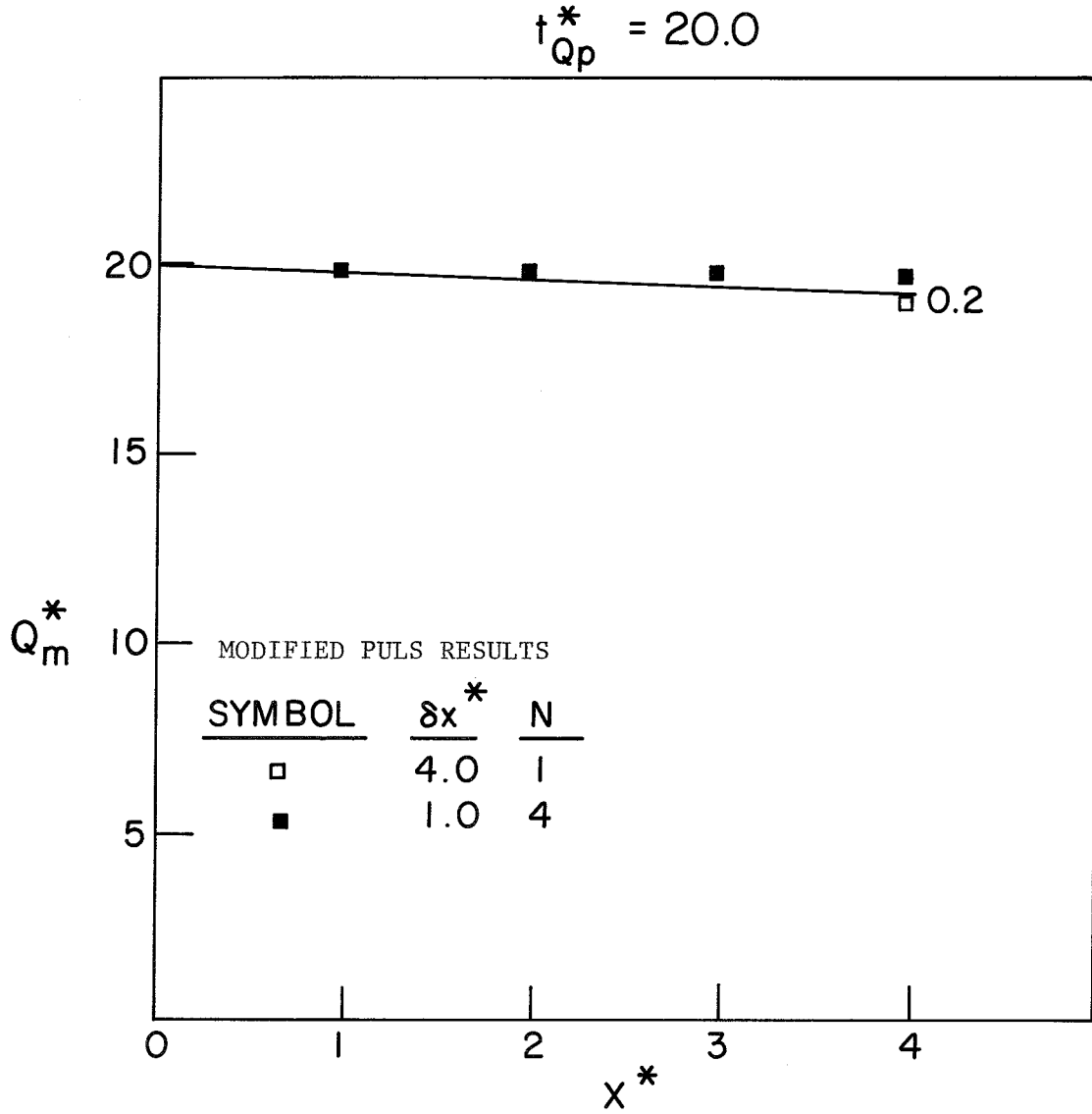
Fig. 10g Attenuation of discharge hydrograph peaks, rectangular channel, normal depth downstream boundary condition.
