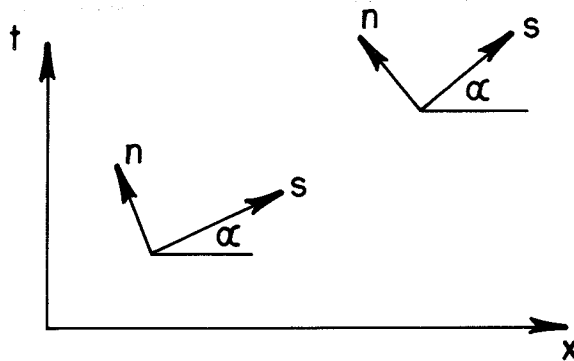
Fig. 4. Characteristic coordinates.
