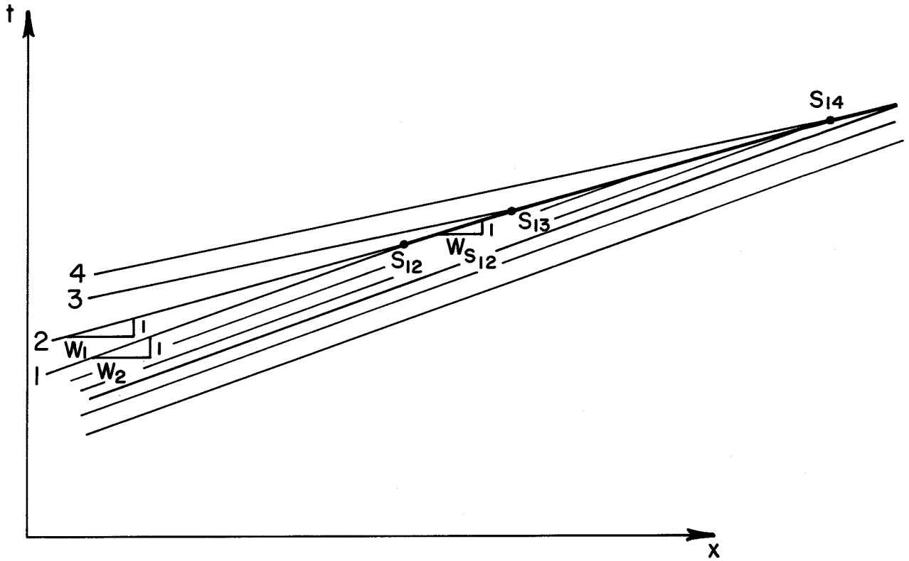
Fig. 7. Formation and propagation of a kinematic shock.
