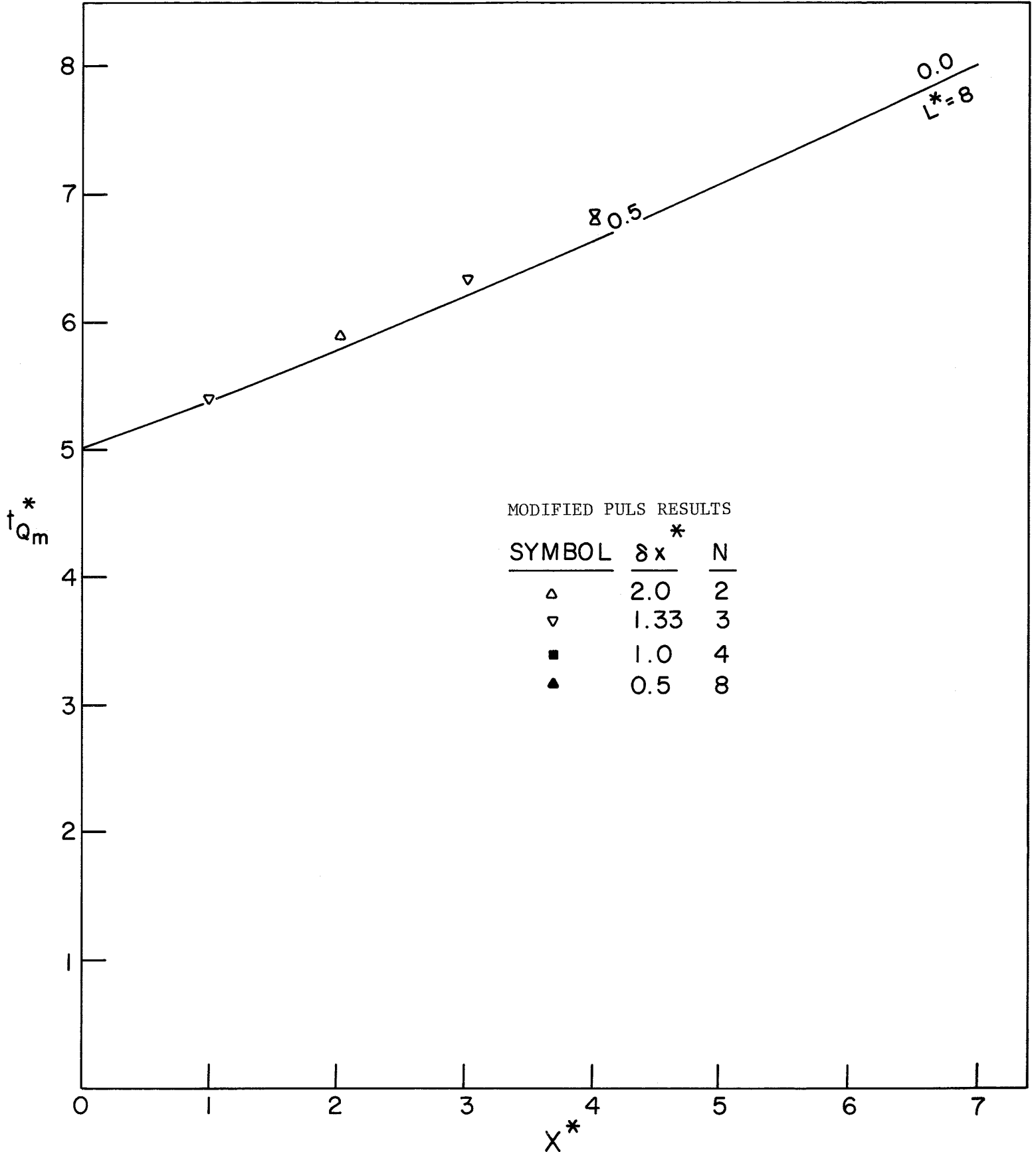
Fig.22d Time of arrival of peak discharge, rectangular channel, normal depth downstream boundary condition.
