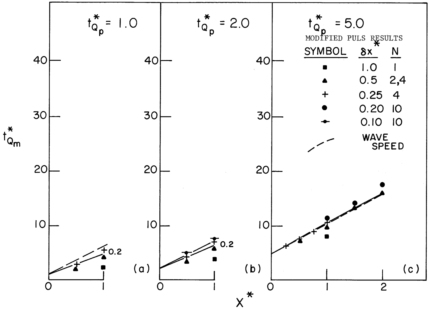
Fig. 27 a-c Time of arrival of peak discharge, channel with floodplain, overfall downstream boundary condition.
