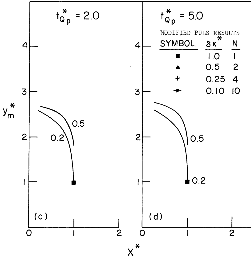
Fig. 18 c-d Attenuation of stage hydrograph peaks, rectangular channel, overfall downstream boundary condition.
