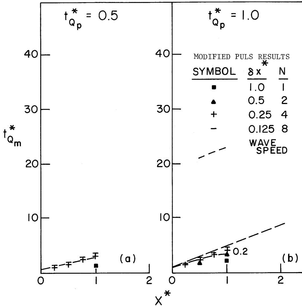
Fig. 26 a-b Time of arrival of peak discharge, channel with floodplain, weir downstream boundary condition.
