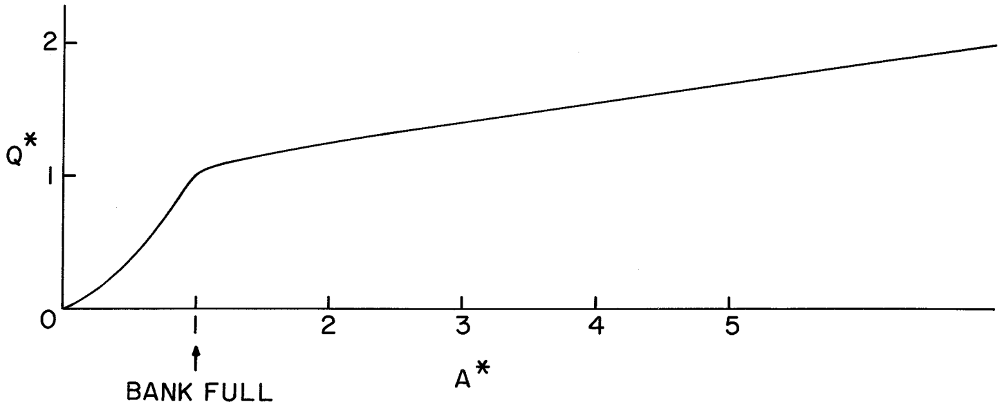
Fig. 8. Discharge-area relation for channel with floodplains.
