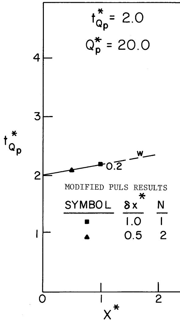
Fig. 23f Time of arrival of peak discharge, rectangular channel, weir downstream boundary condition.
