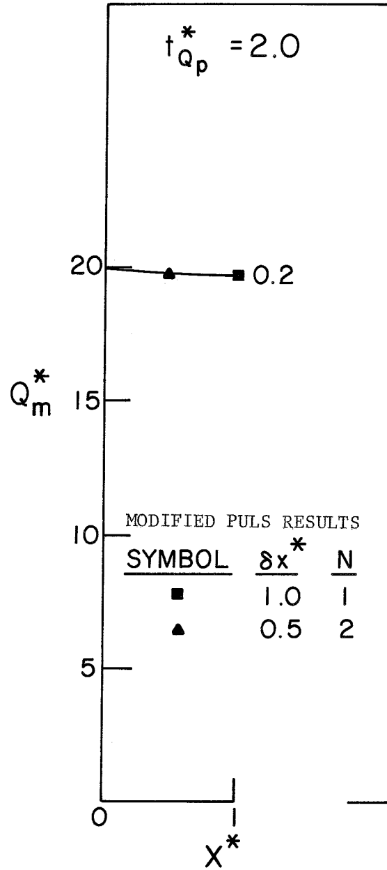
Fig. II f Attenuation of discharge hydrograph peaks, rectangular channel, weir downstream boundary condition.
