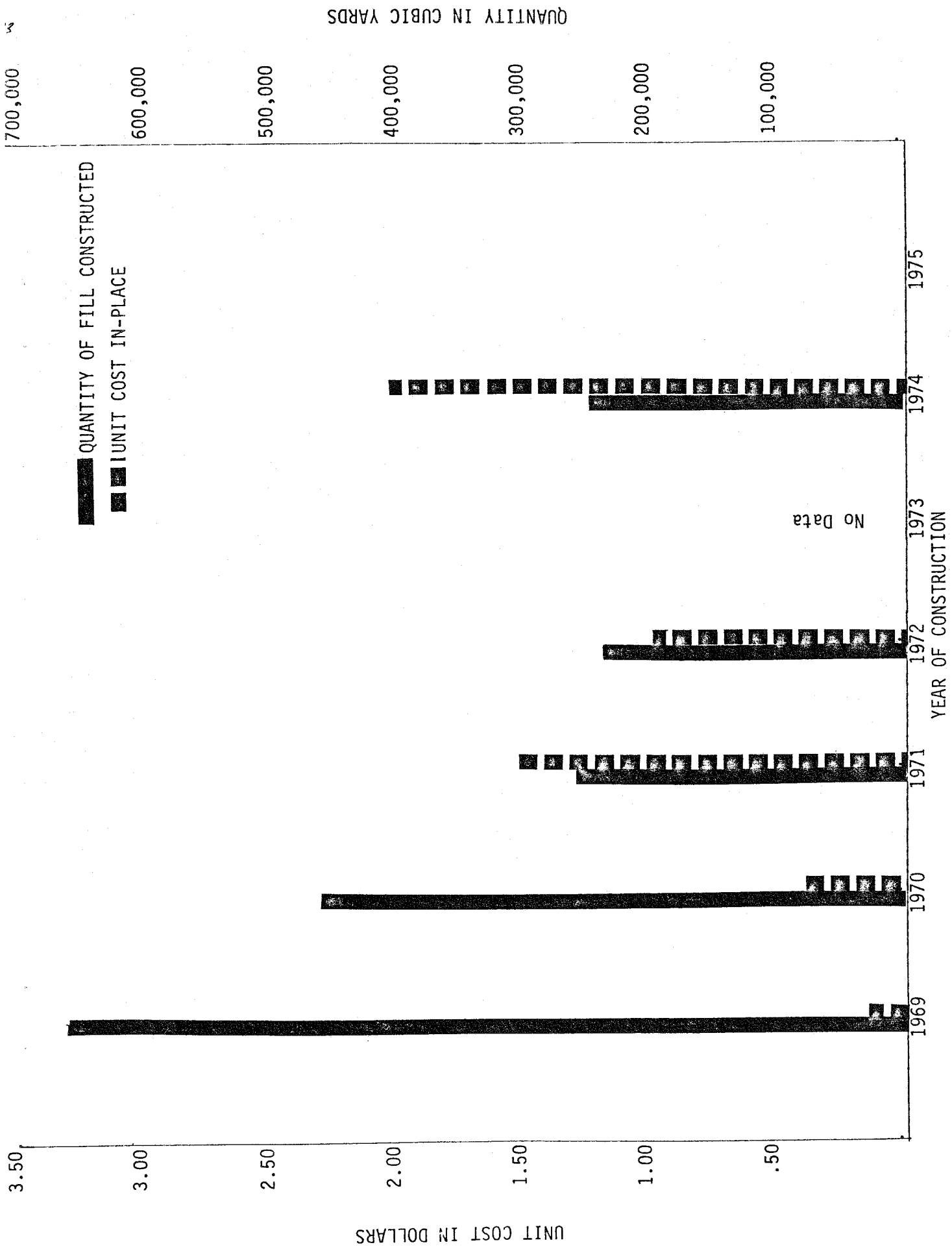
FIGURE 4 - Representative Projects for Semi-Compacted Fills
