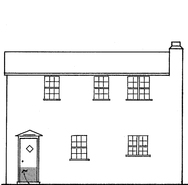
TEMPORARY FLOOD SHIELD WITH RUBBER GASKET SEAL.
