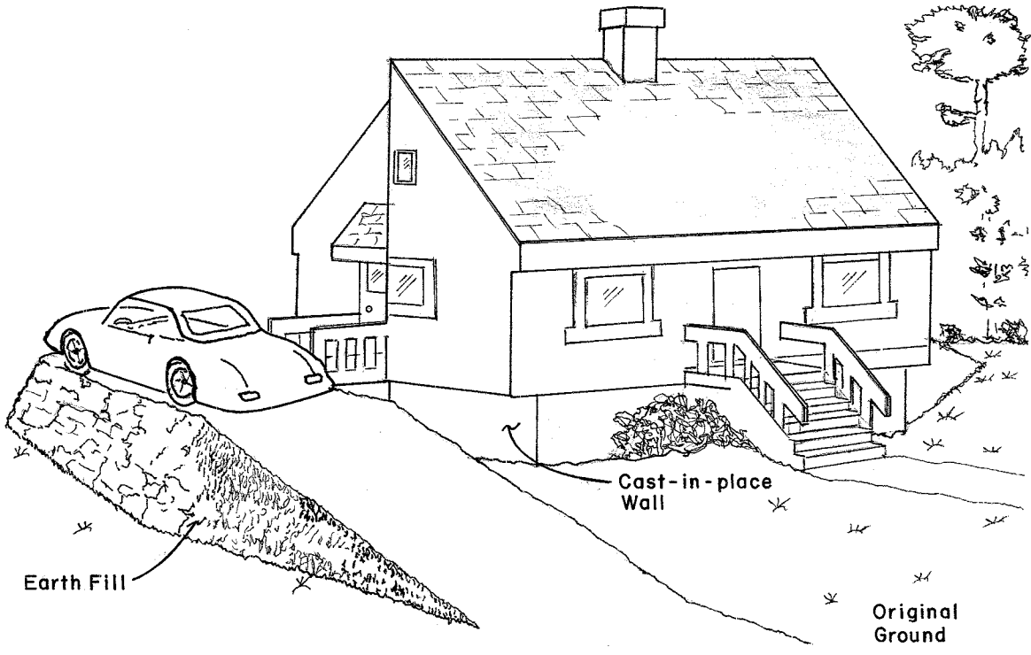
ELEVATION BY CAST-IN-PLACE FOUNDATION WALL
