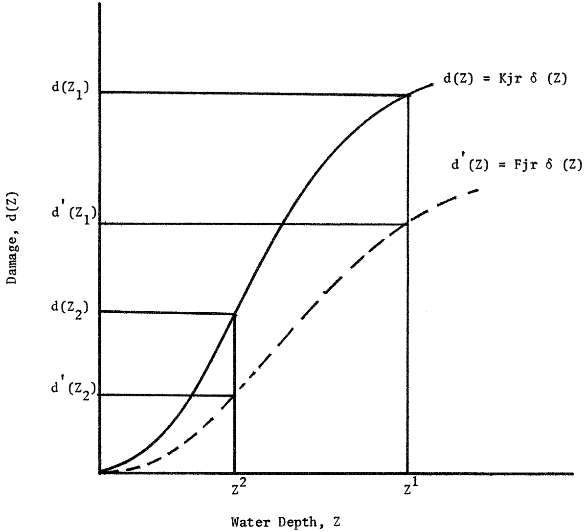
Figure III-4 Two Methods of Floodproofing 8
