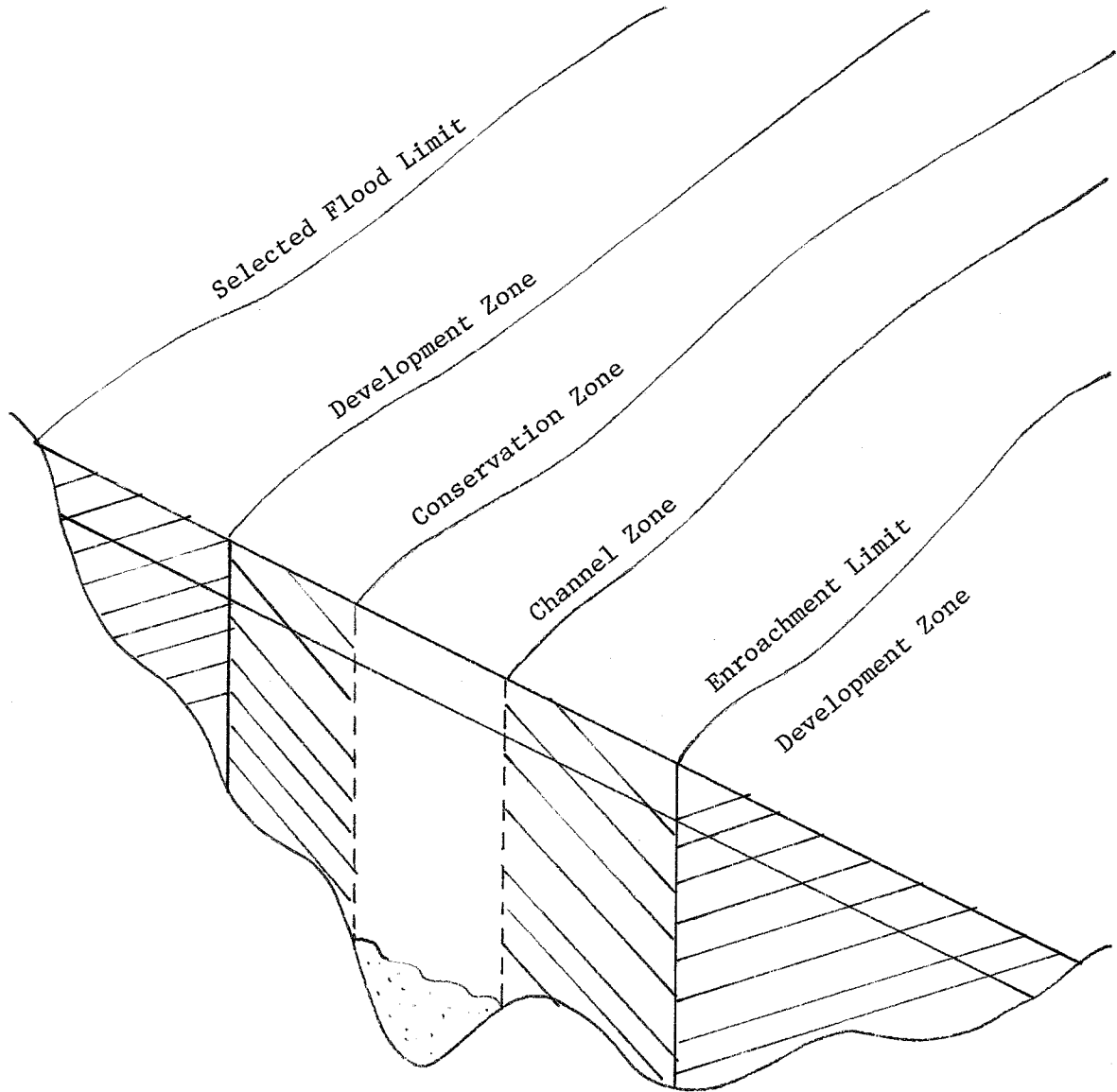
Figure II-3 Floodplain Utilization
