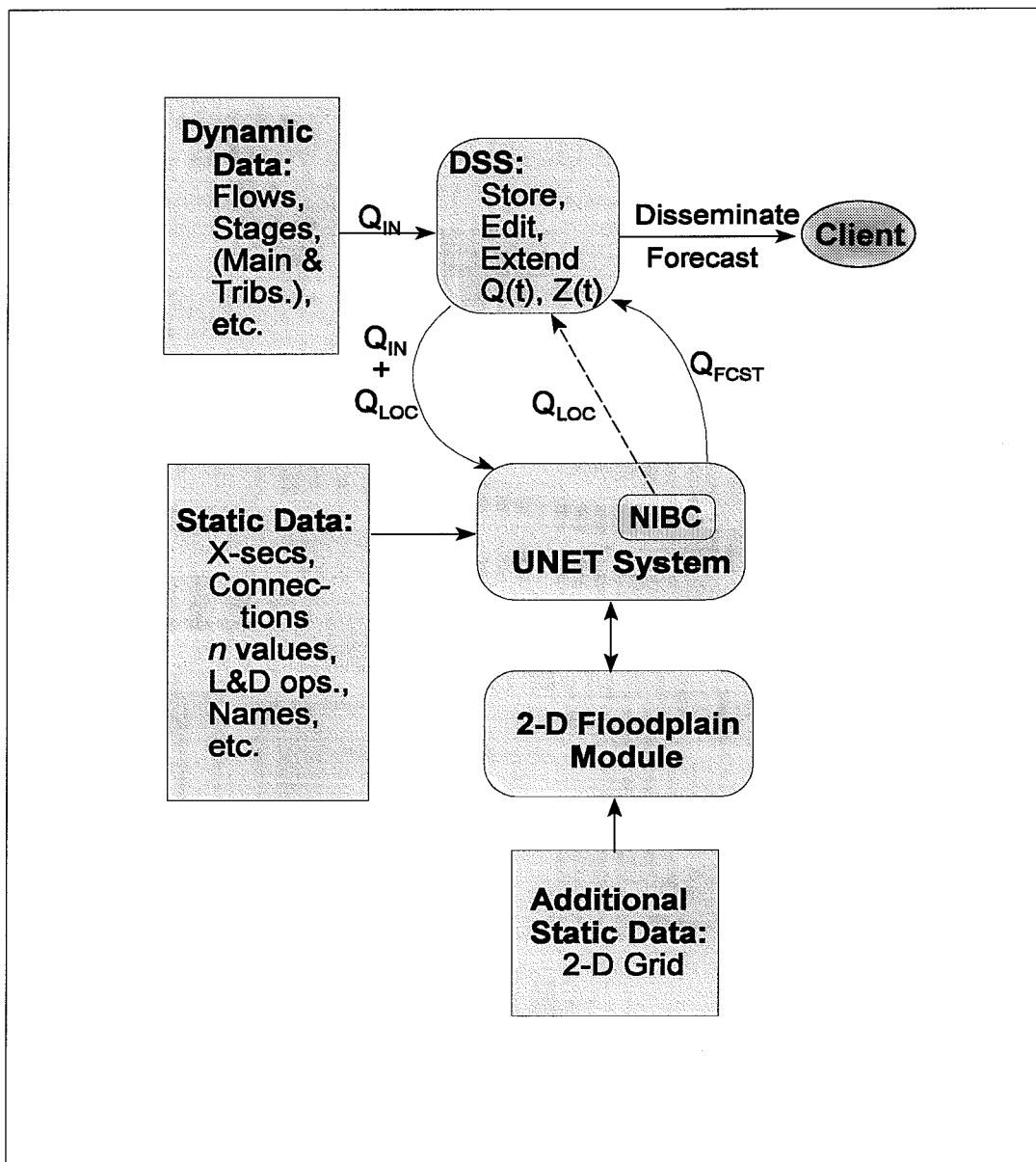
Figure 2.2. Components of the MBMS. NIBC = Null Internal Boundary Condition (Section 3.3.4).
