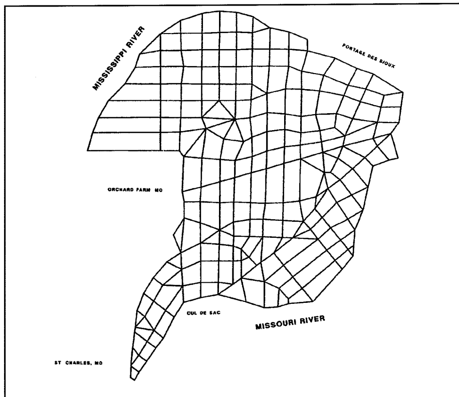
Figure 3-7. Two-Dimensional Model Grid for Crossover Area.
