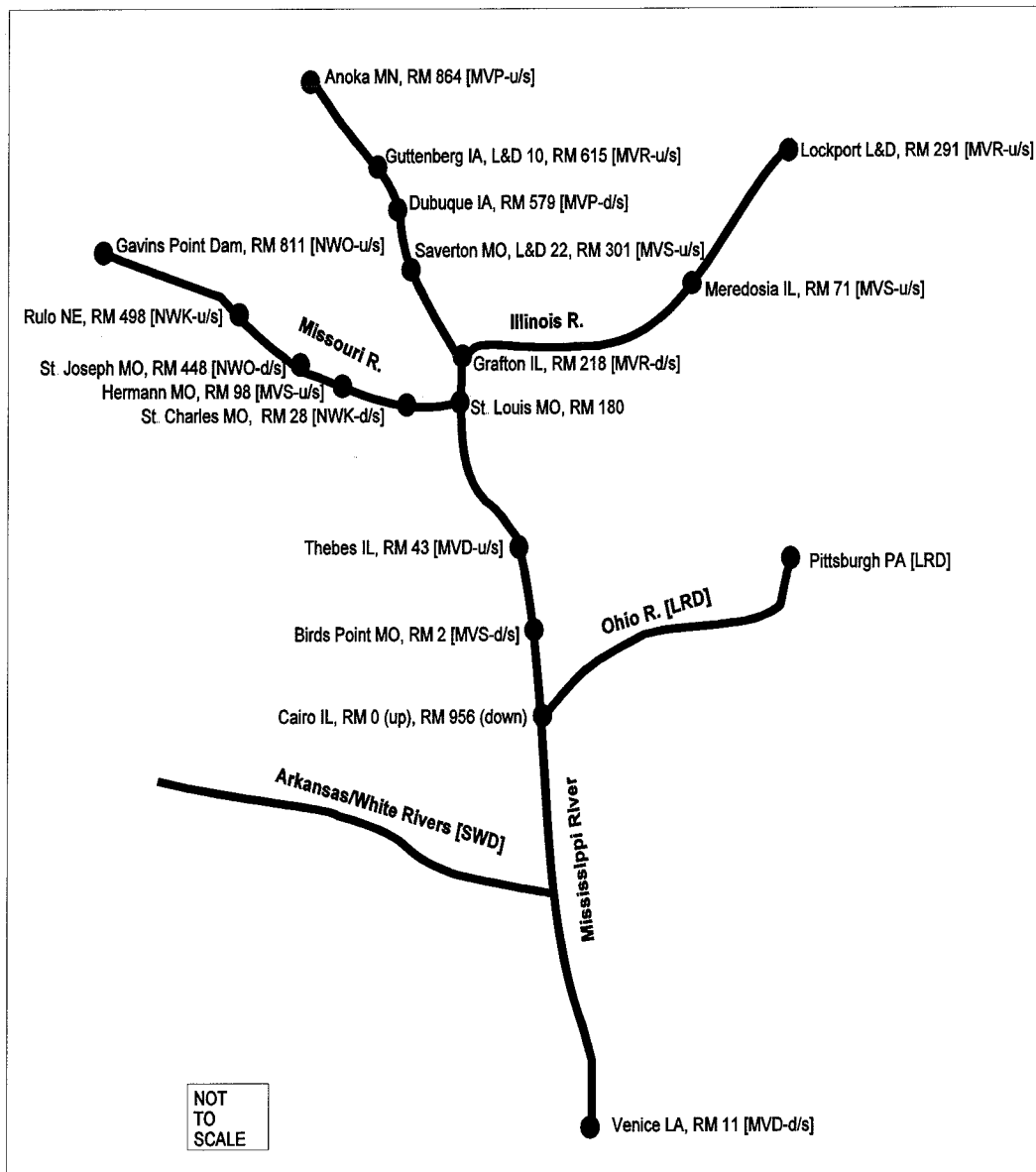
Figure 2-1. Schematic Diagram of MBMS Geographic Extent. (u/s = upstream location of UNET boundary condition, d/s = downstream location of UNET boundary condition.)
