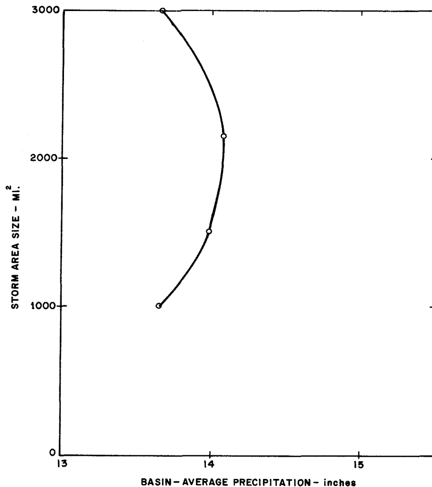
Figure 18. 18-hr Basin-Average Precipitation for 3,660 mi 2 Leon River Basin
