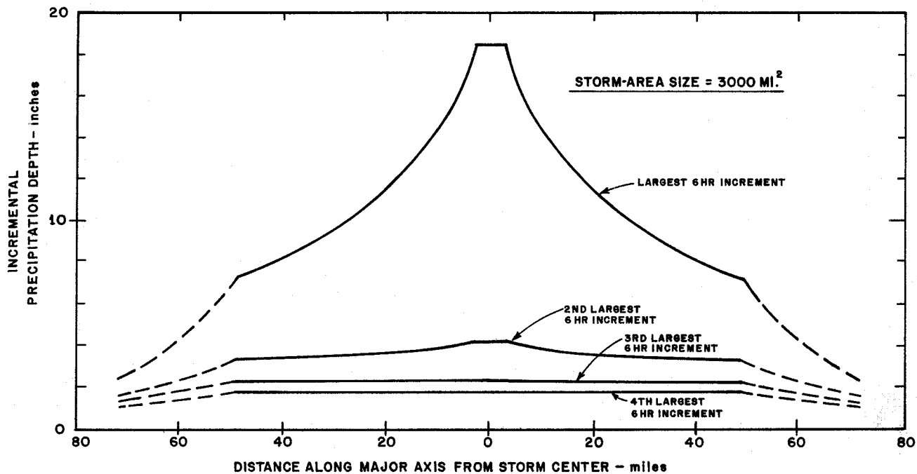
Figure 6. Spatial Variation in PMP Intensities
