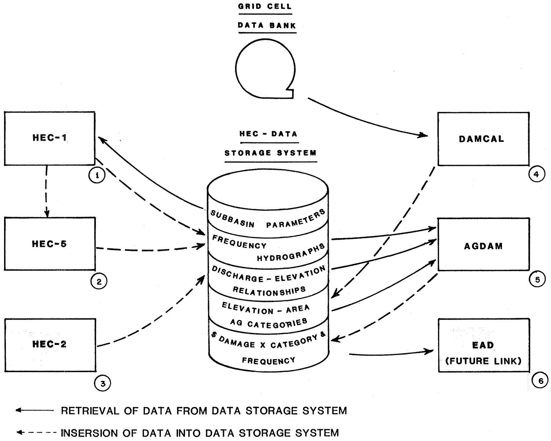
Figure 2.2 AGDAM DATA STORAGE PROCESSING SCHEMATIC
