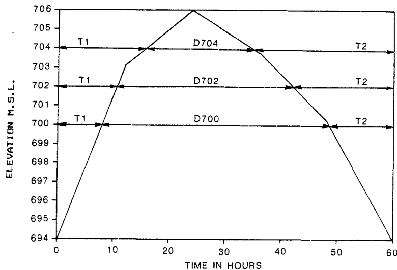
FIGURE E1.3 ELEVATION HYDROGRAPH
