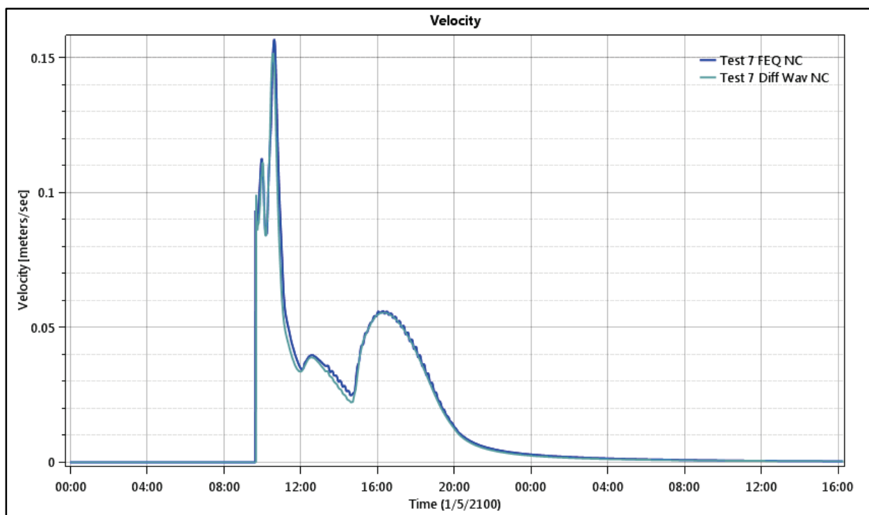
Figure 123. Floodplain 2 - Test Point 8 - Velocity.
