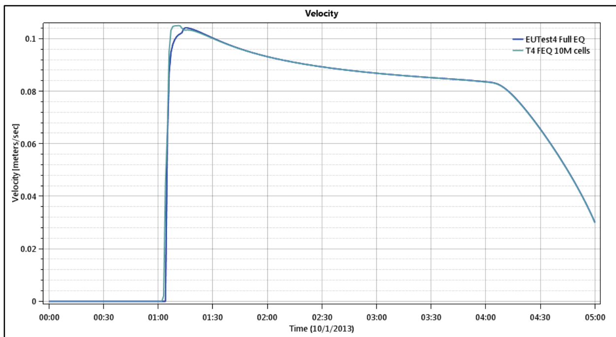
Figure 43. Test Point 6 - Velocity versus Time - 5 and 10 Meter Grids.
