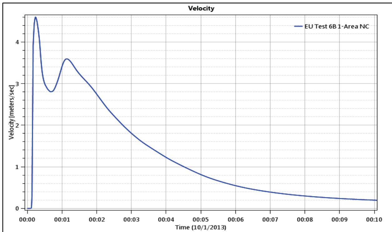
Figure 84. Test Point 2 - Velocity Time Series.
