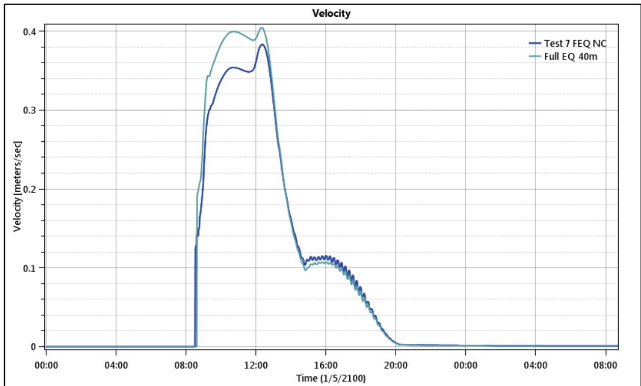
Figure 150. Floodplain 2 - Test Point 7 - Velocity.
