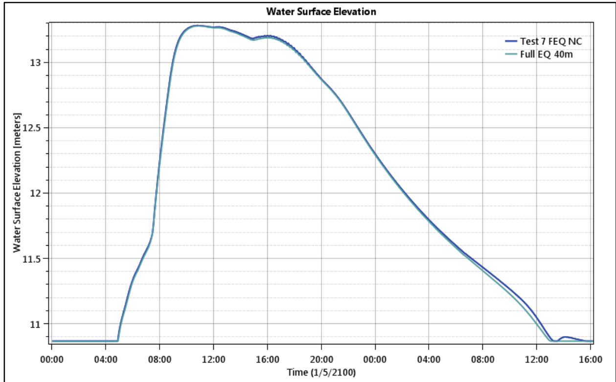
Figure 147. Floodplain 1 - Test Point 6 - Water Level.
