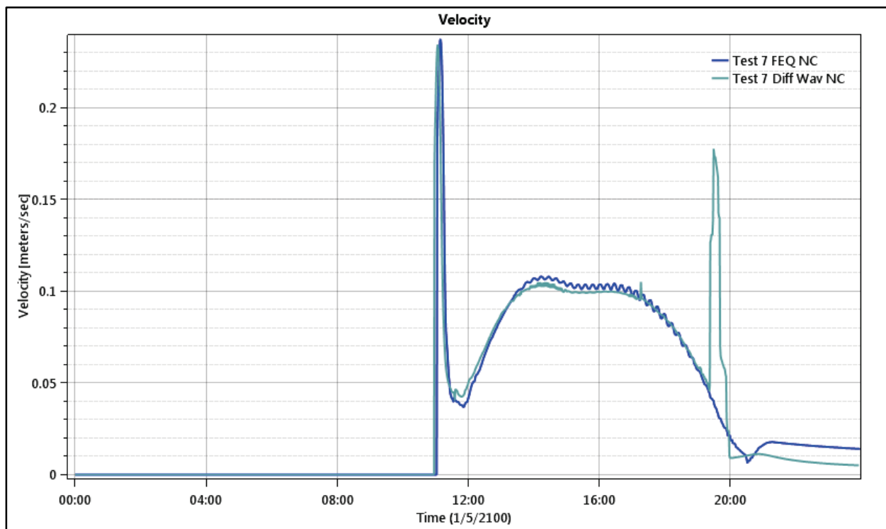
Figure 131. Floodplain 3 - Test Point 12 - Velocity.
