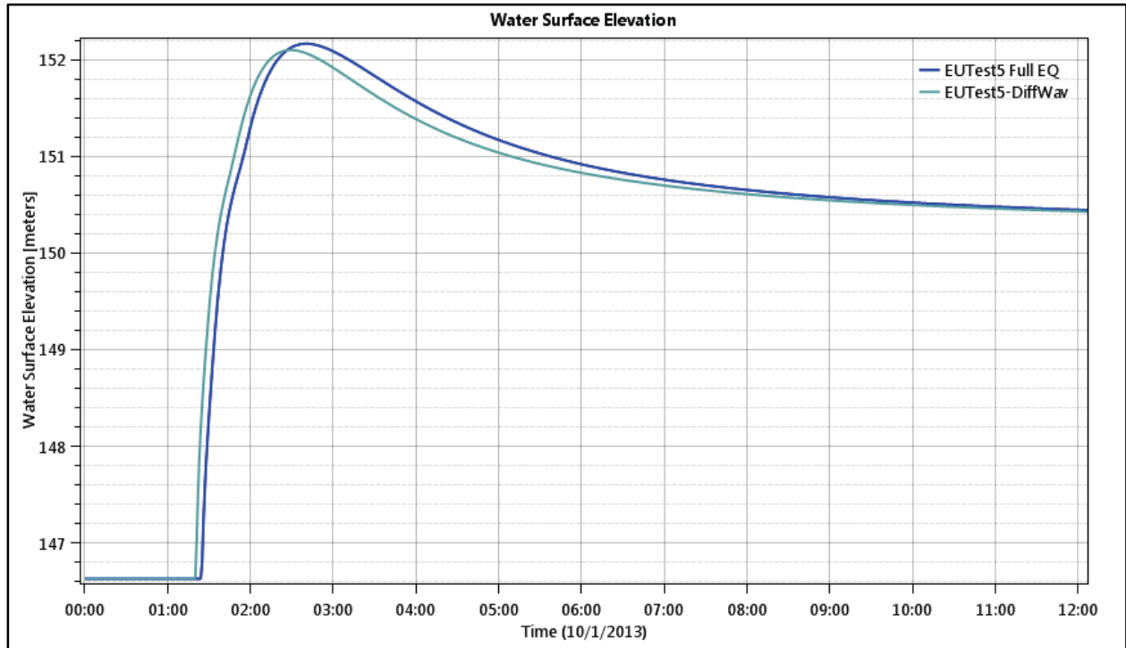
Figure 52. Test Point 4 - Water Level (depth) for Full Equations and Diffusion Wave.
