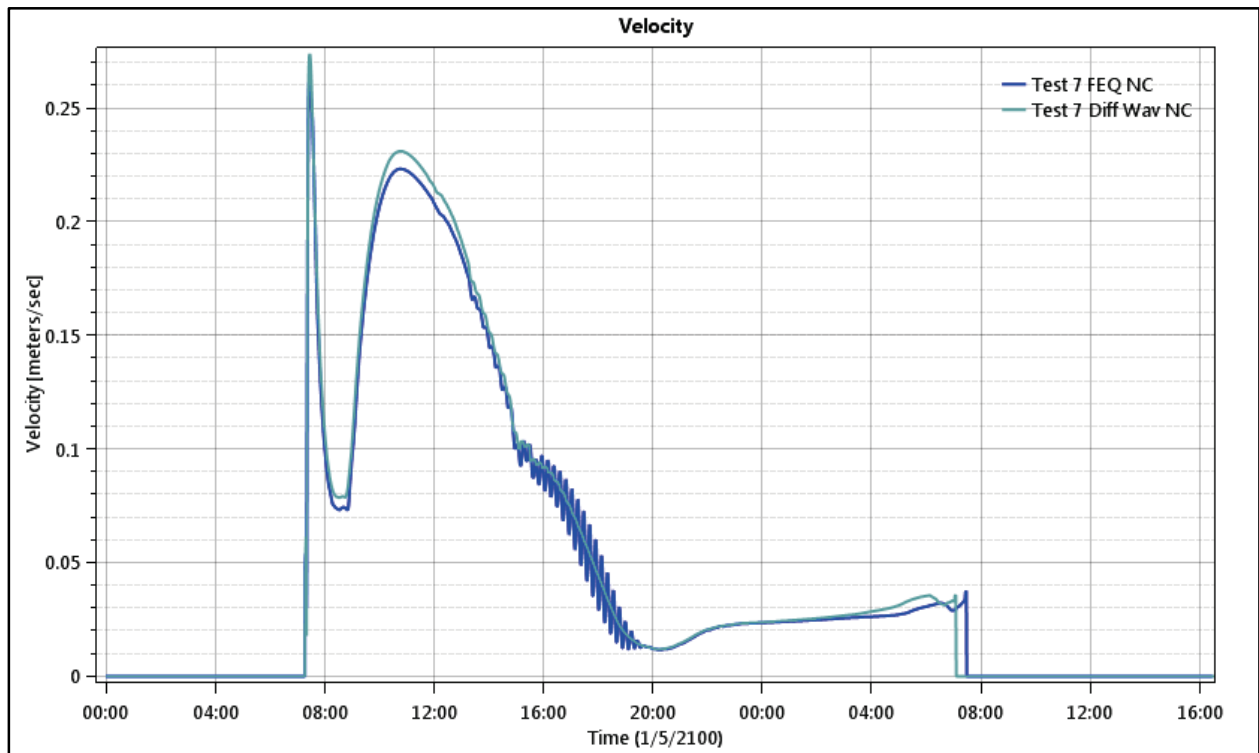
Figure 115. Floodplain 1 - Test Point 4 - Velocity.
