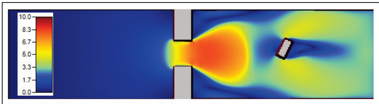
Figure 94. Velocity at time equal to 30 seconds (meter per second).
