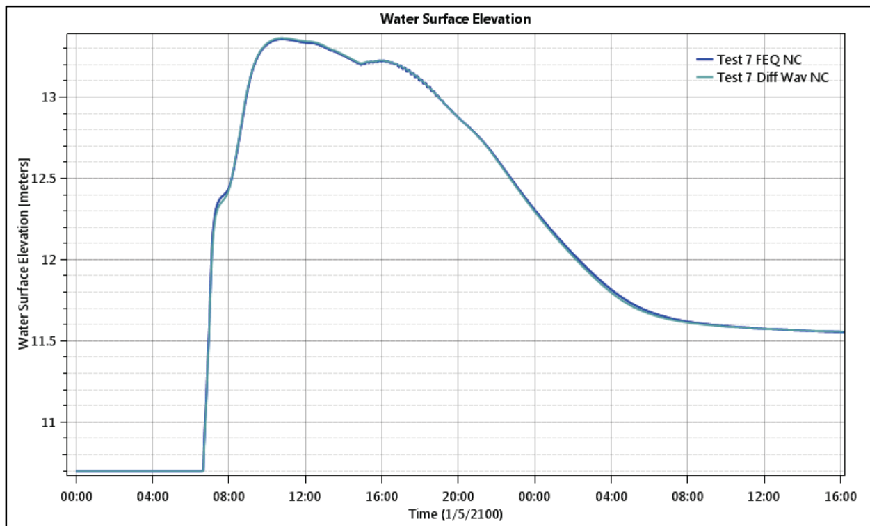
Figure 110. Floodplain 1 - Test Point 2 - Water Level.
