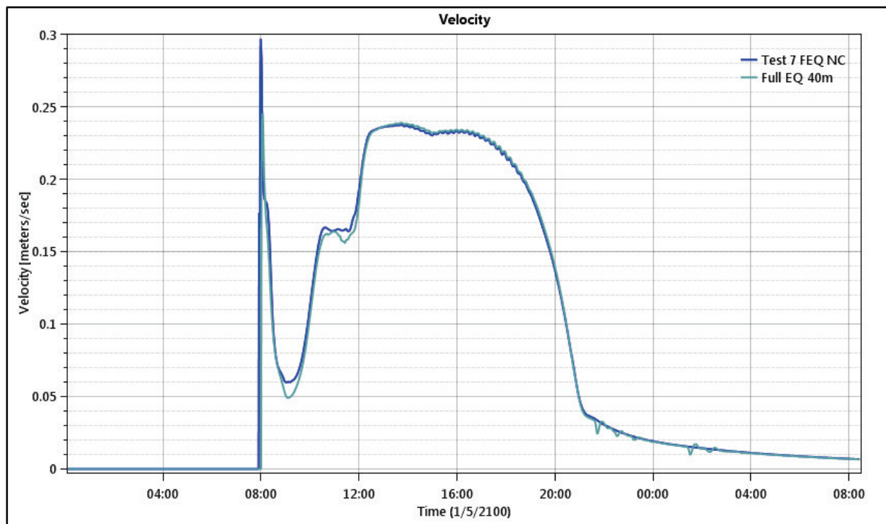
Figure 156. Floodplain 3 - Test Point 15 - Velocity.
