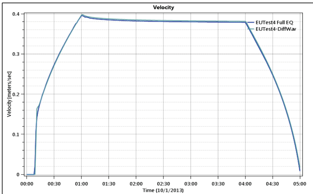
Figure 27. Test Point 1 Velocity Time Series.
