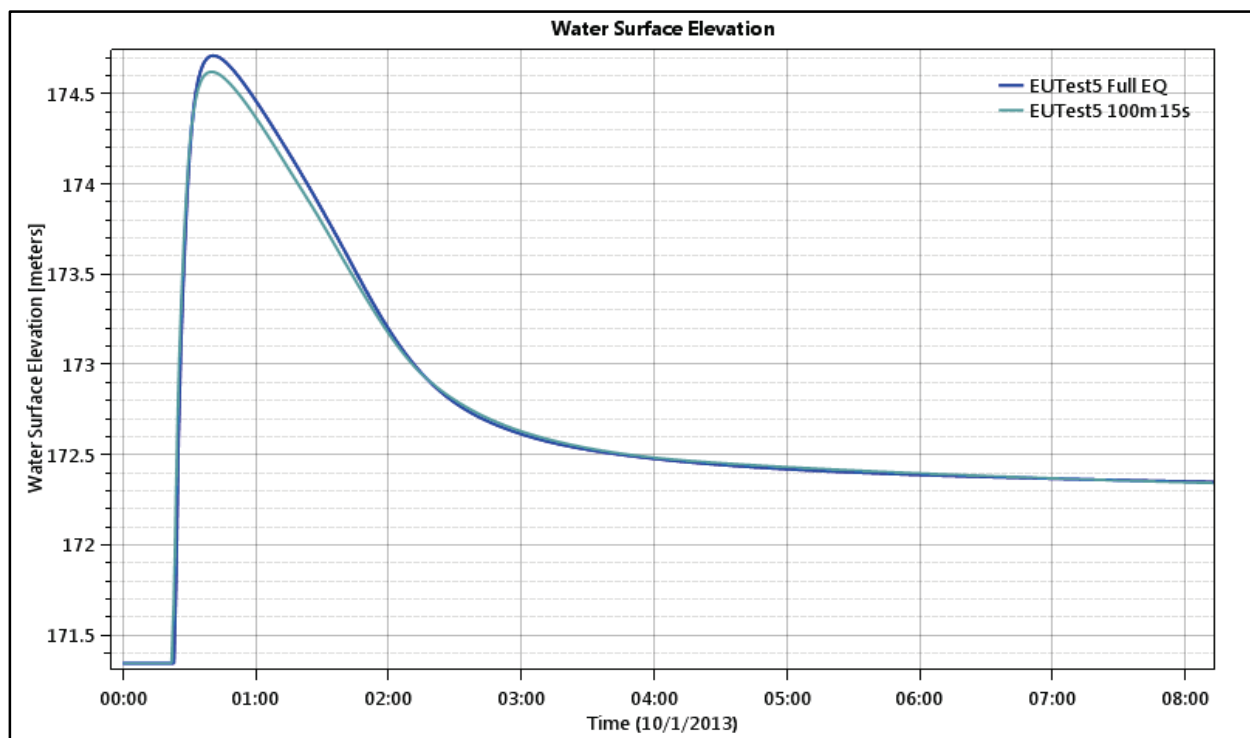
Figure 70. Test Point 1 - Water Level (depth), 50 and 100 meter grids.
