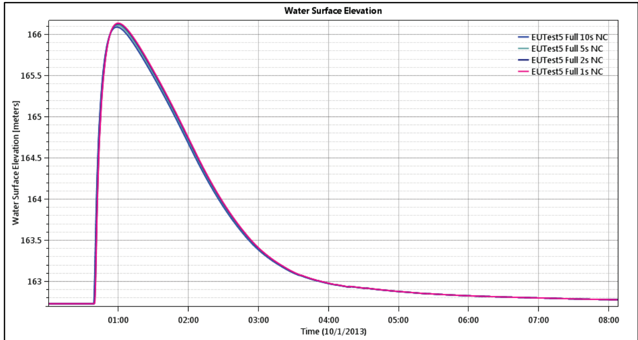
Figure 62. Test Point 2 - Water Level (depth), \Delta T = 1, 2, 5, 10 seconds.
