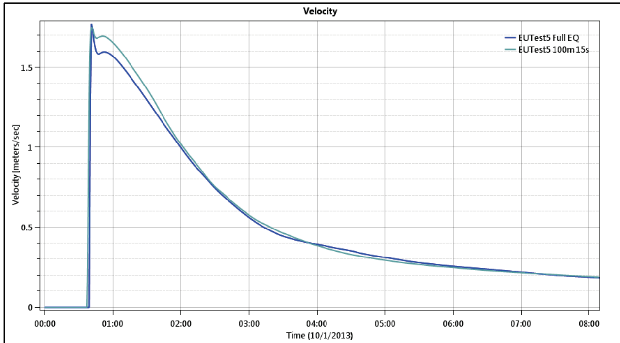
Figure 73. Test Point 2 - Velocity Time Series, 50 and 100 meter grids.
