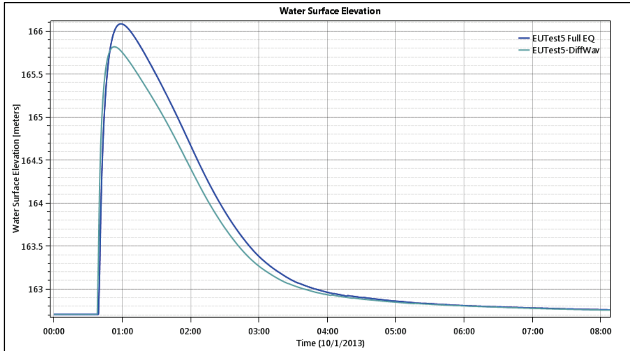
Figure 48. Test Point 2 - Water Level (depth) for Full Equations and Diffusion Wave.
