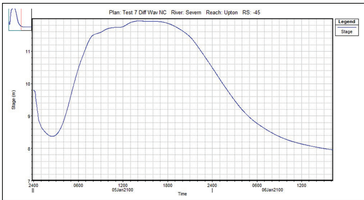
Figure 107. Test Point M045 - Water Level (depth).
