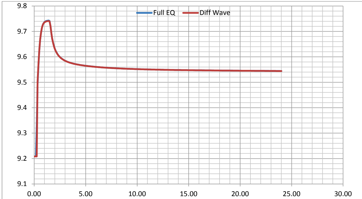
Figure 7. Test Point 4 - Water Level (m) versus Time (hrs).
