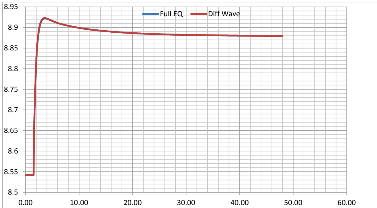
Figure 9. Test Point 2 - Water Level (m) versus Time (hrs).
