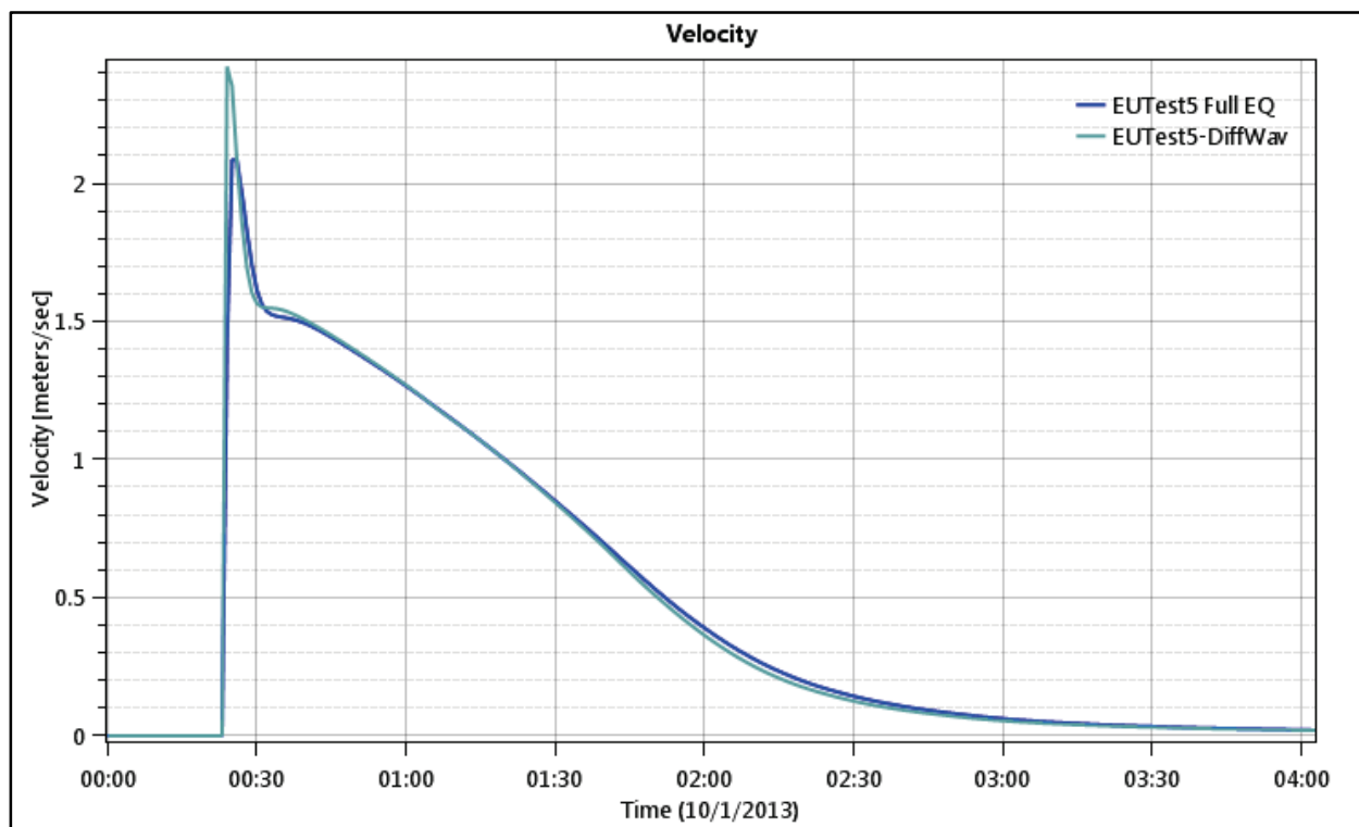
Figure 47. Test Point 1 - Velocity Time Series for Full Equations and Diffusion Wave.
