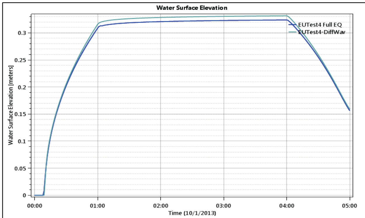
Figure 26. Test Point 1 Water Level (depth).
