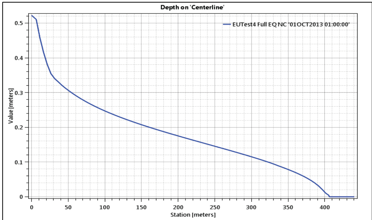
Figure 38. Depth versus Distance at Time 1HOUR.
