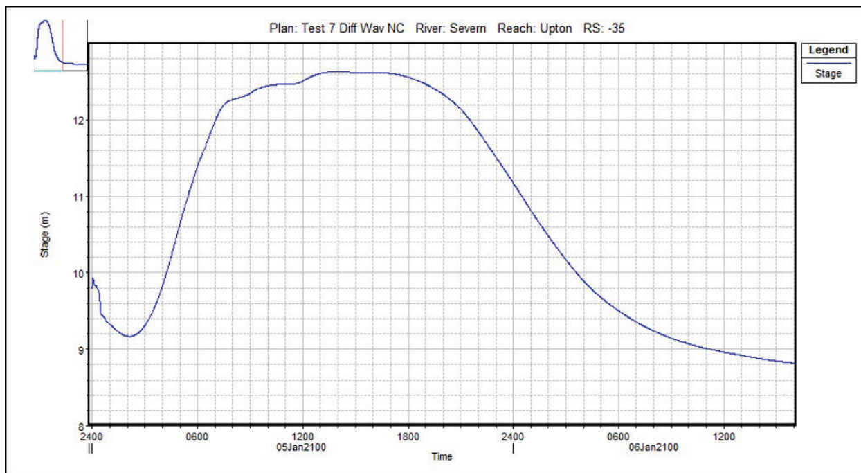
Figure 106. Test Point M035 - Water Level (depth).
