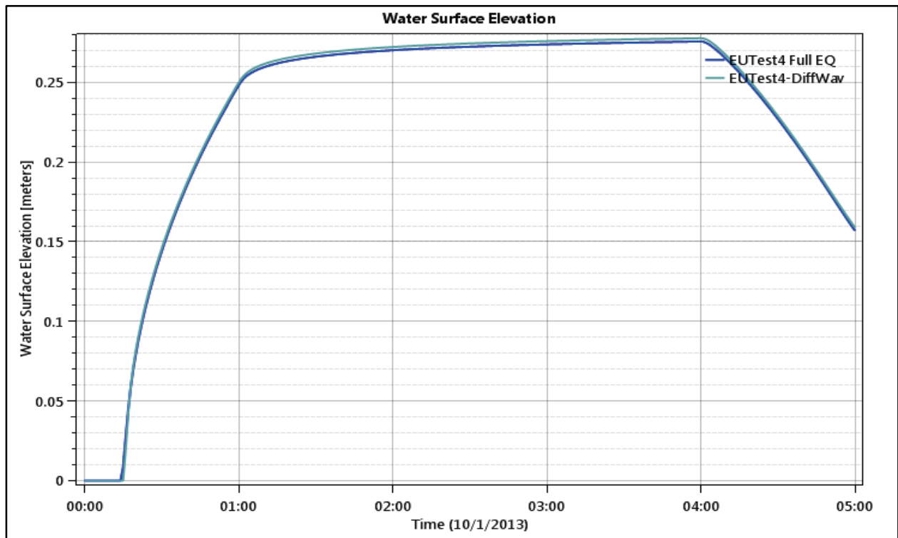
Figure 28. Test Point 2 Water Level (depth).
