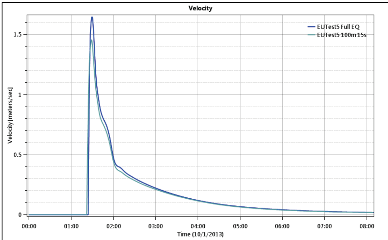
Figure 77. Test Point 4 - Velocity Time Series, 50 and 100 meter grids.
