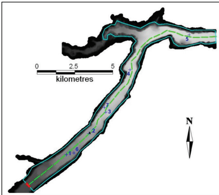
Figure 44. DEM used, with cross-section along the center line, and location of the output points. The red line indicates the location of the boundary condition and the blue polygon is the modeled area.
