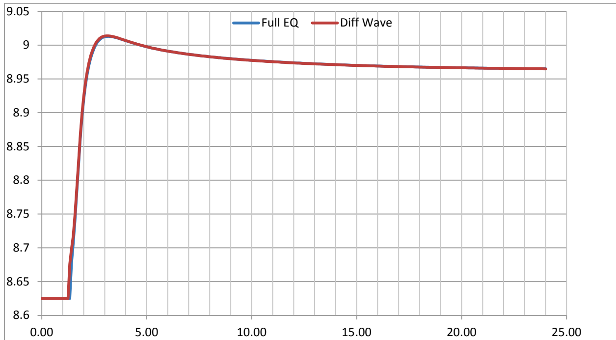
Figure 12. Test Point 7 - Water Level (m) versus Time (hrs).
