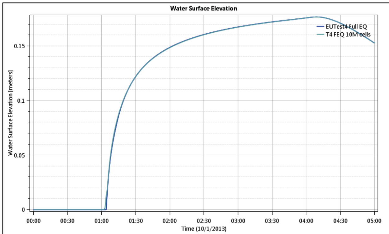
Figure 42. Test Point 6 - Water Surface versus Time - 5 and 10 Meter Grids.
