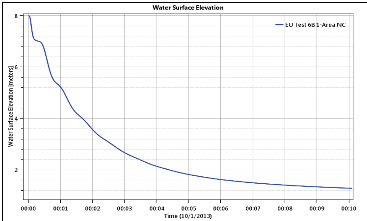
Figure 91. Test Point 6 - Water Level (depth).
