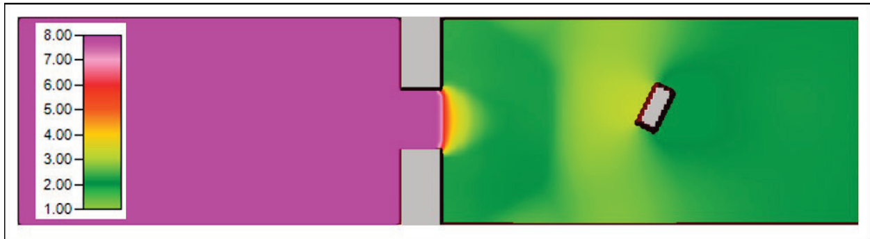
Figure 93. Maximum Water Surface Elevation (meters).
