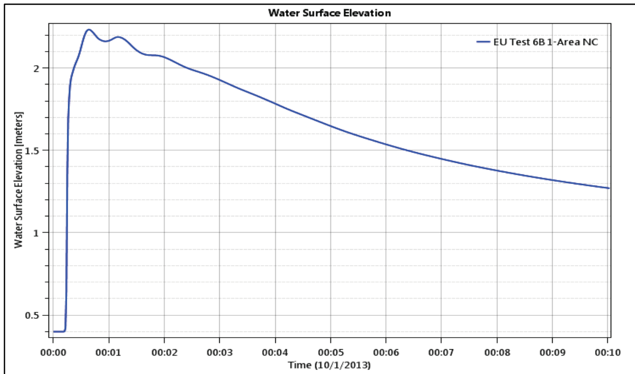
Figure 87. Test Point 4 - Water Level (depth).
