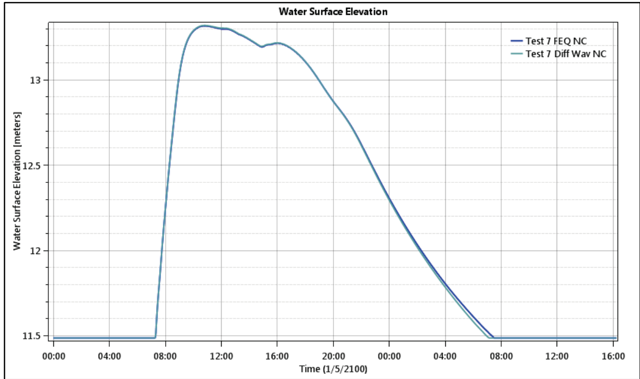
Figure 114. Floodplain 1 - Test Point 4 - Water Level.
