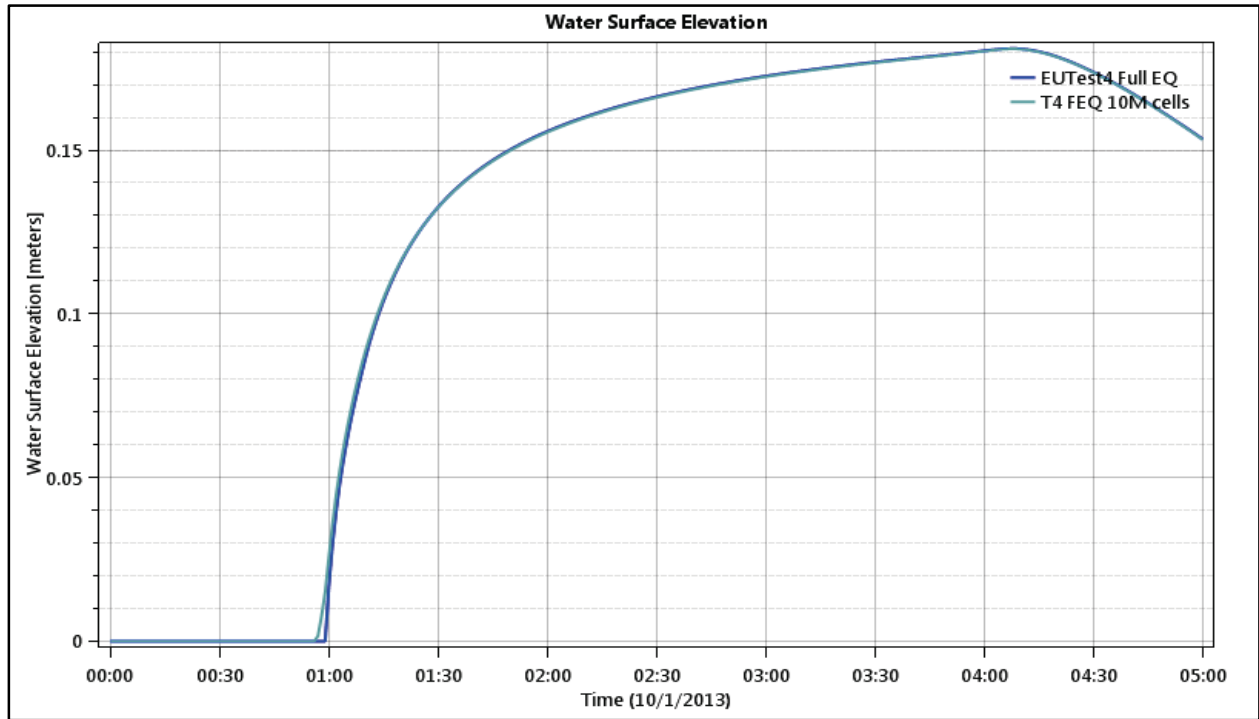
Figure 40. Test Point 5 - Water Surface versus Time - 5 and 10 Meter Grids.
