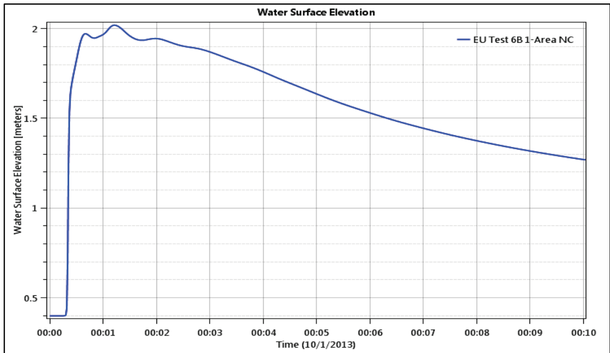
Figure 89. Test Point 5 - Water Level (depth).
