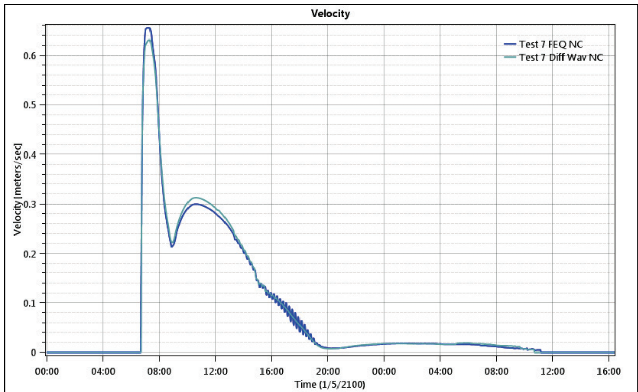
Figure 113. Floodplain 1 - Test Point 3 – Velocity.
