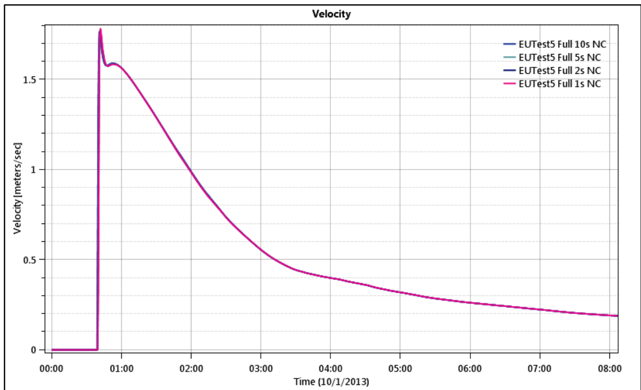
Figure 63. Test Point 2 - Velocity Time Series, \Delta T = 1, 2, 5, 10 seconds.
