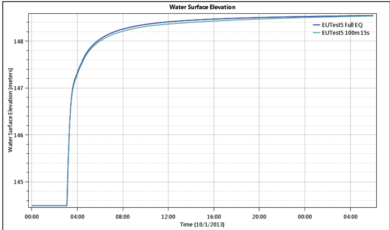
Figure 78. Test Point 5 - Water Level (depth), 50 and 100 meter grids.
