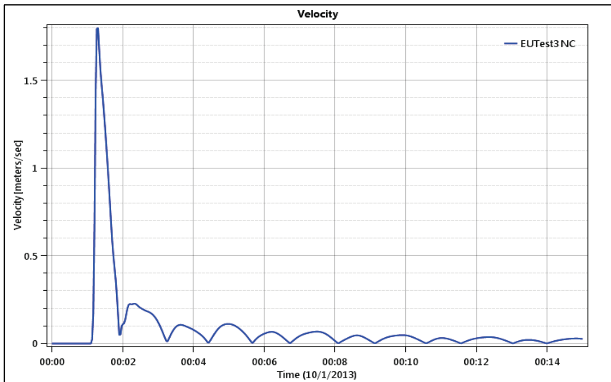
Figure 21. Test Point 1 - Velocity versus Time (minutes).
