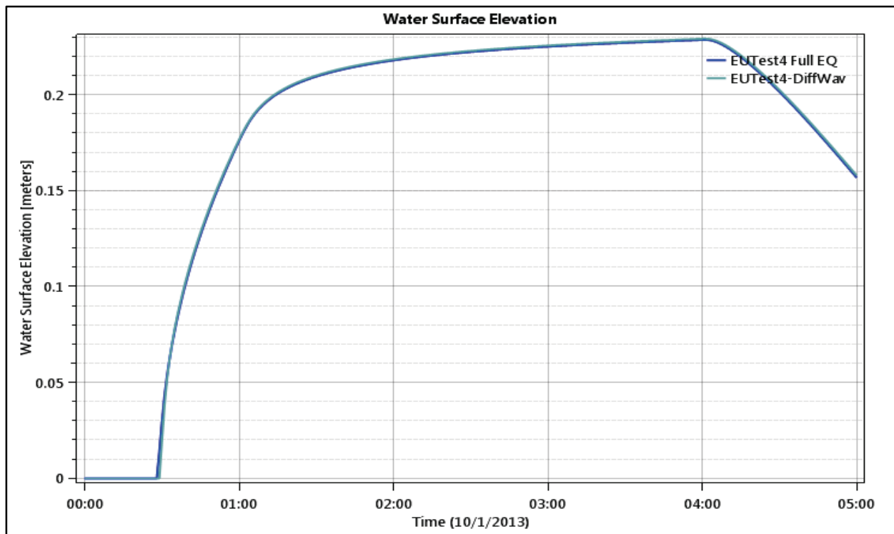
Figure 30. Test Point 3 Water Level (depth).
