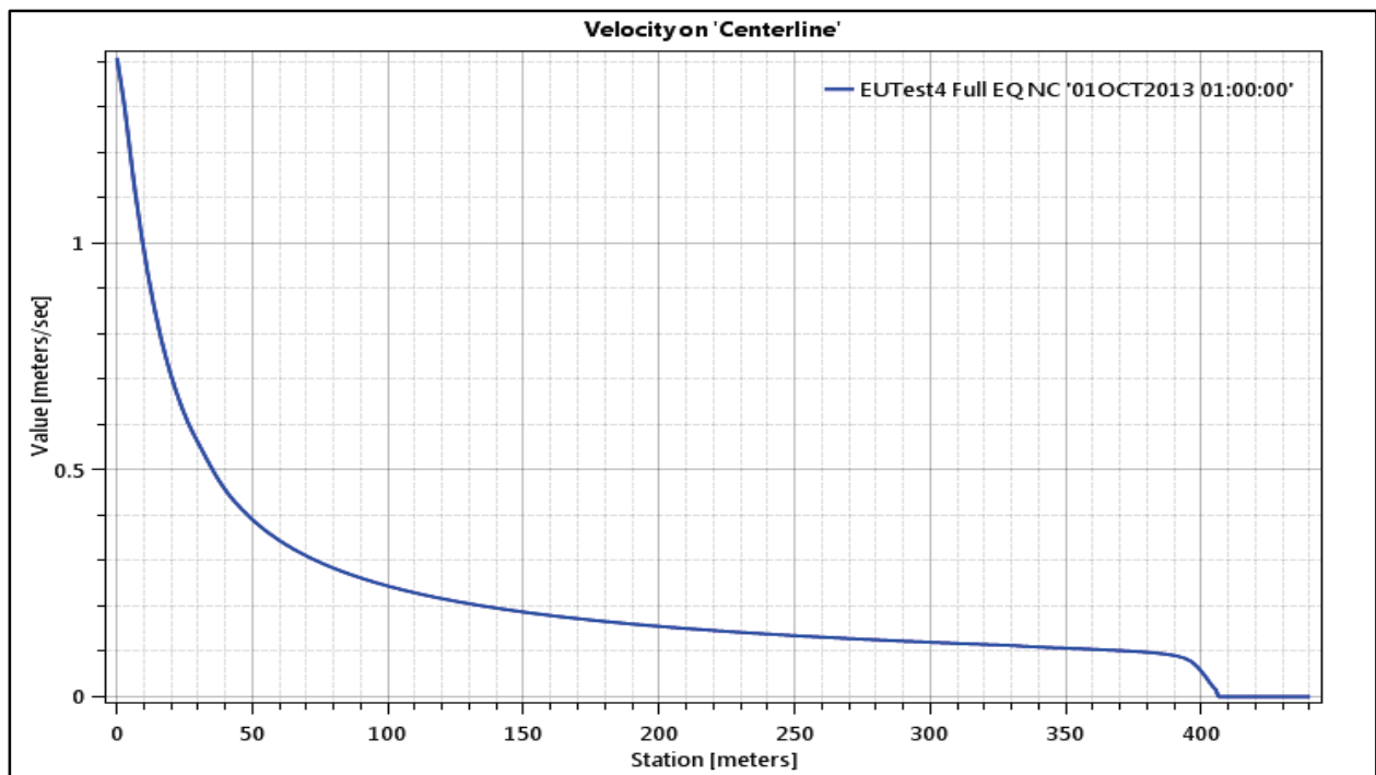
Figure 39. Velocity versus Distance at Time 1HOUR.
