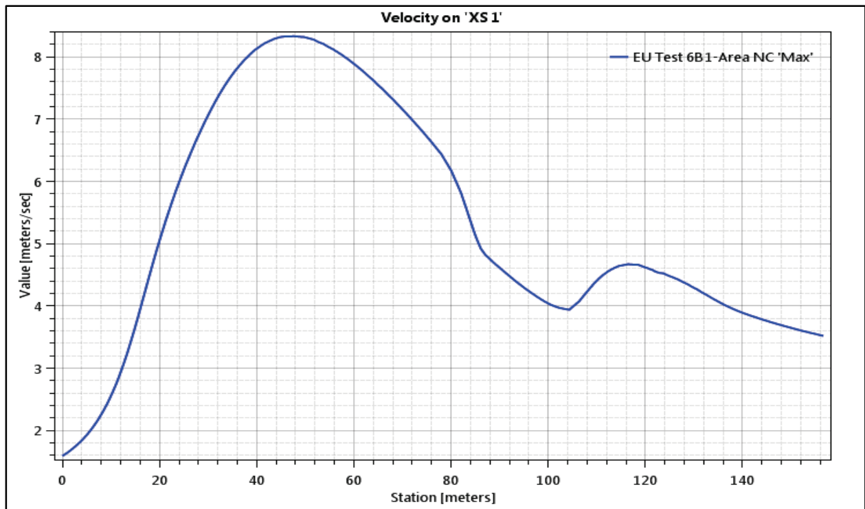
Figure 97. Maximum Velocity along Cross Section 1.
