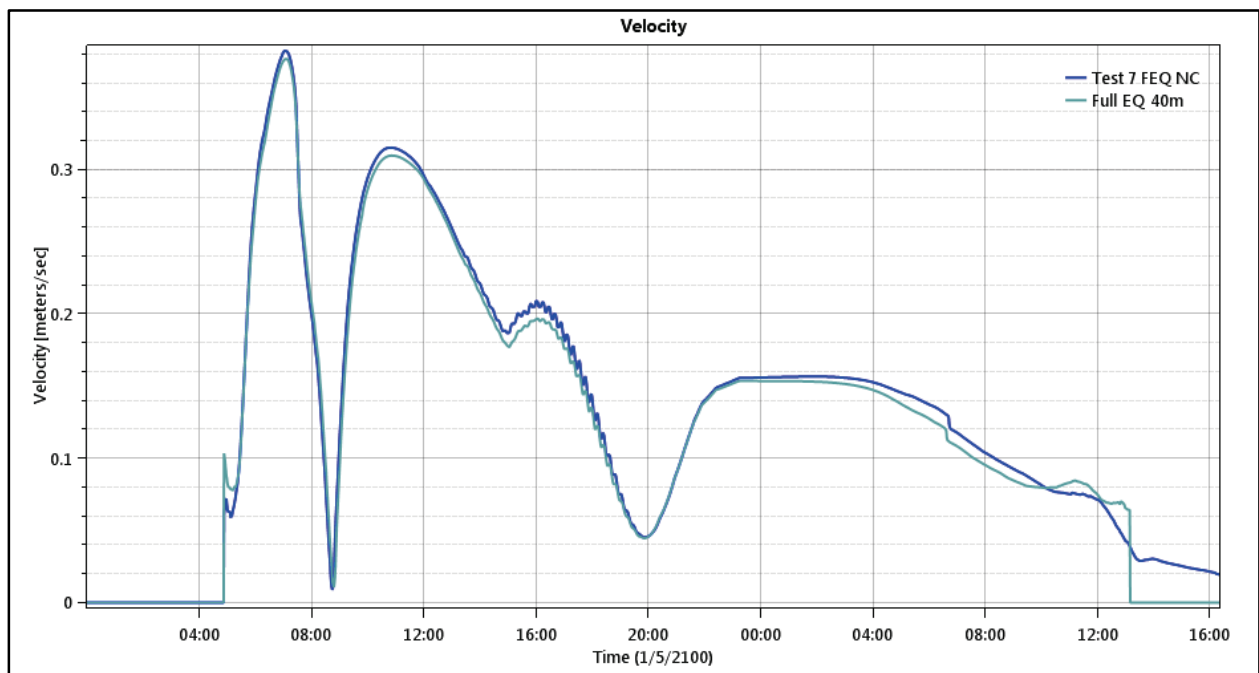
Figure 148. Floodplain 1 - Test Point 6 - Velocity.
