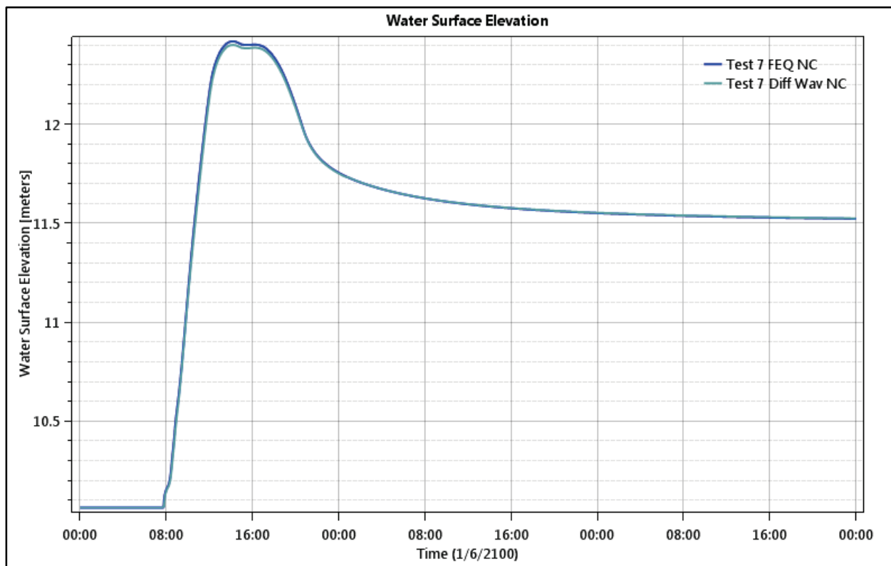
Figure 134. Floodplain 3 - Test Point 14 - Water Level.
