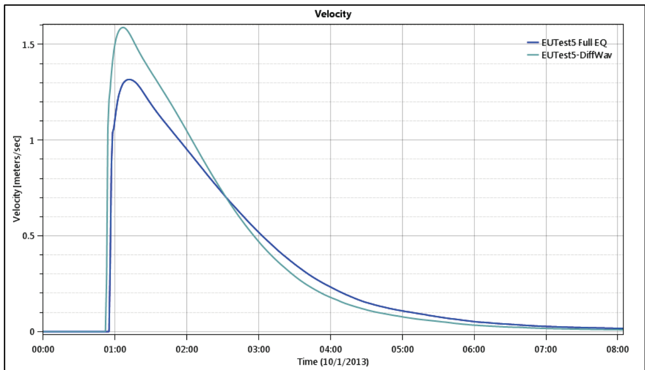
Figure 59. Test Point 7 - Velocity Time Series for Full Equations and Diffusion Wave.
