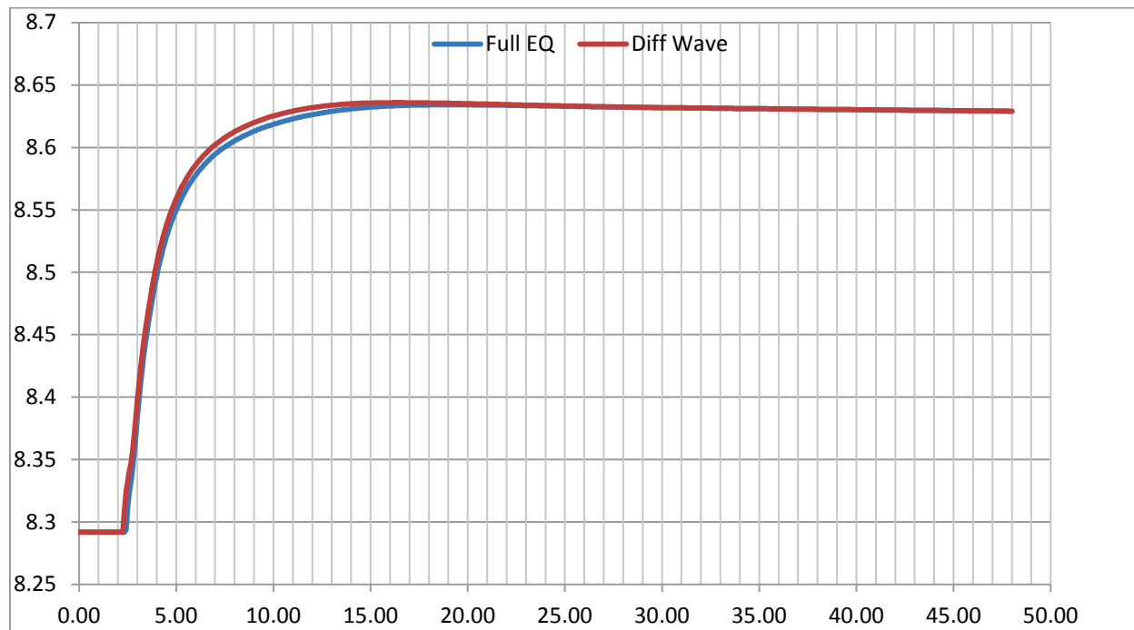
Figure 13. Test Point 6 - Water Level (m) versus Time (hrs).
