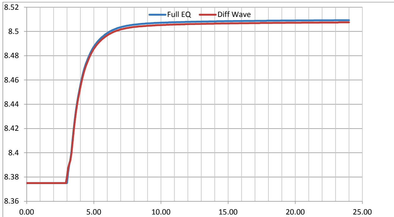
Figure 16. Test Point 11 - Water Level (m) versus Time (hrs).
