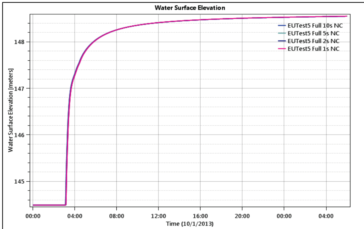
Figure 68. Test Point 5 - Water Level (depth), \Delta T = 1, 2, 5, 10 seconds.
