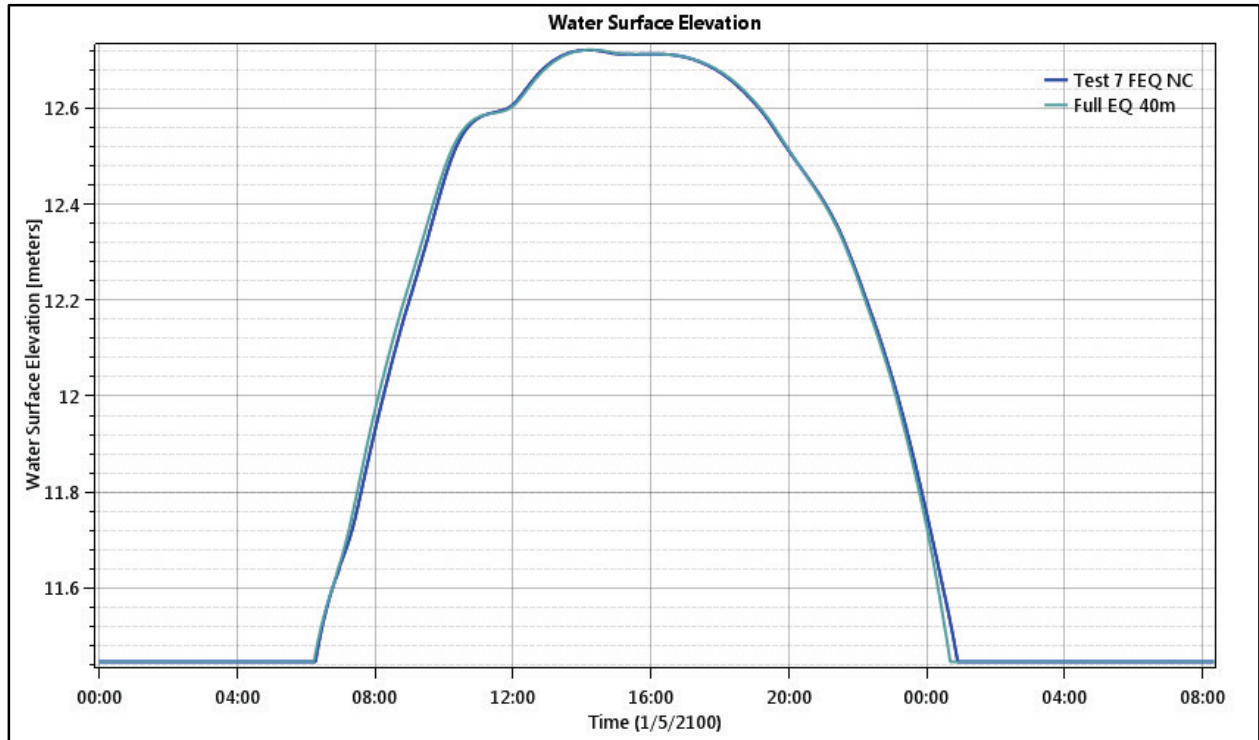
Figure 153. Floodplain 3 - Test Point 10 - Water Level.
