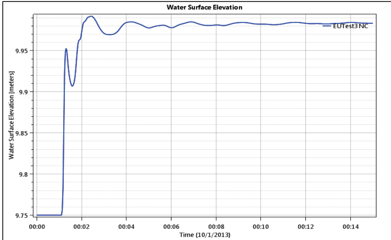
Figure 20. Test Point 1 - Water Level versus Time (minutes).
