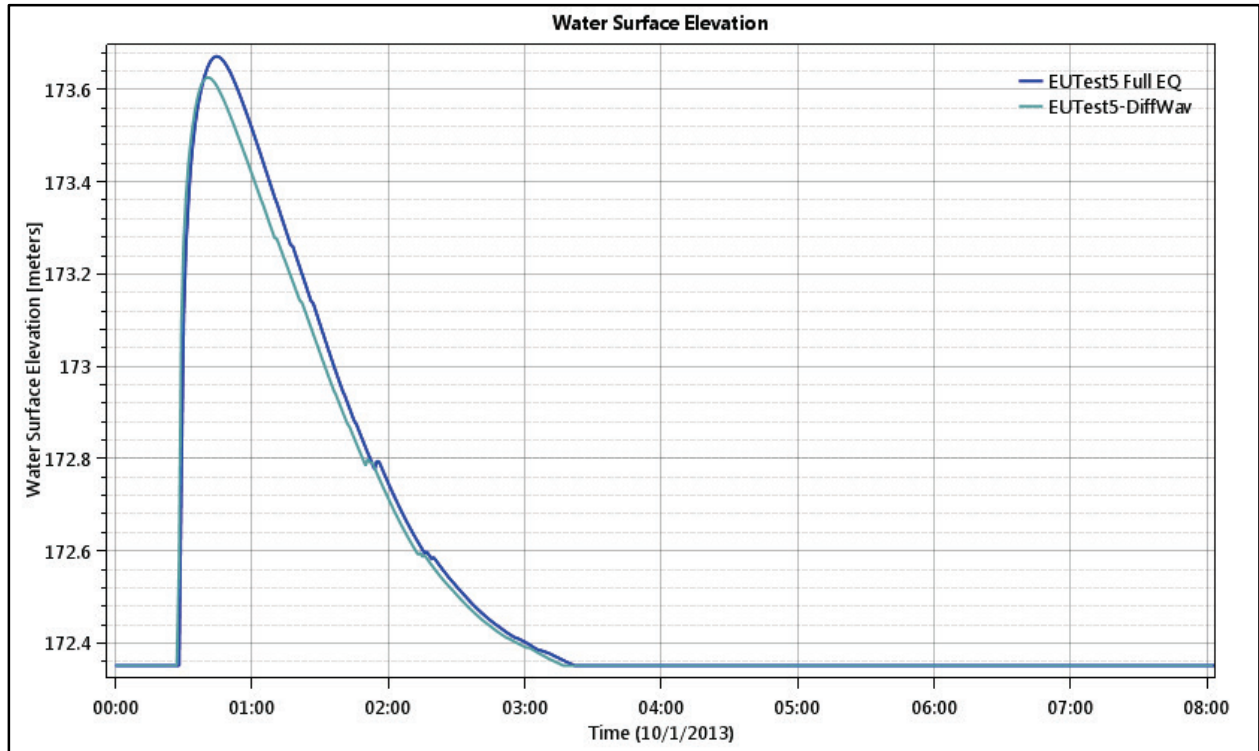
Figure 56. Test Point 6 - Water Level (depth) for Full Equations and Diffusion Wave.
