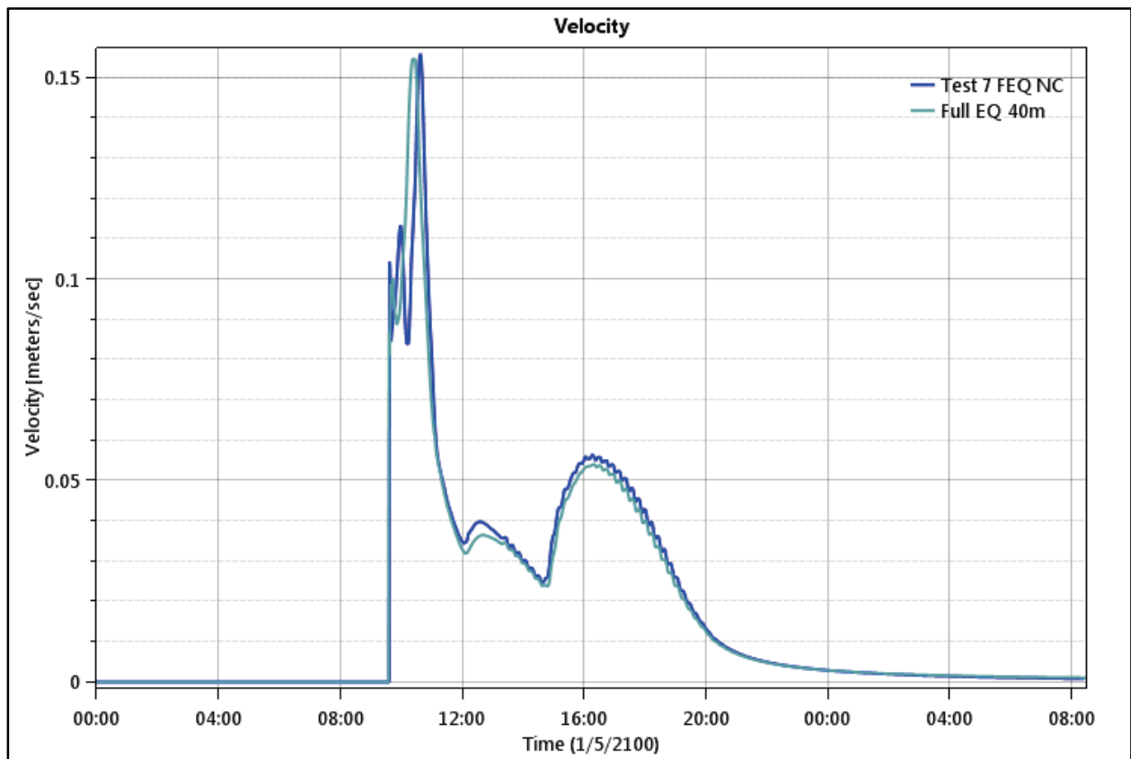
Figure 152. Floodplain 2 - Test Point 8 - Velocity.
