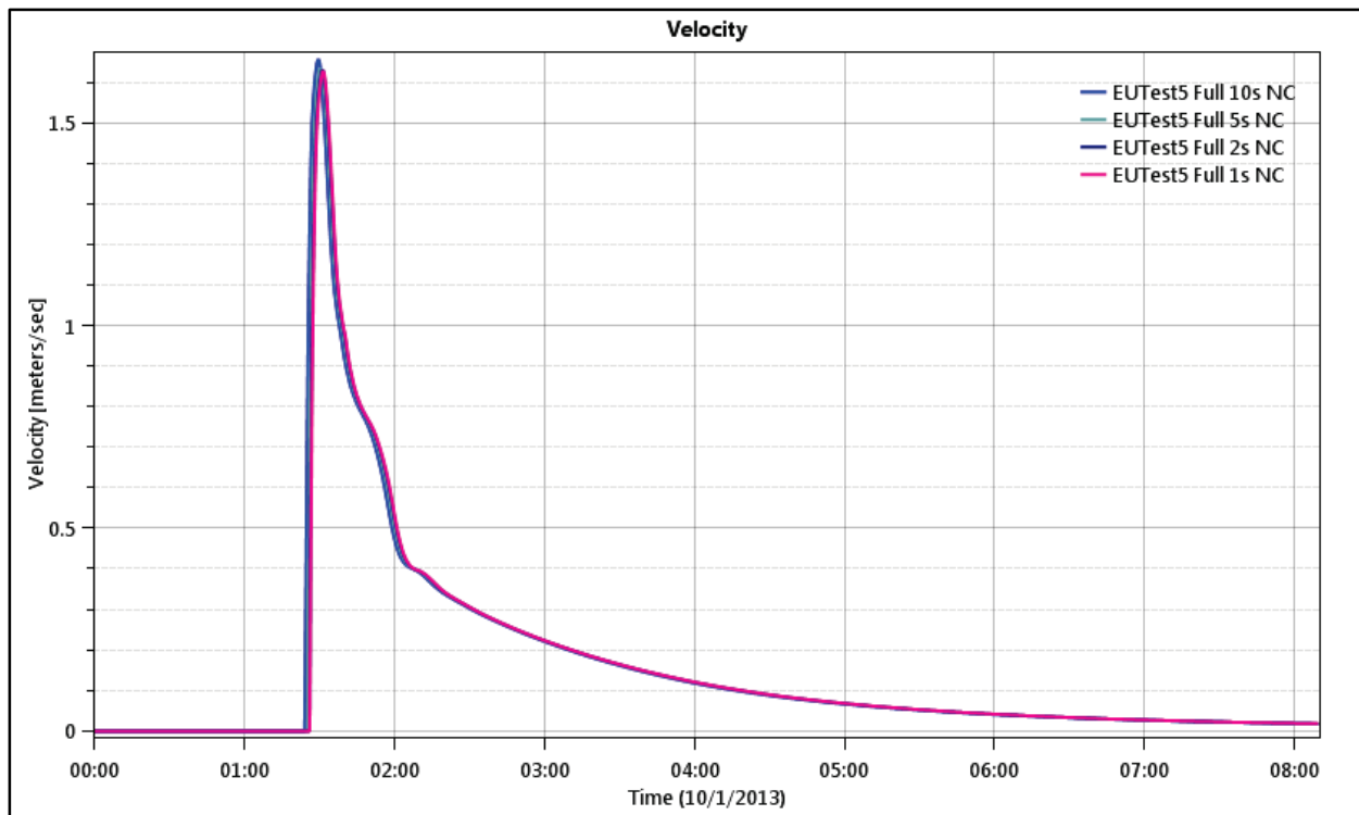
Figure 67. Test Point 4 - Velocity Time Series, \Delta T = 1, 2, 5, 10 seconds.
