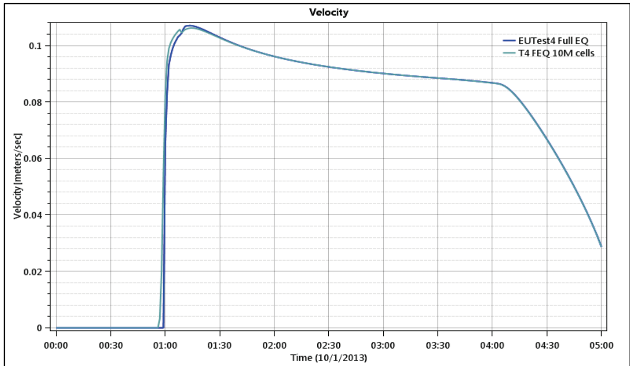
Figure 41. Test Point 5 - Velocity versus Time - 5 and 10 Meter Grids.
