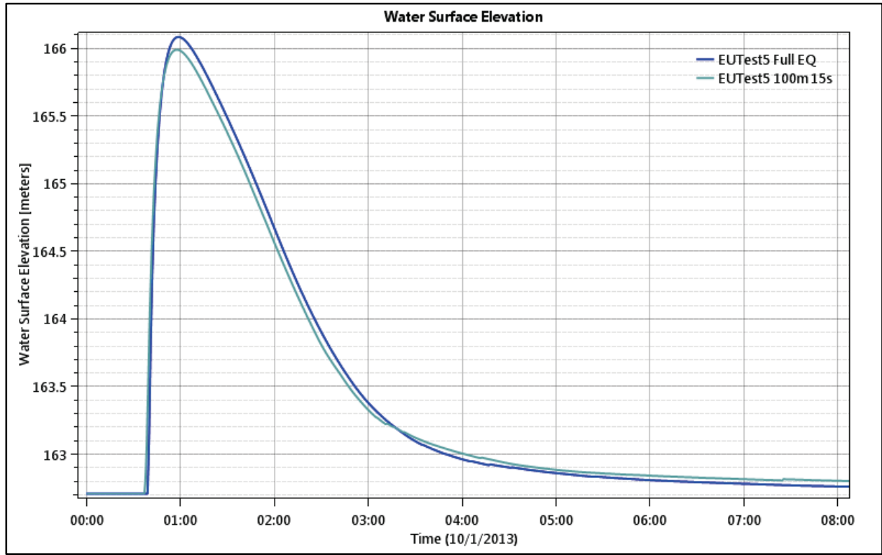
Figure 72. Test Point 2 - Water Level (depth), 50 and 100 meter grids.
