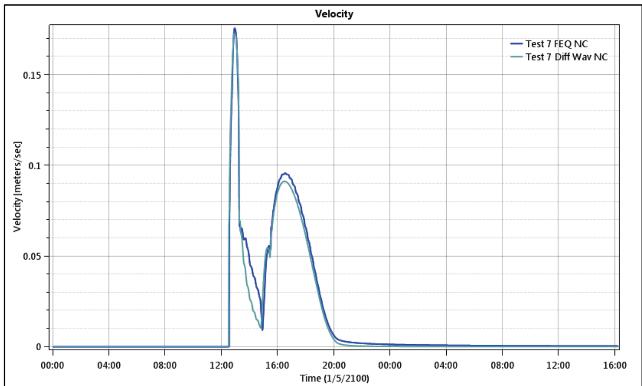
Figure 125. Floodplain 2 - Test Point 9 - Velocity.
