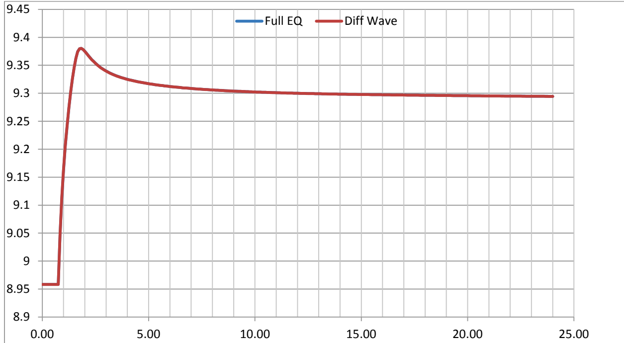
Figure 11. Test Point 8 - Water Level (m) versus Time (hrs).
