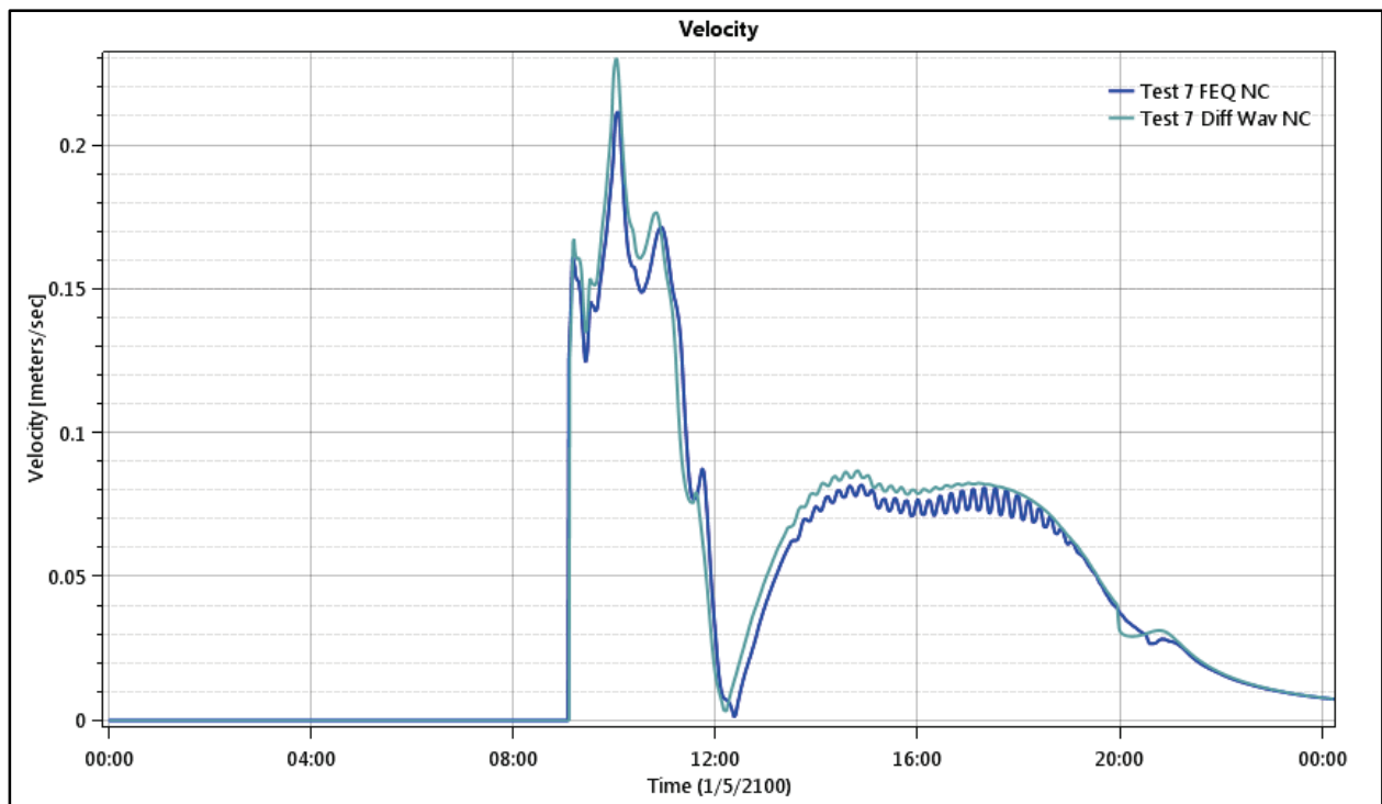
Figure 133. Floodplain 3 - Test Point 13 - Velocity.
