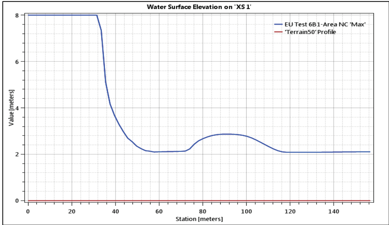
Figure 96. Maximum Water Surface Elevation along Cross Section 1.
