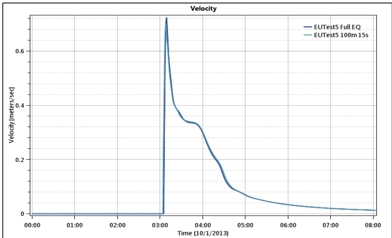
Figure 79. Test Point 4 - Velocity Time Series, 50 and 100 meter grids.
