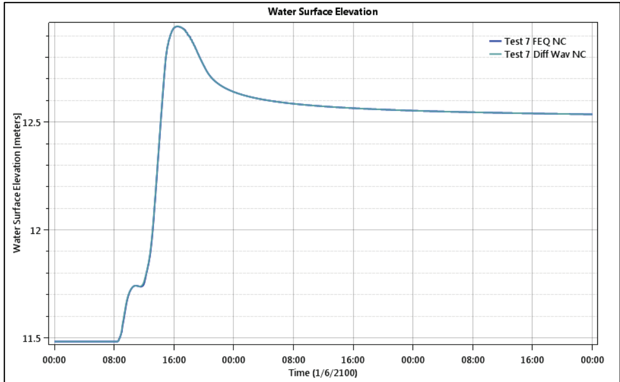
Figure 120. Floodplain 2 - Test Point 7 - Water Level.
