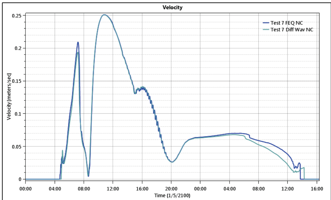
Figure 117. Floodplain 1 - Test Point 5 - Velocity.
