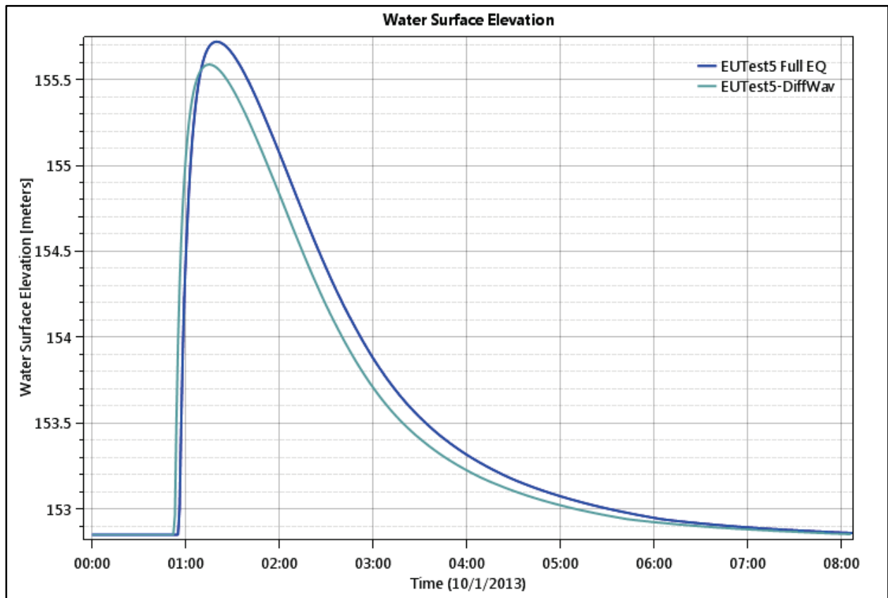
Figure 58. Test Point 7 - Water Level (depth) for Full Equations and Diffusion Wave.
