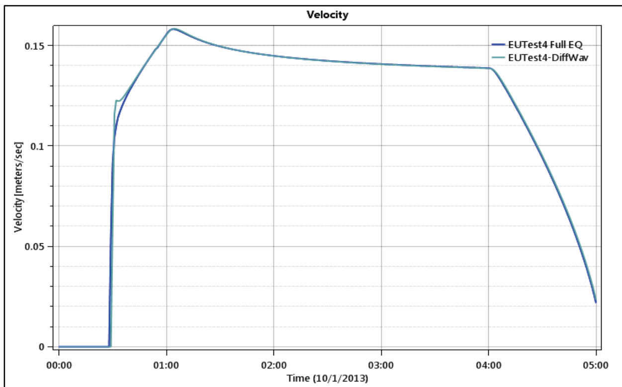
Figure 31. Test Point 3 Velocity Time Series.
