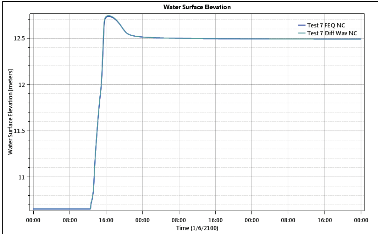
Figure 124. Floodplain 2 - Test Point 9 - Water Level.
