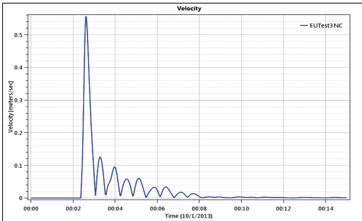
Figure 23. Test Point 2 - Velocity versus Time (minutes).
