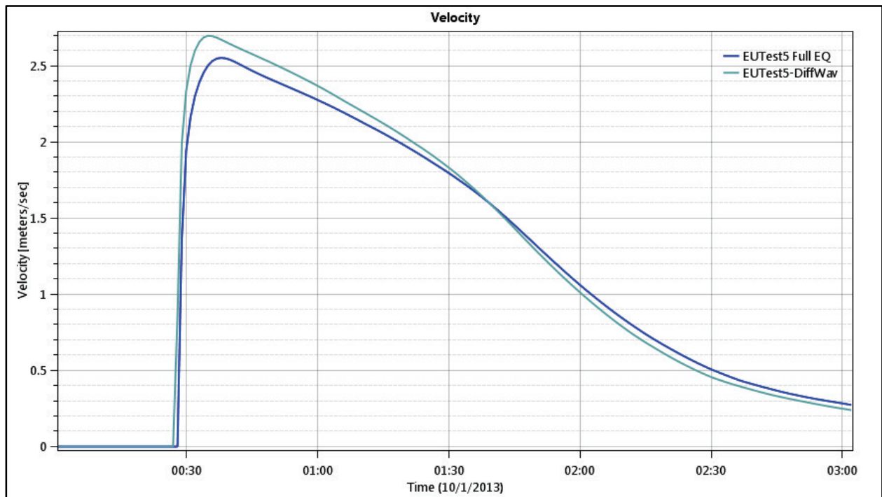
Figure 57. Test Point 6 - Velocity Time Series for Full Equations and Diffusion Wave.
