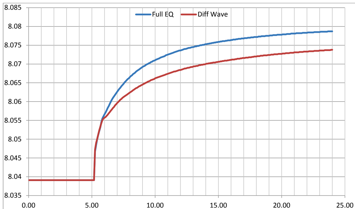
Figure 17. Test Point 10 - Water Level (m) versus Time (hrs).
