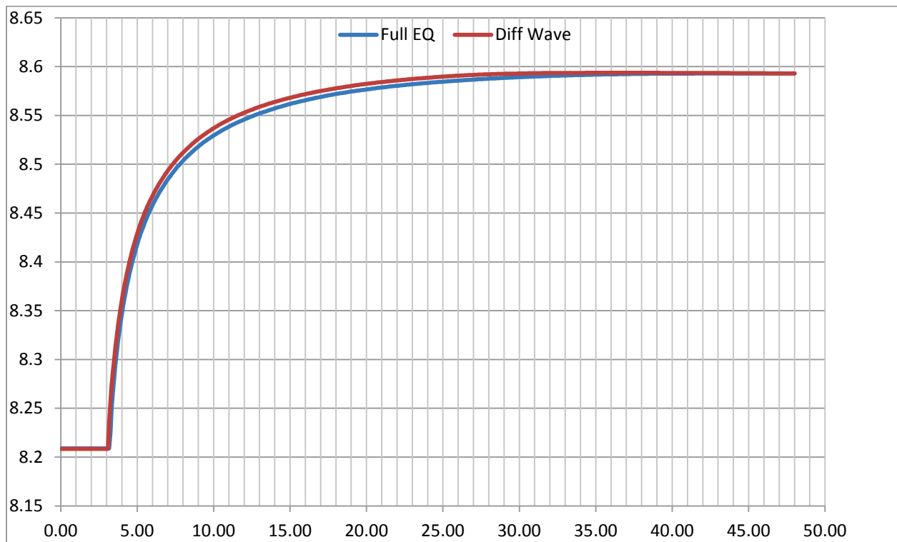
Figure 10. Test Point 1 - Water Level (m) versus Time (hrs).
