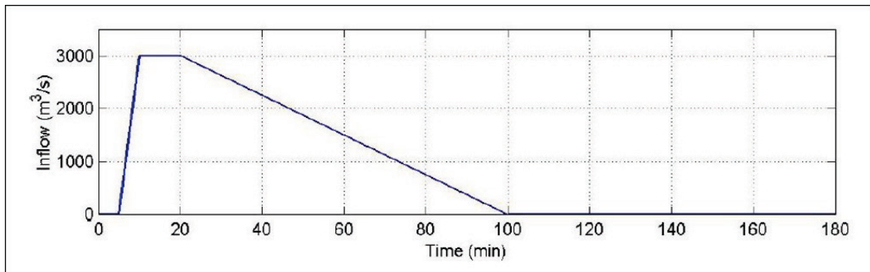
Figure 45. Inflow Hydrograph.
