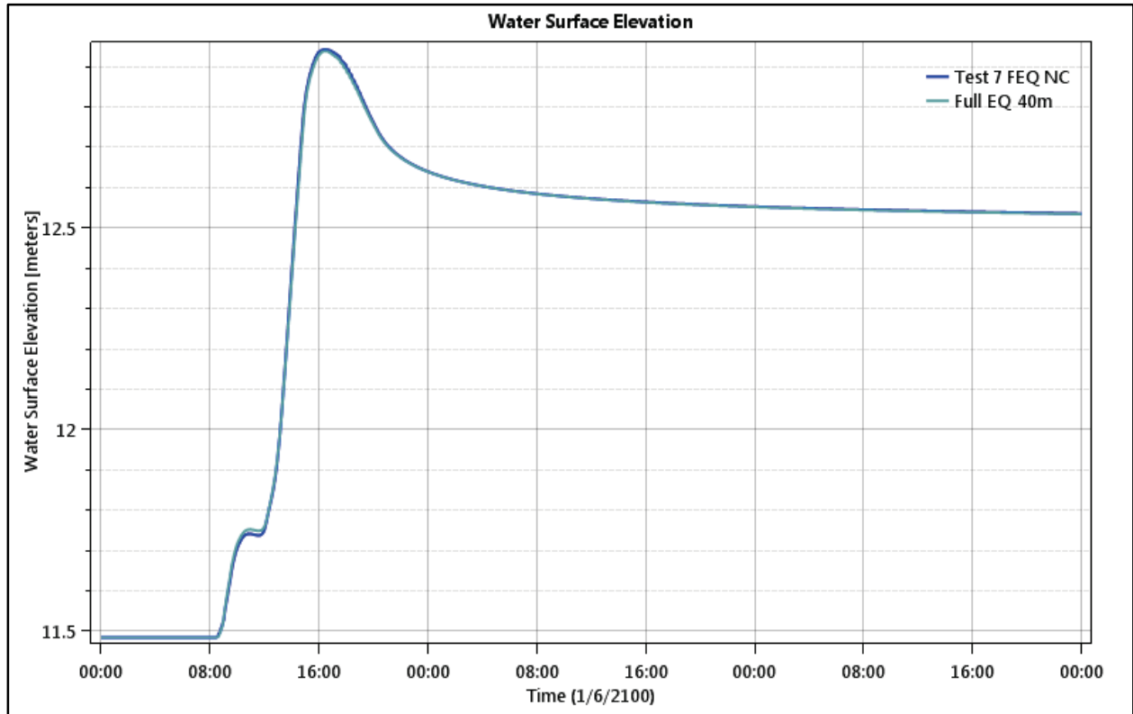
Figure 149. Floodplain 2 - Test Point 7 - Water Level.
