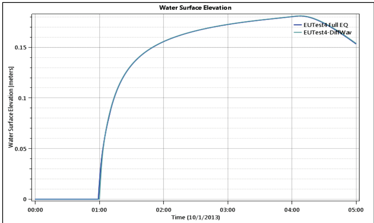
Figure 34. Test Point 5 Water Level (depth).
