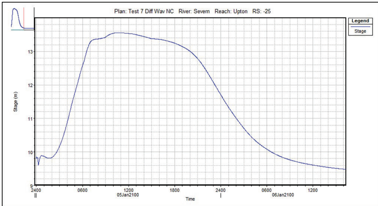
Figure 105. Test Point M025 - Water Level (depth).
