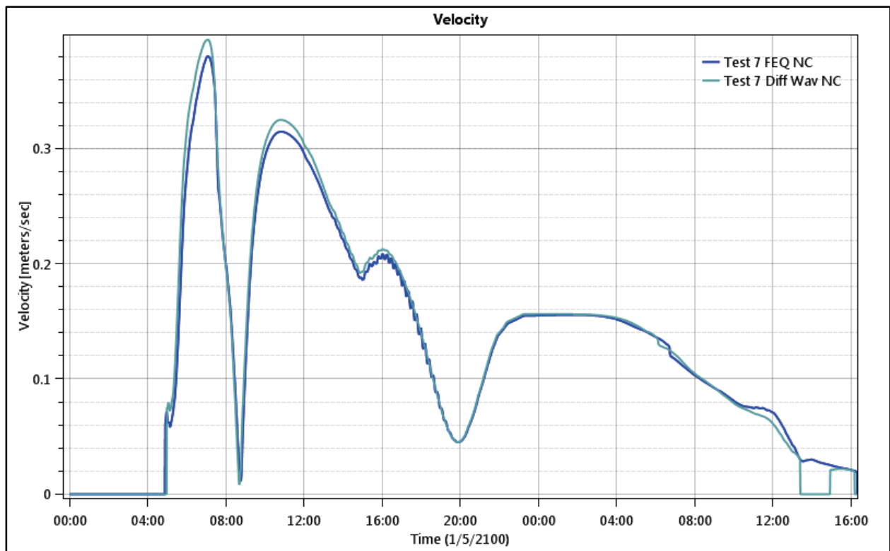
Figure 119. Floodplain 1 - Test Point 6 - Velocity.
