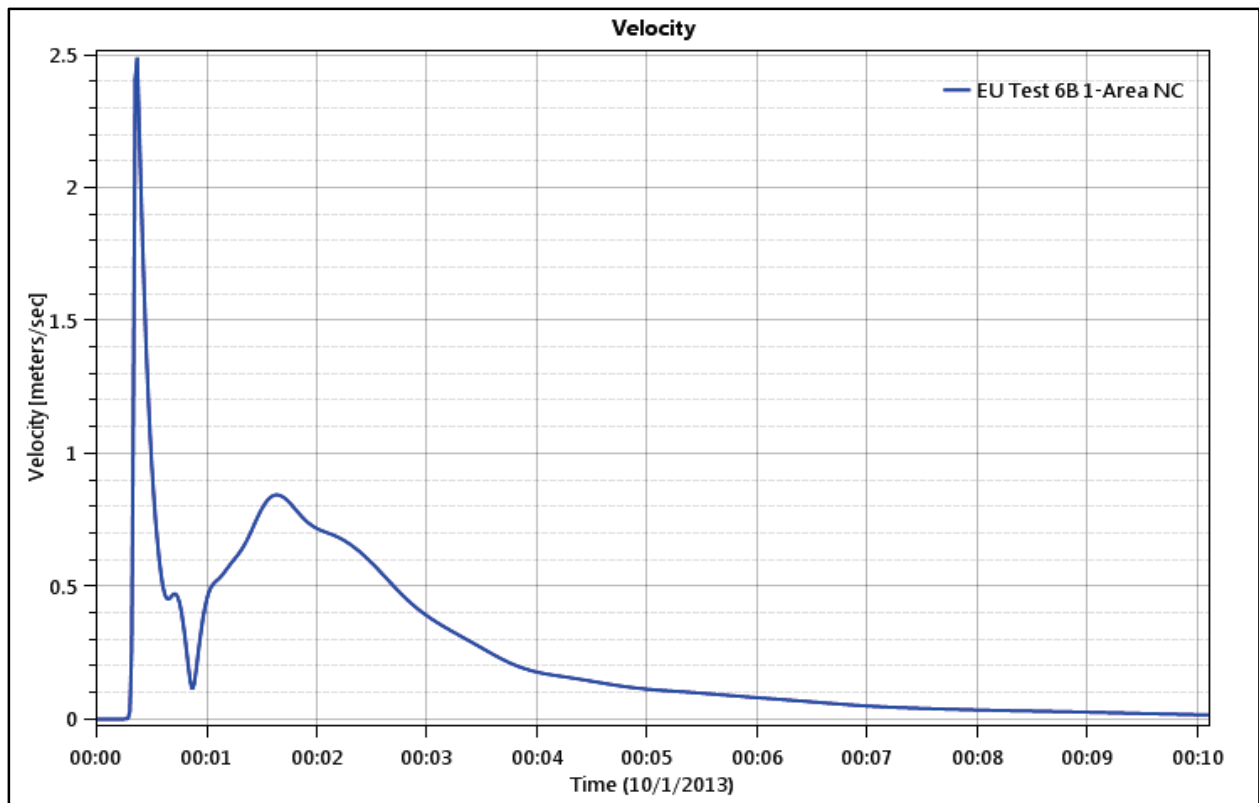
Figure 90. Test Point 5 - Velocity Time Series.
