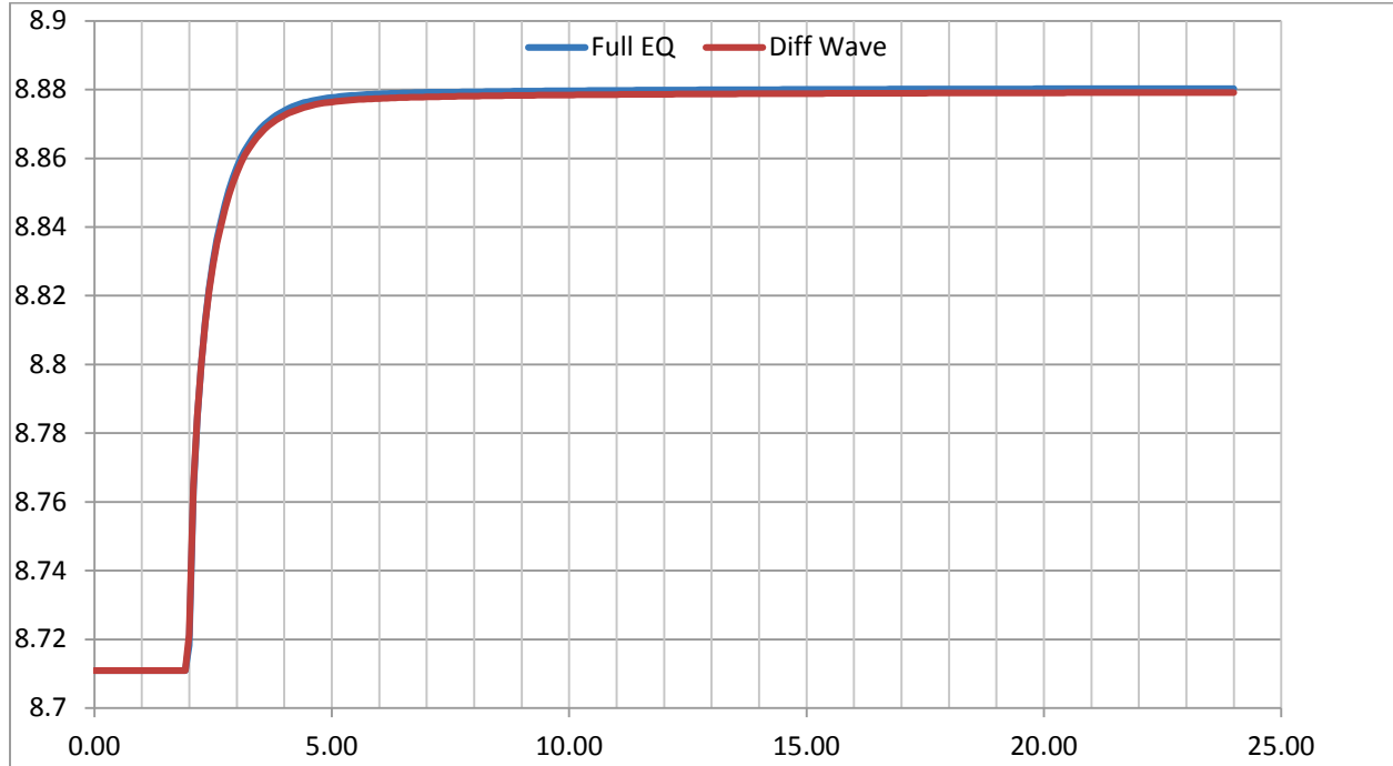
Figure 15. Test Point 12 - Water Level (m) versus Time (hrs).
