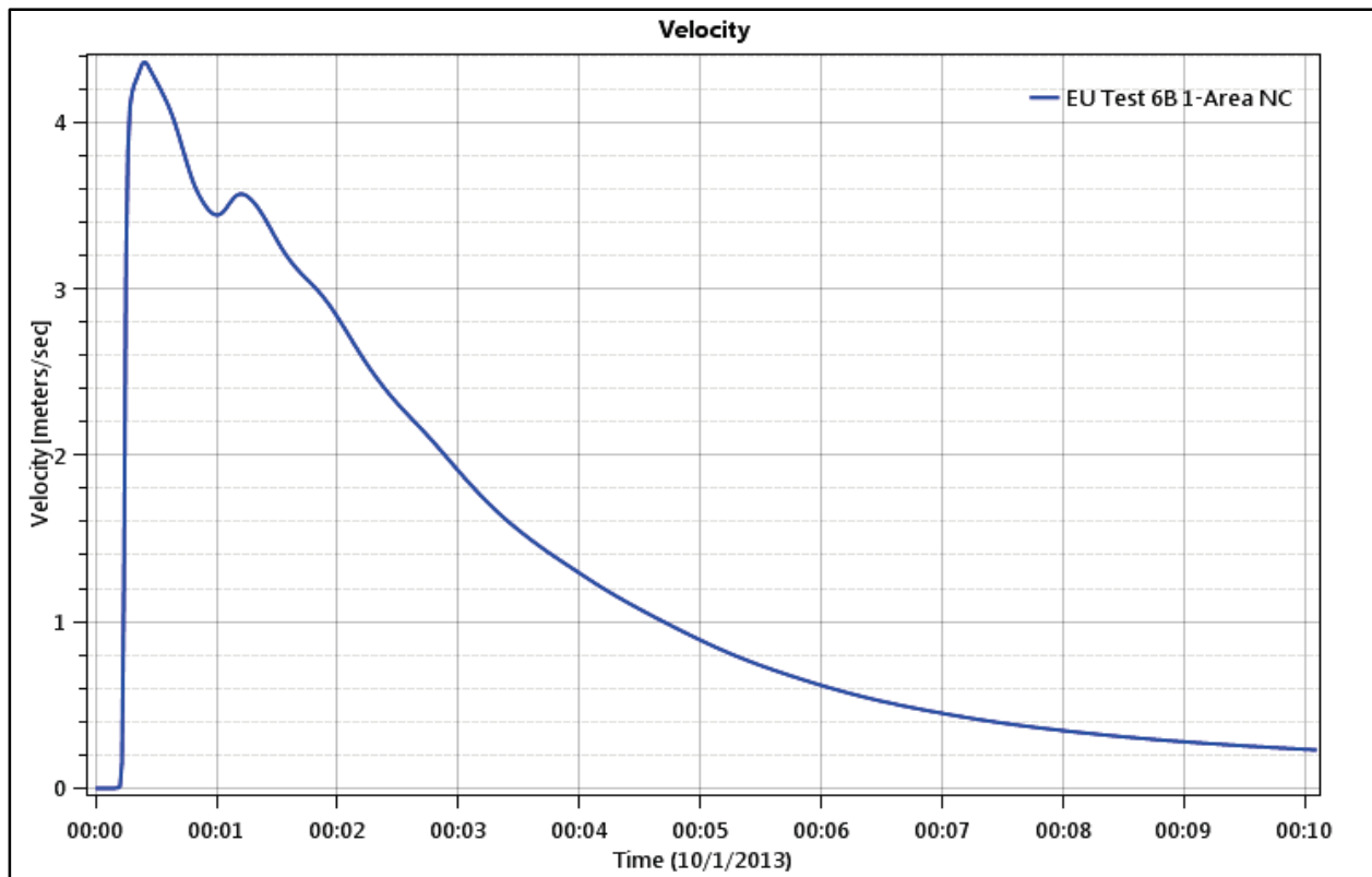
Figure 88. Test Point 4 - Velocity Time Series.
