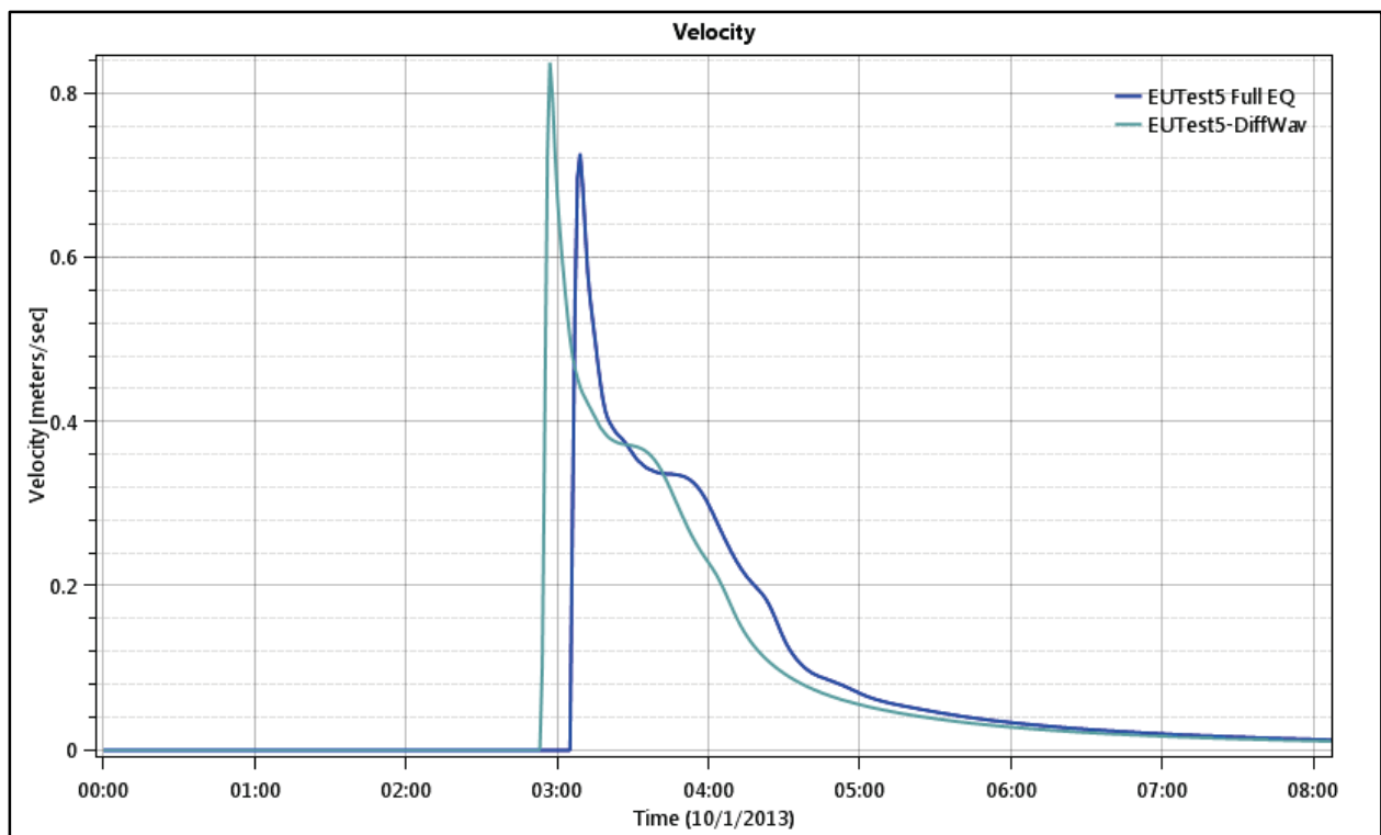
Figure 55. Test Point 5 - Velocity Time Series for Full Equations and Diffusion Wave.
