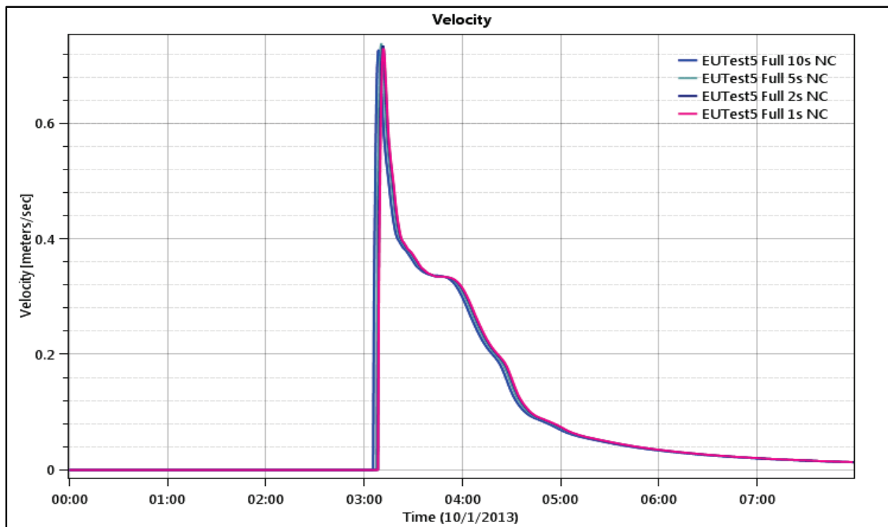
Figure 69. Test Point 5 - Velocity Time Series, \Delta T = 1, 2, 5, 10 seconds.
