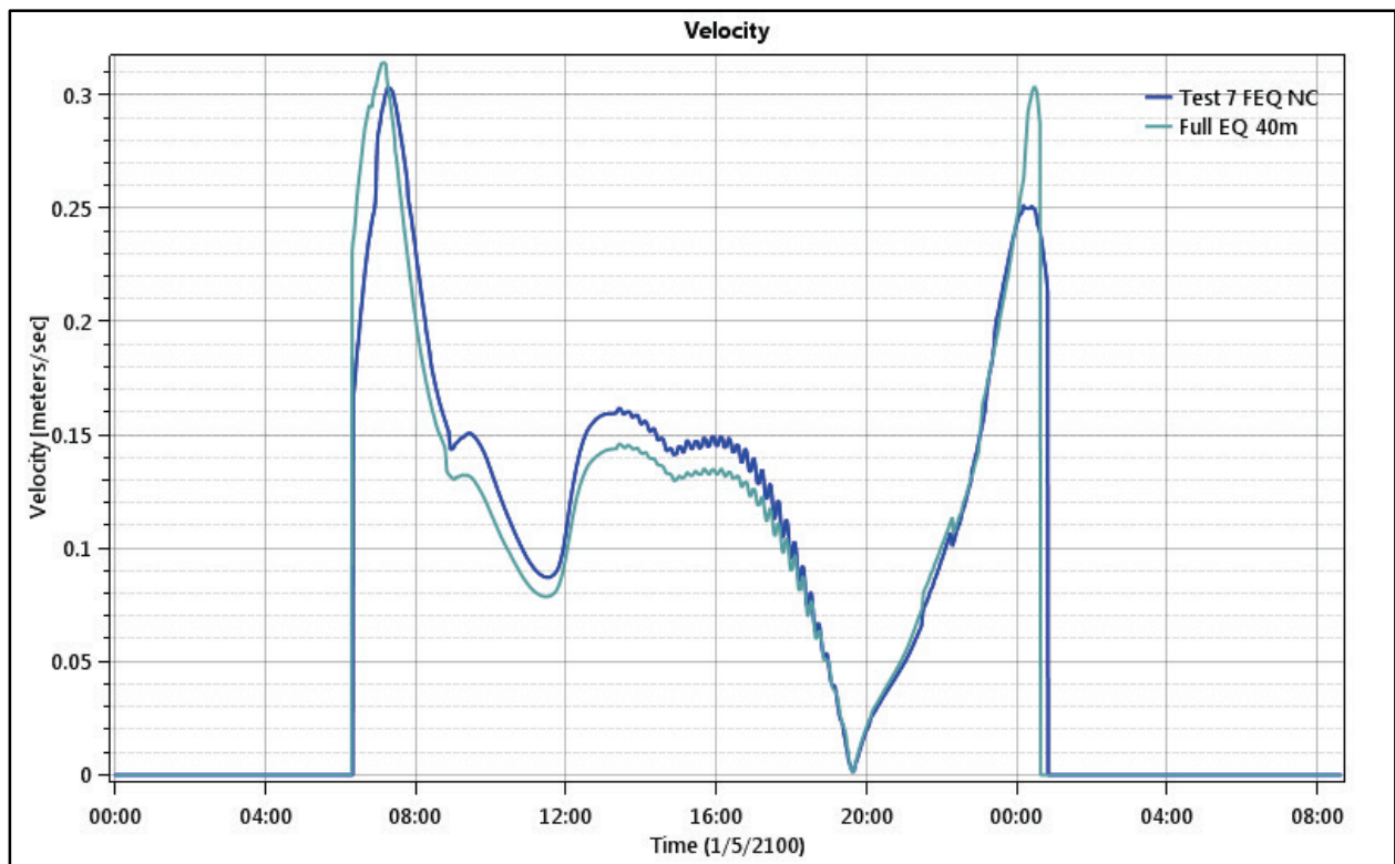
Figure 154. Floodplain 3 - Test Point 10 - Velocity.
