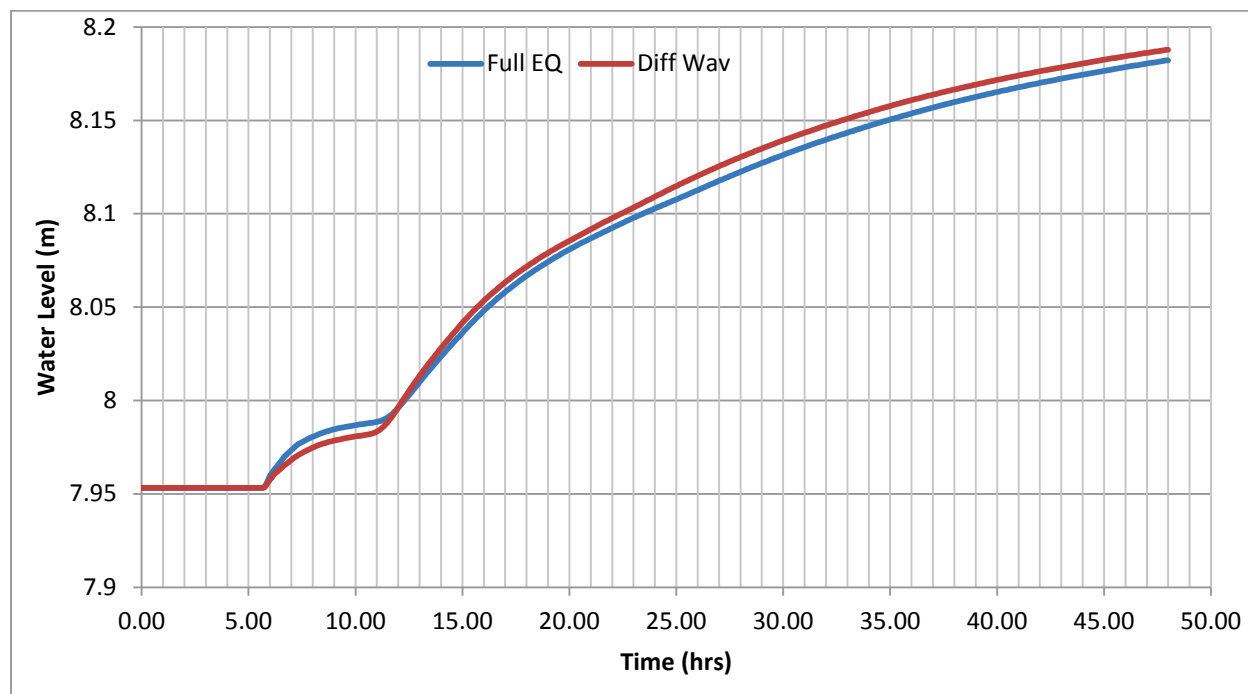
Figure 14. Test Point 5 - Water Level (m) versus Time (hrs).
