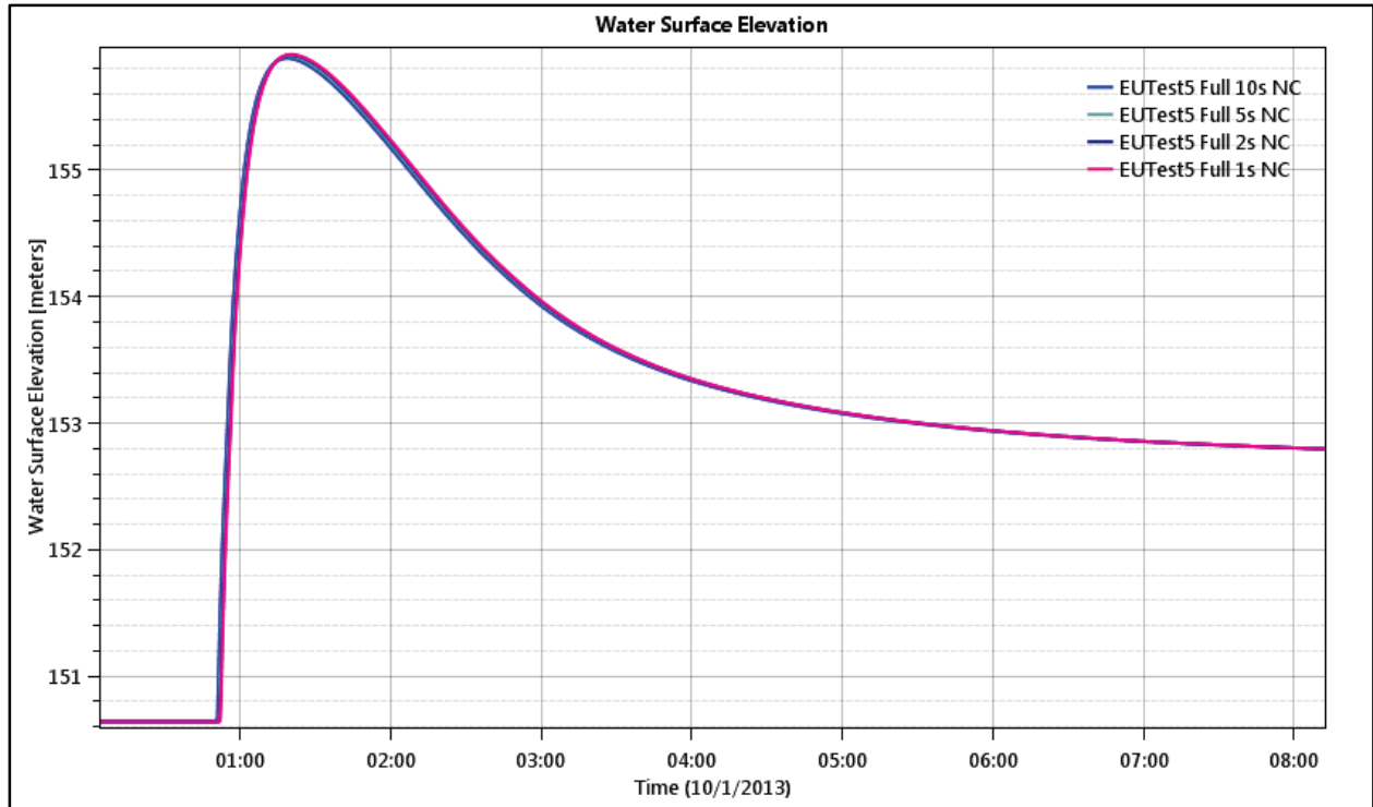
Figure 64. Test Point 3 - Water Level (depth), \Delta T = 1, 2, 5, 10 seconds.
