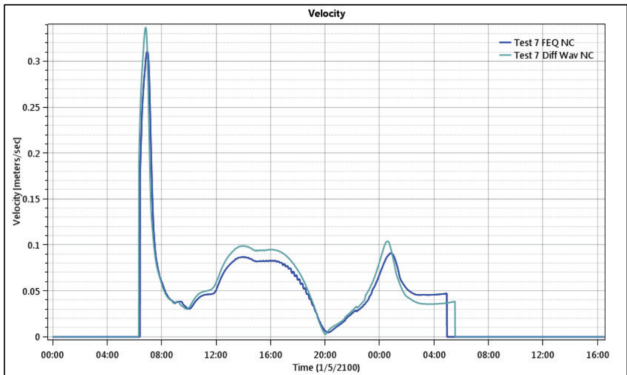
Figure 129. Floodplain 3 - Test Point 11 - Velocity.
