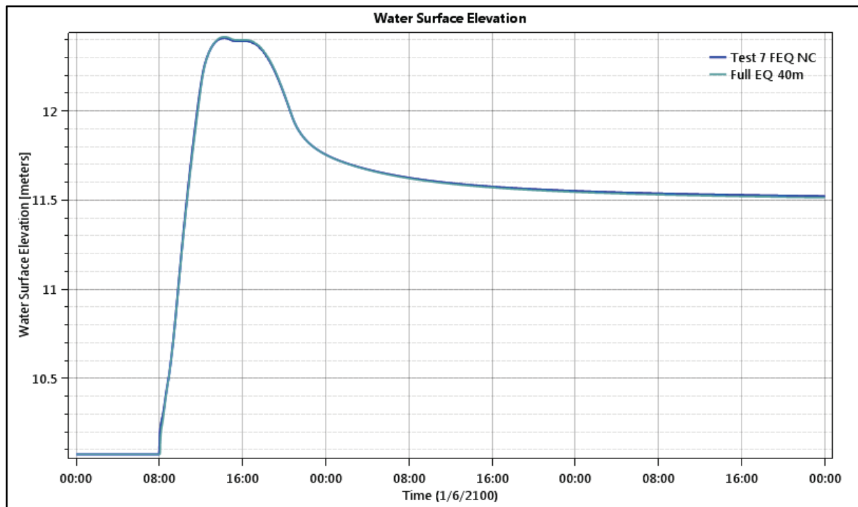
Figure 155. Floodplain 3 - Test Point 15 - Water Level.
