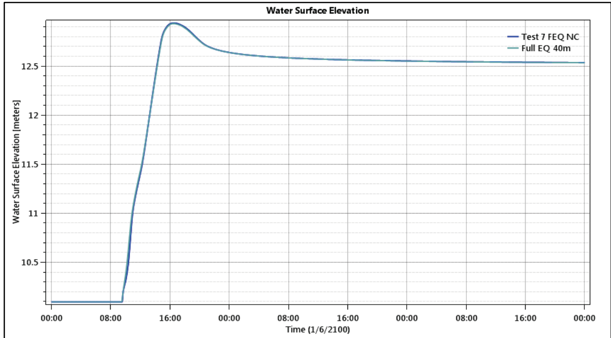
Figure 151. Floodplain 2 - Test Point 8 - Water Level.
