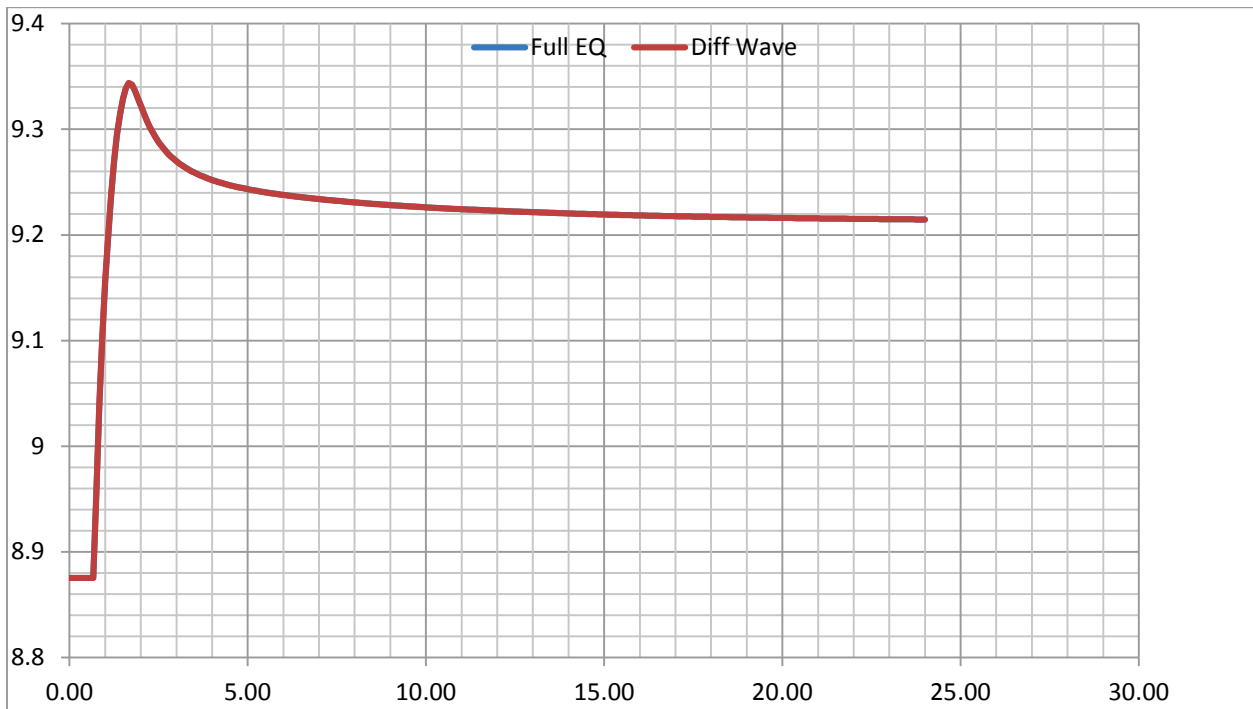
Figure 8. Test Point 3 - Water Level (m) versus Time (hrs).
