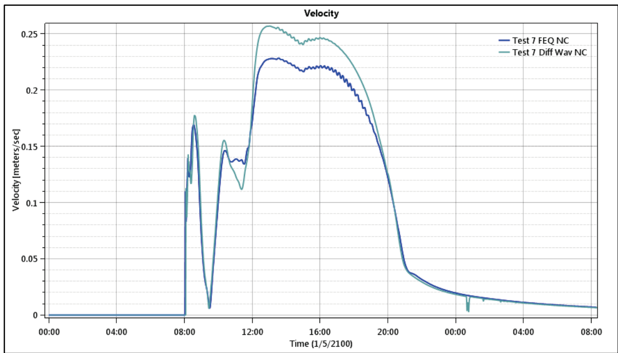
Figure 141. Floodplain 3 - Test Point 17 - Velocity.
