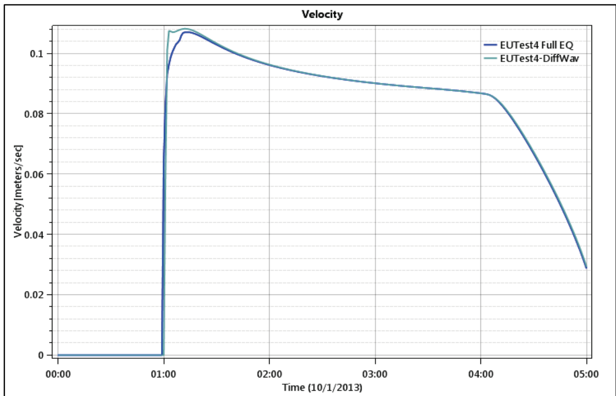
Figure 35. Test Point 5 Velocity Time Series.
