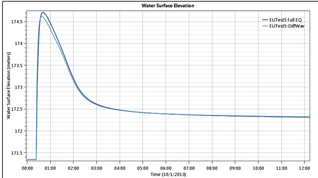
Figure 46. Test Point 1 - Water Level (depth) for Full Equations and Diffusion Wave.
