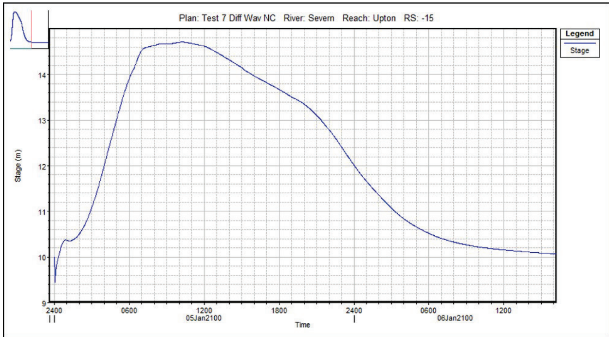
Figure 104. Test Point M015 - Water Level (depth).
