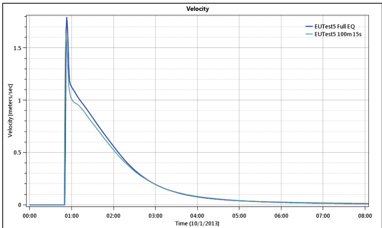
Figure 75. Test Point 3 - Velocity Time Series, 50 and 100 meter grids.
