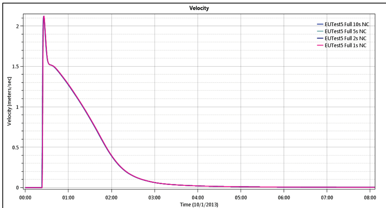
Figure 61. Test Point 1 - Velocity Time Series, \Delta T = 1, 2, 5, 10 seconds.
