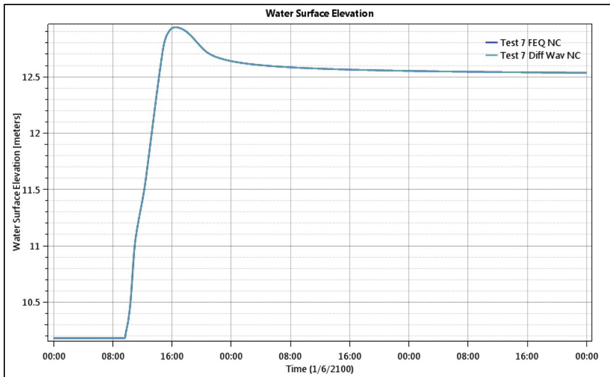
Figure 122. Floodplain 2 - Test Point 8 - Water Level.
