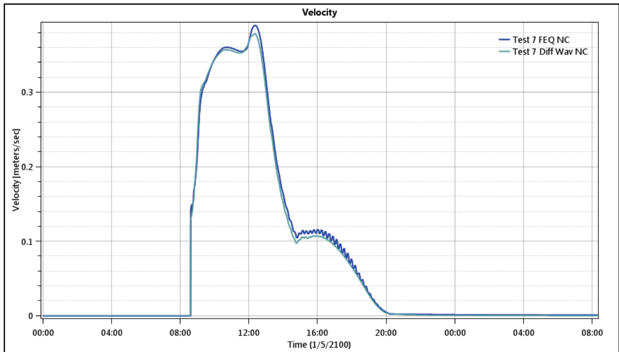
Figure 121. Floodplain 2 - Test Point 7 - Velocity.
