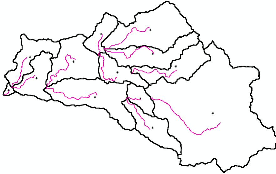
Figure 13-40. Centroidal Longest Flowpath Layer.
