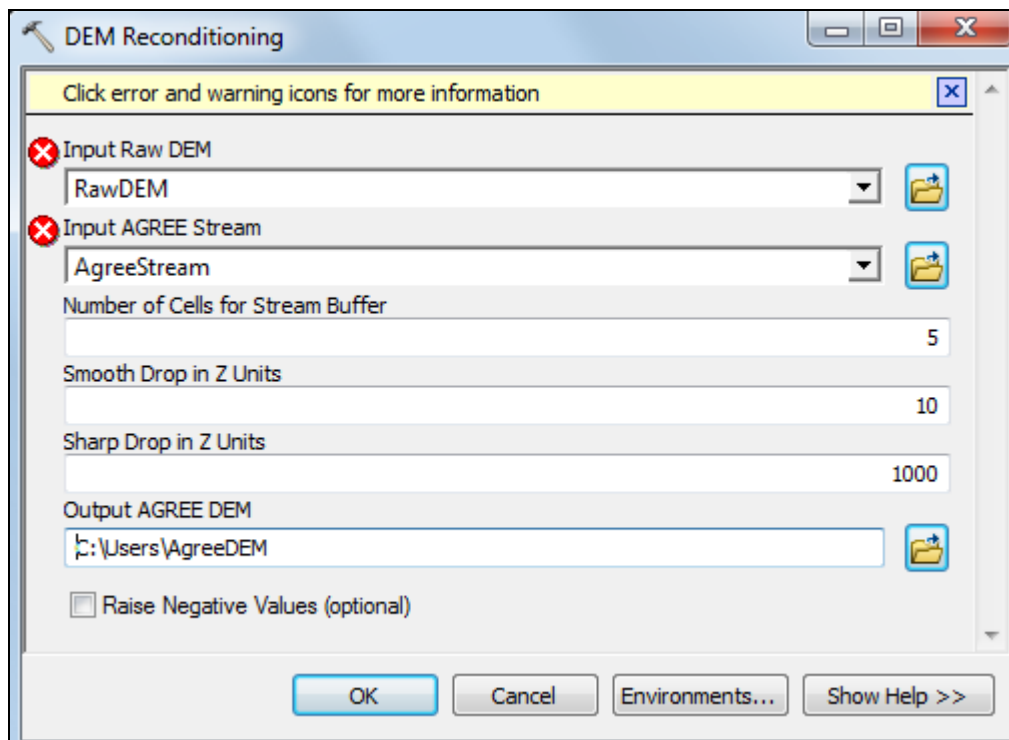
Figure 6-4. DEM Reconditioning Editor.
