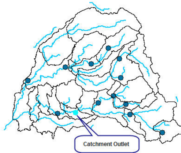
Figure 13-17. Stream Gage used as Catchment Outlet.
