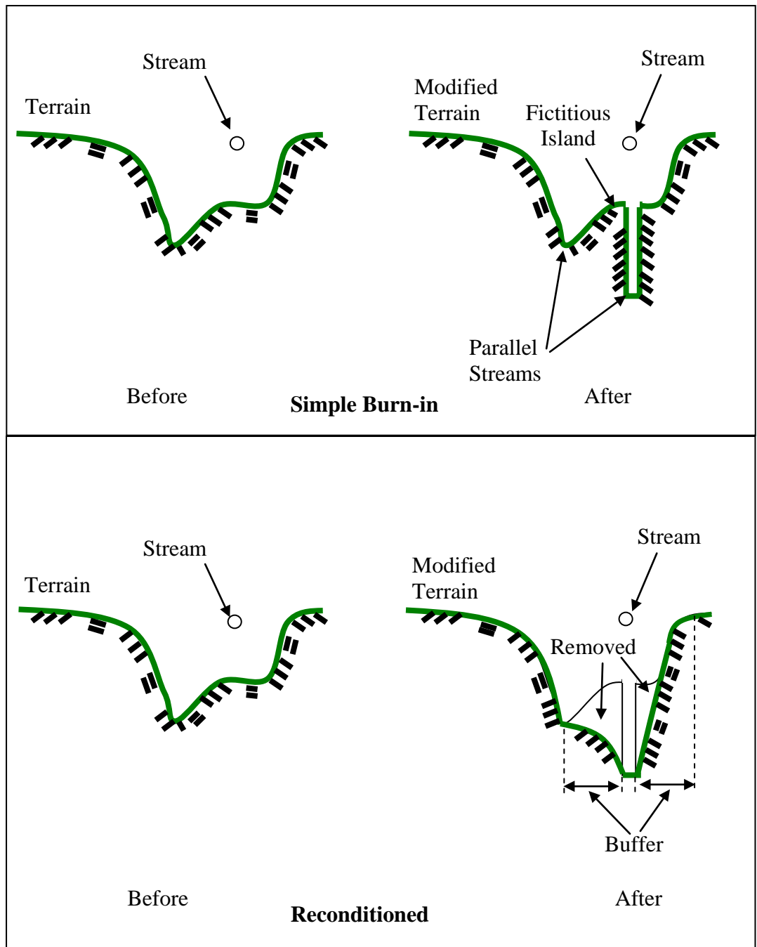
Figure 6-3. Cross-Section View of Burning-In Techniques.
