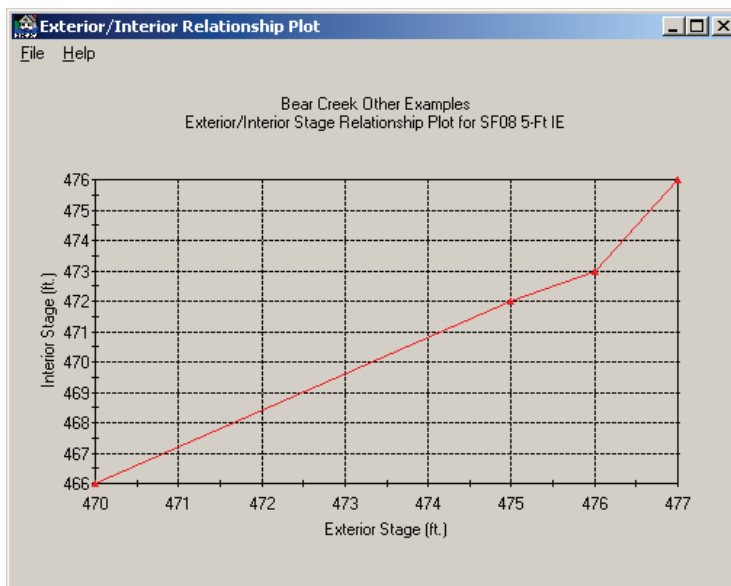
Figure 7.4 Exterior/Interior Relationship Plot Dialog Box
