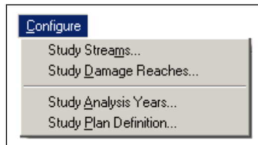
Figure 2.6 Configure Menu
