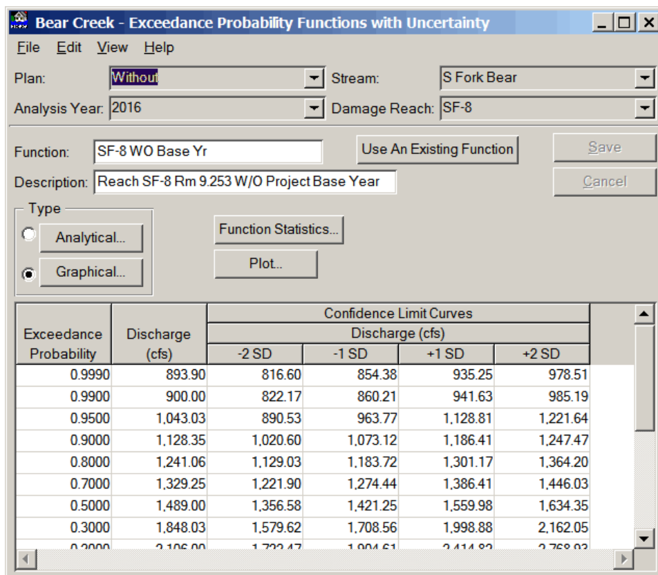
Figure 5.1 Exceedance Probability Functions with Uncertainty Dialog Box
