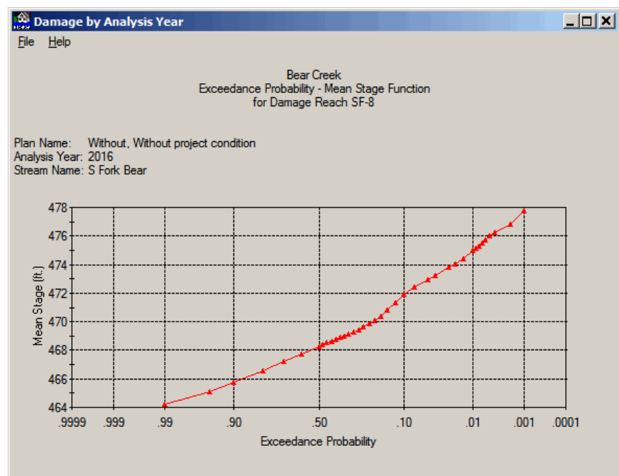
Figure 14.13 Exceedance Probability – Mean Stage Function - Plot
