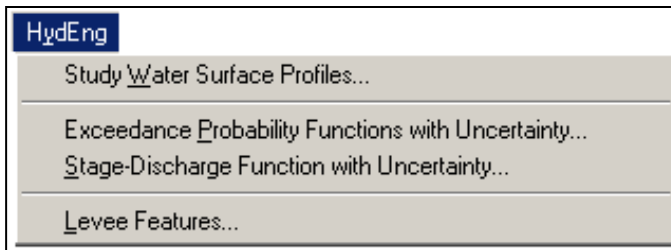
Figure 2.7 HydEng Menu
