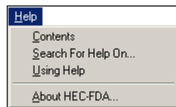
Figure 2.13 Help Menu
