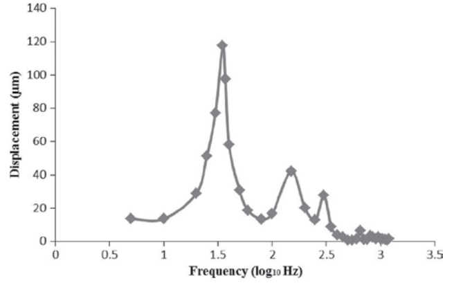
Fig. 11. Frequency response of point C (foot) measured with respect to global coordinates when the vertical actuator array is activated with driving sinusoidal input.
