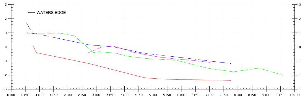
CROSS-SECTION
