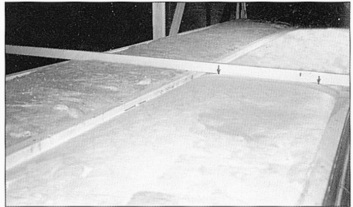
Figure 9. One-inch- (25-mm-) high airways mostly blocked by expansion of fibrous glass insulation.
