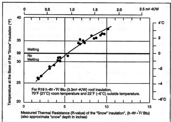
Figure 7. Measured and calculated temperatures of "snow" on the test roof.
