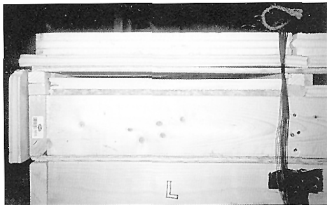
Figure 14. One-inch- (25-mm-) thick extruded polystyrene insulation boards (the light horizontal band below the dark airway) were not bowed by the fibrous glass insulation below. This airway is only ½ inch (13 mm) high. The insulation boards guaranteed its existence. Also note that a gap exists between the plywood roof deck and the "snow" insulation over the right third of this airway. That may explain why the snow insulation provided less thermal resistance than expected.
