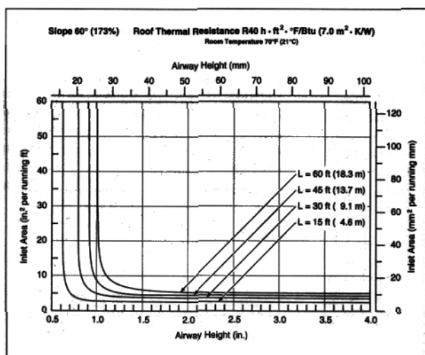
Figure 21. Airway heights and inlet areas for cathedral ceilings with a slope of 60 degrees.
