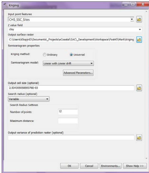
Figure 1: Settings used to create each interpolation.
