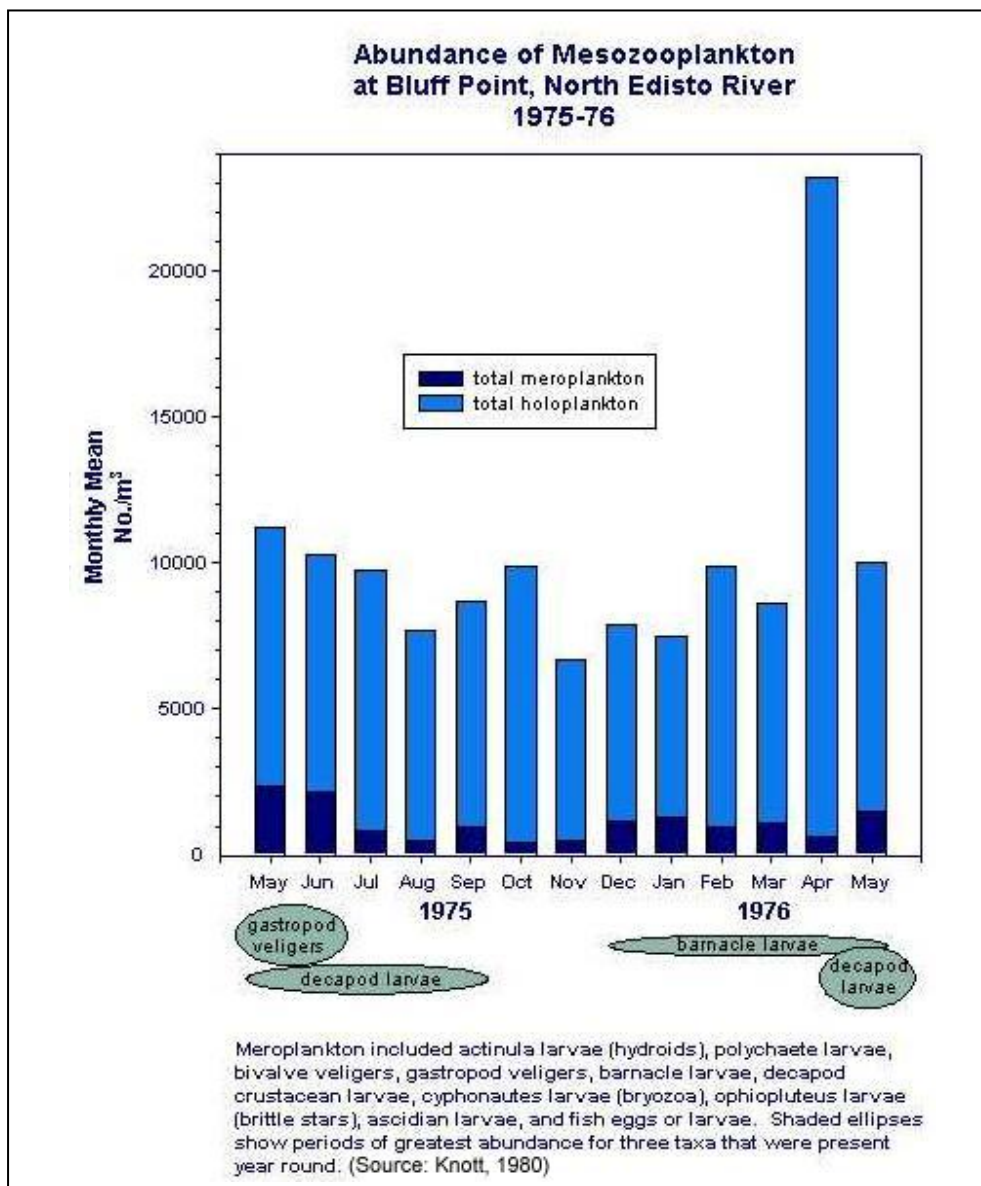
Figure 9 Monthly zooplankton abundance in a South Carolina estuary
