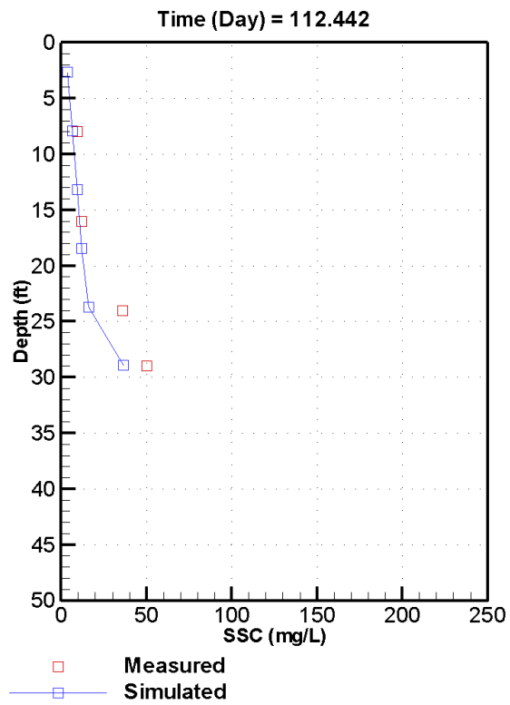
C-36. Measured versus simulated TSS at station T-2W on April 21 and 22, 2003
