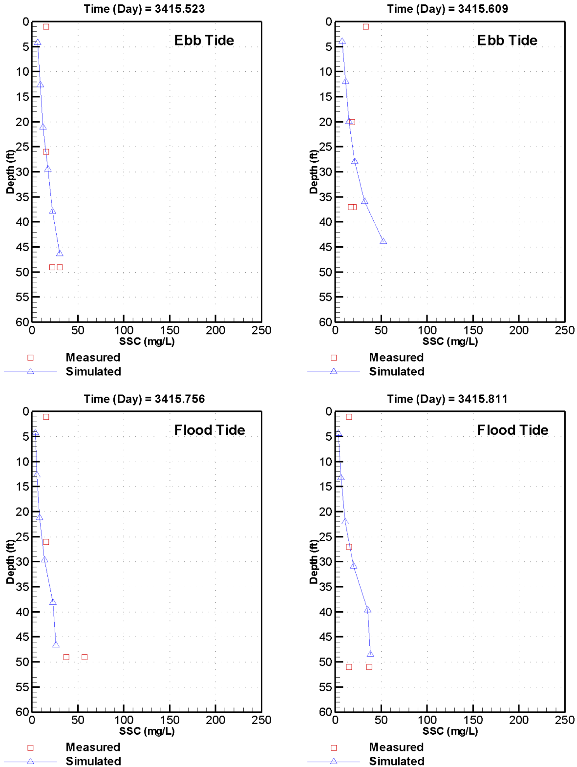
Figure C-3. Measured versus simulated SSC at station CH-2 on May 7, 2012 – spring tide conditions
