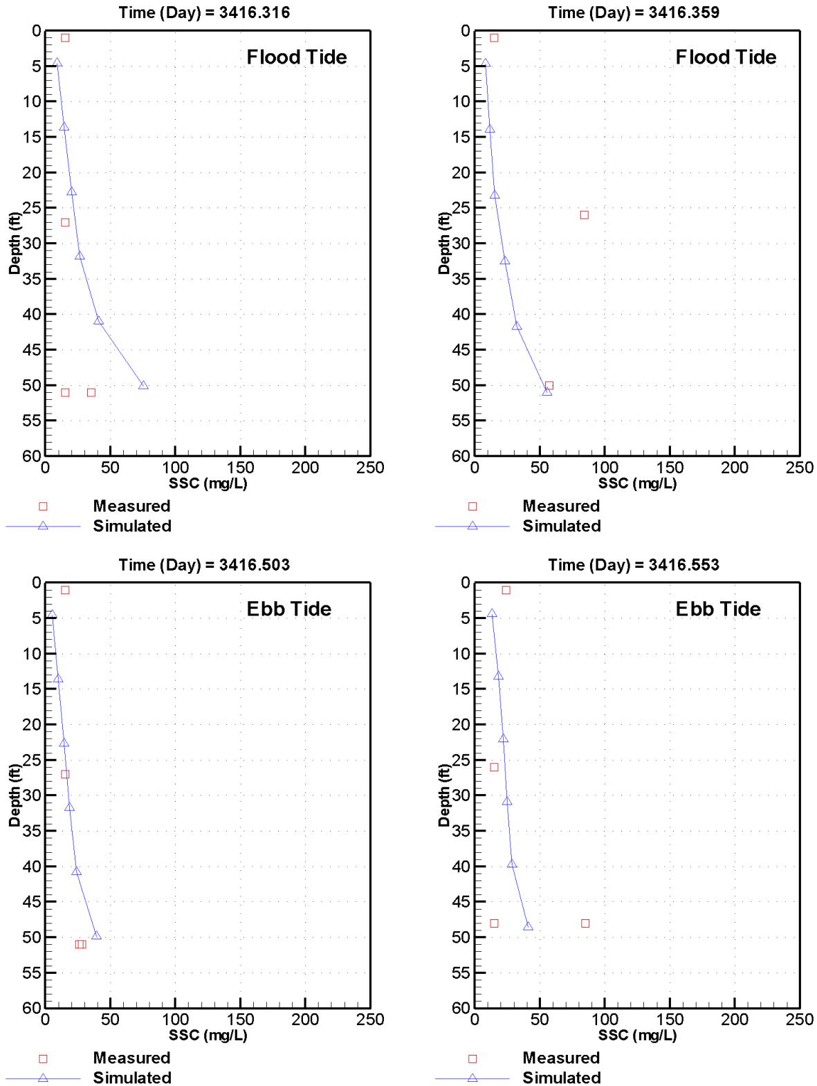
Figure C-15. Measured versus simulated SSC at station CH-8 on May 8, 2012 – spring tide conditions
