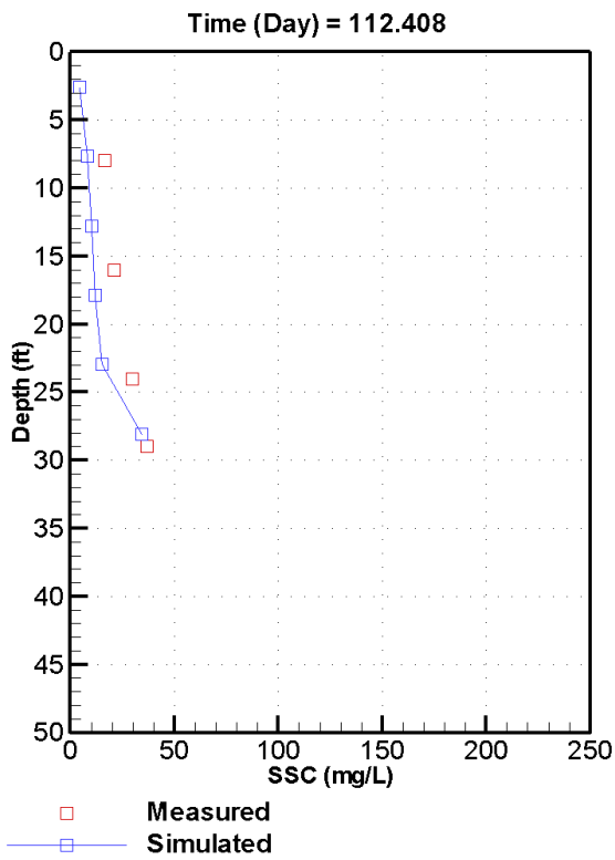
C-36. Measured versus simulated TSS at station T-2W on April 21 and 22, 2003
