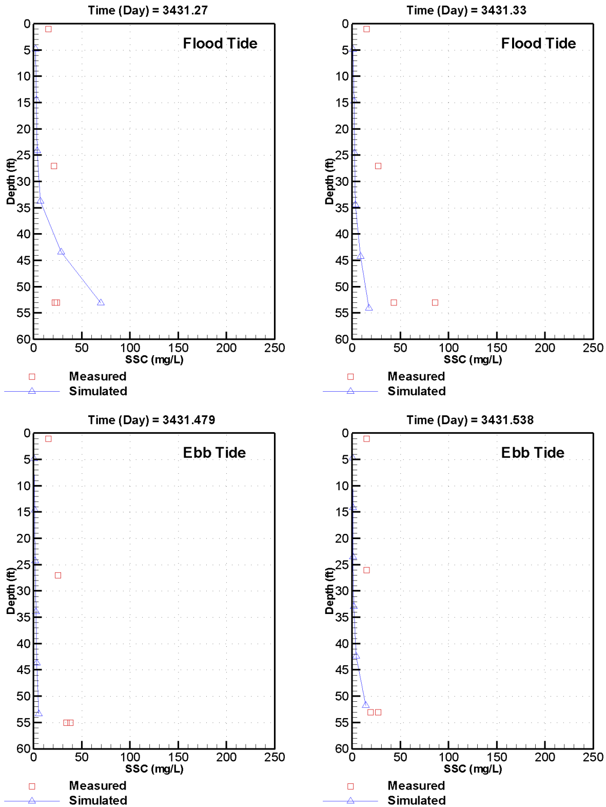
Figure C-24. Measured versus simulated SSC at station CH-12 on May 23, 2012 – neap tide conditions
