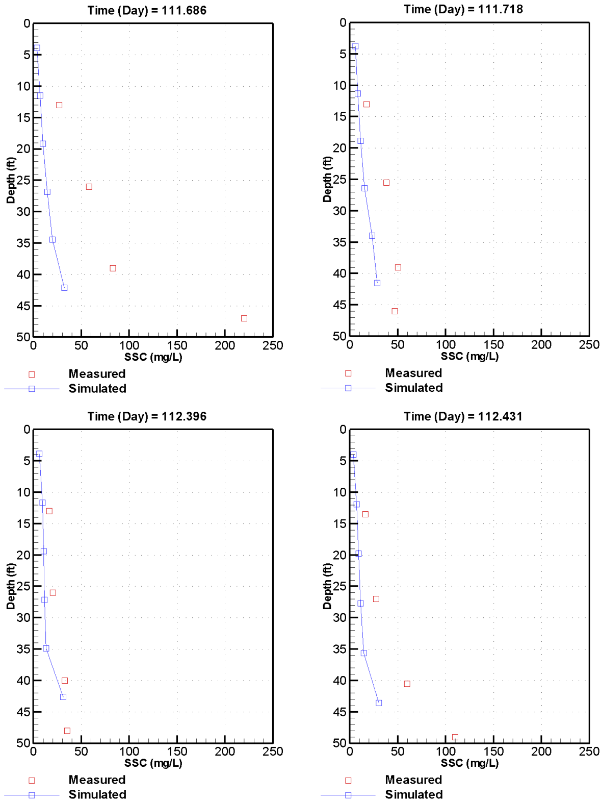
Figure C-28. Measured versus simulated TSS at station T-2C on April 21 and 22, 2003
