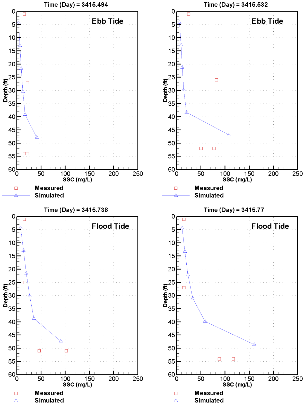
Figure C-11. Measured versus simulated SSC at station CH-6 on May 7, 2012 – spring tide conditions
