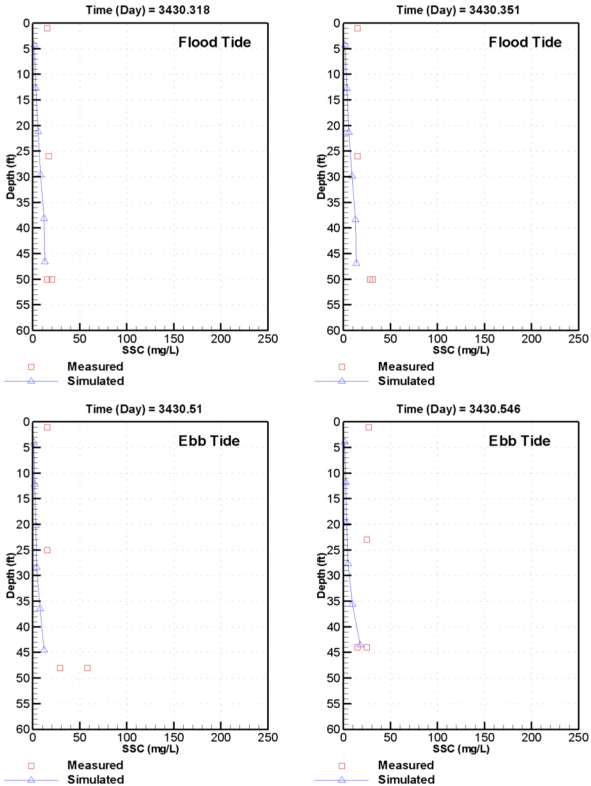
Figure C-8. Measured versus simulated SSC at station CH-4 on May 22, 2012 – neap tide conditions
