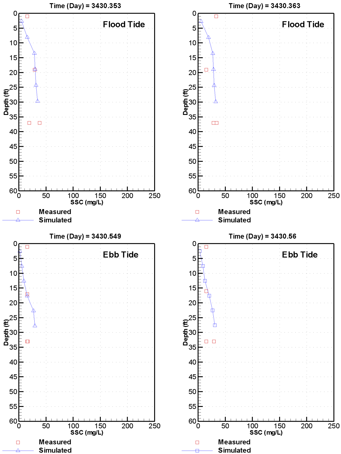
Figure C-2. Measured versus simulated SSC at station CH-1 on May 22, 2012 – neap tide conditions
