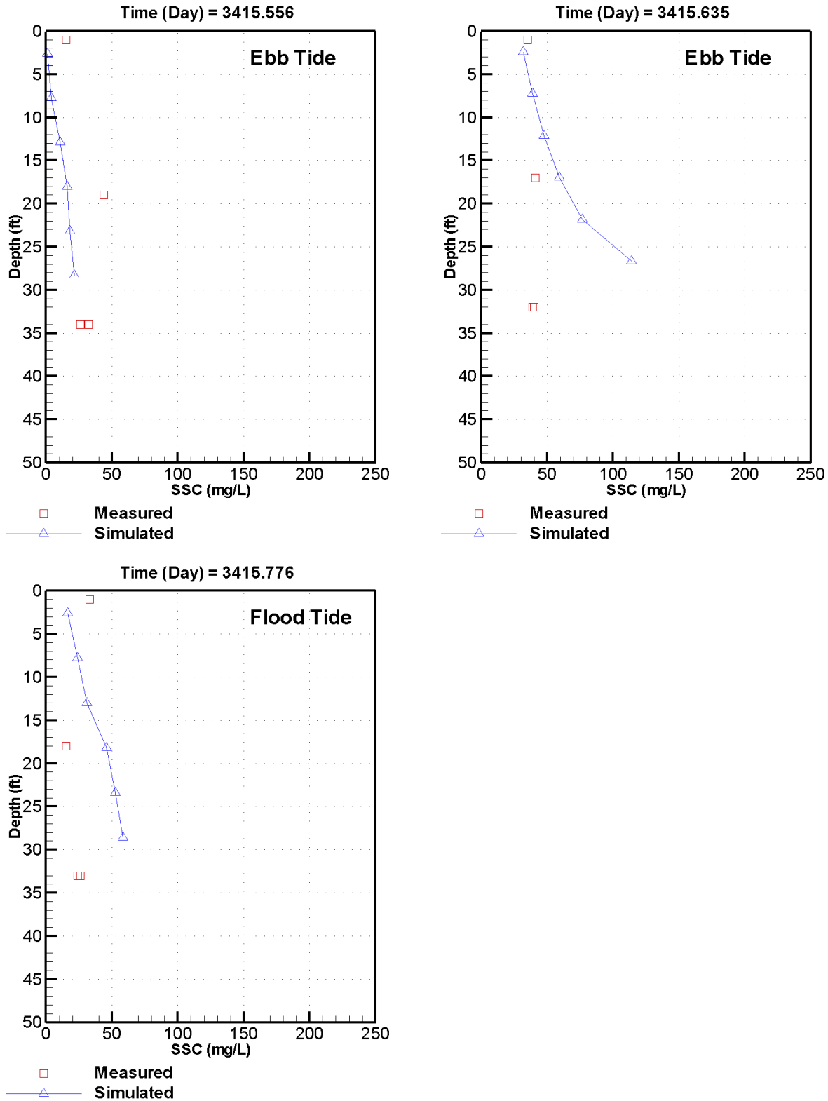
Figure C-1. Measured versus simulated SSC at station CH-1 on May 7, 2012 – spring tide conditions
