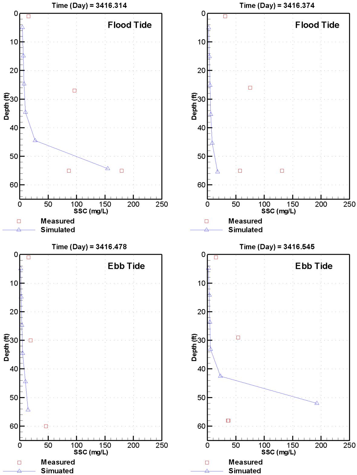
Figure C-23. Measured versus simulated SSC at station CH-12 on May 8, 2012 – spring tide conditions
