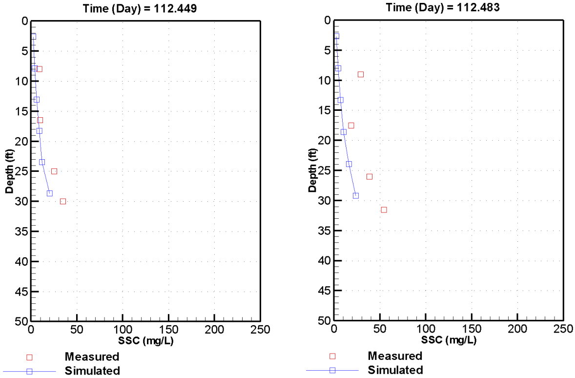
C-37. Measured versus simulated TSS at station T-2W on April 22, 2003
