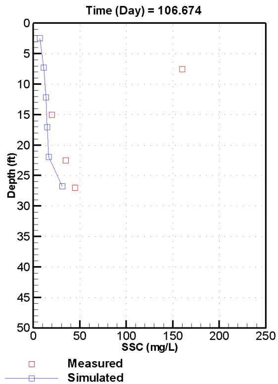
C-30. Measured versus simulated TSS at station T-2E on April 15 and 16, 2003
