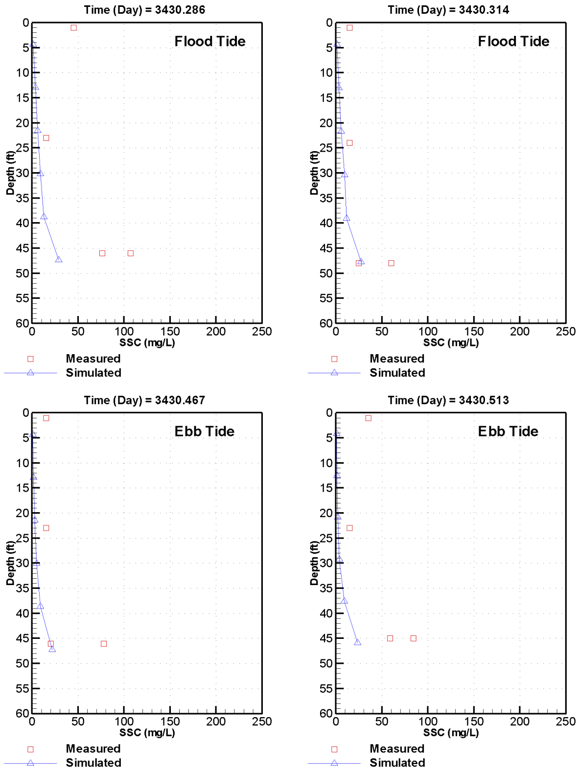
Figure C-6. Measured versus simulated SSC at station CH-3 on May 22, 2012 – neap tide conditions
