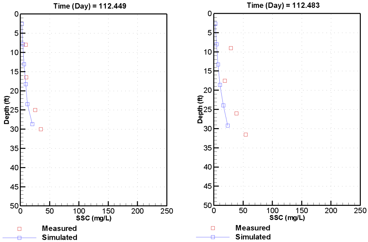
C-33. Measured versus simulated TSS at station T-2E on April 22, 2003
