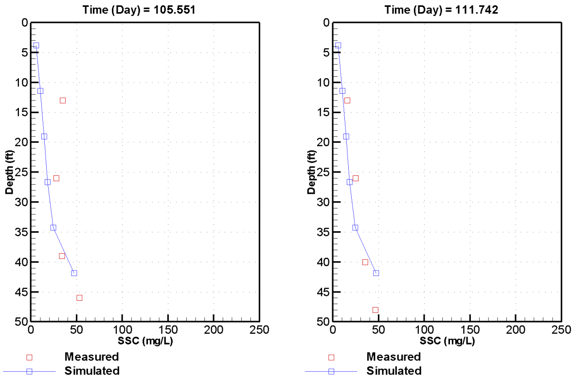
C-38. Measured versus simulated TSS at station T-6 on April 15 and 21, 2003
