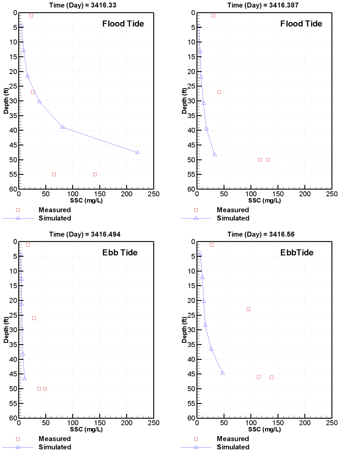
Figure C-21. Measured versus simulated SSC at station CH-11 on May 8, 2012 – spring tide conditions
