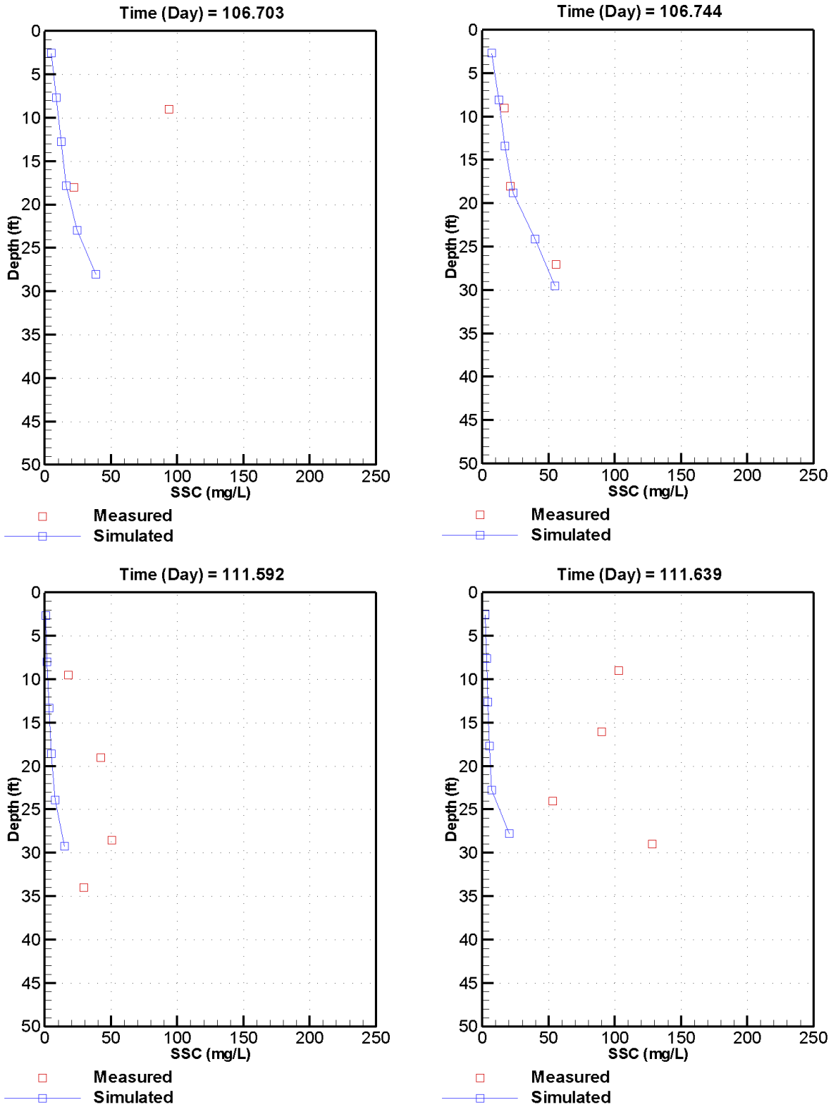
C-31. Measured versus simulated TSS at station T-2E on April 16 and 21, 2003
