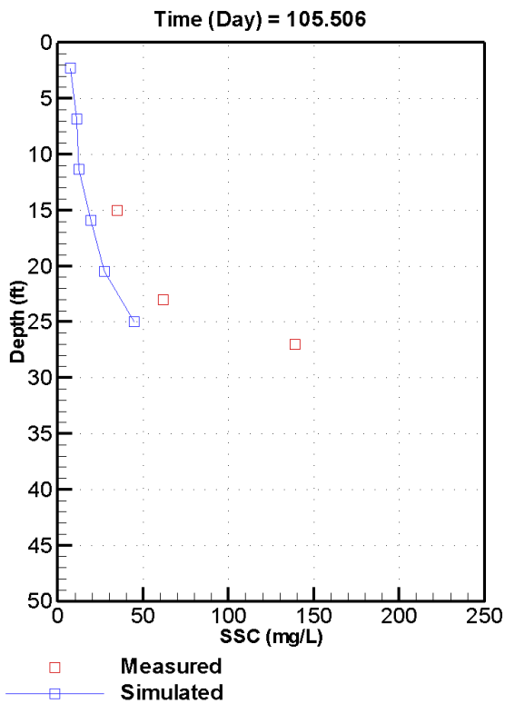
C-30. Measured versus simulated TSS at station T-2E on April 15 and 16, 2003
