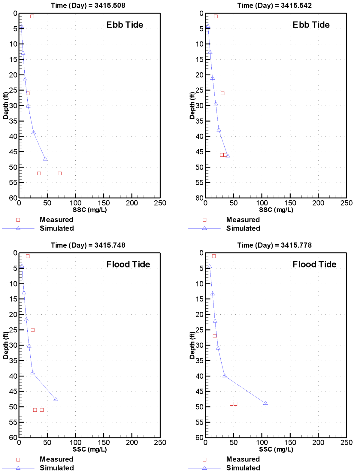
Figure C-9. Measured versus simulated SSC at station CH-5 on May 7, 2012 – spring tide conditions
