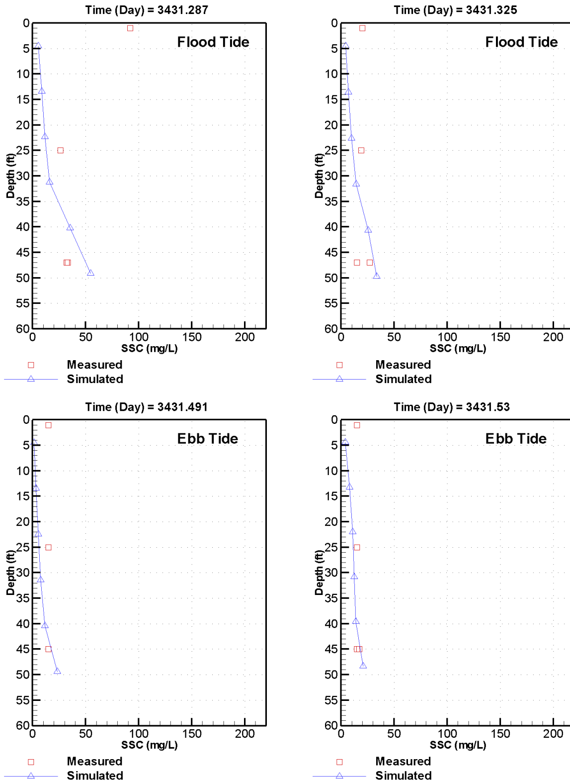
Figure C-16. Measured versus simulated SSC at station CH-8 on May 23, 2012 – neap tide conditions
