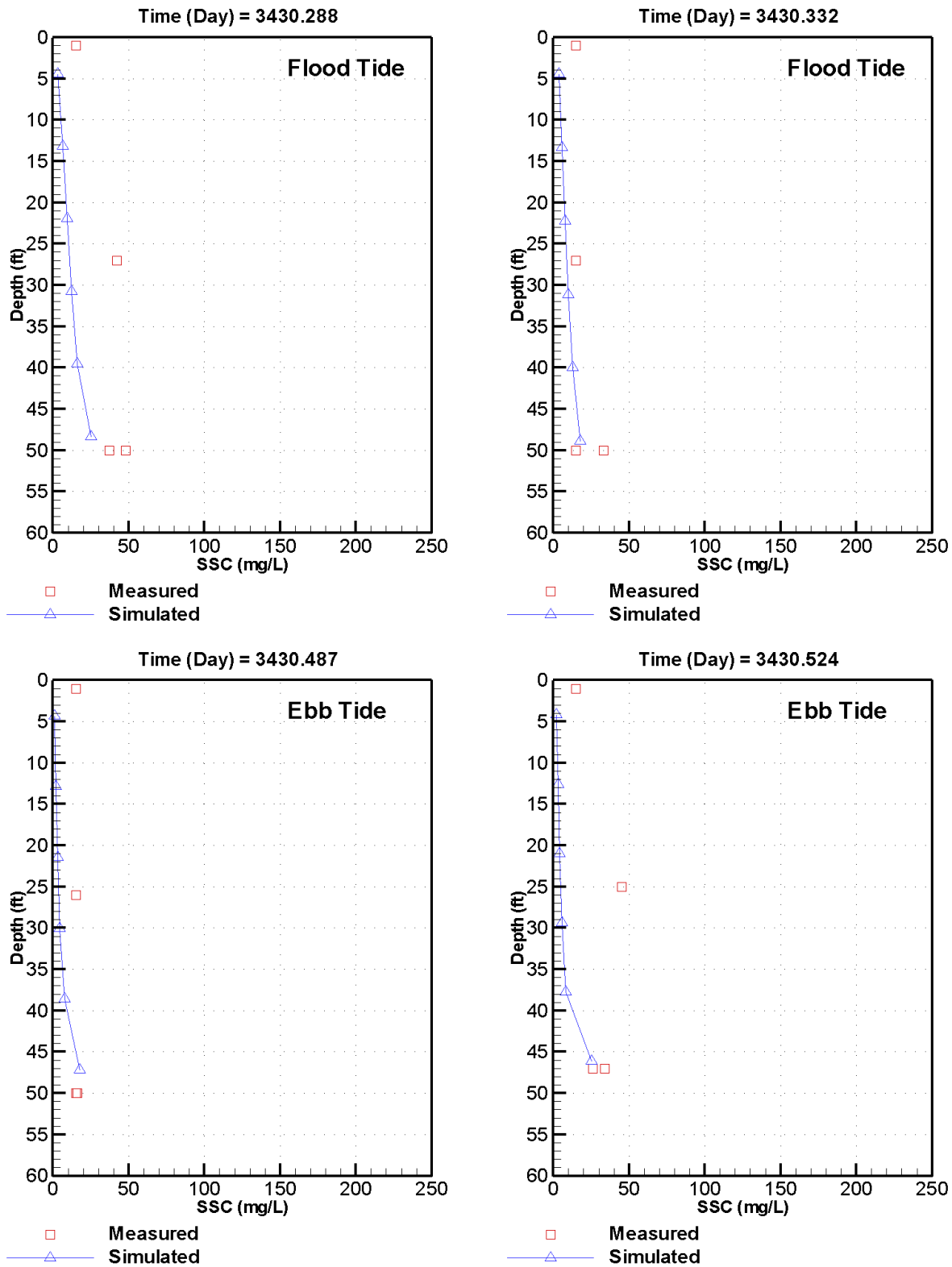
Figure C-12. Measured versus simulated SSC at station CH-6 on May 22, 2012 – neap tide conditions
