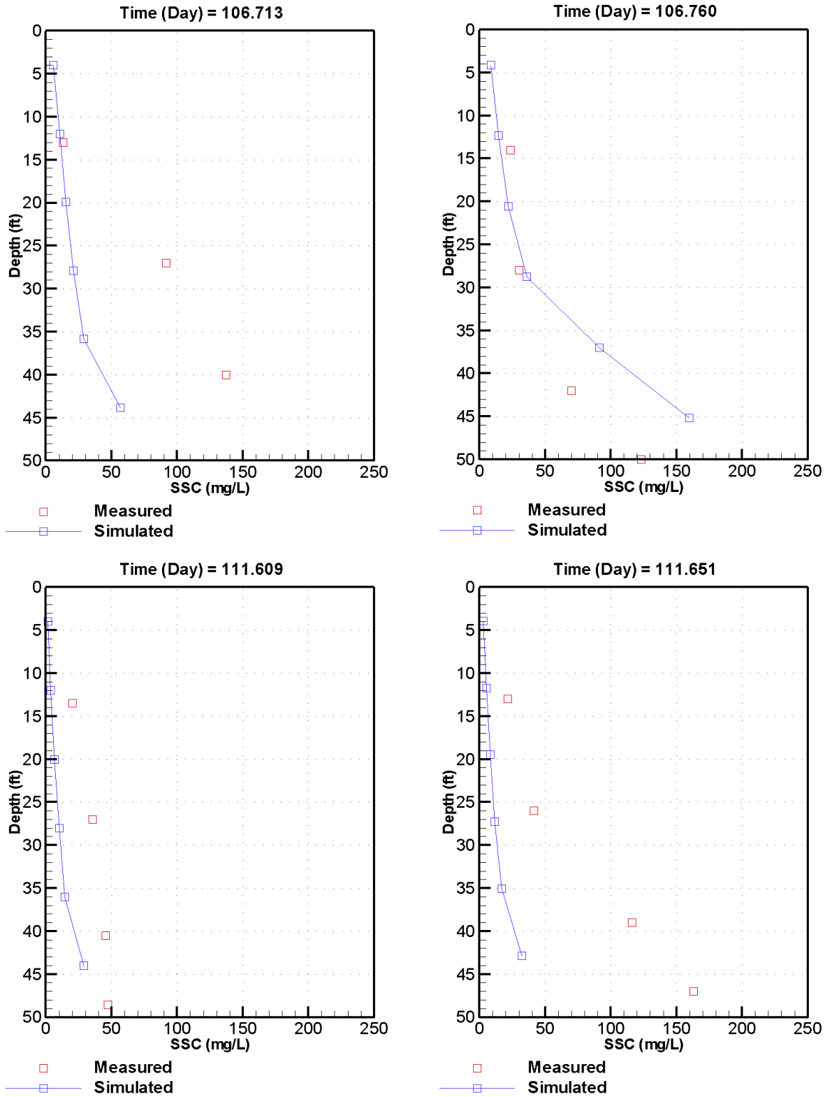
Figure C-27. Measured versus simulated TSS at station T-2C on April 16 and 21, 2003
