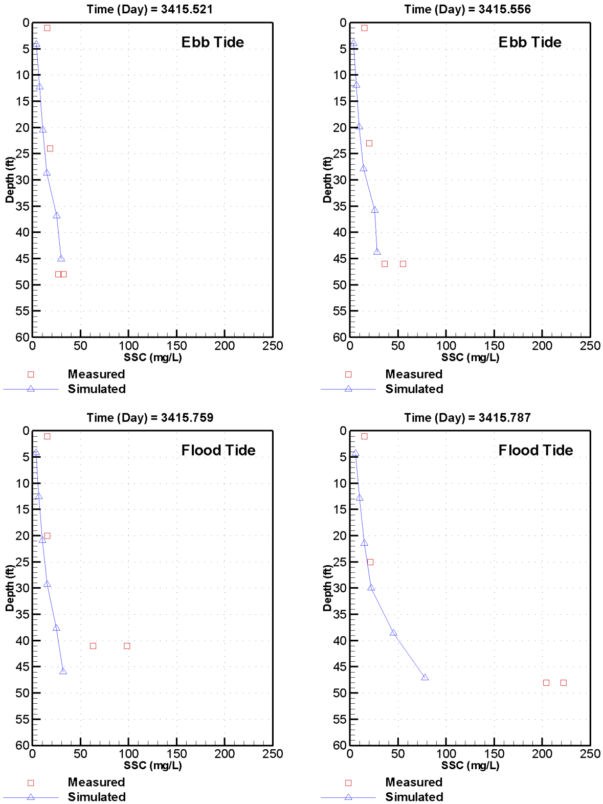
Figure C-7. Measured versus simulated SSC at station CH-4 on May 7, 2012 – spring tide conditions
