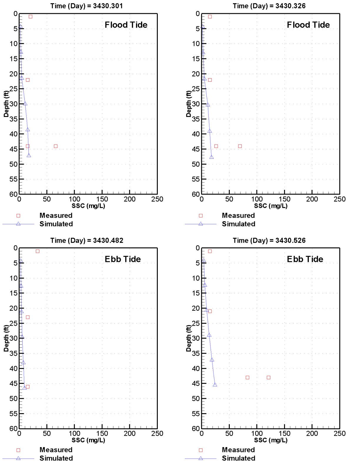
Figure C-4. Measured versus simulated SSC at station CH-2 on May 22, 2012 – neap tide conditions
