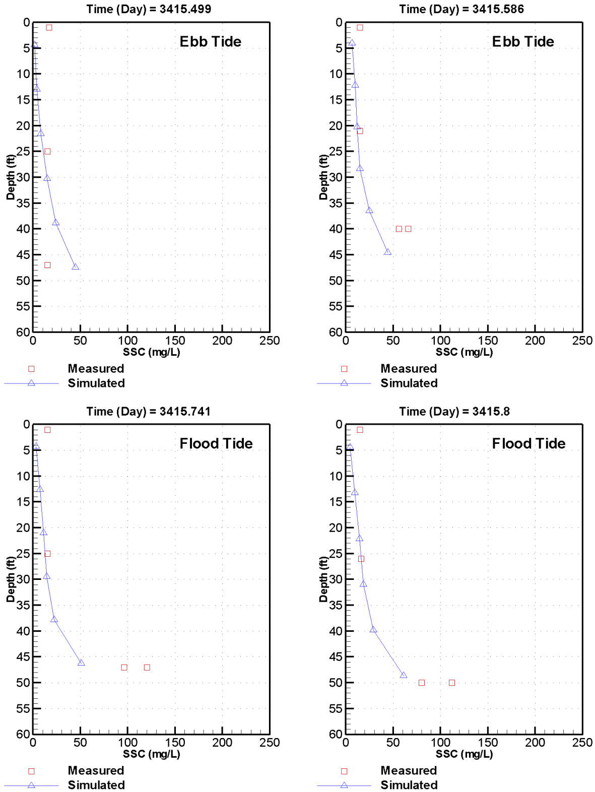
Figure C-5. Measured versus simulated SSC at station CH-3 on May 7, 2012 – spring tide conditions
