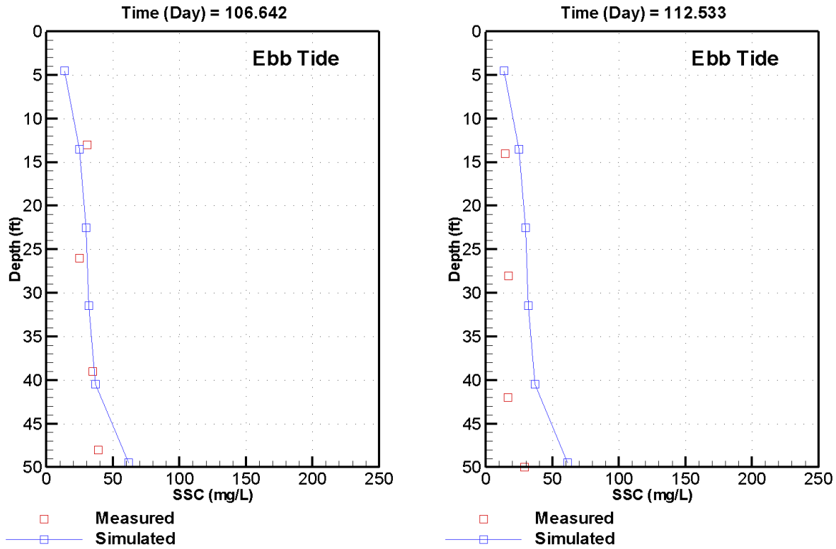
Figure C-25. Measured versus simulated TSS at station T-1 on April 16 and April 22, 2003
