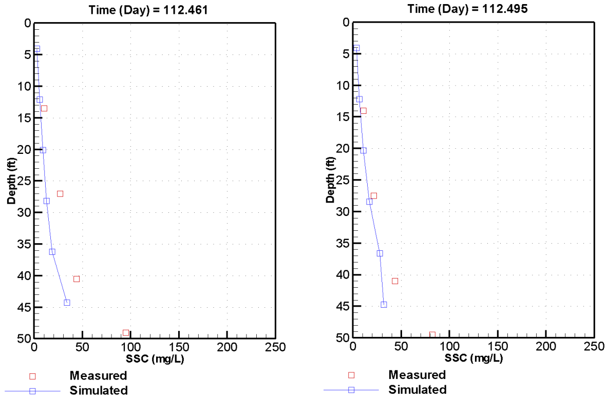
Figure C-29. Measured versus simulated TSS at station T-2C on April 22, 2003
