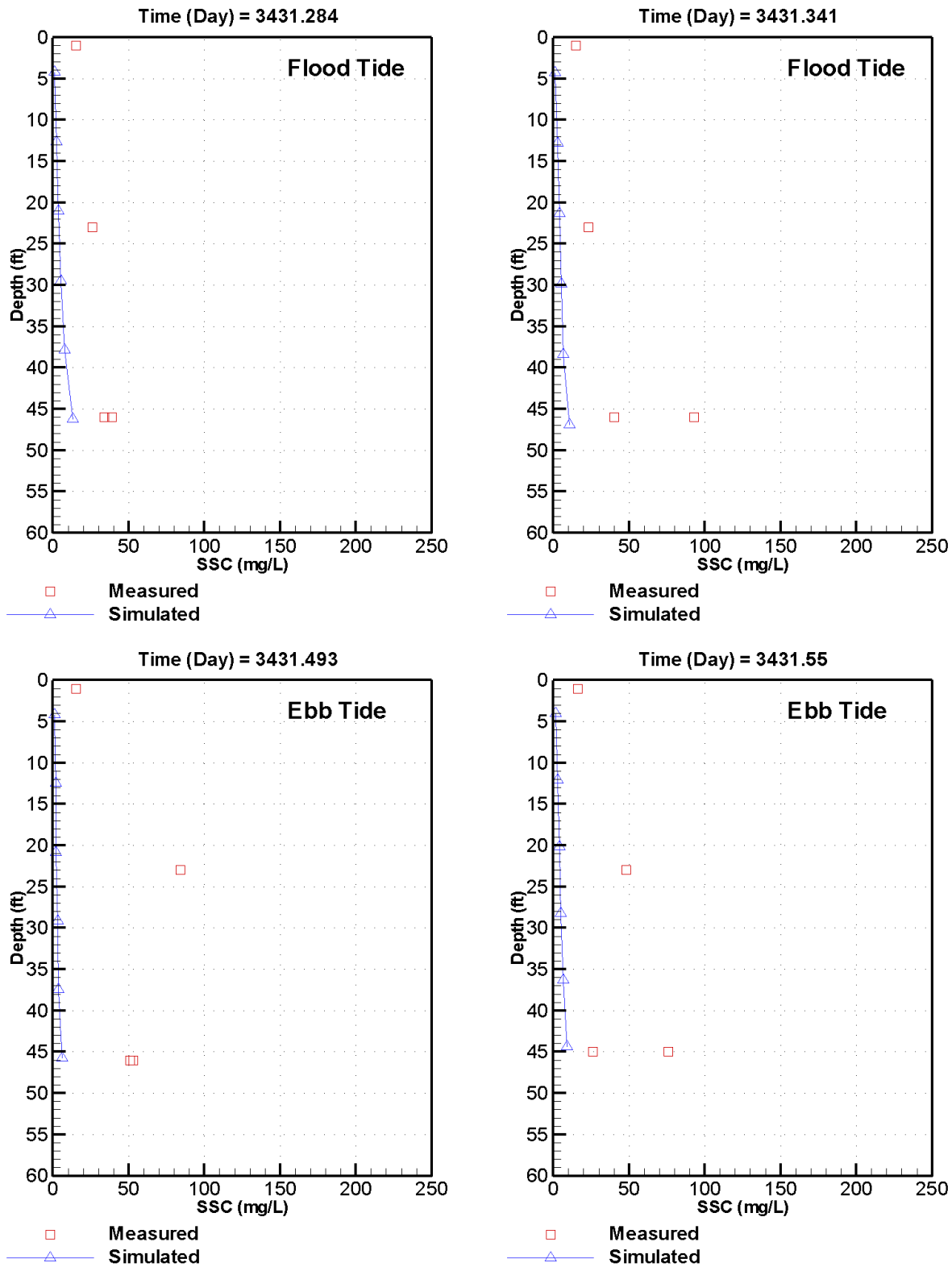
Figure C-22. Measured versus simulated SSC at station CH-11 on May 23, 2012 – neap tide conditions
