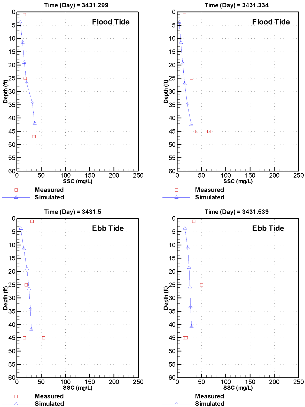
Figure C-14. Measured versus simulated SSC at station CH-7 on May 23, 2012 – neap tide conditions
