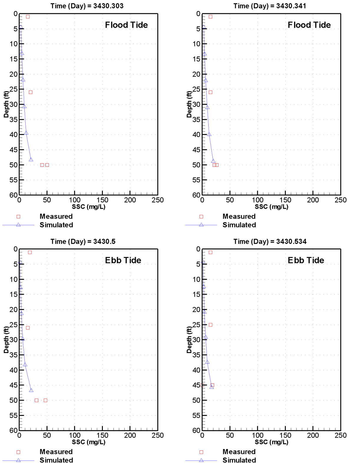
Figure C-10. Measured versus simulated SSC at station CH-5 on May 22, 2012 – neap tide conditions
