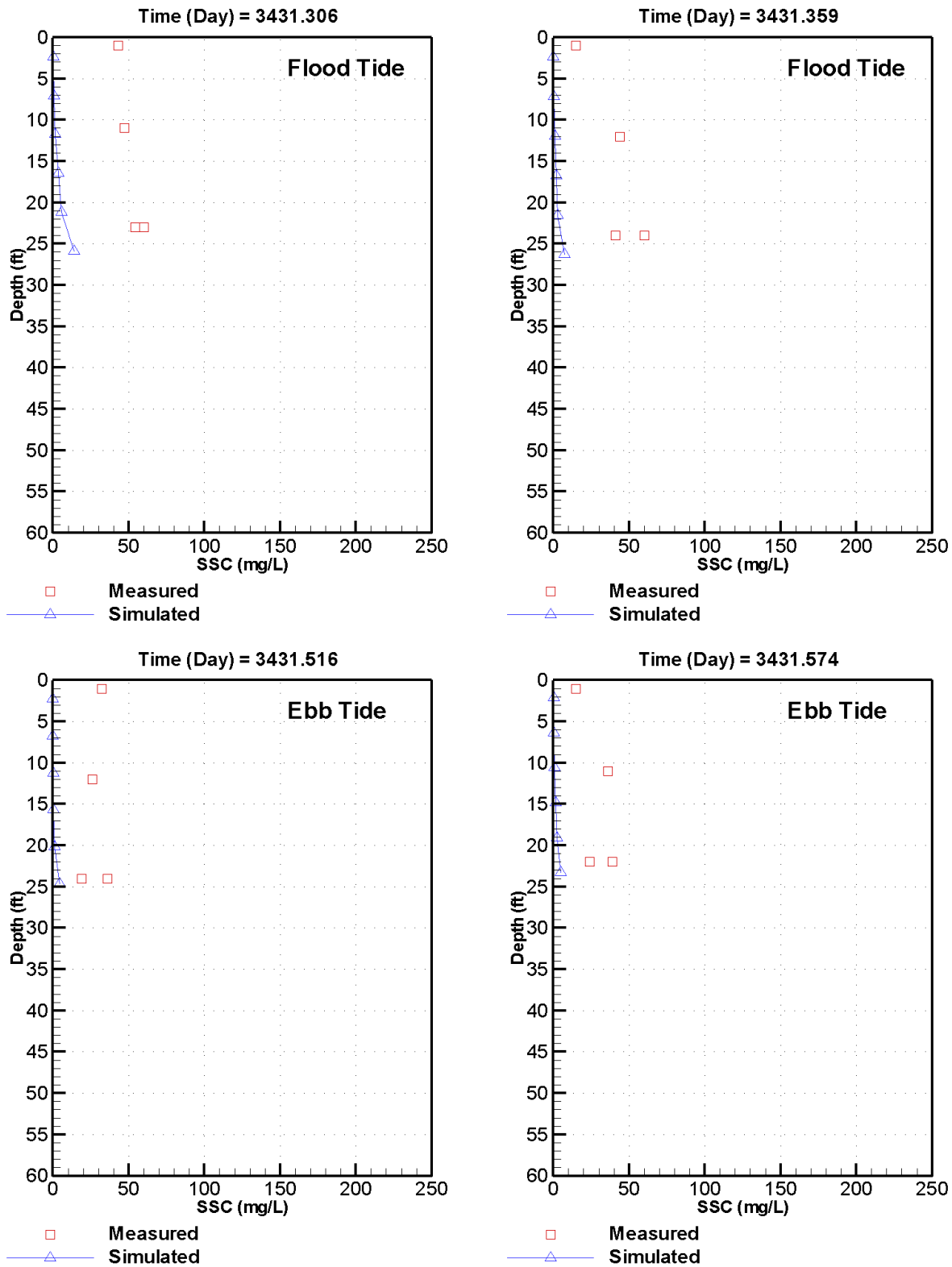
Figure C-20. Measured versus simulated SSC at station CH-10 on May 23, 2012 – neap tide conditions
