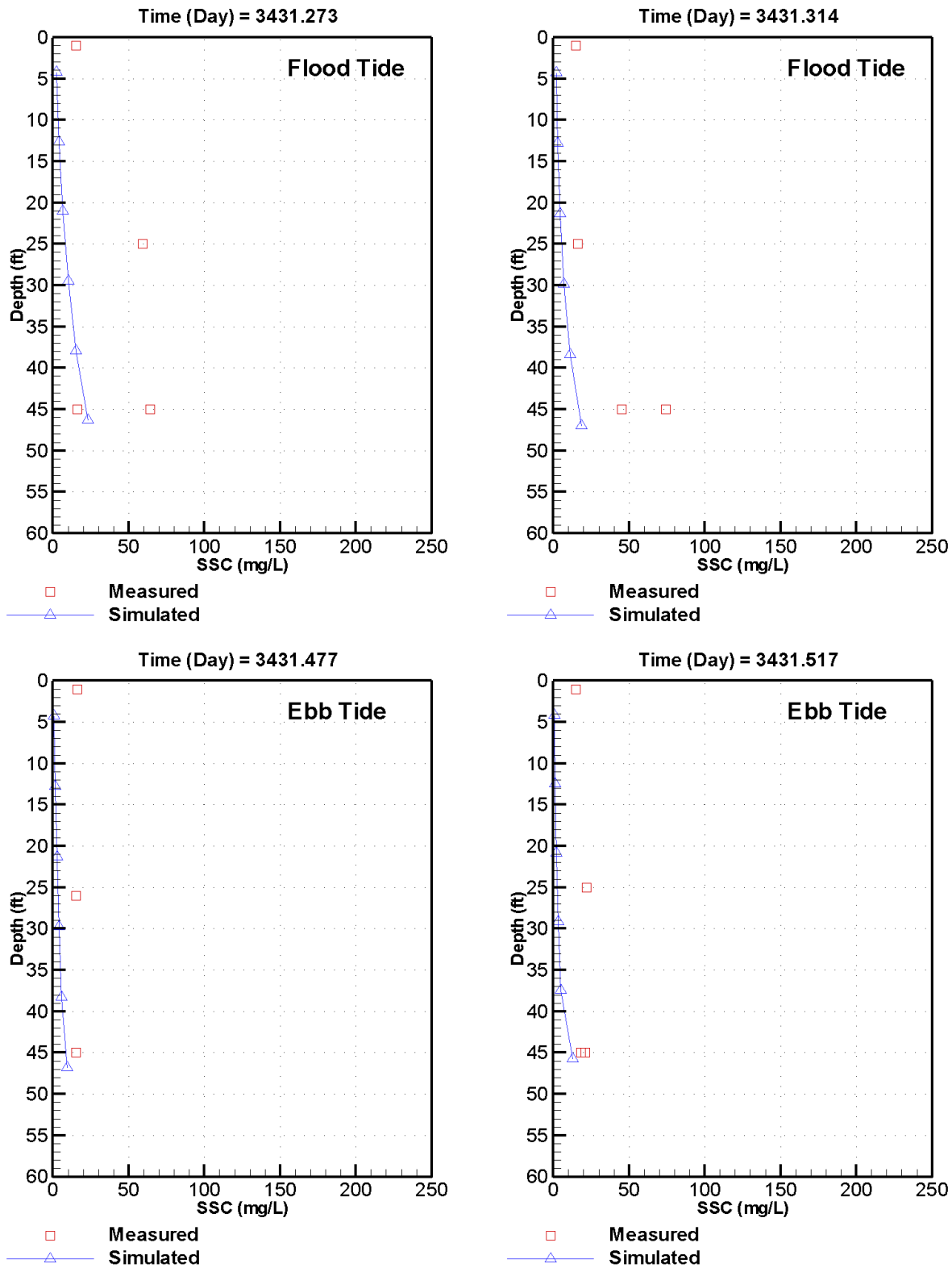
Figure C-18. Measured versus simulated SSC at station CH-9 on May 23, 2012 – neap tide conditions
