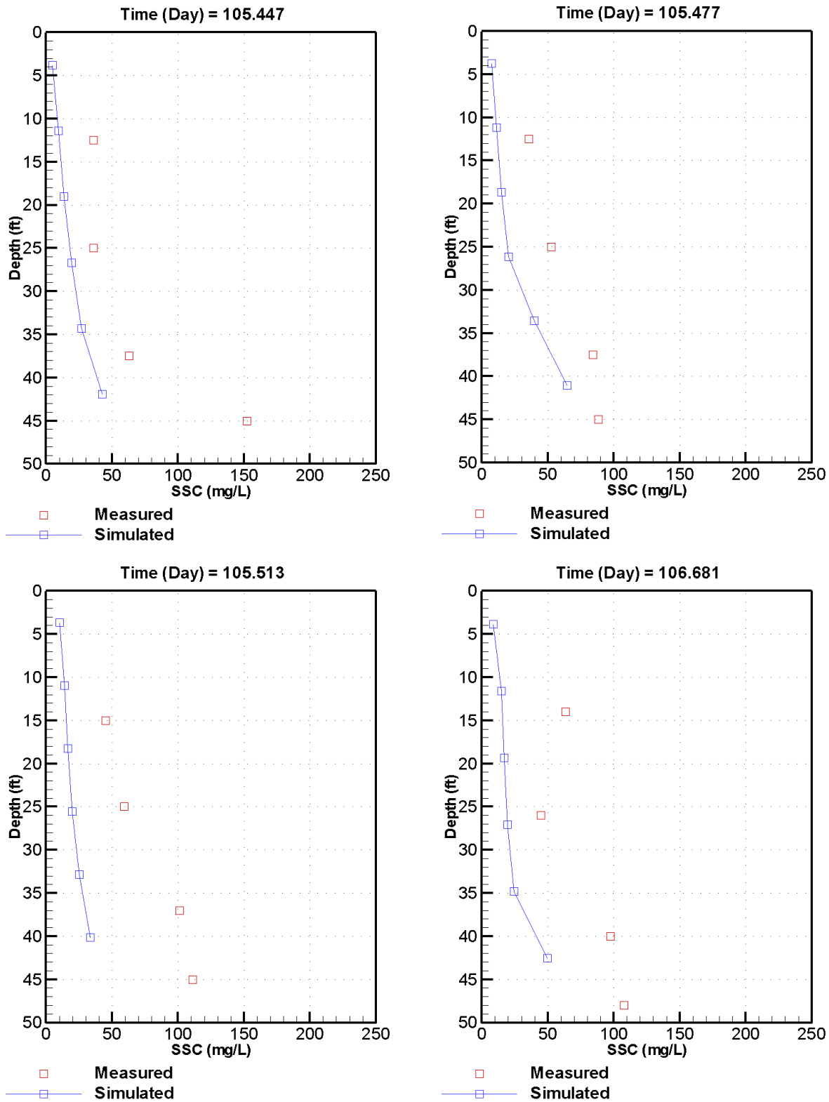
Figure C-26. Measured versus simulated TSS at station T-2C on April 15 and 16, 2003
