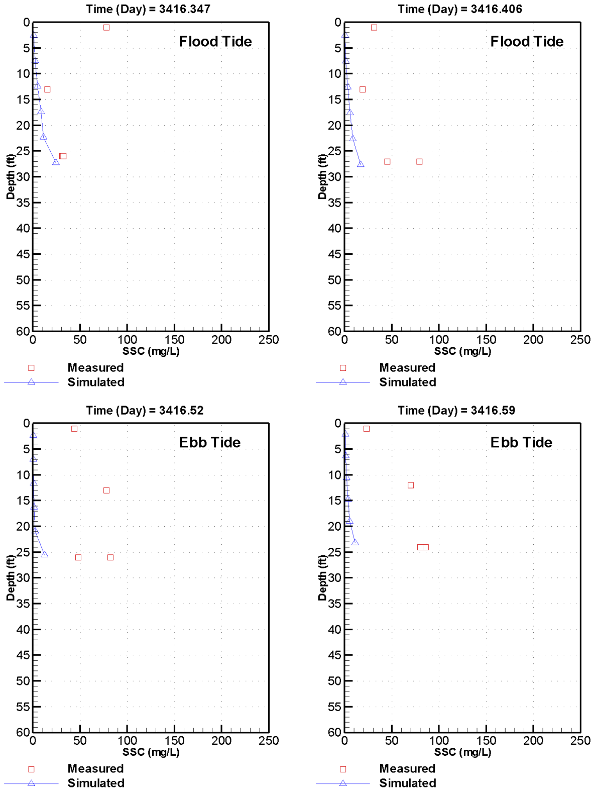
Figure C-19. Measured versus simulated SSC at station CH-10 on May 8, 2012 – spring tide conditions
