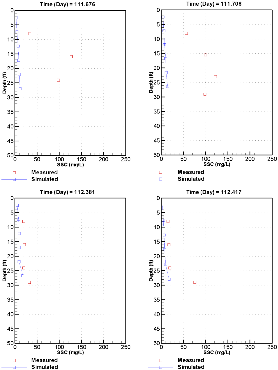
C-32. Measured versus simulated TSS at station T-2E on April 21 and 22, 2003
