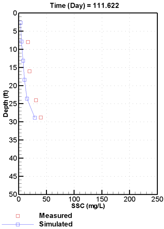
C-35. Measured versus simulated TSS at station T-2W on April 16 and 21, 2003
