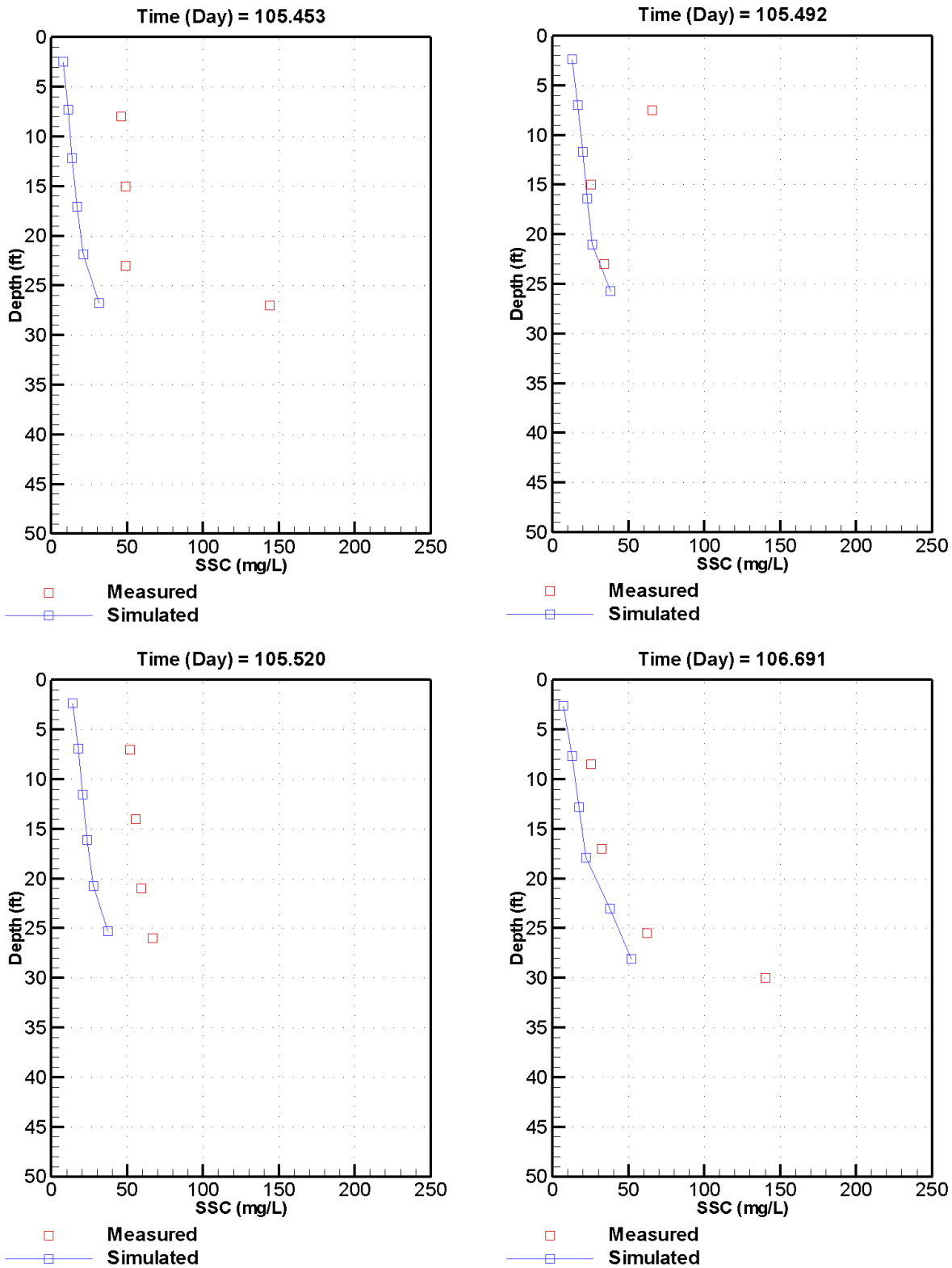
C-34. Measured versus simulated TSS at station T-2W on April 15 and 16, 2003
