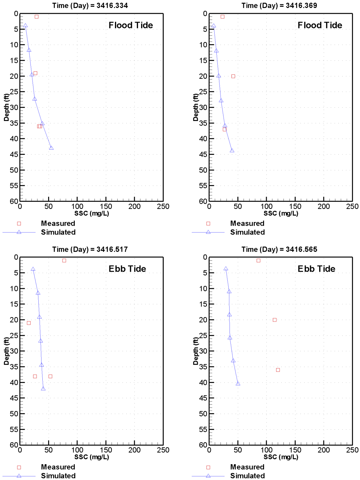
Figure C-13. Measured versus simulated SSC at station CH-7 on May 8, 2012 – spring tide conditions
