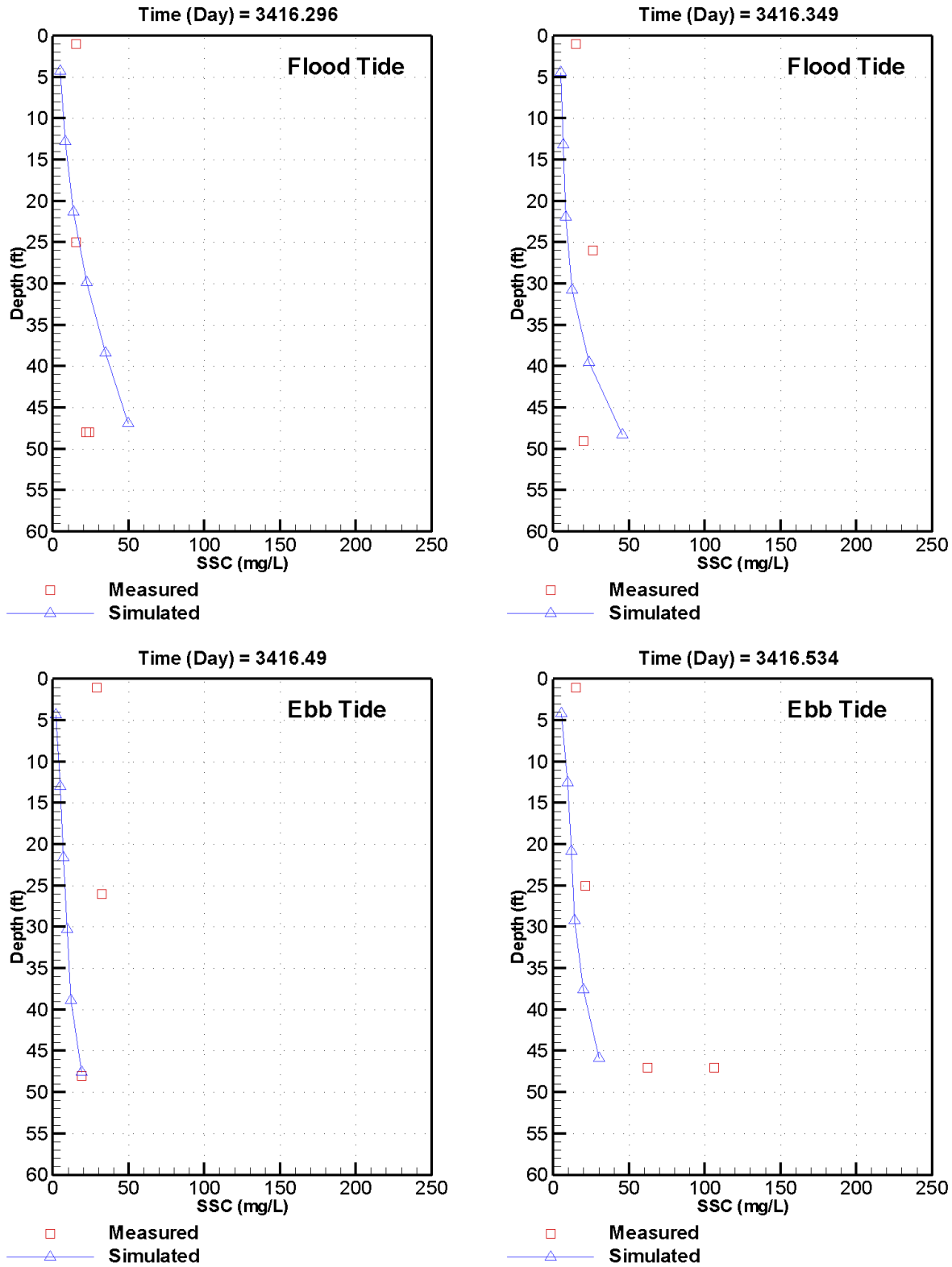
Figure C-17. Measured versus simulated SSC at station CH-9 on May 8, 2012 – spring tide conditions
