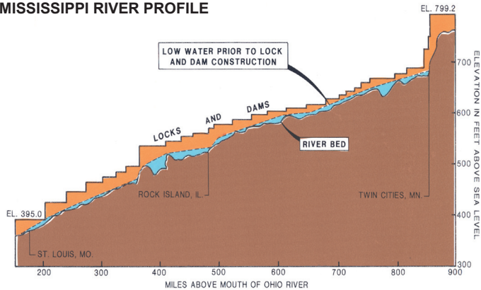
MISSISSIPPI RIVER PROFILE
