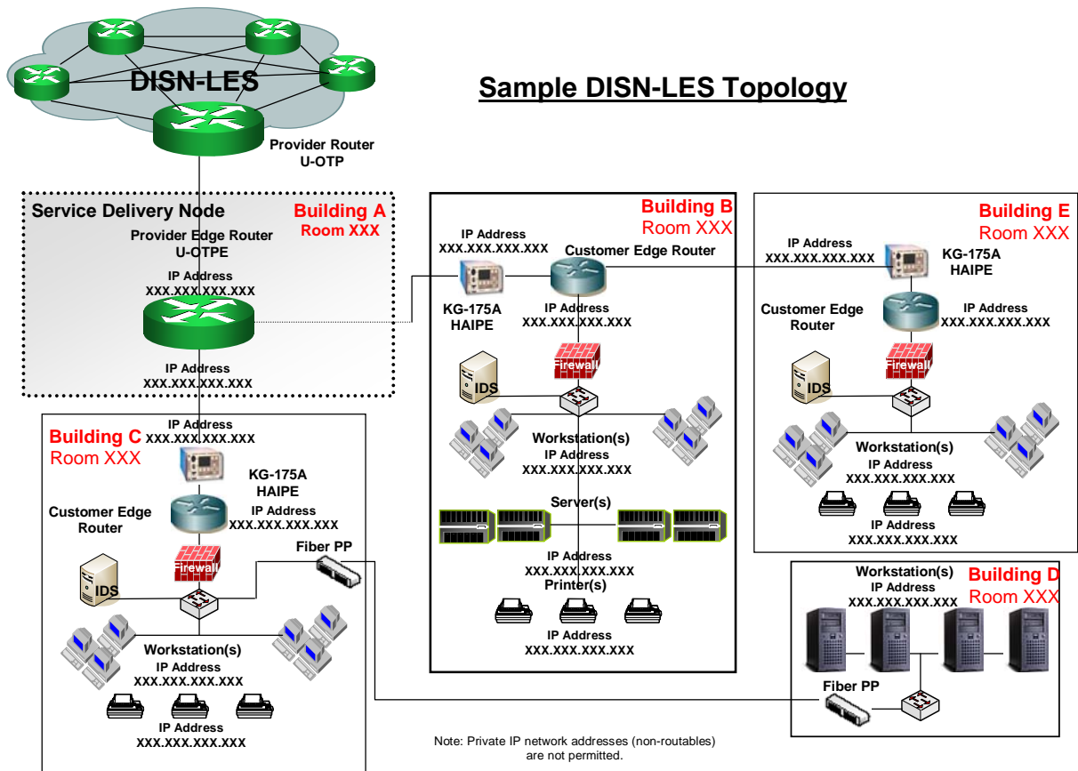
Figure 1 Sample DISN-LES Topology
