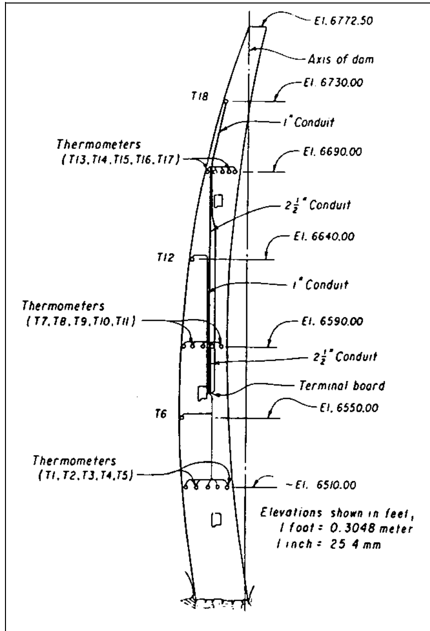
Figure 12-7. Layout for thermometer installation (USBR 1987)
