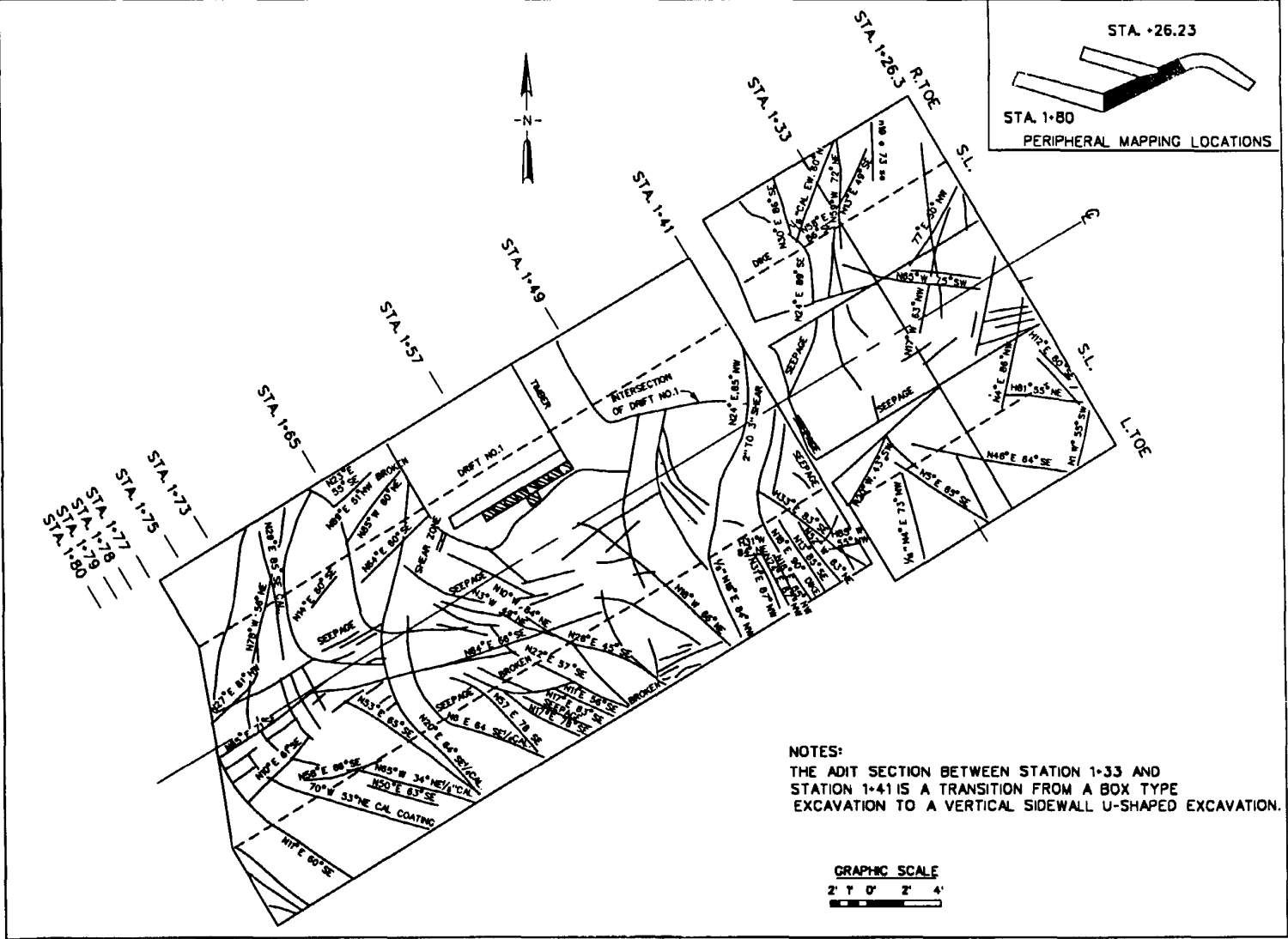
Figure 10-3. Adit periphery mapping plan view from Portugues Dam Design Memorandum No. 22 (USAED, Jacksonville, 1988b)
