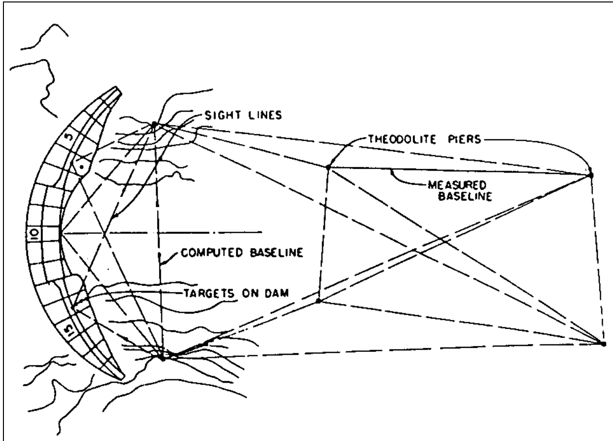
Figure 12-6. Layout for triangular or trilateration network
