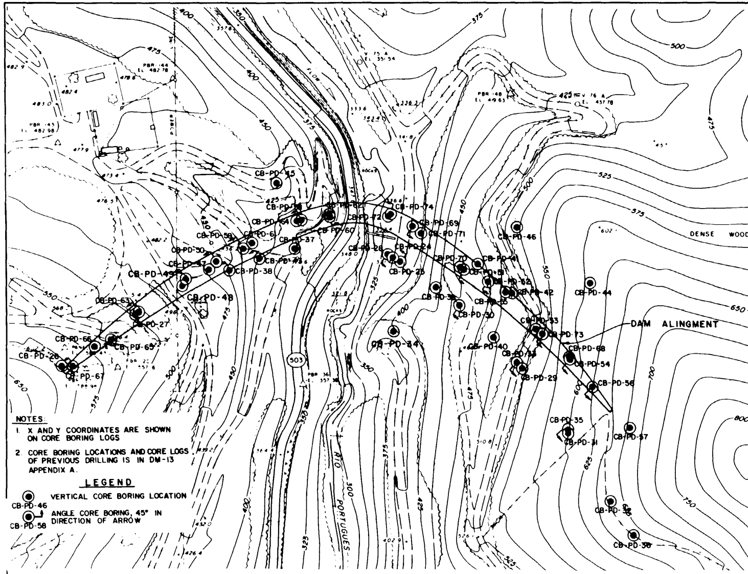
Figure 10-1. Arch dam boring layout plan from Portugues Dam Design Memorandum No. 22 (USAED, Jacksonville, 1988b)
