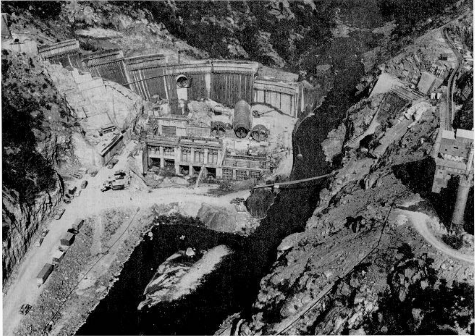
Figure 13-6. Channel used in the Phase I diversion for Smith Mountain Dam (photograph courtesy of Appalachian Power Company)
