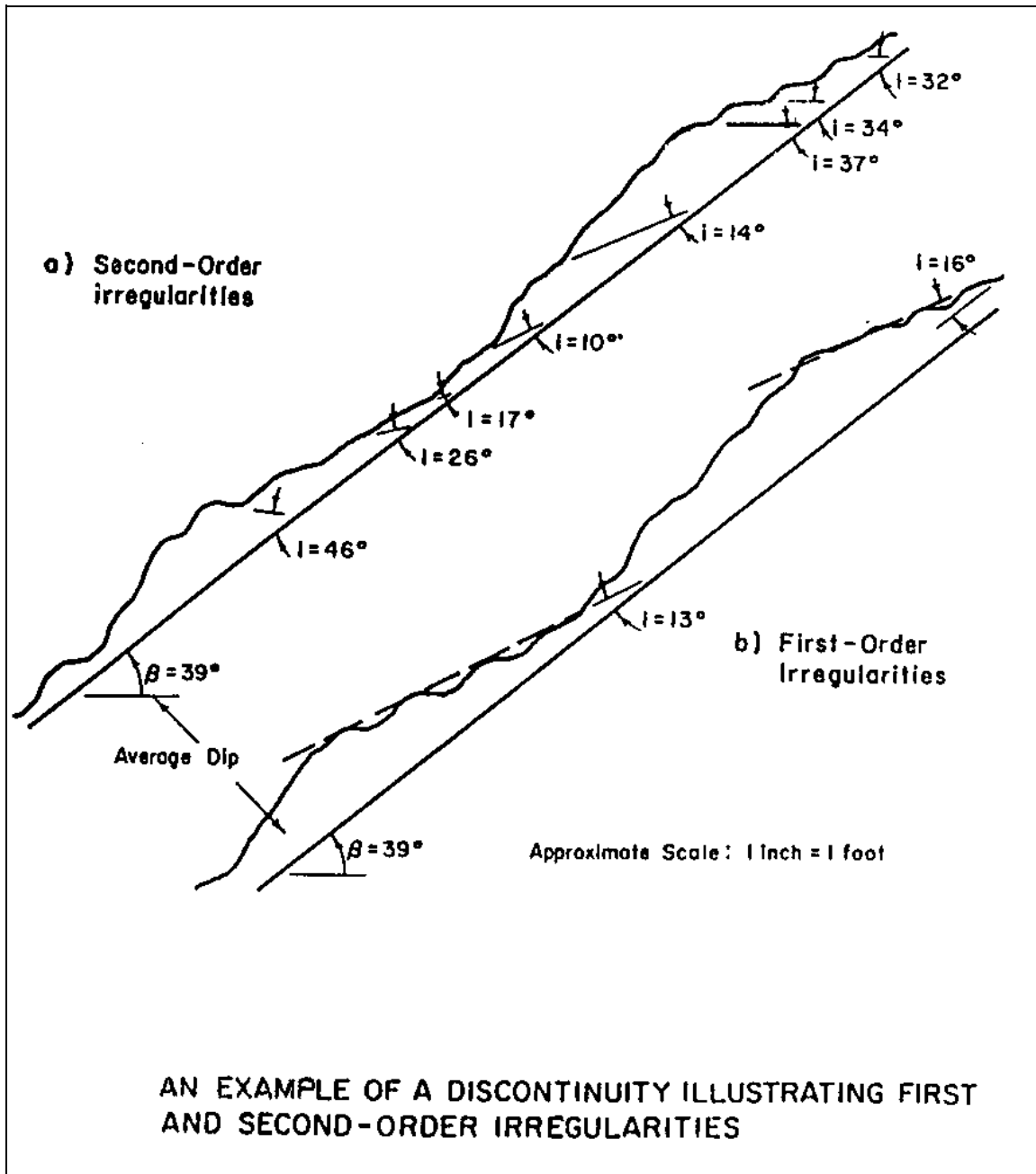
Figure 10-7. Diagram of asperity angle "i" measurement (Hendron, Cording, and Aiyer 1971)
