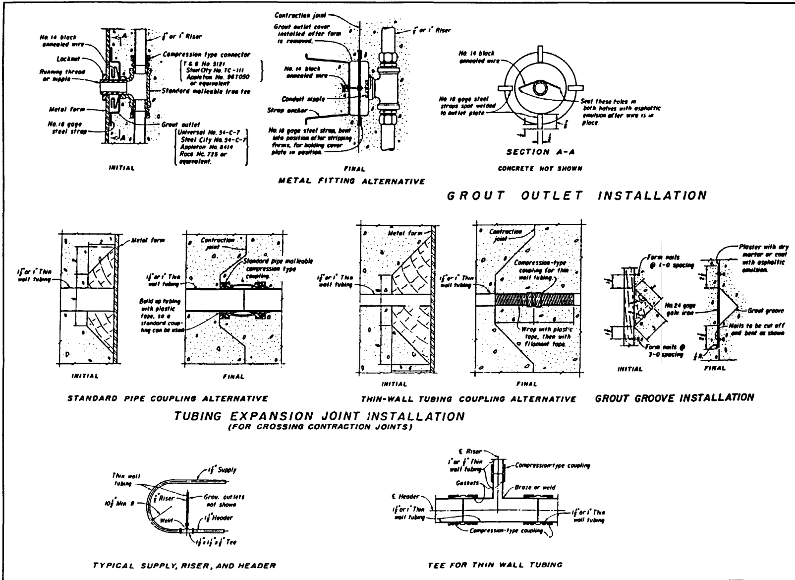
Figure 13-15. Example of grouting system details (USBR) (Continued)
