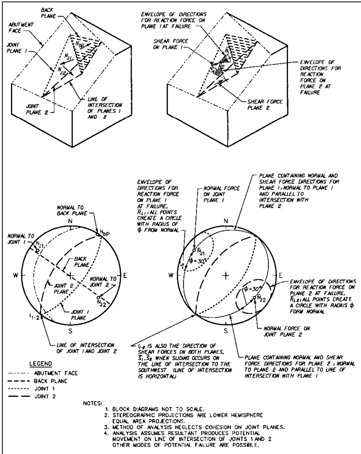
Figure 10-10. Illustration of both the vector and graphical stereonet technique of slope stability analysis from Portugues Dam Design Memorandum No. 24, (USAED, Jacksonville, 1990) (Continued)
