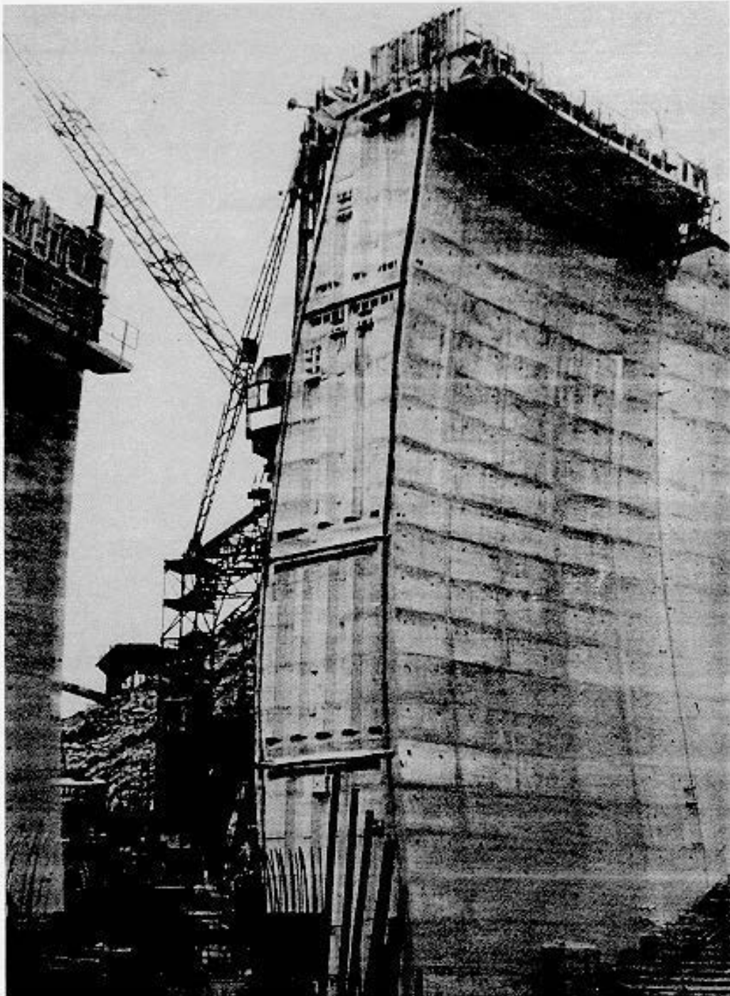
Figure 13-11. Vertical keys at monolith joints of Monar Dam, Scotland
