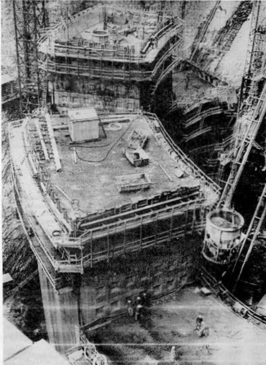
Figure 13-13. Waffle keys at the vertical monolith joints of Gordon Dam, Australia
