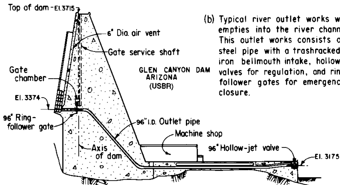
SECTION THRU RIVER OUTLETS (b)
