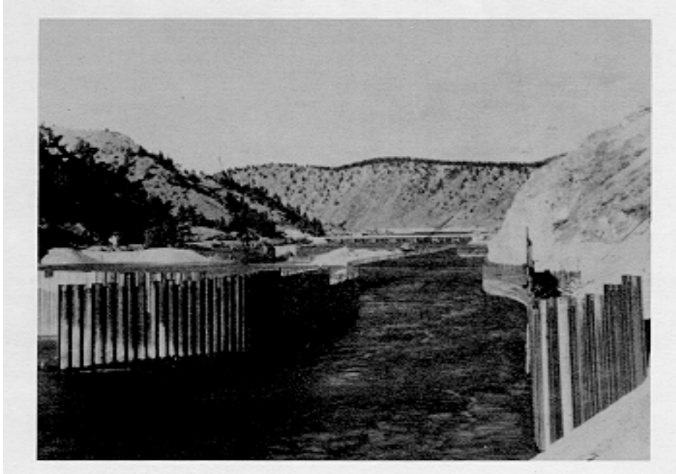
Figure 13-5. Complete diversion flume at Canyon Ferry damsite in use for first stage diversion (USBR)
