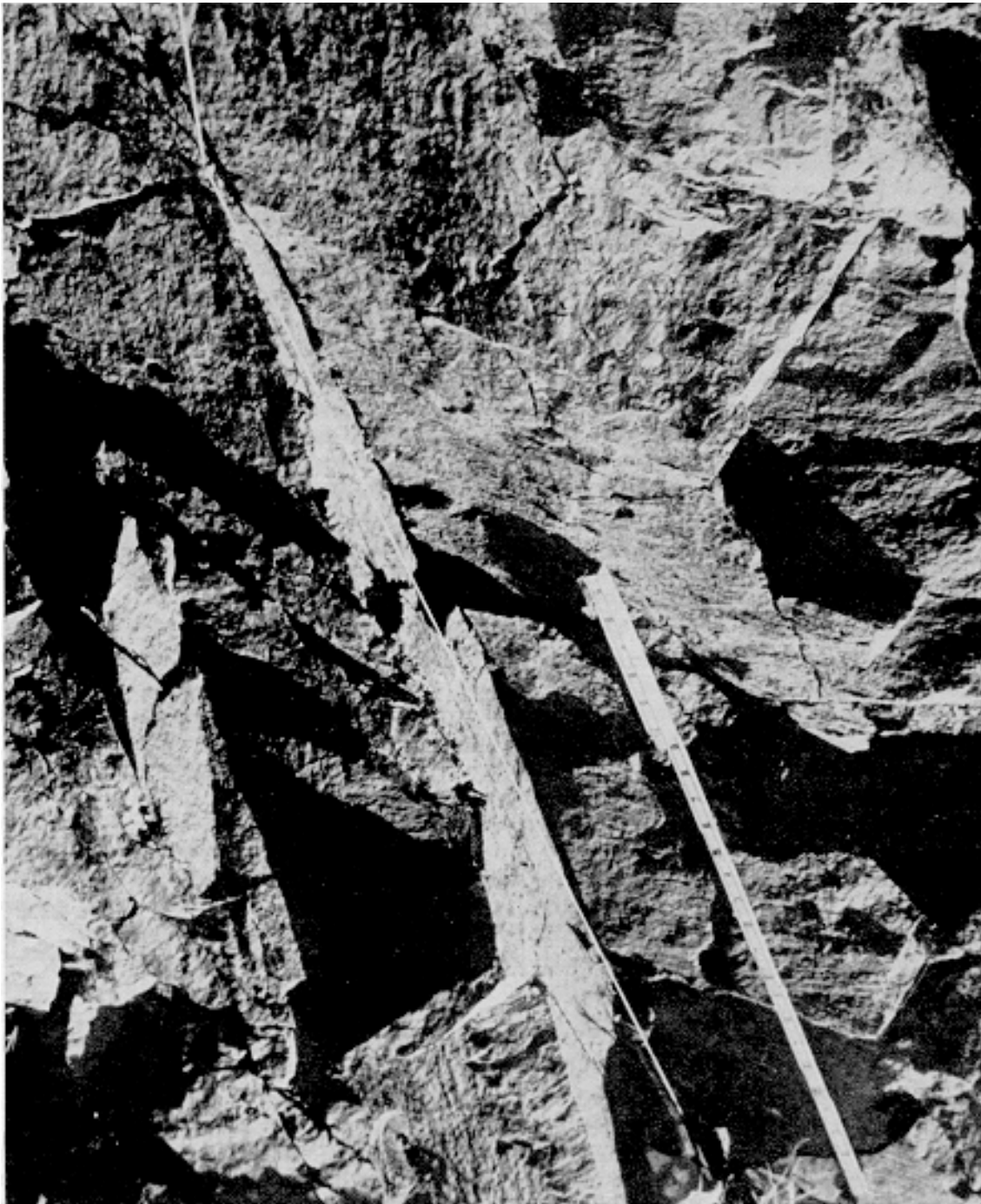
Figure 10-8. Picture of asperity angle "i" measured in the field utilizing a string line for orientation from Portugues Dam Design Memorandum No. 22 (USAED, Jacksonville, 1988b)
