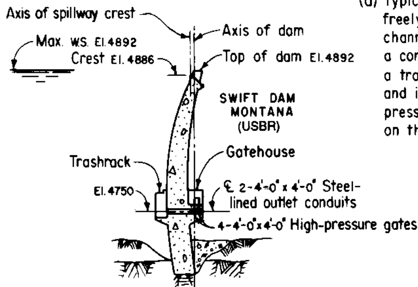
SECTION THRU RIVER OUTLETS (a)
