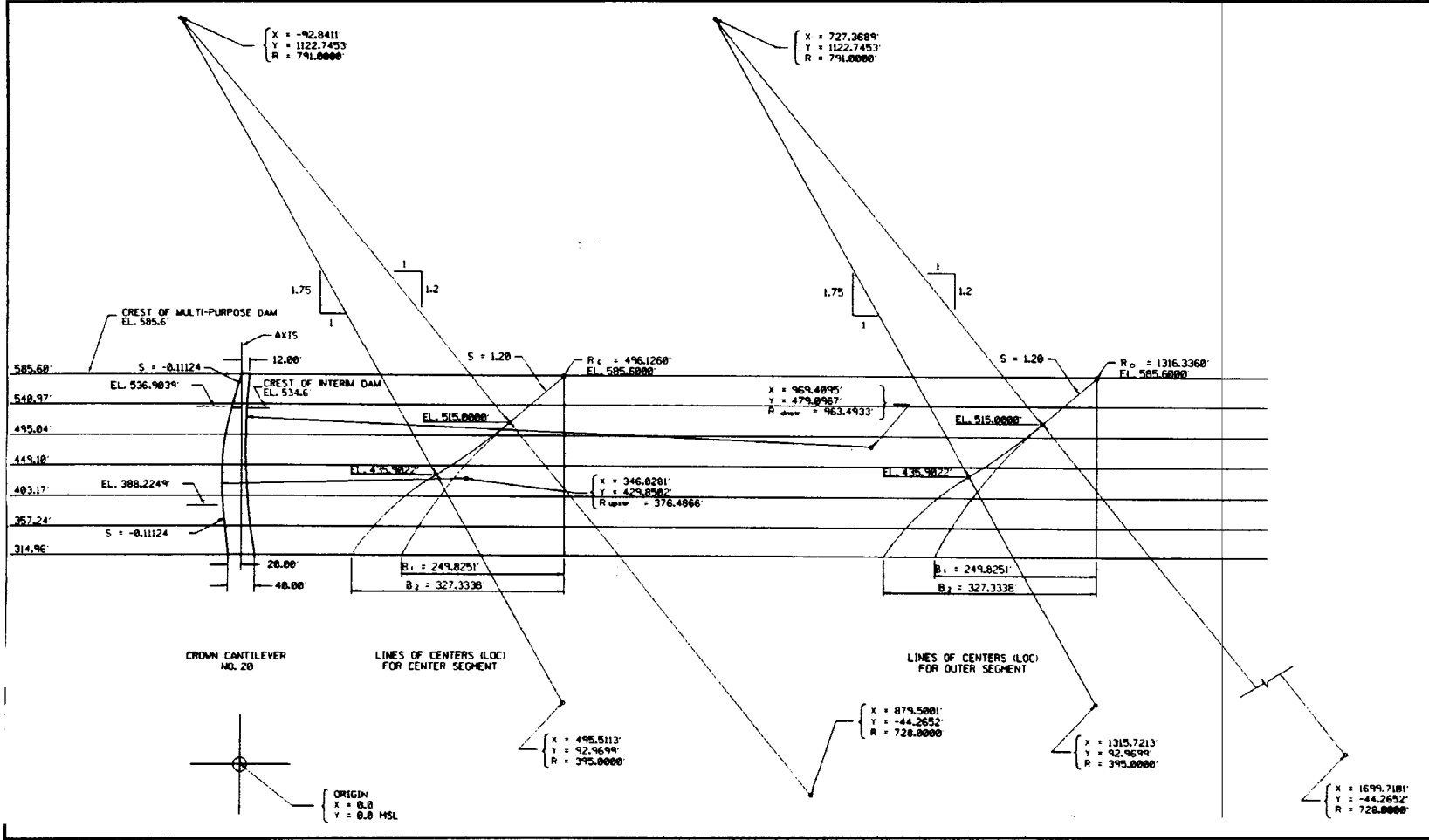
Figure 1-6. Section along reference plane of plane shown in Figure 1-5
