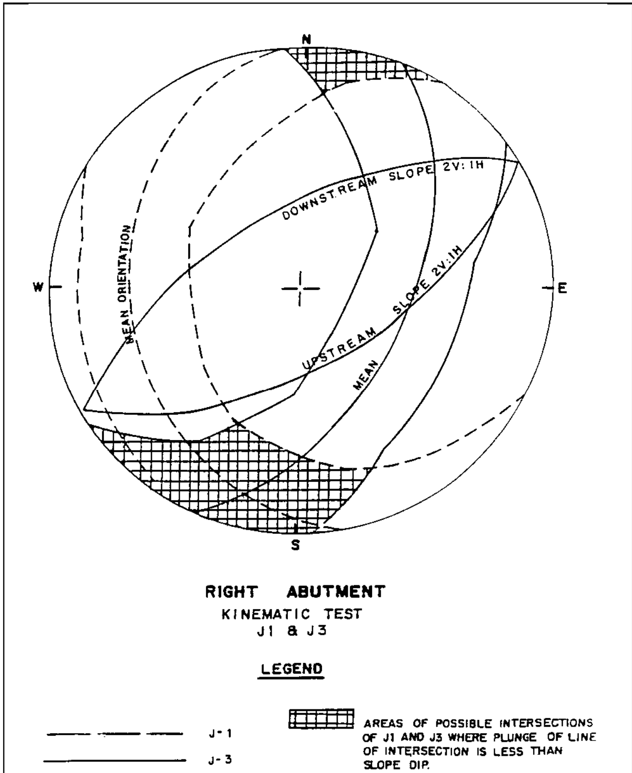
Figure 10-9. An equatorial angle stereonet plot showing two intersecting joint sets and two cut slopes demonstrating kinematic capability for failure from Portugues Dam Design Memorandum No. 24 (USAED, Jacksonville, 1990)
