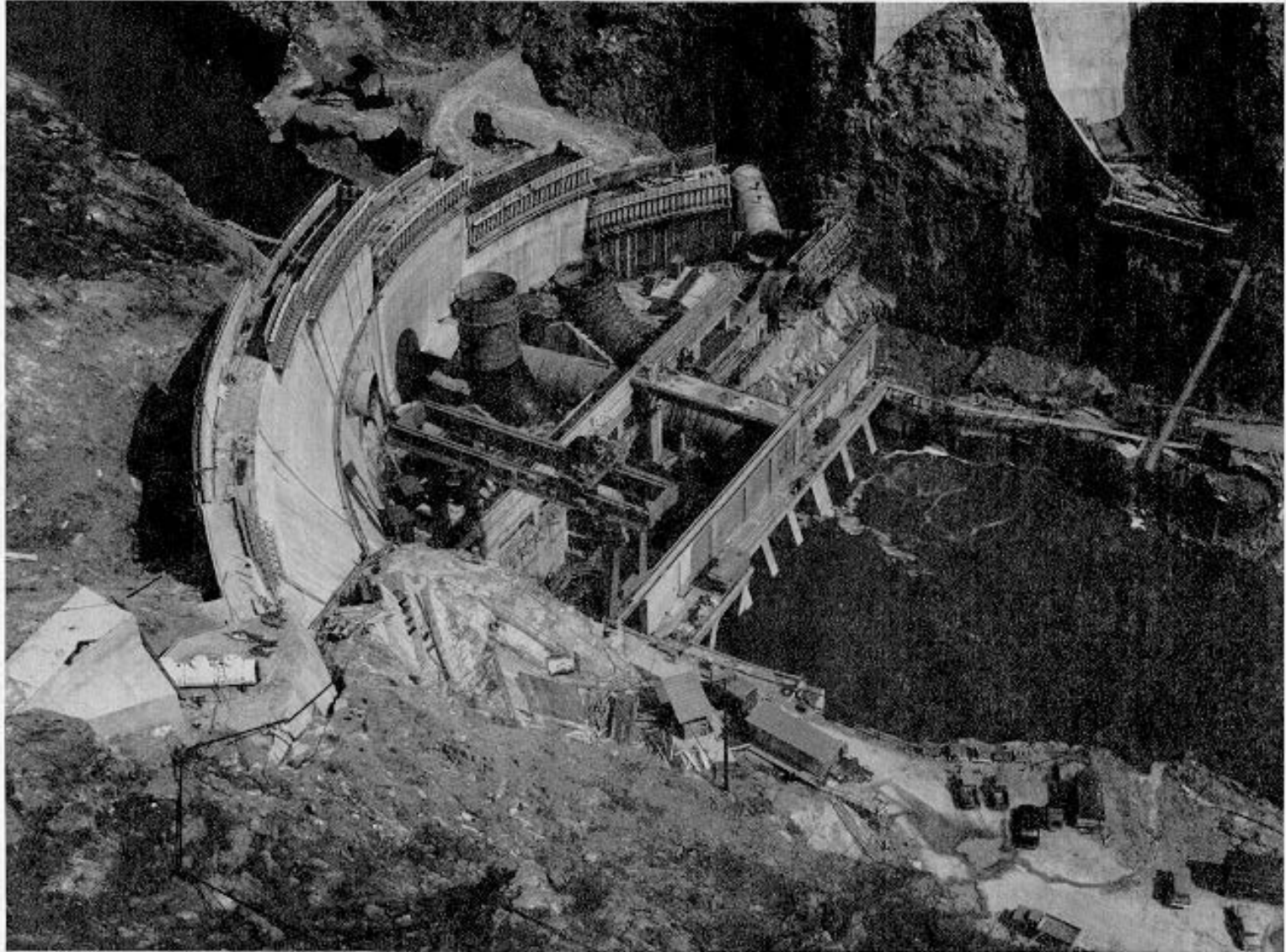
Figure 13-7. Sluice used in the Phase II diversion for Smith Mountain dam (photograph courtesy of Appalachian Power Company)
