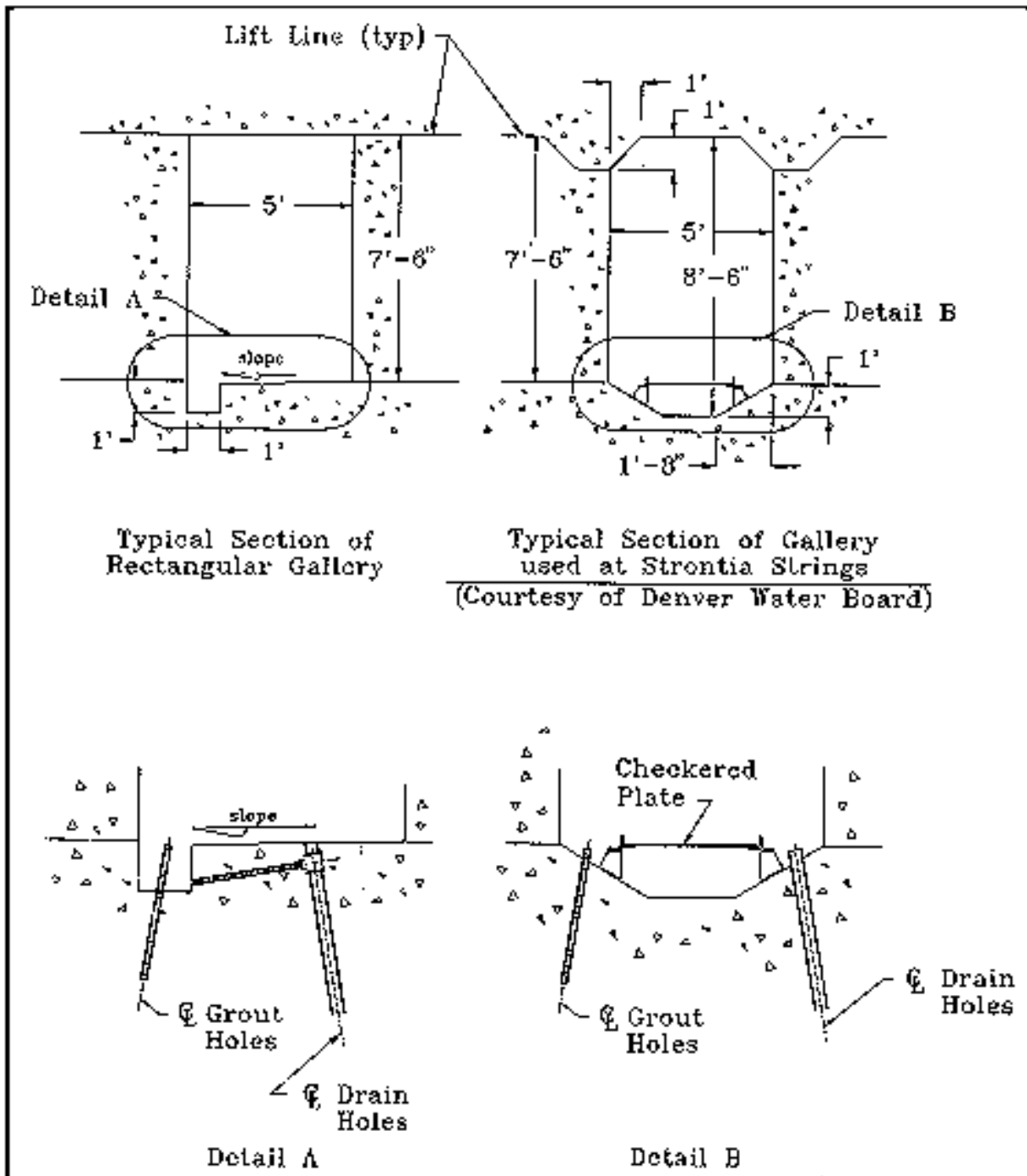
Figure 13-16. Typical gallery details
