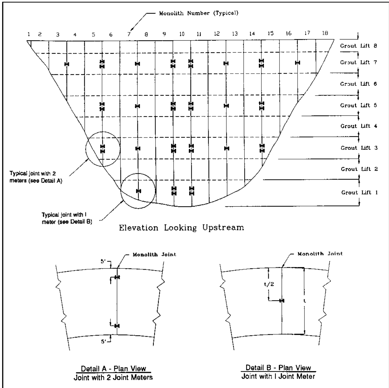
Figure 12-5. Layout for joint meters
