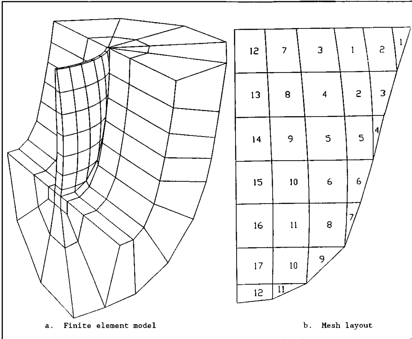
Figure 6-1. Finite element model of Morrow Point Dam and foundation
