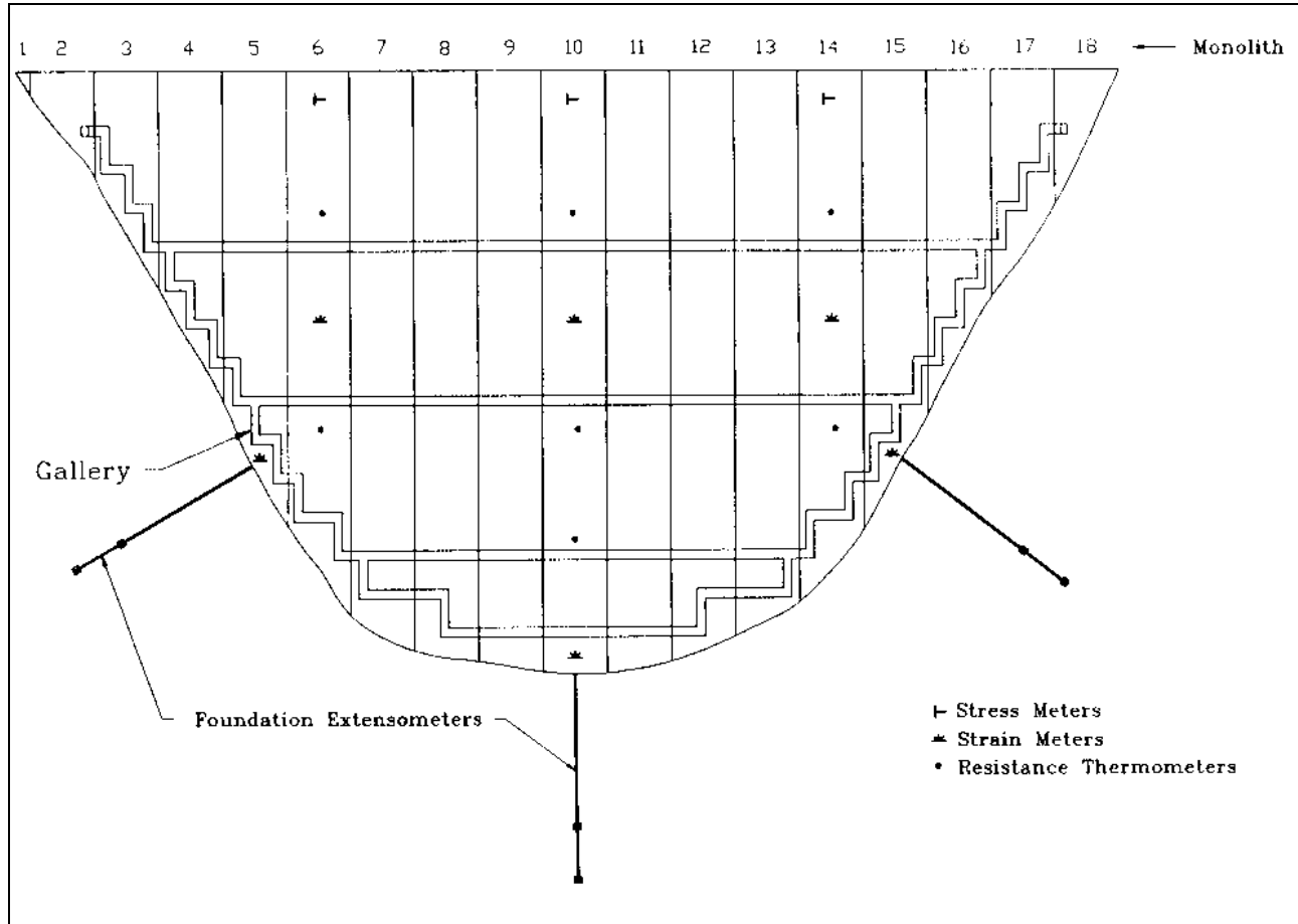
Figure 12-3. Recommended location of embedded instruments in arch dams (elevation looking upstream)
