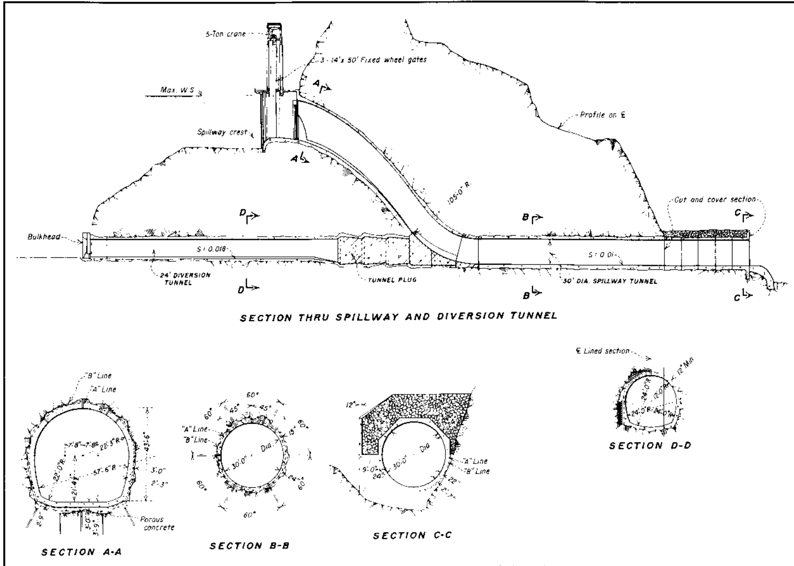
Figure 13-4. Typical diversion tunnel plug (USBR)
