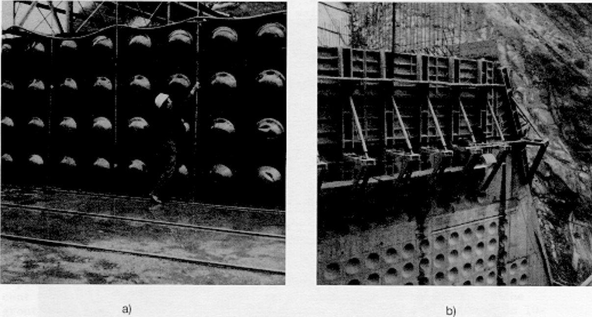
Figure 13-12. Dimple shear keys
