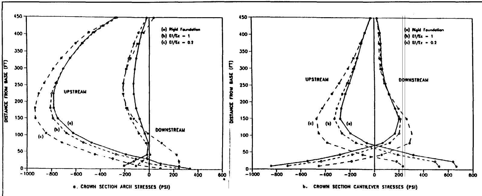
Figure 6-8. Crown section arch and cantilever stresses of Morrow Point Dam for different foundation-to-concrete modulus ratios with (c & d) and without (a & b) water loads acting on valley floor (Continued)
