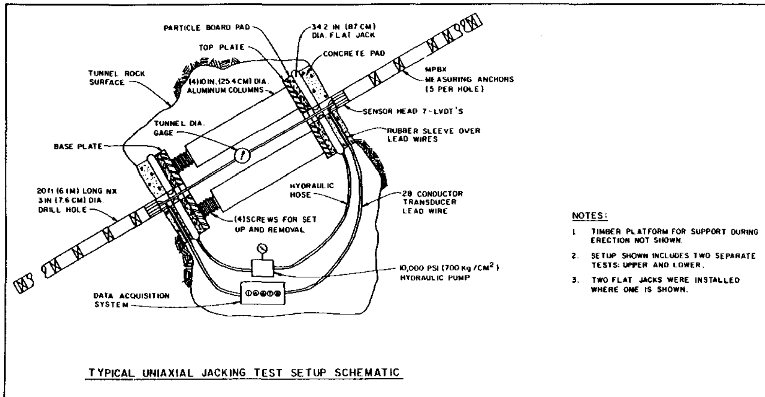
Figure 10-6. Uniaxial jacking test diagram from Portugues Dam Design Memorandum No. 22 (USAED, Jacksonville, 1988b)
