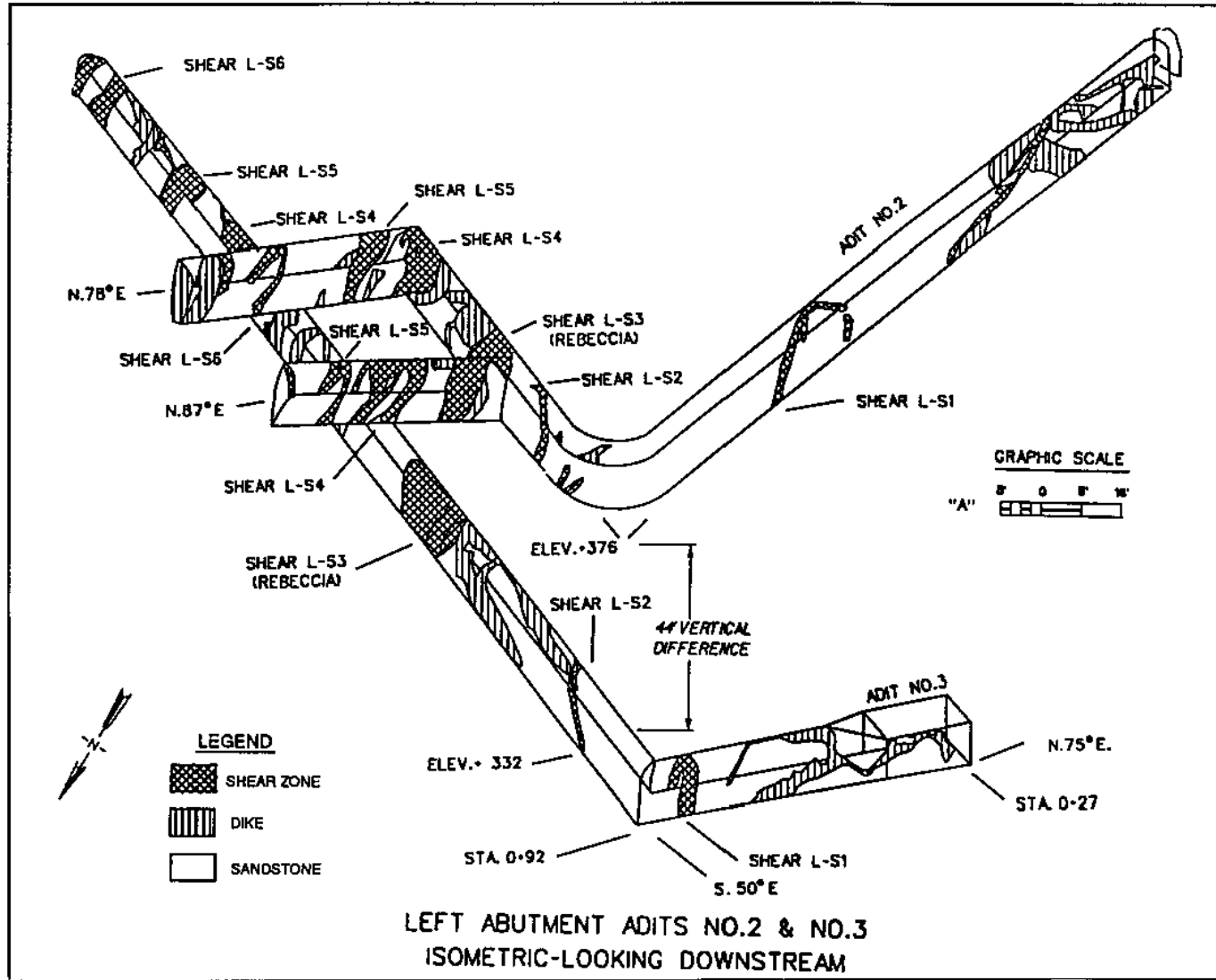
Figure 10-4. Adit periphery mapping isometric view from Portugues Dam Design Memorandum No. 22 (USAED, Jacksonville, 1988b)
