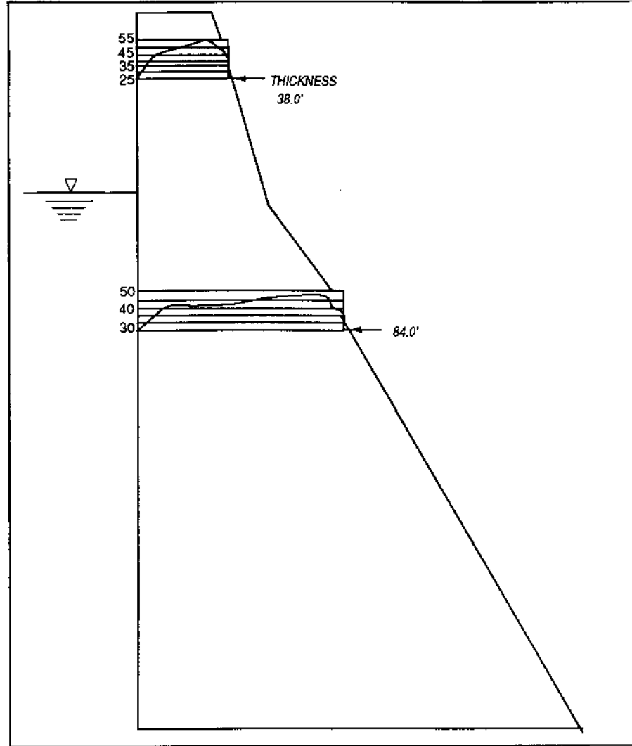
Figure 8-2. Measured temperature distributions in December for a relatively thick dam
