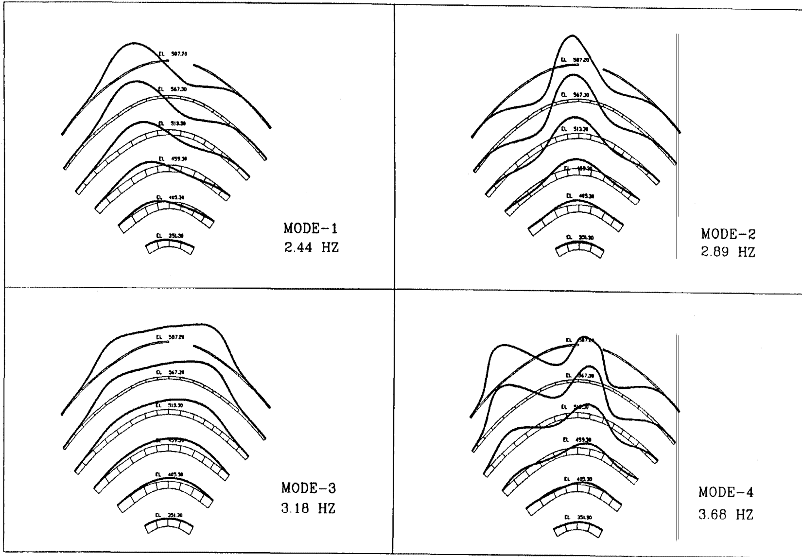
Figure 7-4. Four lowest vibration modes of Portugues Arch Dam
