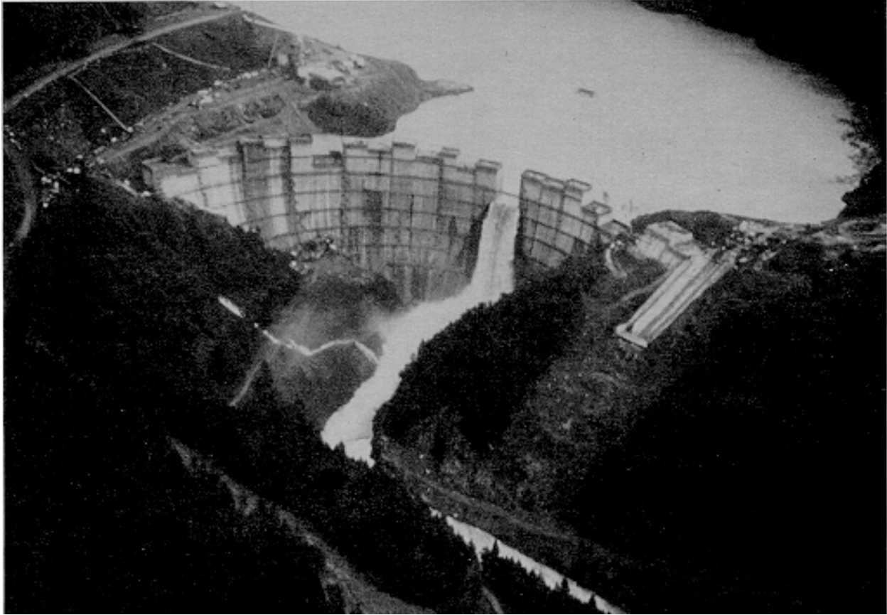
Figure 13-8. Aerial view of partially completed New Bullards Bar Dam in California showing water flowing over the low blocks (photograph courtesy of Yuba County Water Agency)
