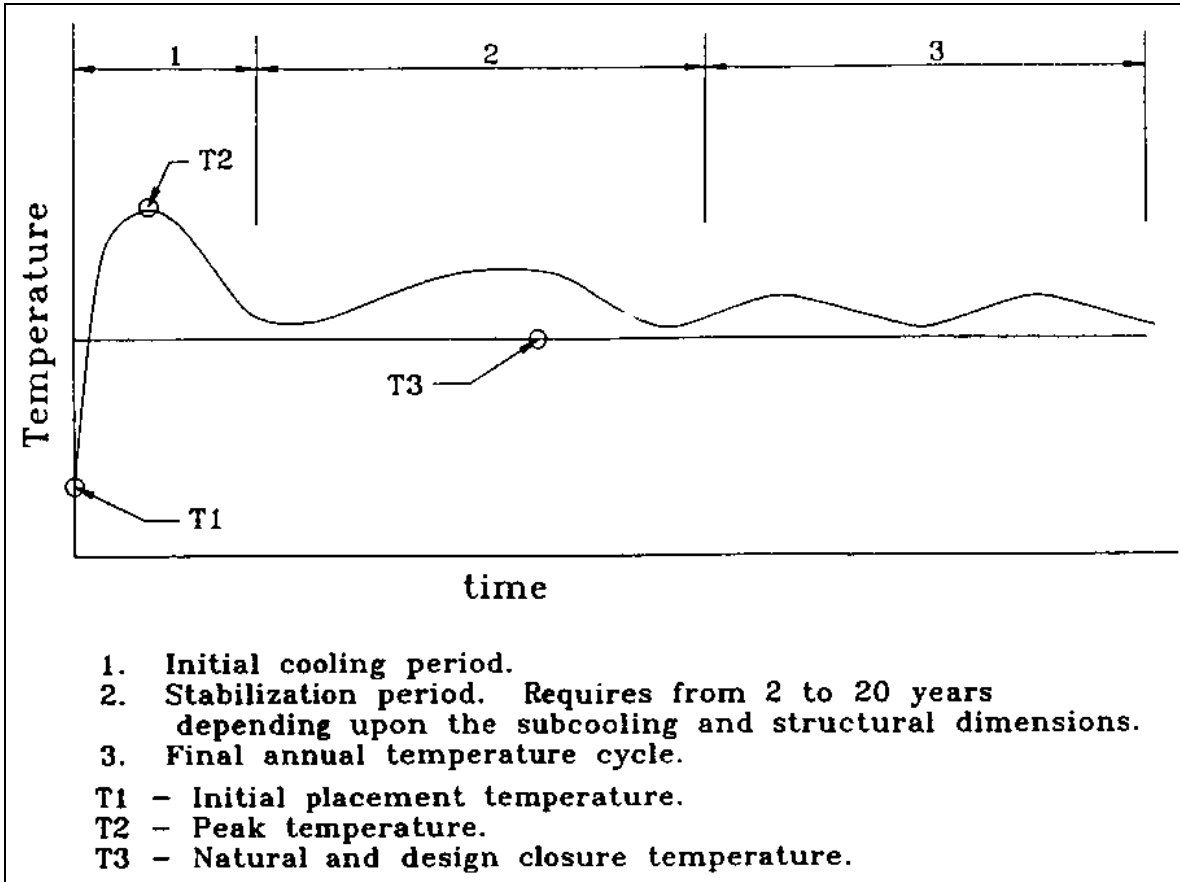
Figure 8-10. Temperature history for artificially cooled concrete where monolith joints are not grouted
