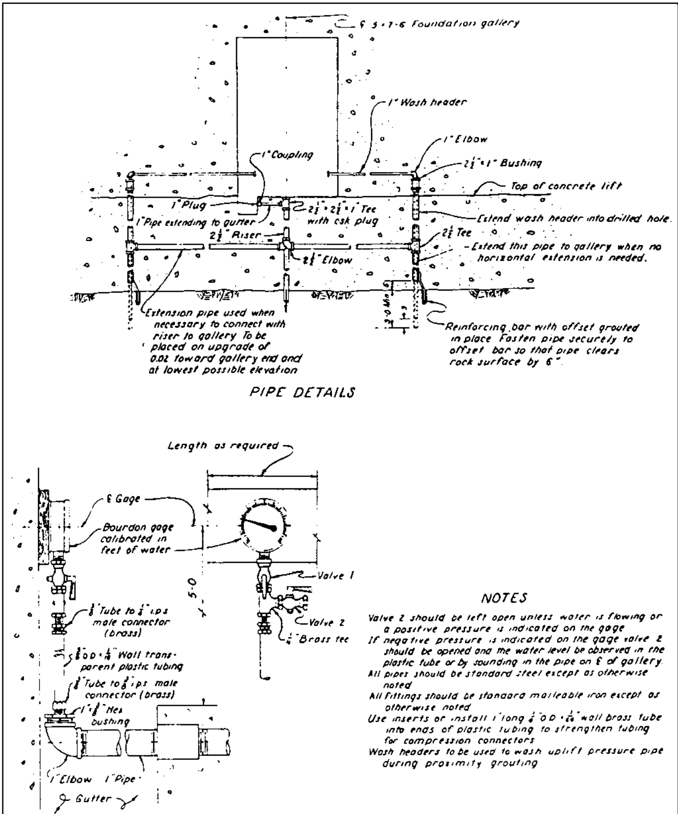
Figure 12-2. Typical Bourdon gauge installation (USBR 1987)
