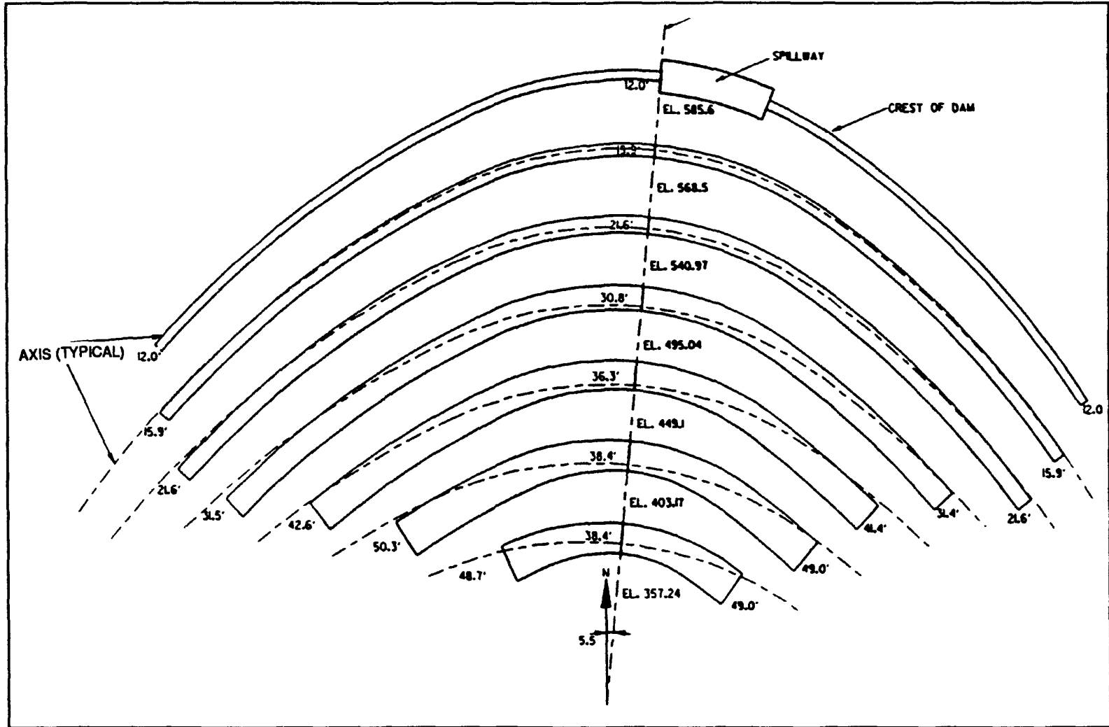
Figure 5-15. Arch sections
