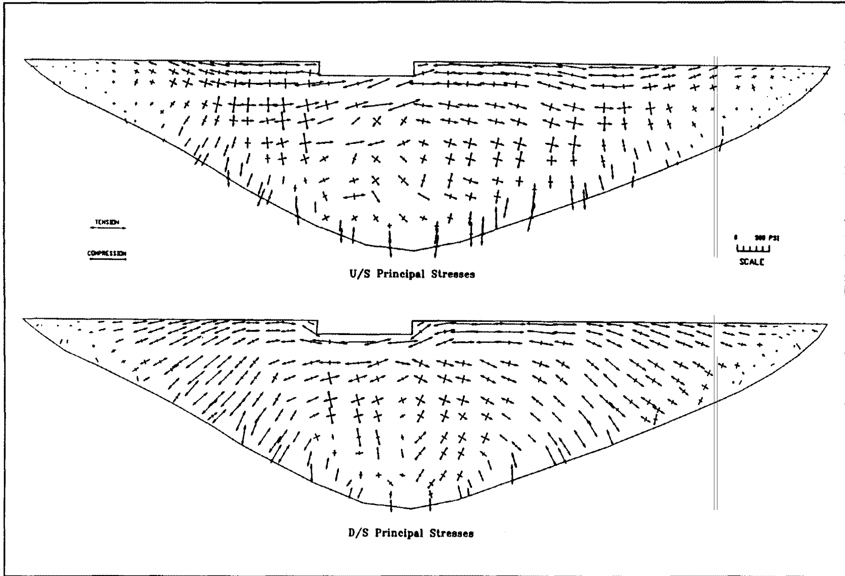
Figure 7-8. Envelope of maximum principal stresses with their corresponding perpendicular pair
