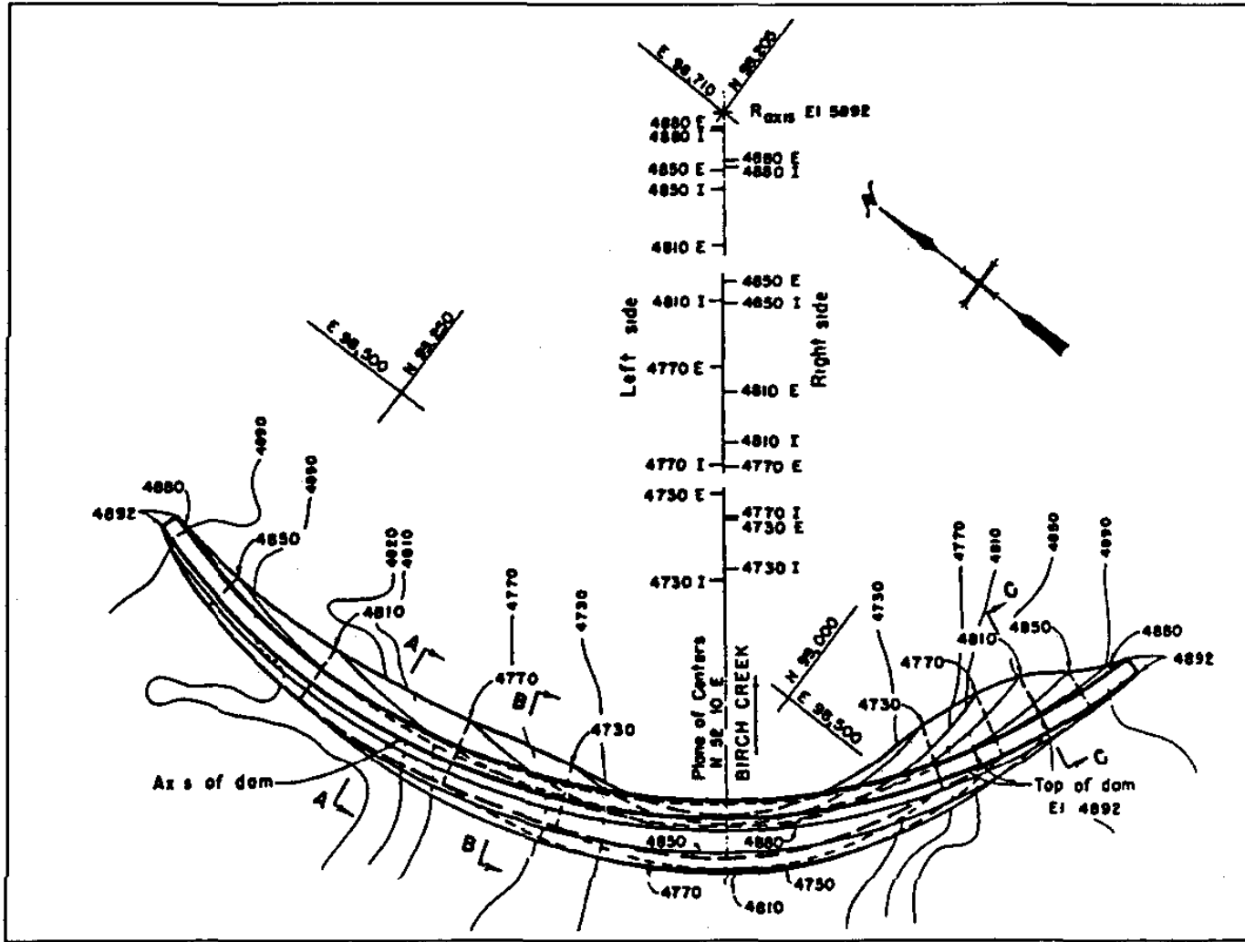
Figure 1-4. Typical two-centered variable-thickness arch dam in a nonsymmetrical site
