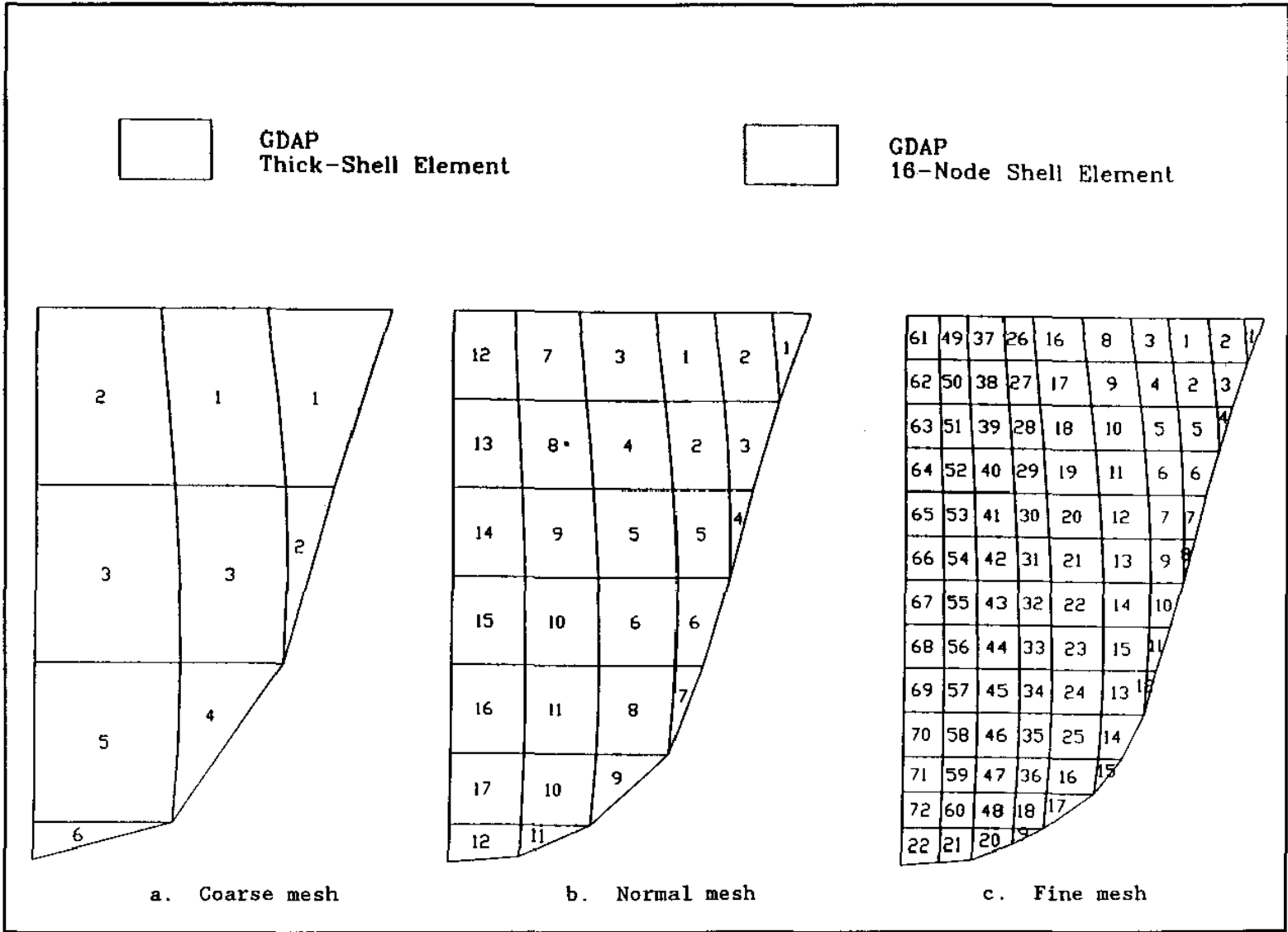
Figure 6-2. Alternative meshes for Morrow Point Dam
