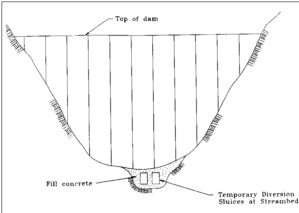
Figure 13-3. Diversion sluices through concrete pad at the base of a dam
