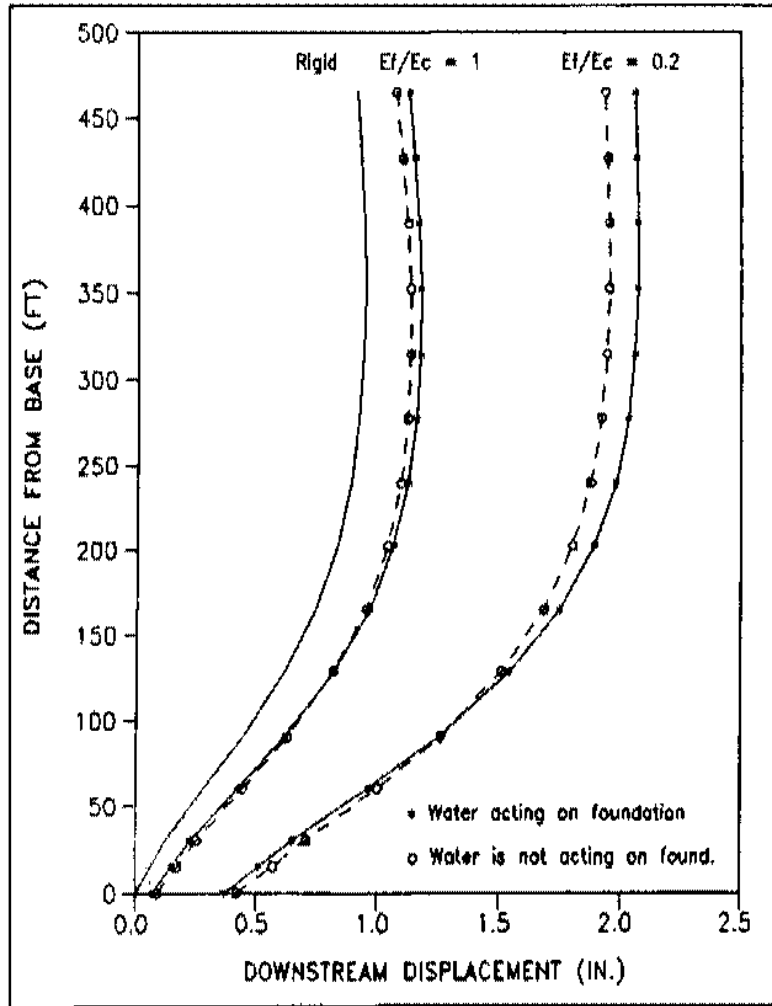
Figure 6-6. Crown section displacements of Morrow Point Dam for different foundation-to-concrete modulus ratios with and without water acting on valley floor
