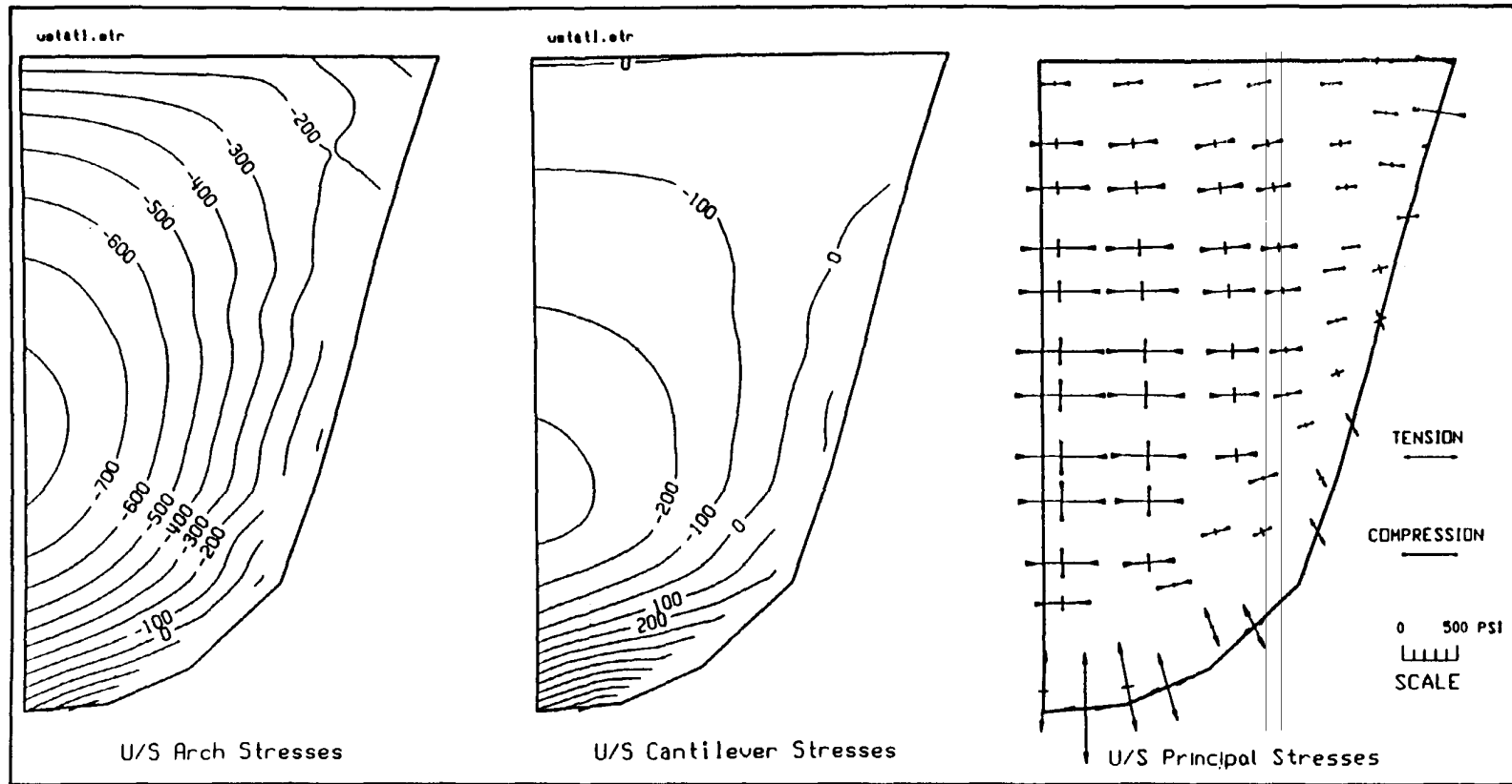
Figure 6-9. Arch and cantilever stress contours and vector plot of principal stresses for upstream face of Morrow Point Dam
