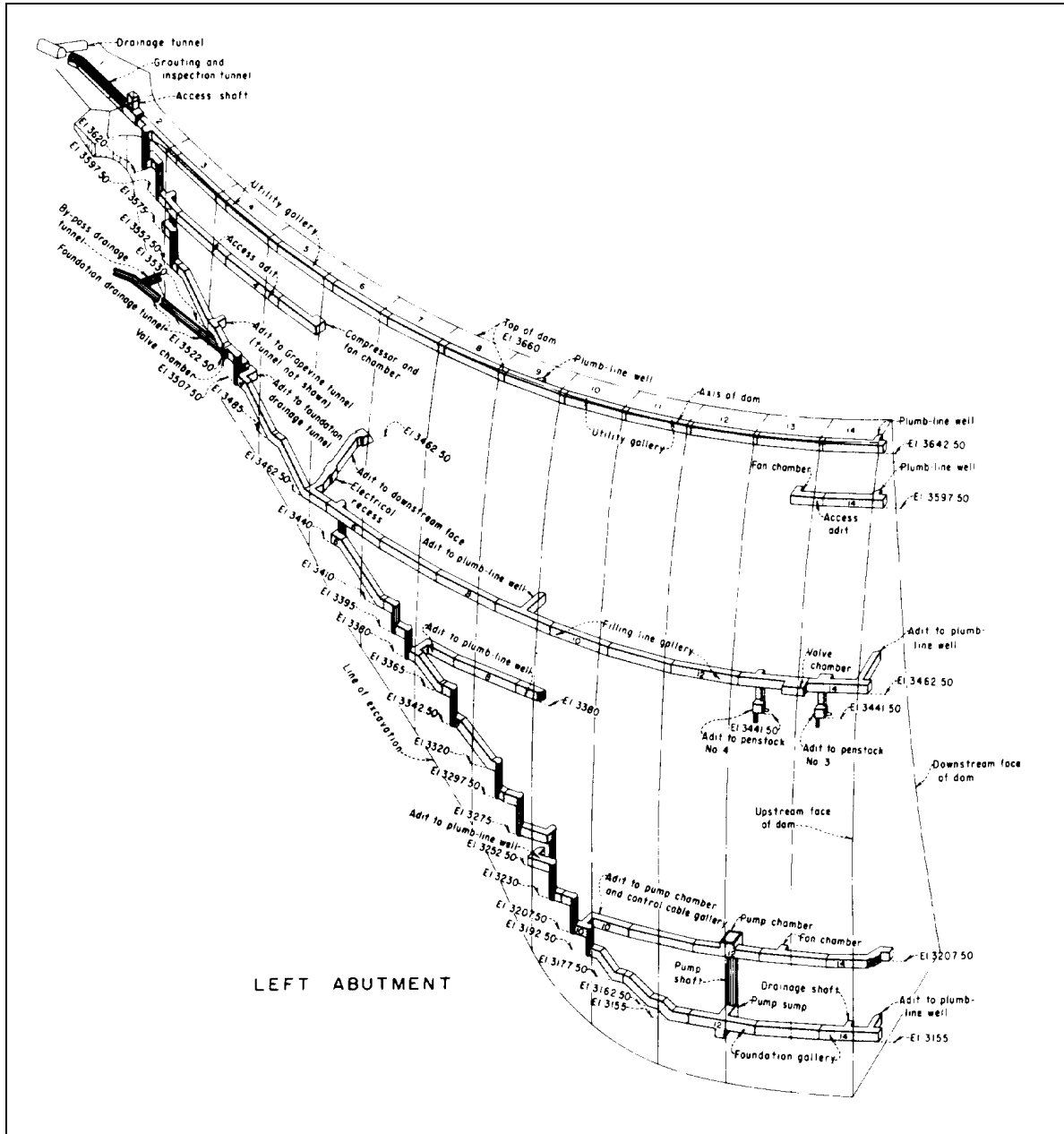
Figure 13-17. Left abutment gallery system for Yellowtail Dam (USBR)
