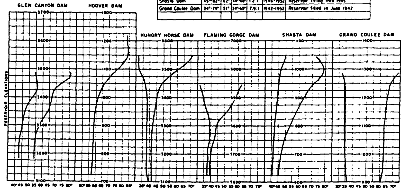
Figure 8-3. Typical reservoir temperature distributions (USBR)
