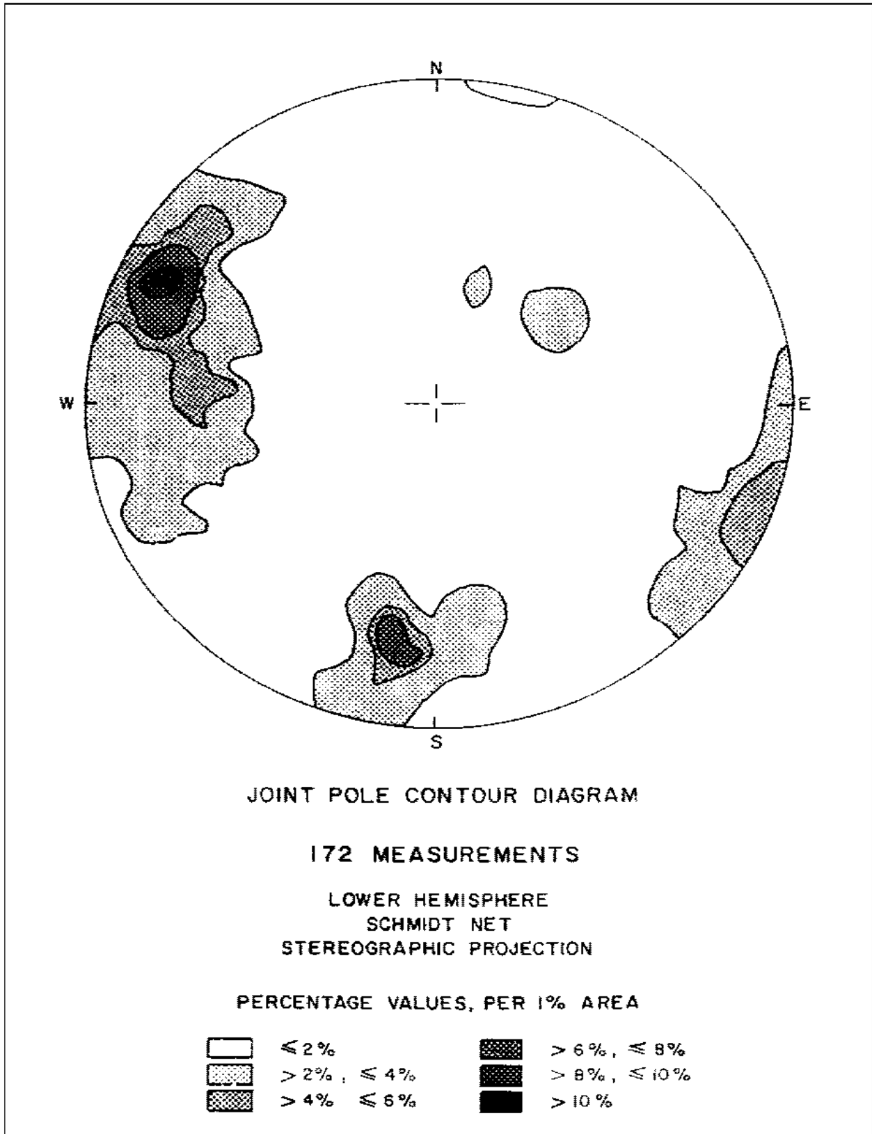
Figure 10-5. Equal area joint pole contour diagram from Portugues Dam Design Memorandum No. 22 (USAED, Jacksonville, 1988b)
