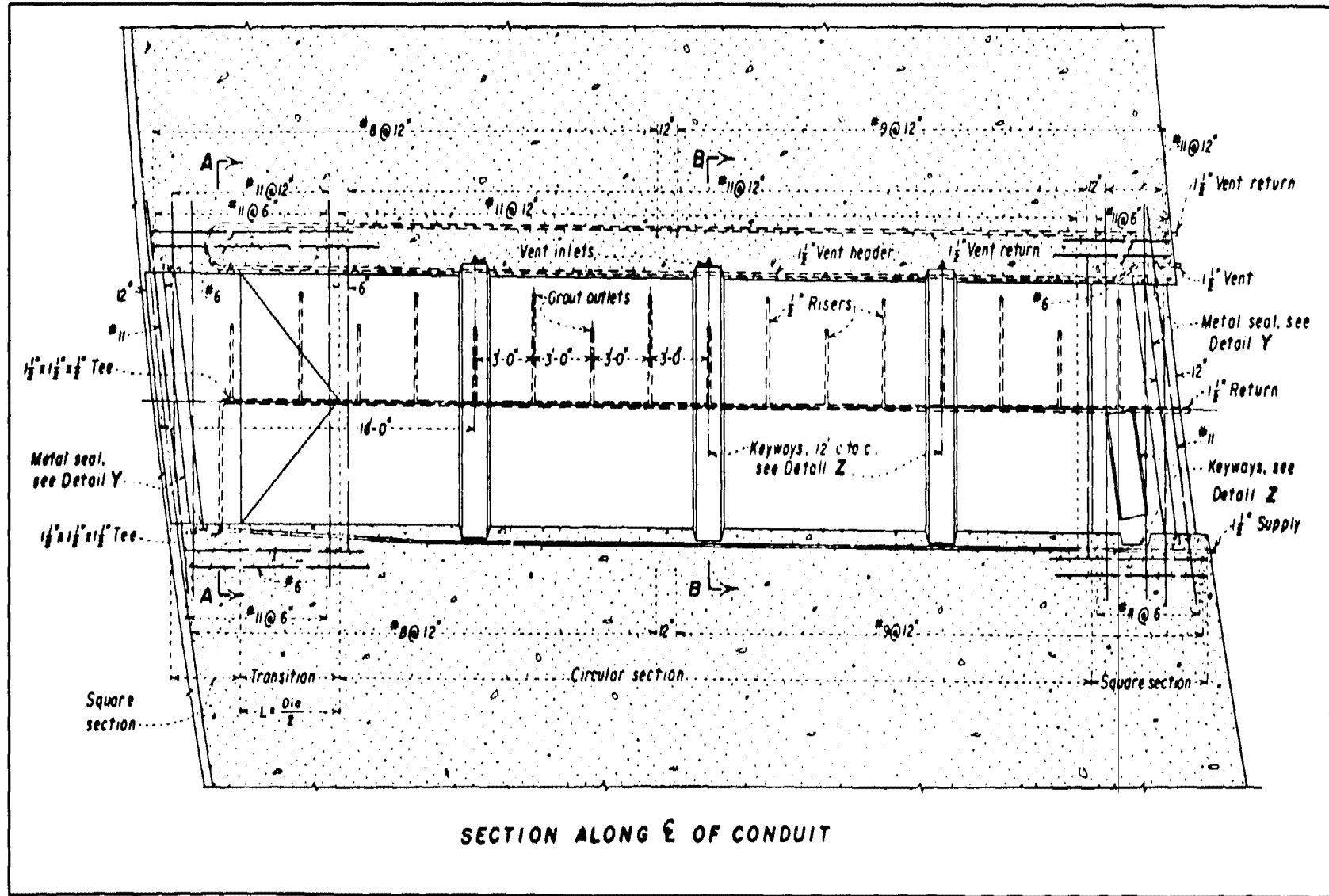
Figure 13-9. Diversion conduit through Morrow Point Dam (USBR) (Continued)
