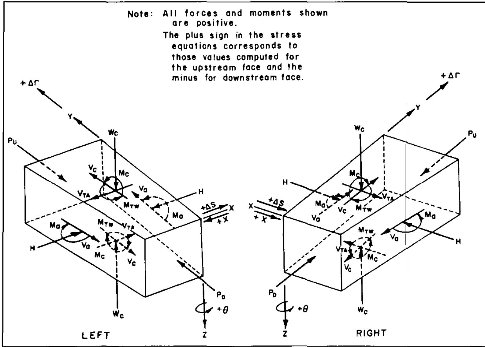
Figure 5-13. Sign convention for arch computations in ADSAS
