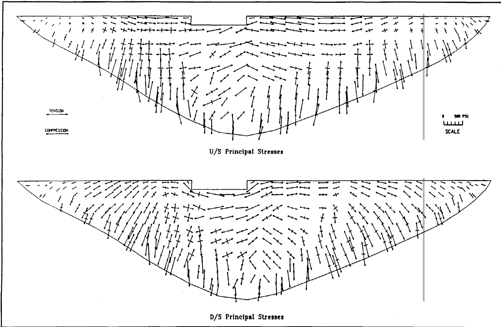
Figure 7-9. Envelope of maximum-minimum principal stresses with their corresponding perpendicular pair
