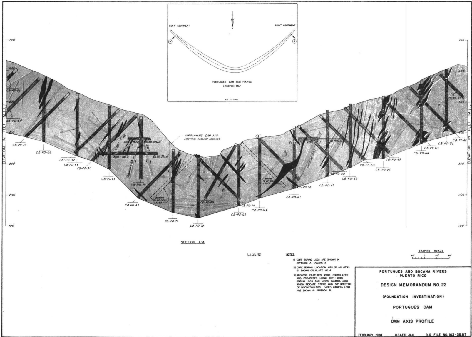
Figure 10-2. Arch dam boring profile from Portugues Dam Design Memorandum No. 22 (USAED, Jacksonville, 1988b)
