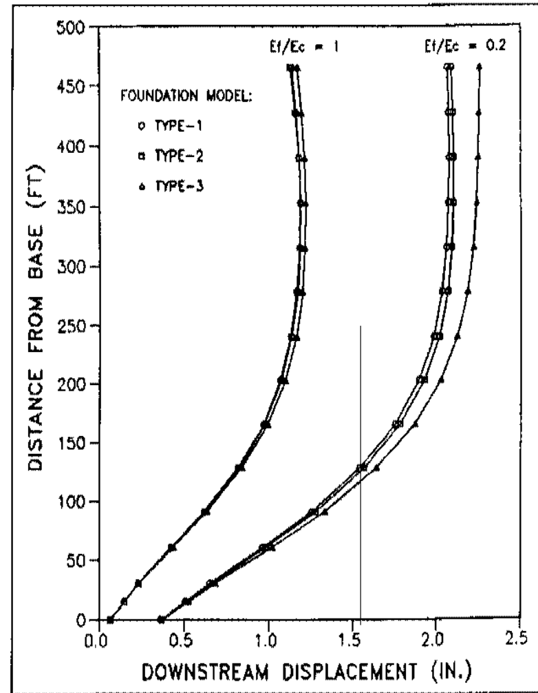
Figure 6-7. Crown section displacements of Morrow Point Dam for two foundation-to-concrete modulus ratios and for three foundation mesh types
