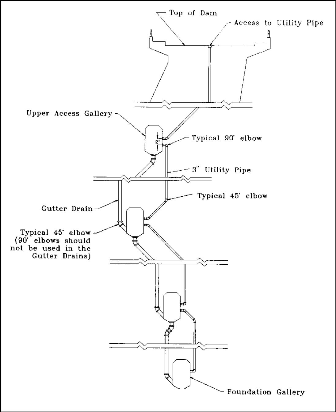
Figure 13-19. Details of gutter drains and utility piping
