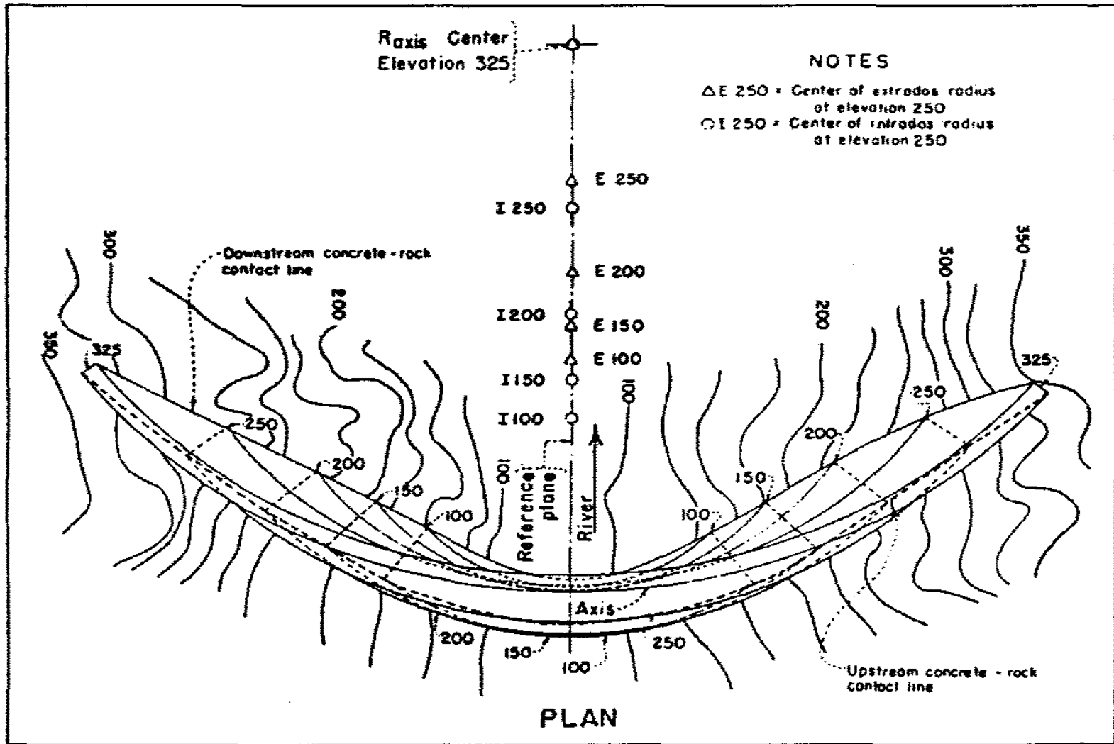
Figure 1-3. Typical single-center variable thickness arch dam in a symmetrical site
