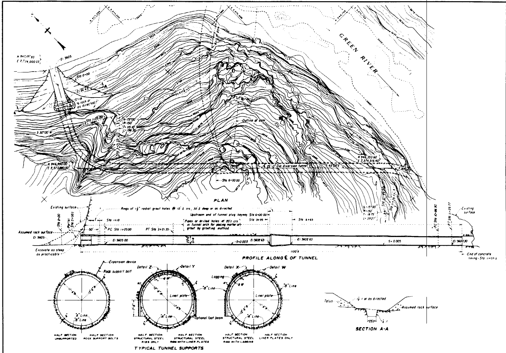
Figure 13-2. Diversion tunnel for Flaming Gorge Dam (USBR)
