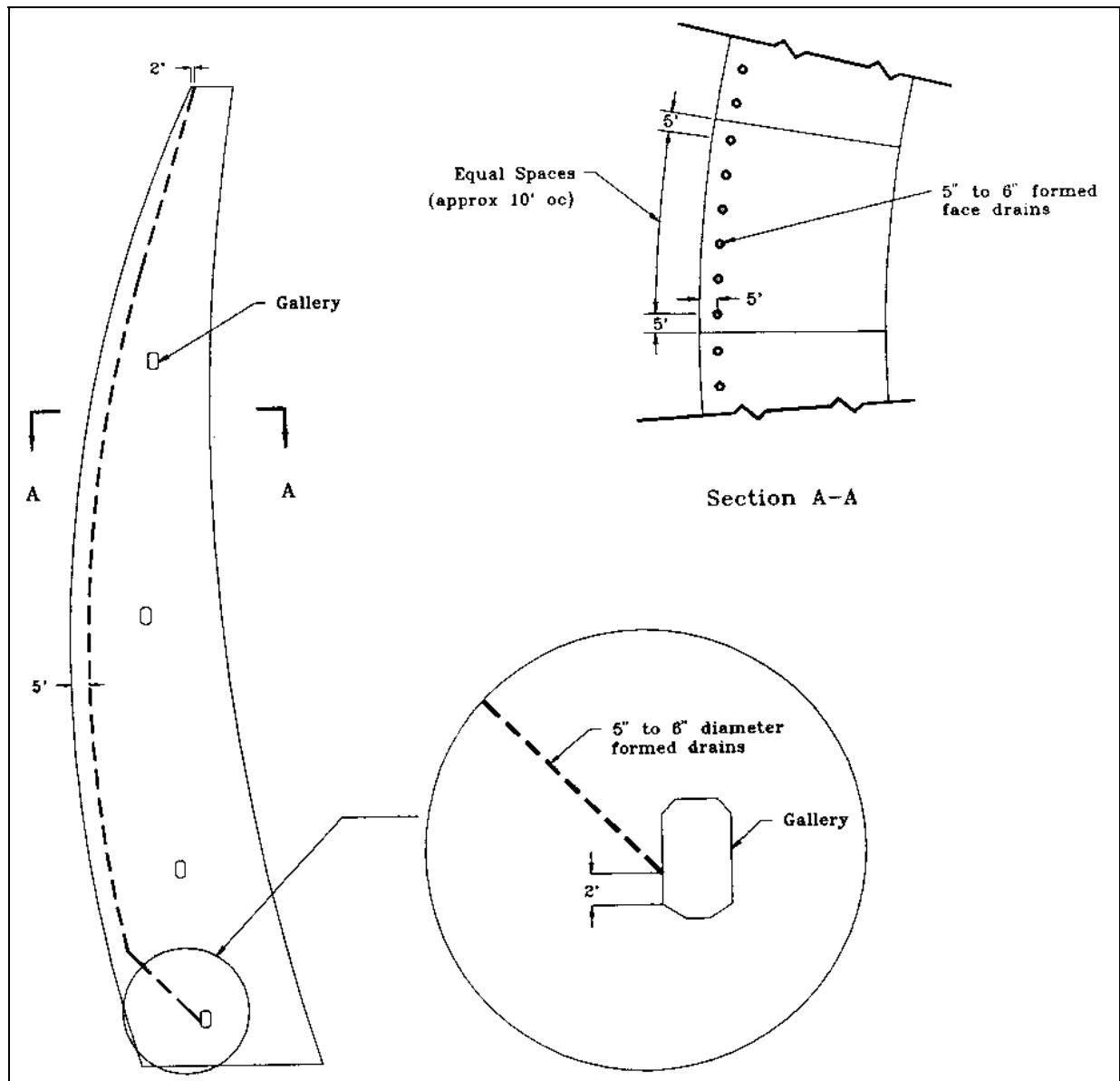
Figure 13-18. Details of face drains
