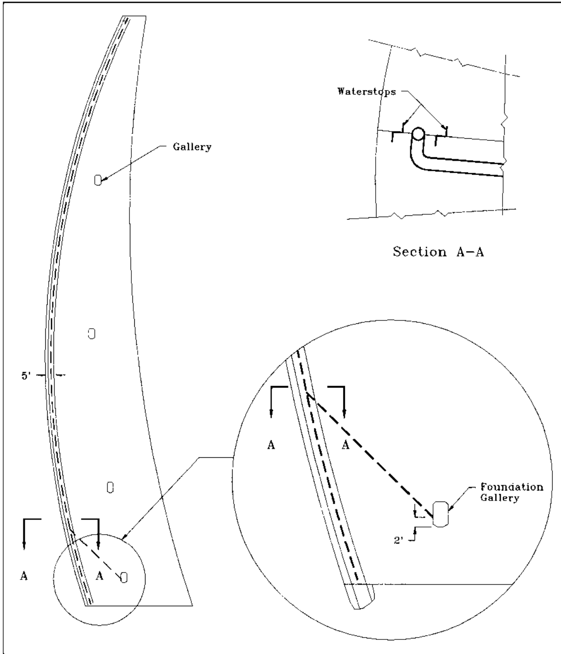
Figure 13-20. Details of joint drains
