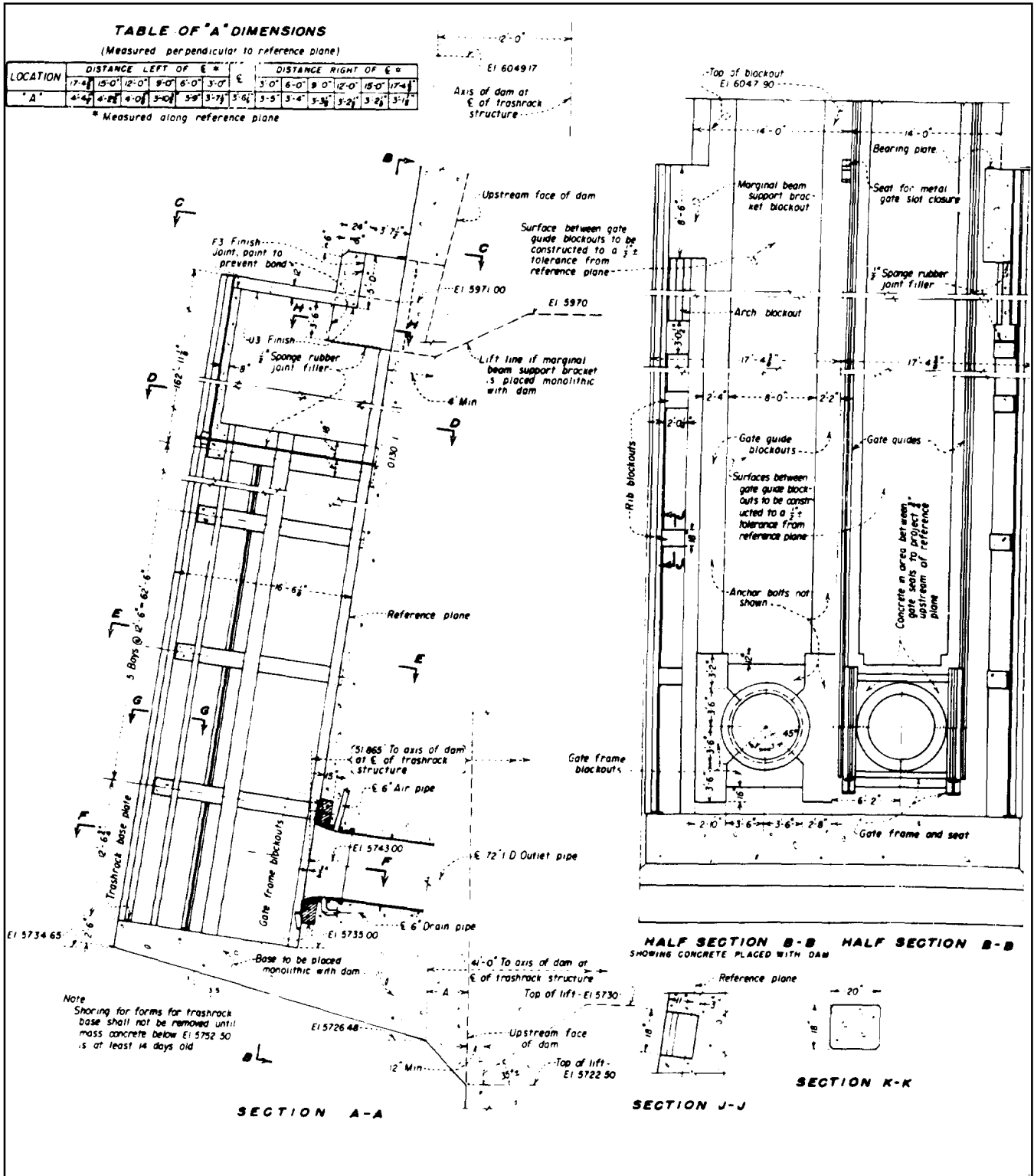
Figure 3-8. Typical river outlets trashrack structure (USBR)
