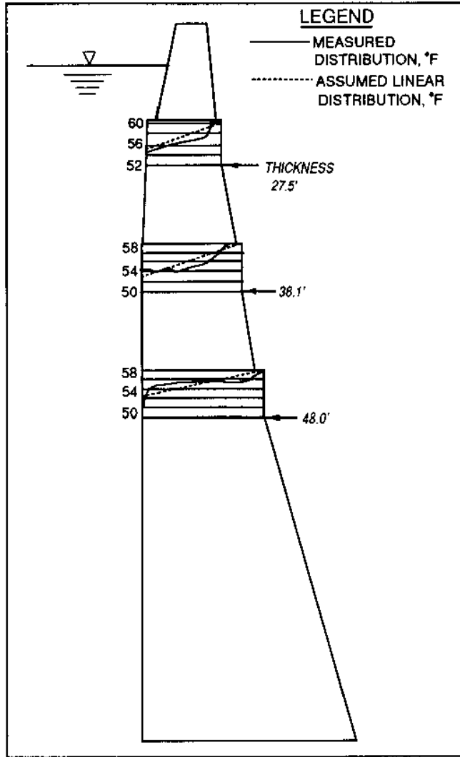
Figure 8-1. Measured temperature distributions in March for a relatively thin dam
