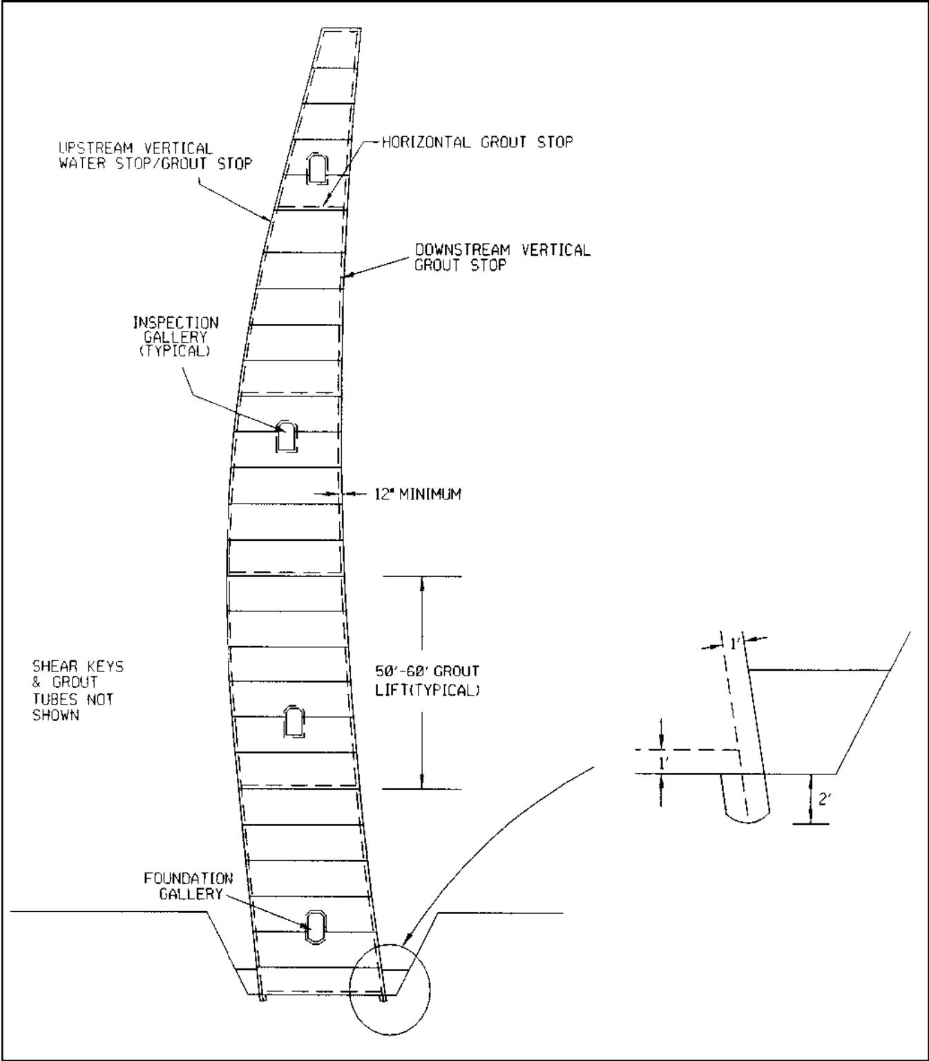
Figure 13-10. Water stop and grout stop details
