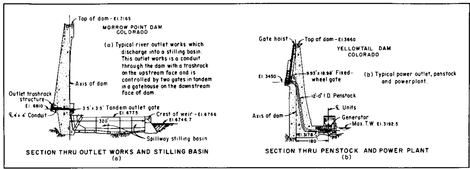
Figure 3-9. Typical river outlet works and power outlet (USBR)
