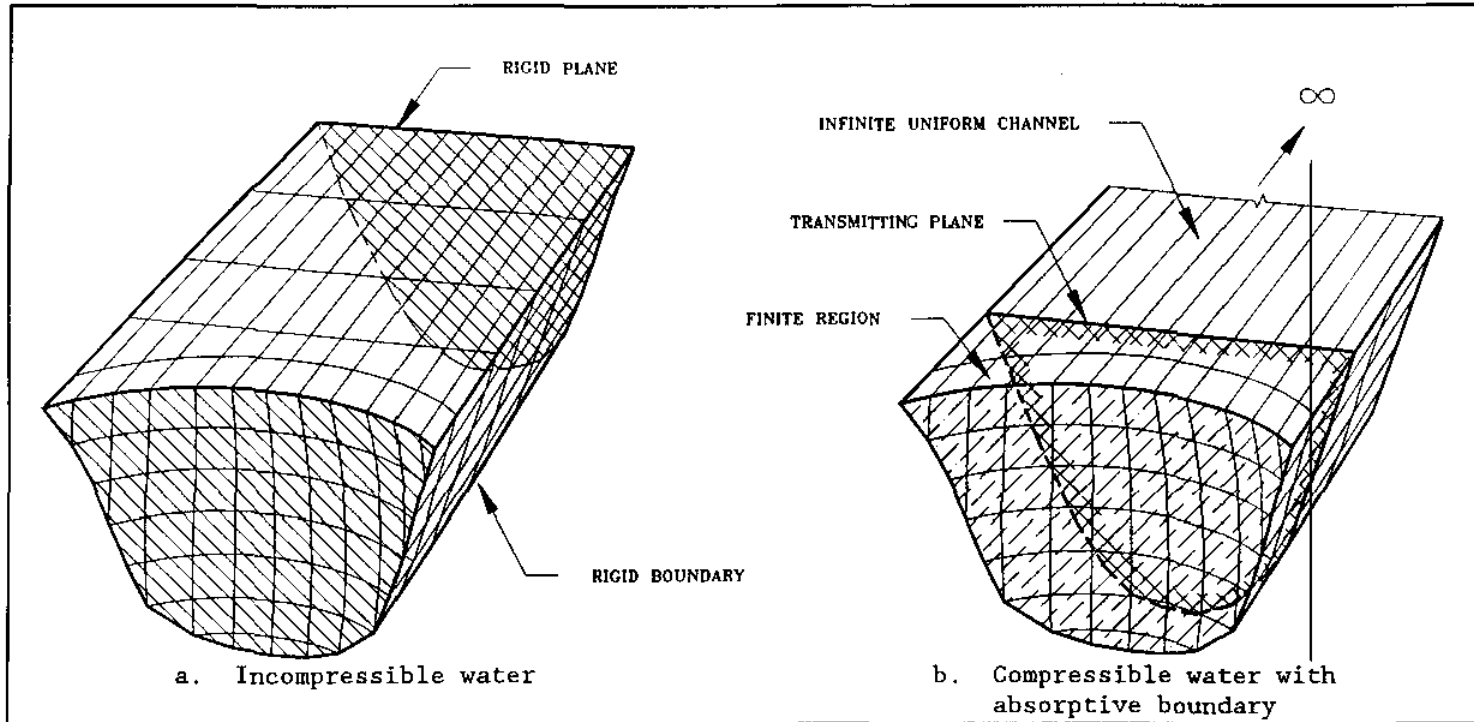
Figure 7-3. Finite element models of fluid domain with and without water compressibility
