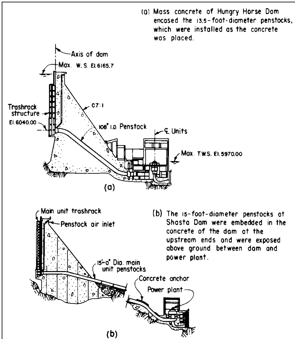
Figure 3-10. Typical penstock installations (USBR)
