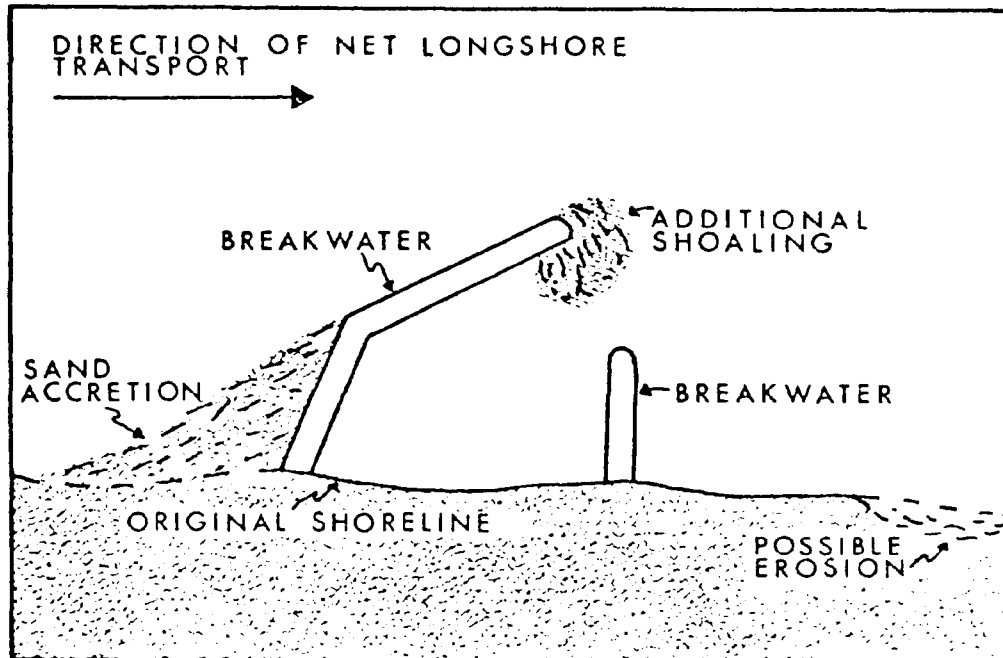
ATTACHED BREAKWATER
