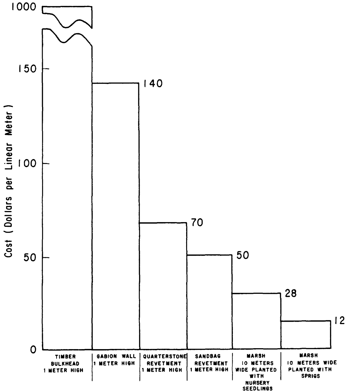
Figure 6-3. Cost comparison of alternative erosion control measures (after Knutson and Woodhouse 1983)
