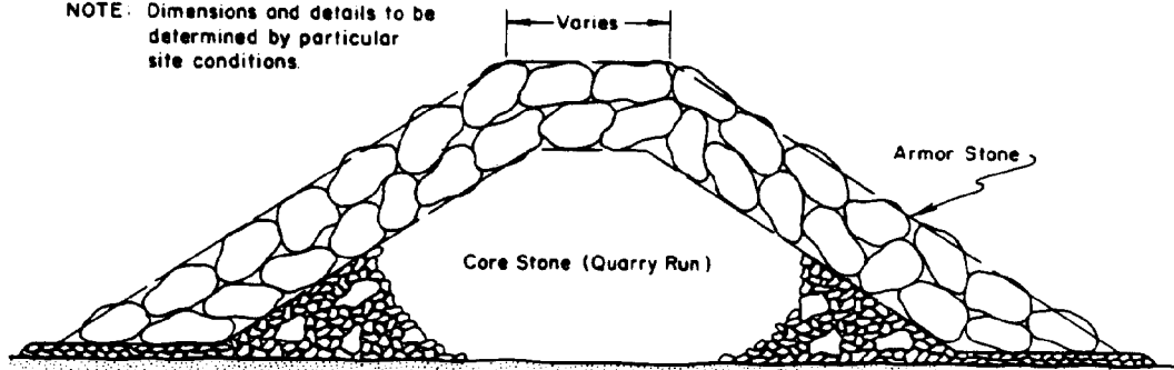
Figure 5-9. Rubble-mound groin
