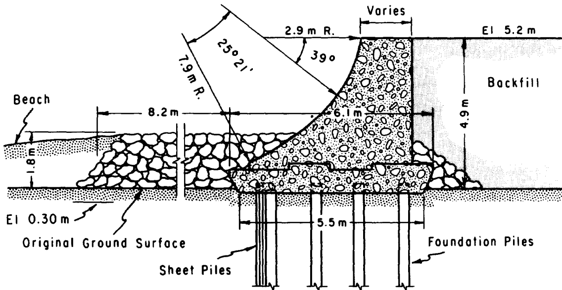
Figure 5-2. Concrete curved-face seawall
