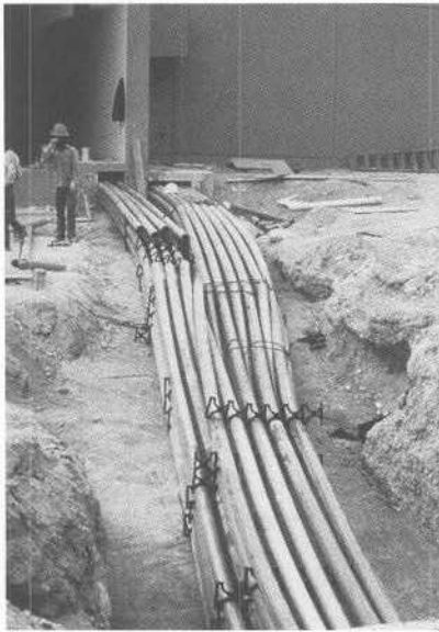
Utility ducts (left); a backfilled and compacted utility trench.
