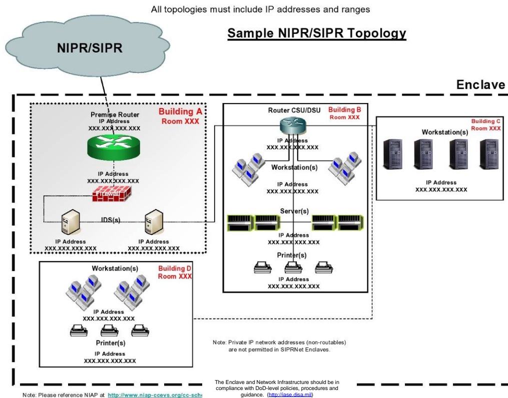
Figure 1 NIPRNET/SIPRNET Topology Sample
