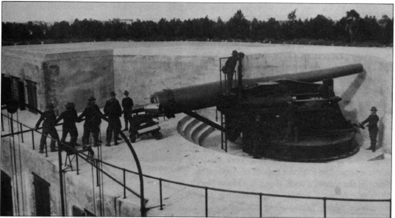
Loading position of a 10-inch disappearing gun, Sandy Hook, New Jersey.
