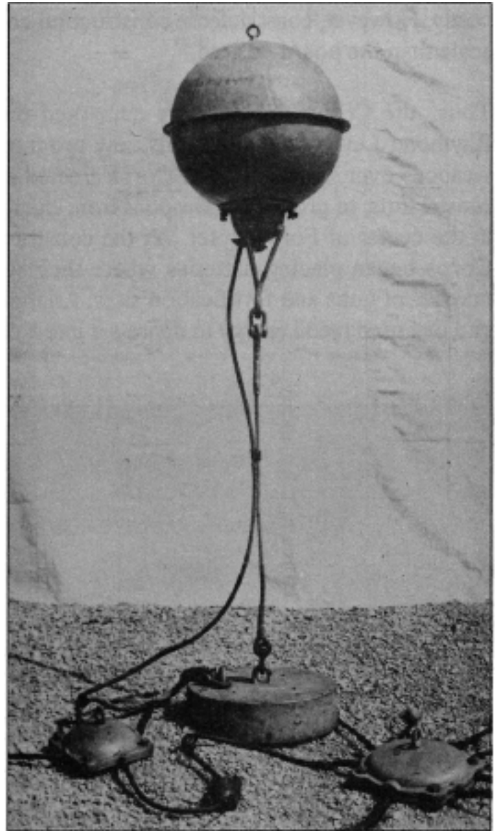
A buoyant torpedo (submarine mine) and connections. National Archives, 77-F-179-39-61
