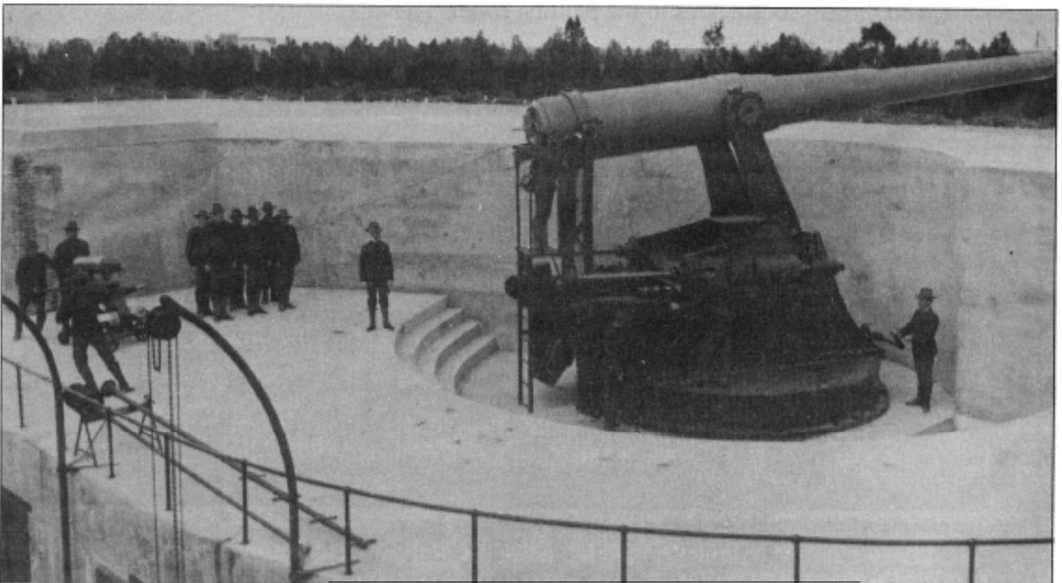
Firing position of a 10-inch disappearing gun, Sandy Hook, New Jersey.
