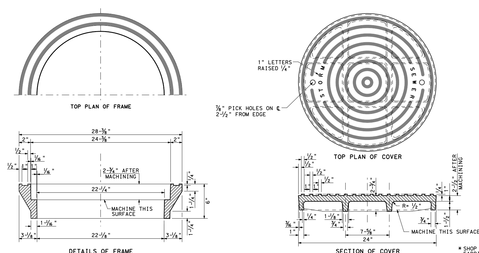
MANHOLE FRAME AND COVER TYPE A
