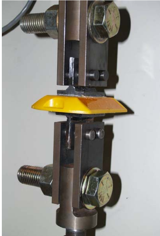
Figure 102. View of RRPM Type 3 and Tee-Stubs Inserted into Tension Test Fixtures.
