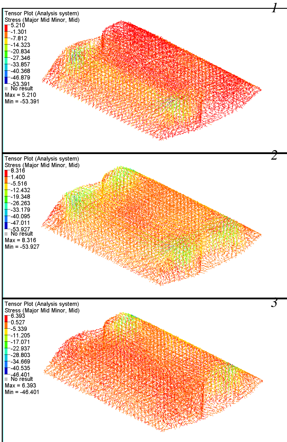
Figure 31. Stress Tensor Plots for RRPM Type B on Rigid Pavement.
