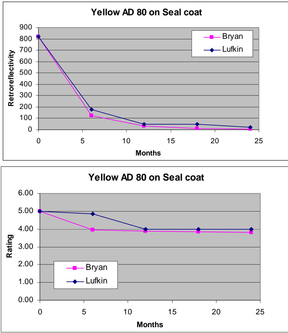
Figure 96. Performance of AD80 Marker on Seal Coat Surface.
