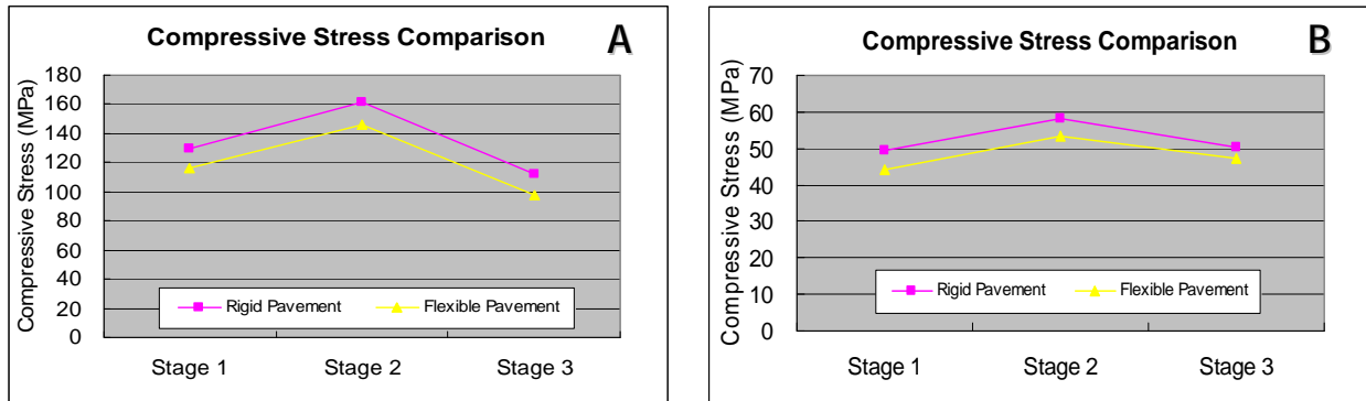
Figure 39. Comparison of Critical Compressive Stress for RRPM Types A and B.
