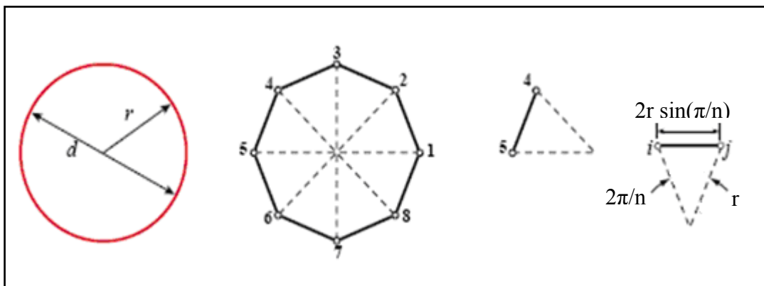
Figure 13. Simple Example Illustrating FEM (33).
