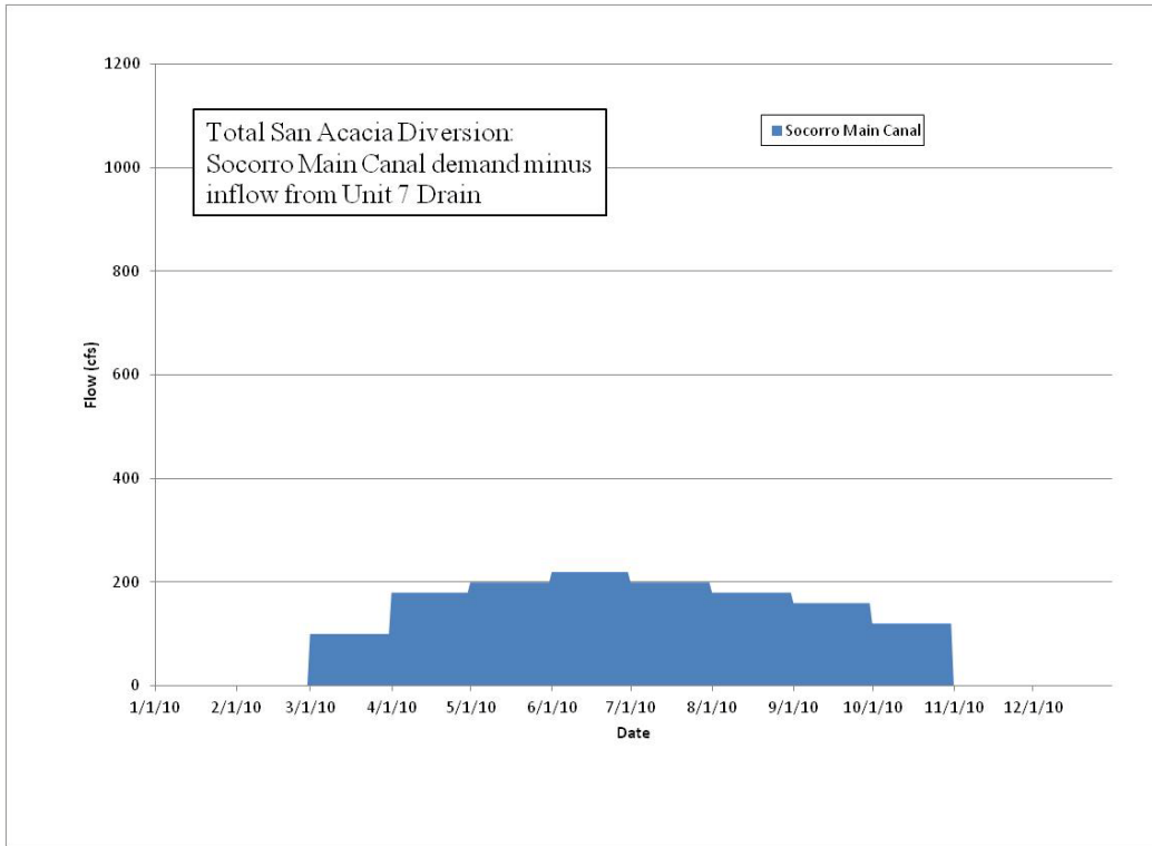
Figure 4. Total MRGCD Demand at Diversions to the San Acacia Division.
