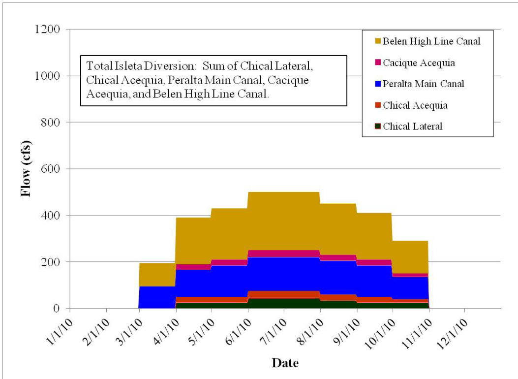
Figure 3. Total MRGCD Demand at Diversions to the Isleta Division.
