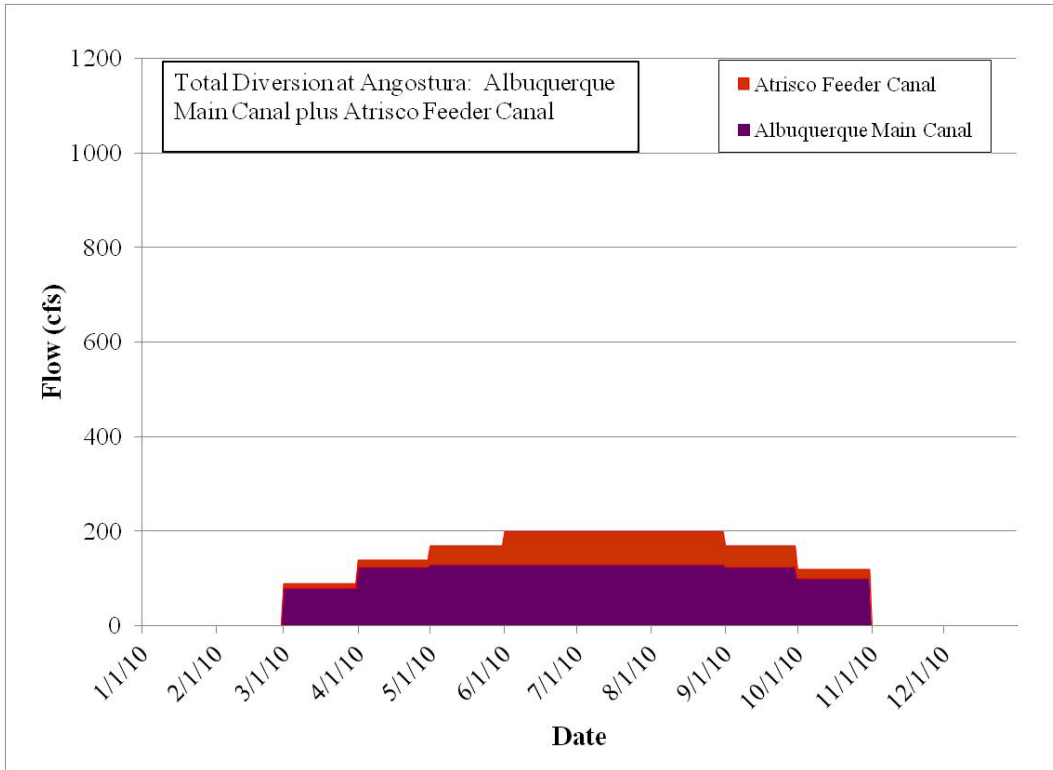
Figure 2: MRGCD Demand at Diversions to the Albuquerque Division.
