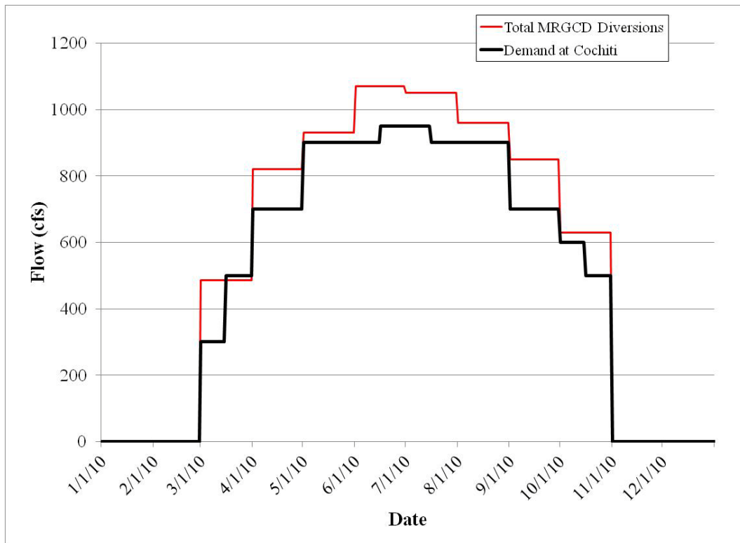
Figure 6. Comparison of Total MRGCD Demand at Cochiti to Total of Demand at All Diversions (difference is due to return flows).
