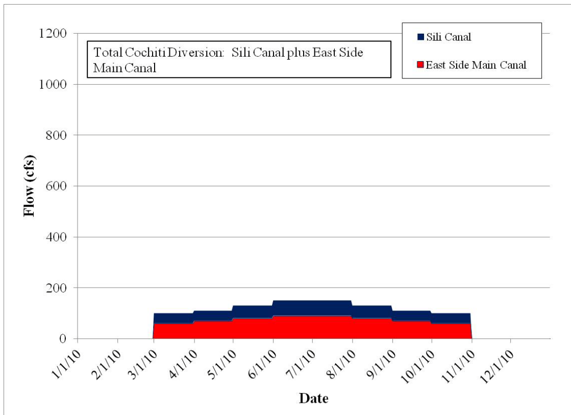
Figure 1. MRGCD Demand at Diversions to the Cochiti Division.
