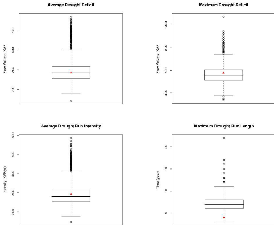
Figure 6. Distributions of statistics of drought for the traces generated by the HMC
