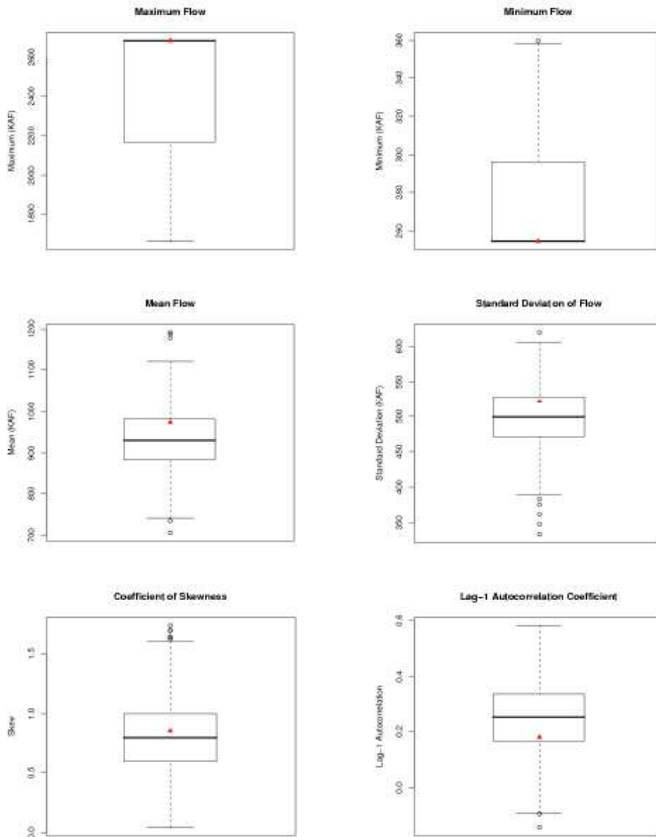
Figure 3. Distributions of statistics of annual flows for the traces generated by the NHMC.
