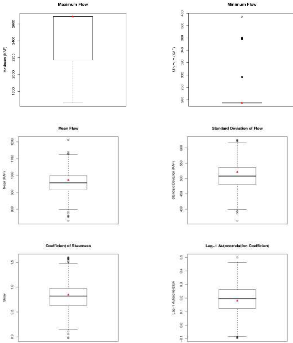
Figure 5. Distributions of statistics of annual flows for the traces generated by the HMC.
