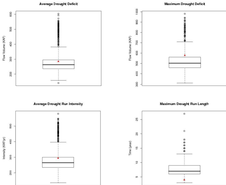
Figure 4. Distributions of statistics of drought for the traces generated by the NHMC
