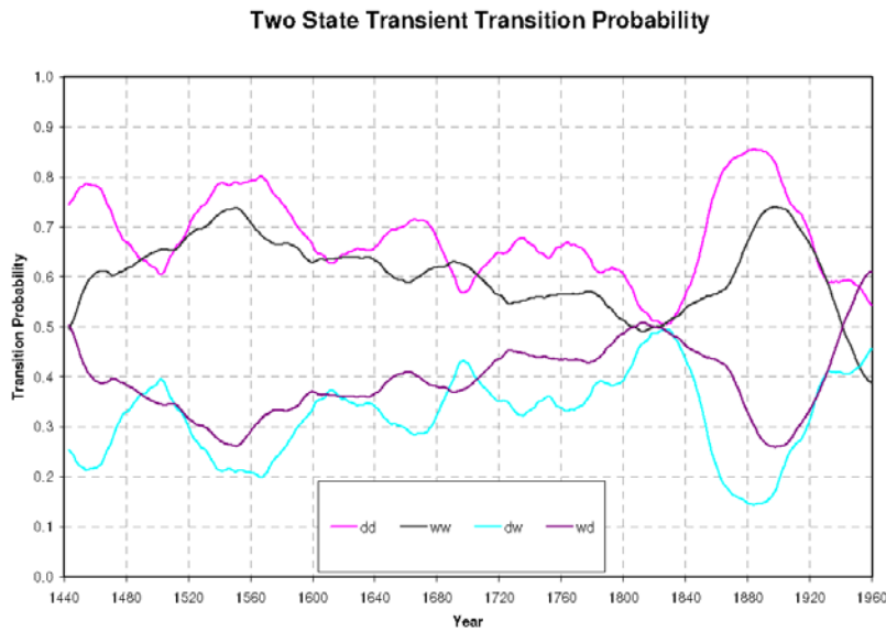
Figure 2. Two state – four transitions (dd, dw, wd, ww) transient transition probability based on the binary dry/wet time series of length 604 (1400-2003).
