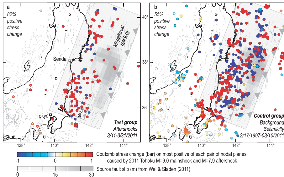
Fig. 1. Stress imparted by the Wei and Sladen (2011) source model and the M = 7.9 aftershock are resolved on both nodal planes of NIED F-net aftershock (a) and background, or pre-Tohoku (b) focal mechanisms. Although both planes are used for the calculations summarized in Table 1, the most positively-stressed of each pair of nodal planes is shown here. The effect of the mainshock stress imparted to the mechanisms is judged from the percent gain in positively-stressed mechanisms after the mainshock (the test group) relative to the background shocks (the control group). Results for all 6 models are given in Table 1.
