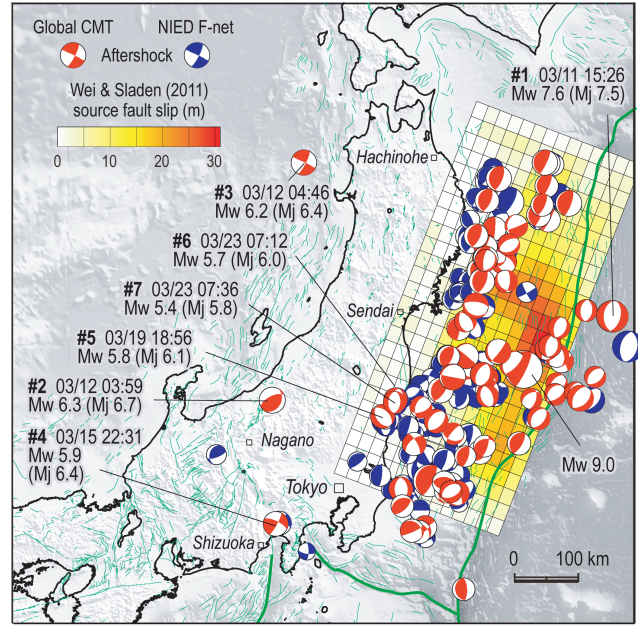
Fig. 2. Focal mechanisms of the March 2011 Tohoku Earthquake aftershocks from two catalogs, with important aftershocks examined for stress transfer keyed to Table 2. The mainshock promotes failure of five of the seven events regardless of nodal plane or friction; for the remaining two events (#1–2) only one of the nodal planes is promoted (see Table 2). All aftershocks east of the mainshock are outer trench slope normal events, but there is also a group of coastal normal events midway between Tokyo and Sendai.
