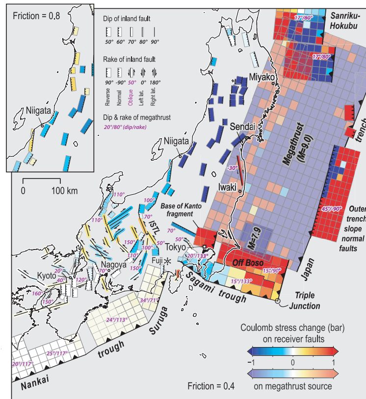
Fig. 3. Stress imparted by the Wei and Sladen (2011) source model and the M = 7.9 aftershock to surrounding active faults (Research Group for Active Faults in Japan, 1991; Headquarters for Earthquake Research Promotion, 2011), resolved in their inferred rake directions (oblique rakes are labeled). Top depth and bottom depths of most of the active faults are set to 0 and 15 km.
