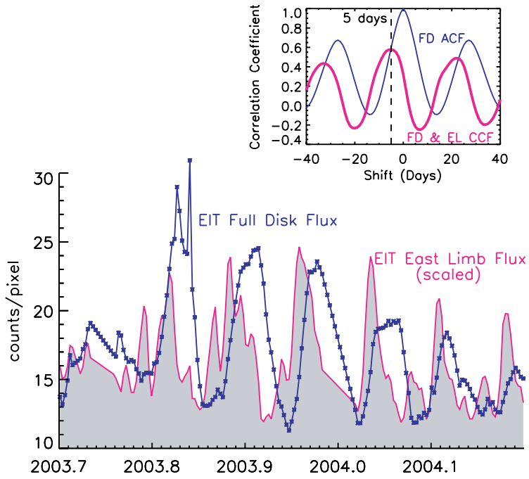
FIGURE 7 The net, disk-integrated solar EUV radiation at 28.4 nm from Fig. 6(a) is compared with the radiation from the east limb (left side of each image in Fig. 6). As the cross-correlation function in the inset figure shows, the east limb (EL) flux peaks approximately five days prior to the full disk (FD) flux.
