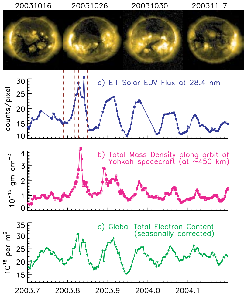
FIGURE 6 Images of the Sun made by SOHO EIT 1 at 28.4 nm show the movement of bright active regions across the Sun's disk as a result of its rotation on its axis. Shown in (a) are the resultant changes in the net solar EUV radiation obtained by summing all pixels in each image during a period of six solar rotations. During the same period, total mass densities in the upper atmosphere estimated along the track of the Yohkoh spacecraft (altitude ~450 km) from TLEs 2 varied as shown in (b). The total electron content variations shown in (c) are derived from GPS by CODE. 3
