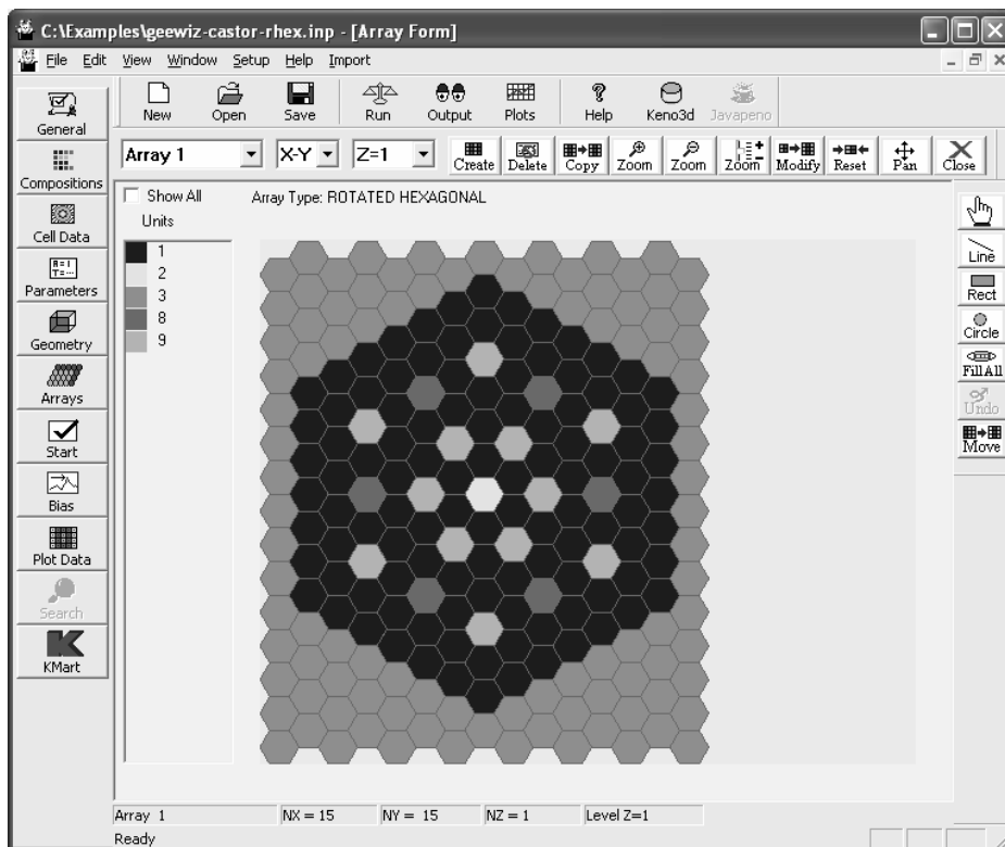
Figure 1. Array form for rotated hexagonal array in KENO-VI.
