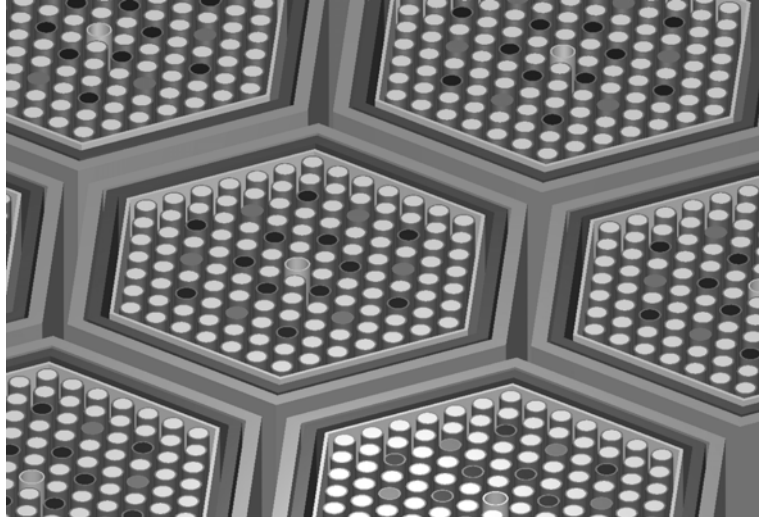
Figure 3. KENO3D close-up view of assemblies in cask.
