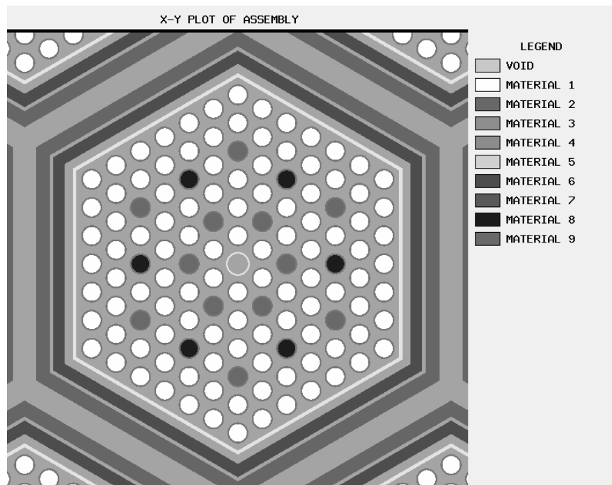
Figure 2. Sample 2-D KENO-VI geometry plot.
