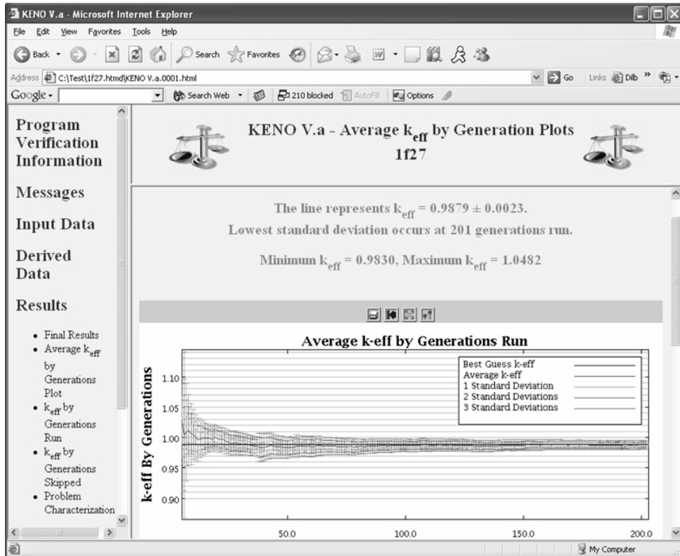
Figure 6. Plot of average k_{\text{eff}} by generations run.
