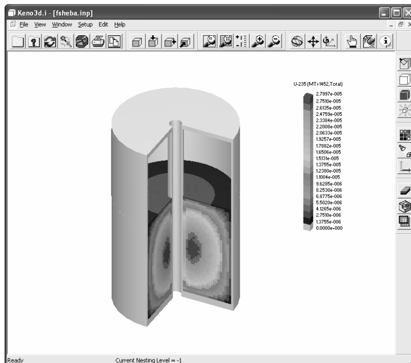
Figure 4. KENO3D plot of the ^{235}\text{U} fission activity.
