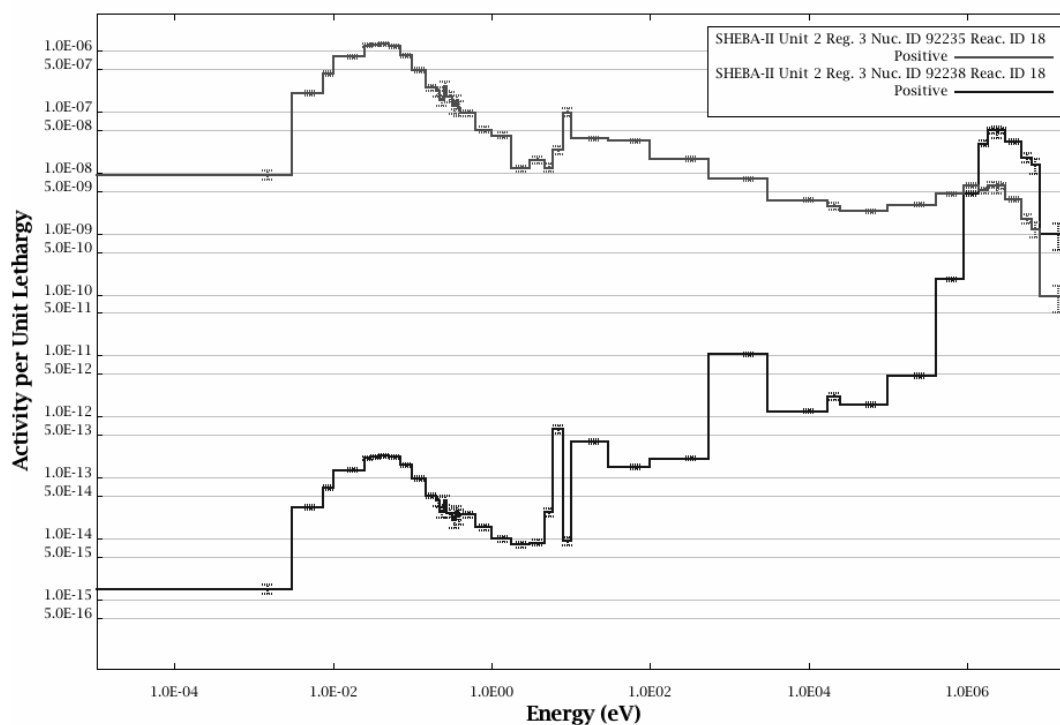
Figure 5. Javapeño plot of ^{235}\text{U} and ^{238}\text{U} fission activities.
