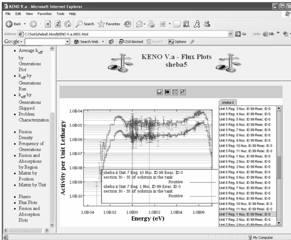
Figure 7. Plot of flux spectra by region.
