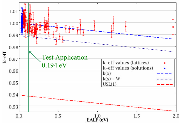
Fig. 2. Trend plot of k_{\text{eff}} vs. EALF for 214 benchmarks.
