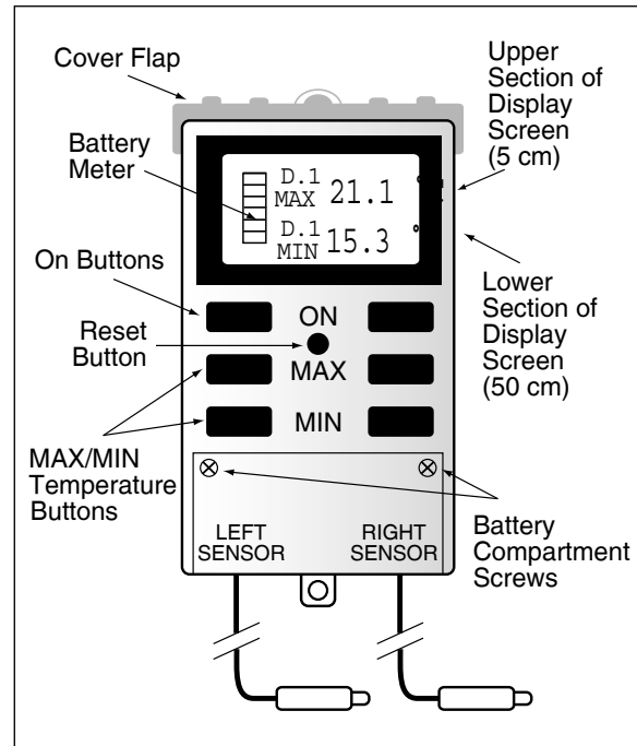
Figure SO-MU-1: Digital Multi-Day Max/Min Thermometer
