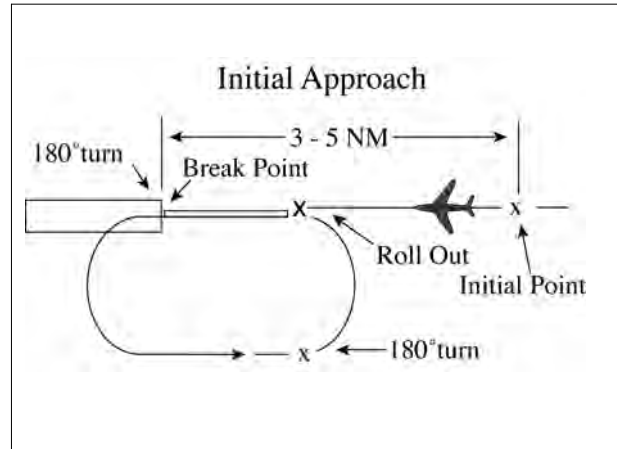
FIG 3-10-13 Overhead Maneuver
