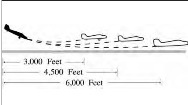
FIG 3-10-5 Same Runway Separation
