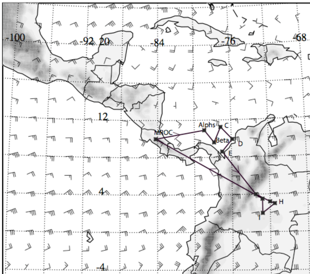
NCEP GFS Wind Flags (knots) on Press 250. hPa Init:2007080706 Valid:2007081018
