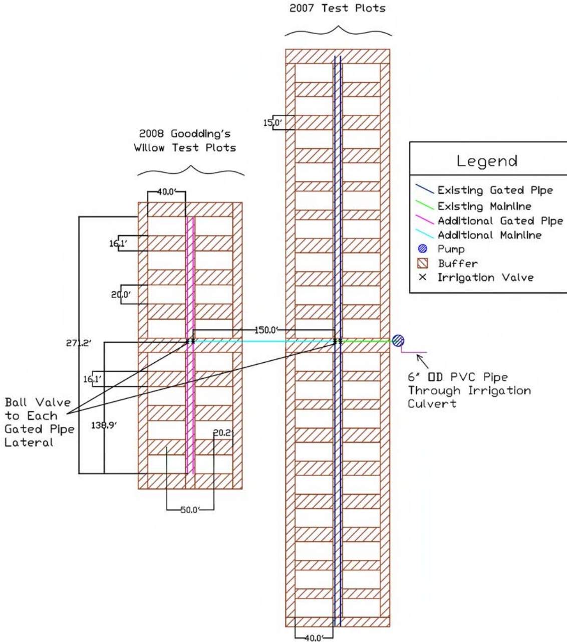
Figure 30. As-built irrigation specifications for 2007 and 2008 Goodding's willow small-scale study at Cibola NWR Field 51.
