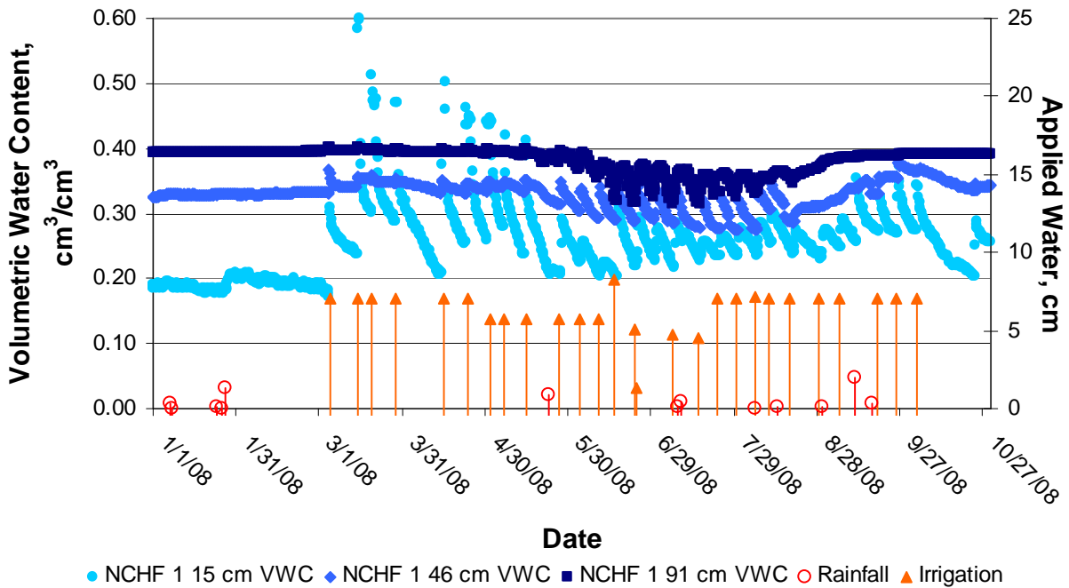
Figure 40. Soil volumetric water content for 2007 small-scale study plot NCHF 1 during the 2008 growing season.
