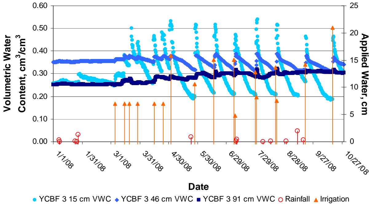
Figure 41. Soil volumetric water content for 2007 small-scale study plot YCBF 3 during the 2008 growing season.
