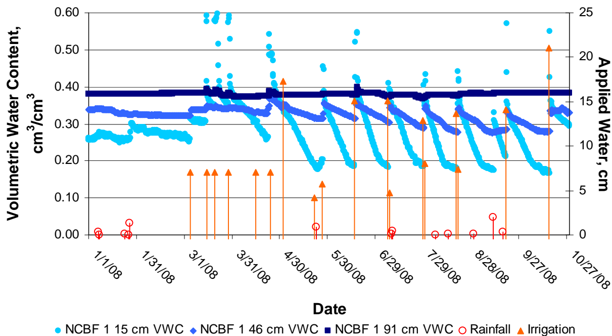
Figure 38. Soil volumetric water content for 2007 small-scale study plot NCBF 1 during the 2008 growing season.
