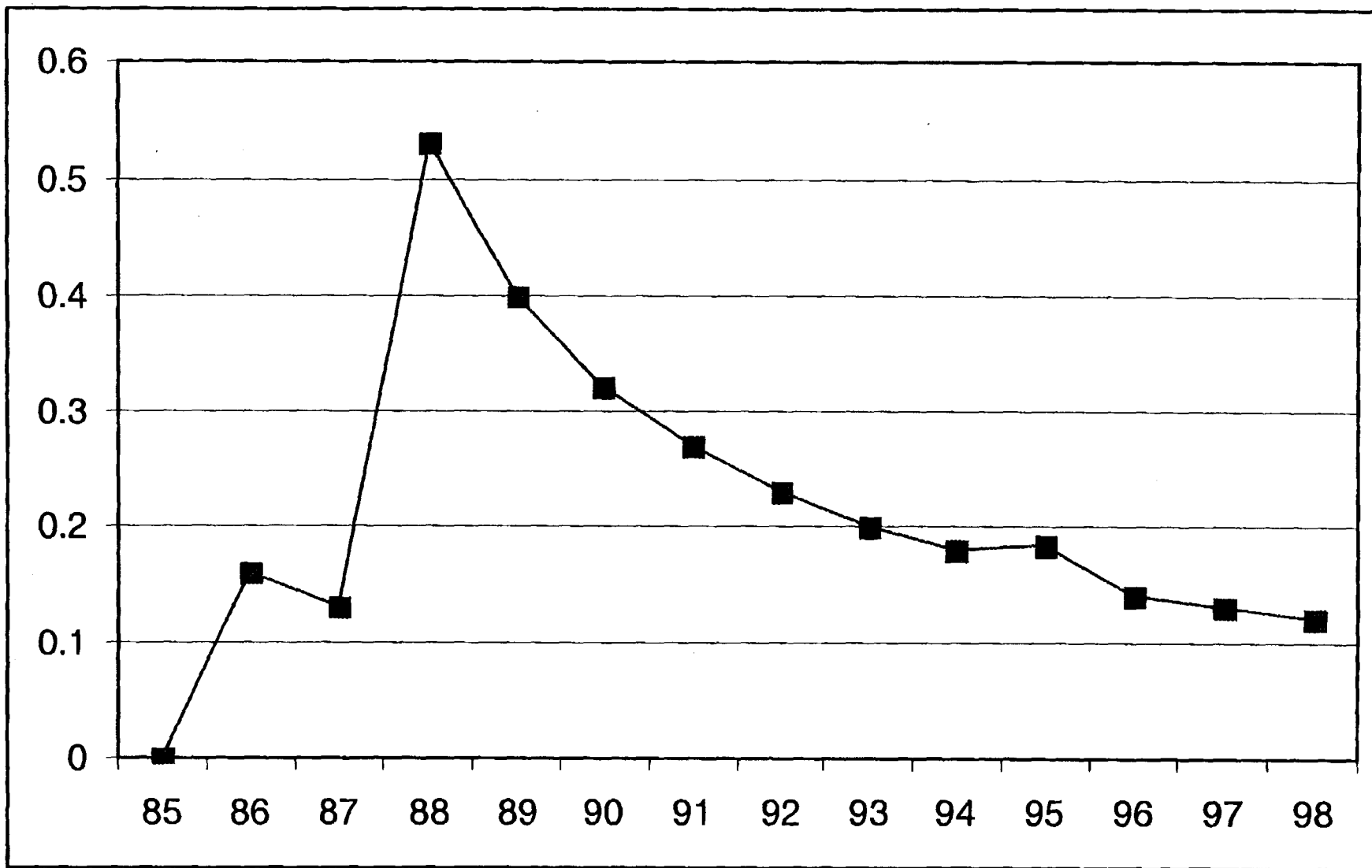
Figure 1. Corrosion probe data (in MYP) for the electrical resistance, direct buried probes in the CPP-749 storage area.
