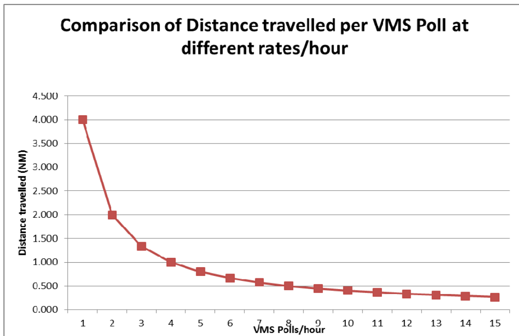
Figure 8. Relationship between the distances a vessel travels (nm) and increasing VMS polls per hour. Source: USCG.
