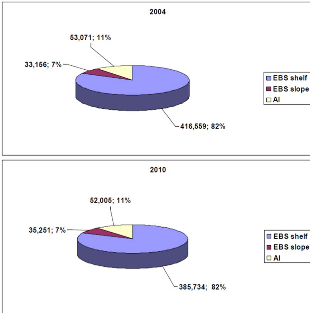
Figure 57 Distribution of skate biomass in the three sub-regions of the BSAI (Eastern Bering Sea shelf and slope, and the Aleutian Islands) from 2004 to 2010. Data are biomass estimates from the annual AFSC groundfish surveys. Source: AFSC and NPFMC.
