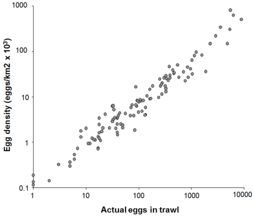
Figure 51 Relationship between skate eggs encountered in the trawl and expansion to egg density. Source: AFSC.
