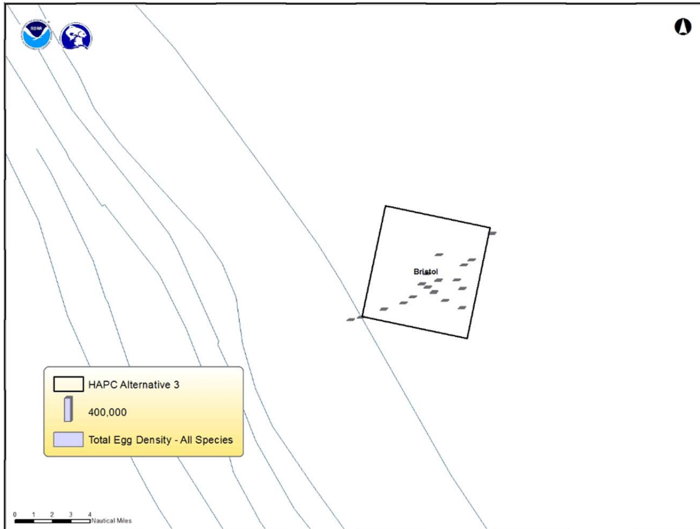
Figure 16 Total skate egg density/km 2 for all skate species in the Bristol site under Alternative 3. Source: NMFS HCD and AFSC.
