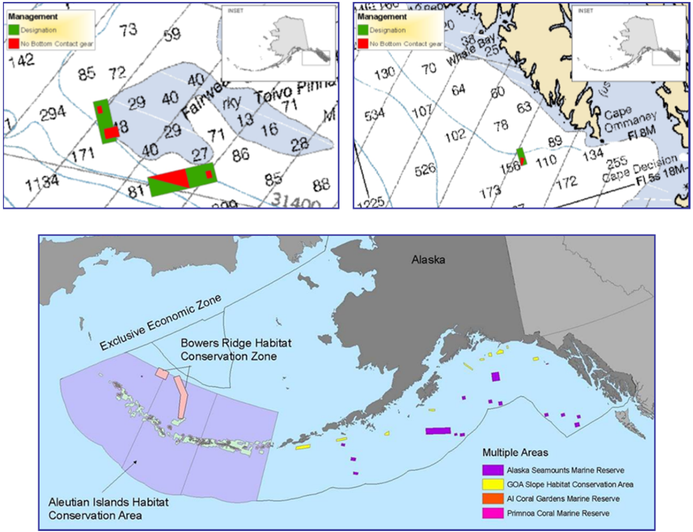
Figure 1 Locations of current HAPC areas. Source: NPFMC.
