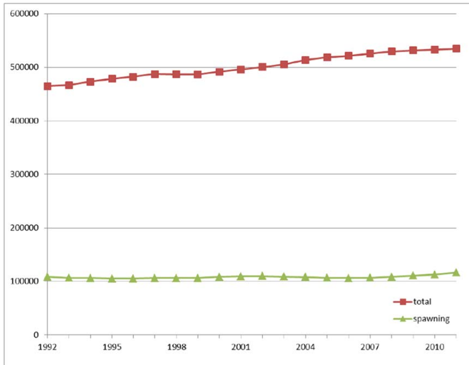
Figure 66 Time series of model estimates for total (age 0+) biomass (t) and female spawning biomass (t).
