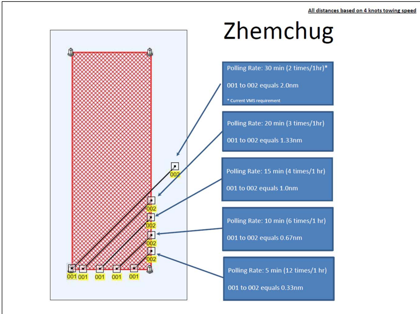
Figure 29 Evaluation of different VMS polling rates relative to skate site boundaries described by Alternative 2 for the Zhemchug HAPC. Source: NMFS HCD.
