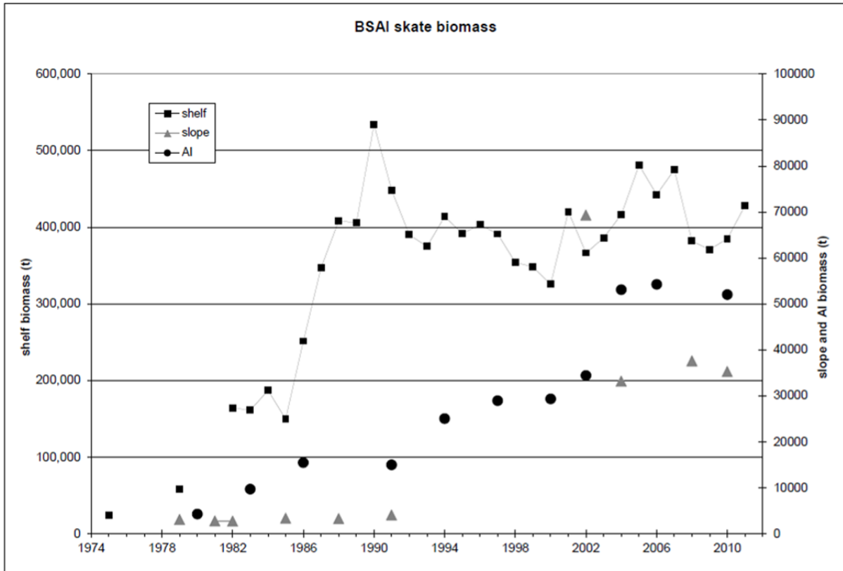
Figure 67 Aggregated skate biomass (mt) estimated from RACE bottom trawl surveys in each of the three major habitat areas in the eastern Bering Sea, from 1975 to 2011. Note that slope and AI estimates are much smaller and pertain to the secondary y-axis.
