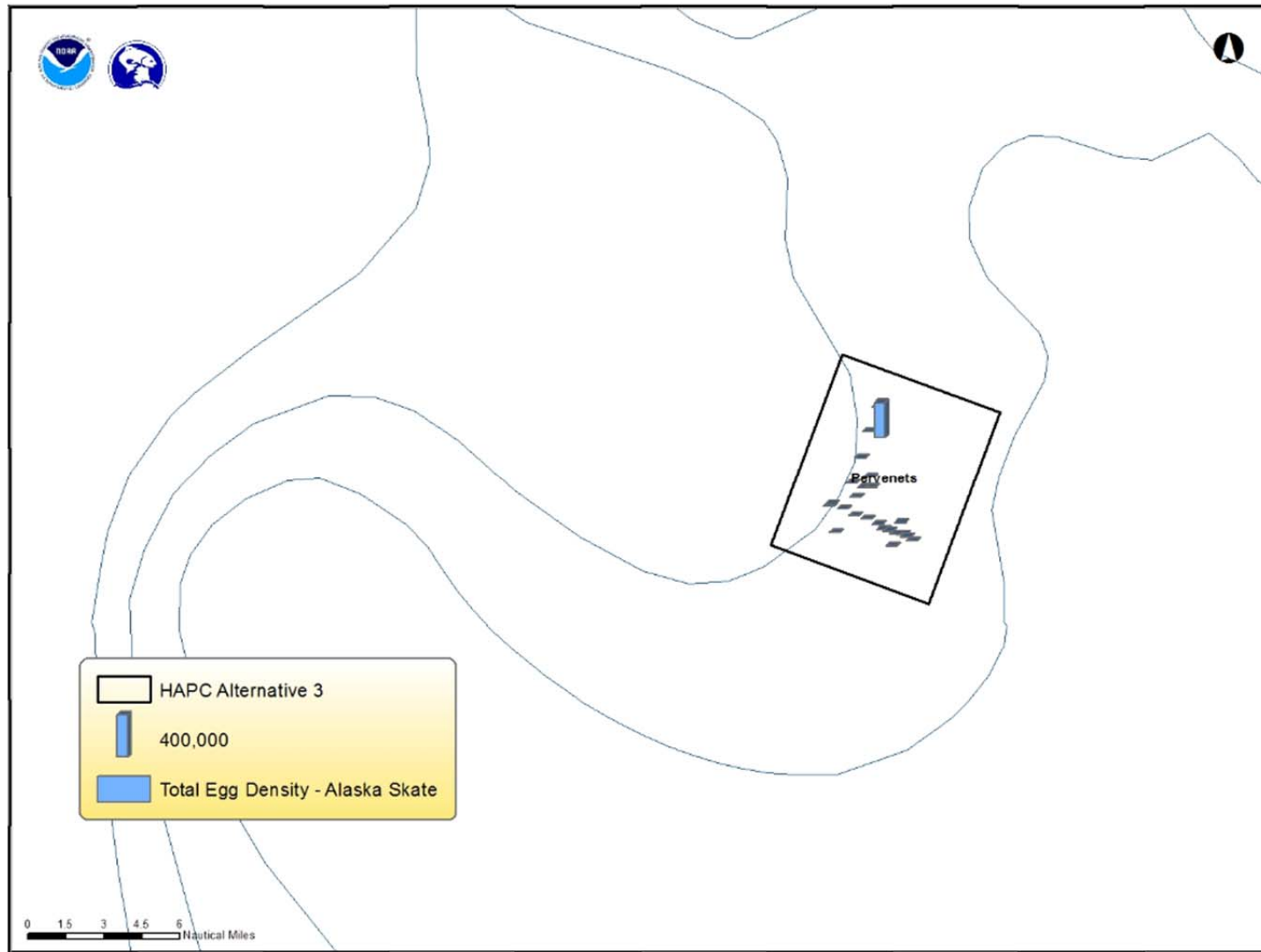
Figure 17 Total Alaska skate egg density/km 2 in the Pervenets site under Alternative 3. Source: NMFS HCD and AFSC.
