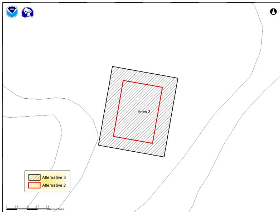
Figure 4 Bering 2 site under Alternative 2 (17.5 nm 2 , red boundary) and Alternative 3 (40.9 nm 2 , black boundary).
