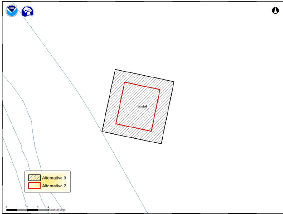
Figure 5 Bristol site under Alternative 2 (13.7 nm 2 , red boundary) and Alternative 3 (34.4nm 2 , black boundary). Source: NMFS HCD.
