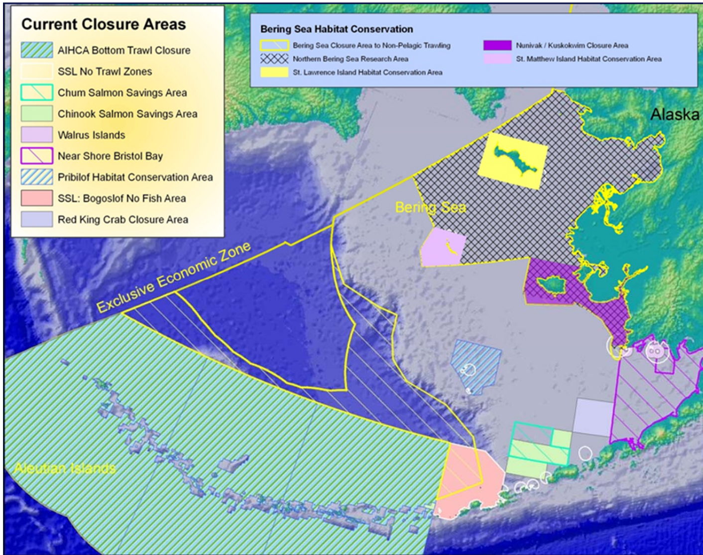
Figure 2 Current Eastern Bering Sea habitat conservation and bottom trawl closure areas. Source: NPFMC.
