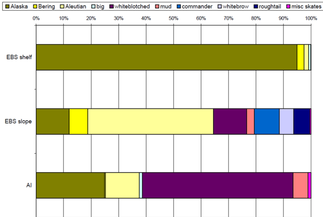
Figure 55 Skate species composition (by weight) by BSAI subregion, from surveys conducted in each region in 2010. “Misc. skates” contains longnose, deepsea, and unidentified skates. Source: AFSC.
