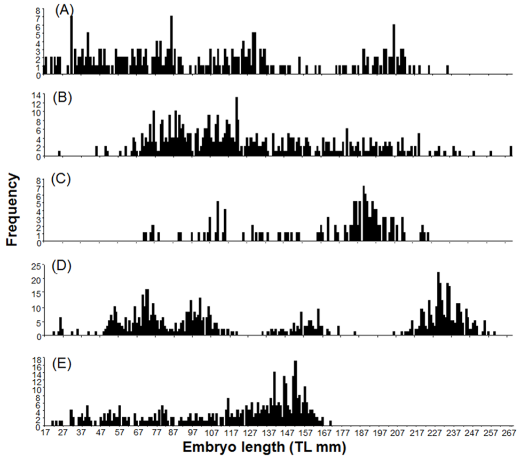
Figure 53 Embryo length frequencies from five areas of skate egg concentration for three skate species in the eastern Bering Sea: A) the Alaska skate-Bering Canyon; B) the Alaska skate-Pervenets Canyon; C) the Aleutian skate-Bering Canyon; D) the Aleutian skate-Pervenets Canyon; and E) the Bering skate-Pervenets Canyon.
