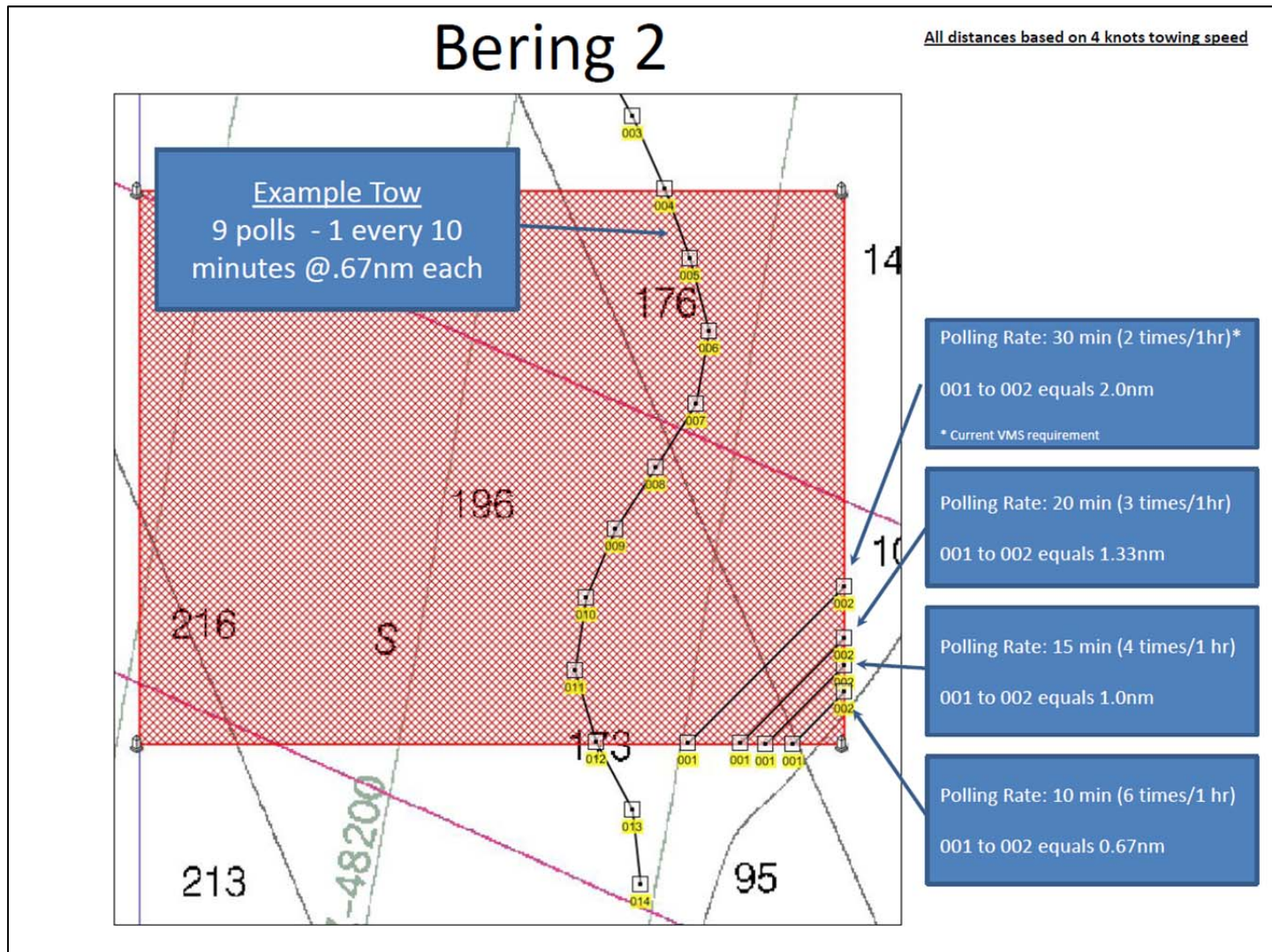
Figure 31 Evaluation of different VMS polling rates relative to skate site boundaries described by Alternative 2 for the Bering 2 HAPC. Source: NMFS HCD.
