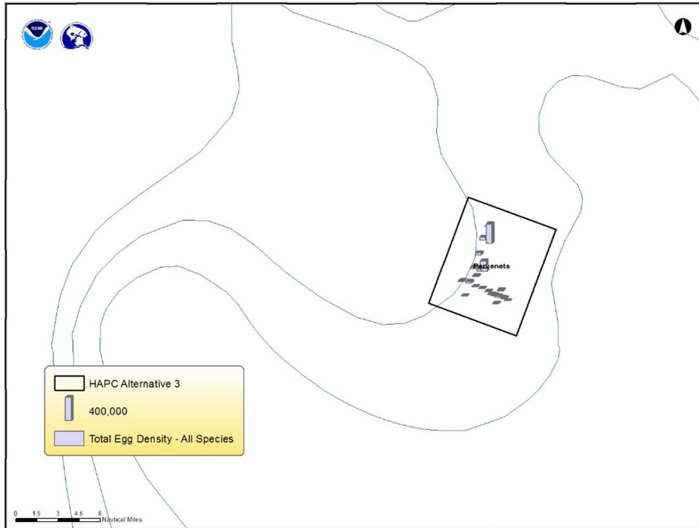
Figure 20 Total skate egg density/km 2 for all skate species in the Pervenets site under Alternative 3. Source: NMFS HCD and AFSC.
