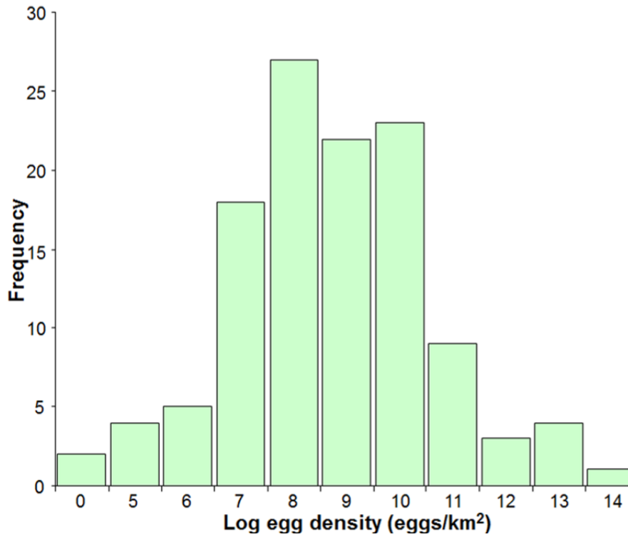
Figure 52 Distribution of egg densities from all trawls in areas of skate egg concentration. Source: AFSC.
