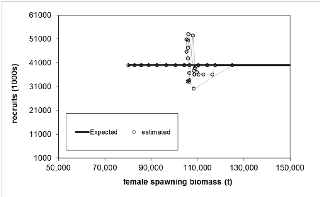
Figure 65 Relationship between female spawning biomass (t) and the number of age 0 recruits (in thousands of fish). Time series of individual year class estimates from SS2 is shown with a Beverton-Holt stock-recruit relationship with a steepness of 1.0.
