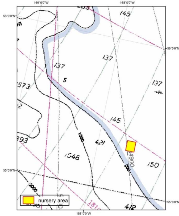
Figure 47 Map detail of the Bristol HAPC site in the vicinity of the Bristol Canyon under Alternative 2. Source: AFSC.
