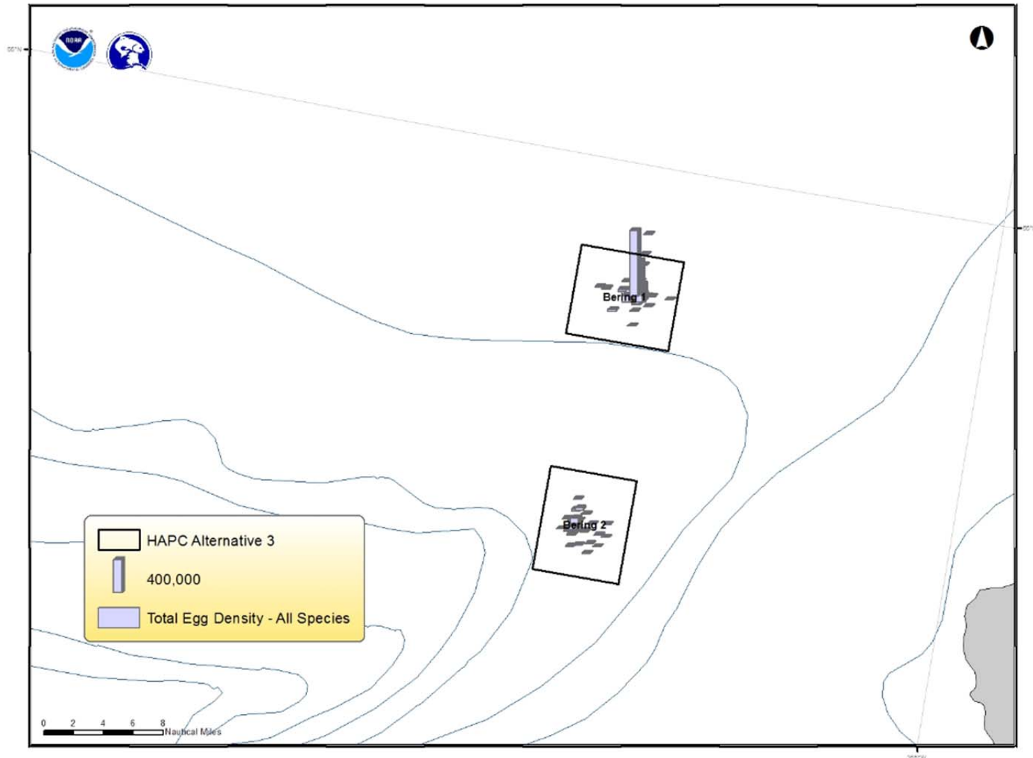
Figure 12 Total skate egg density/ \text{km}^2 , for all skate species, in the Bering 1 and 2 sites under Alternative 3. Source: NMFS HCD and AFSC.
