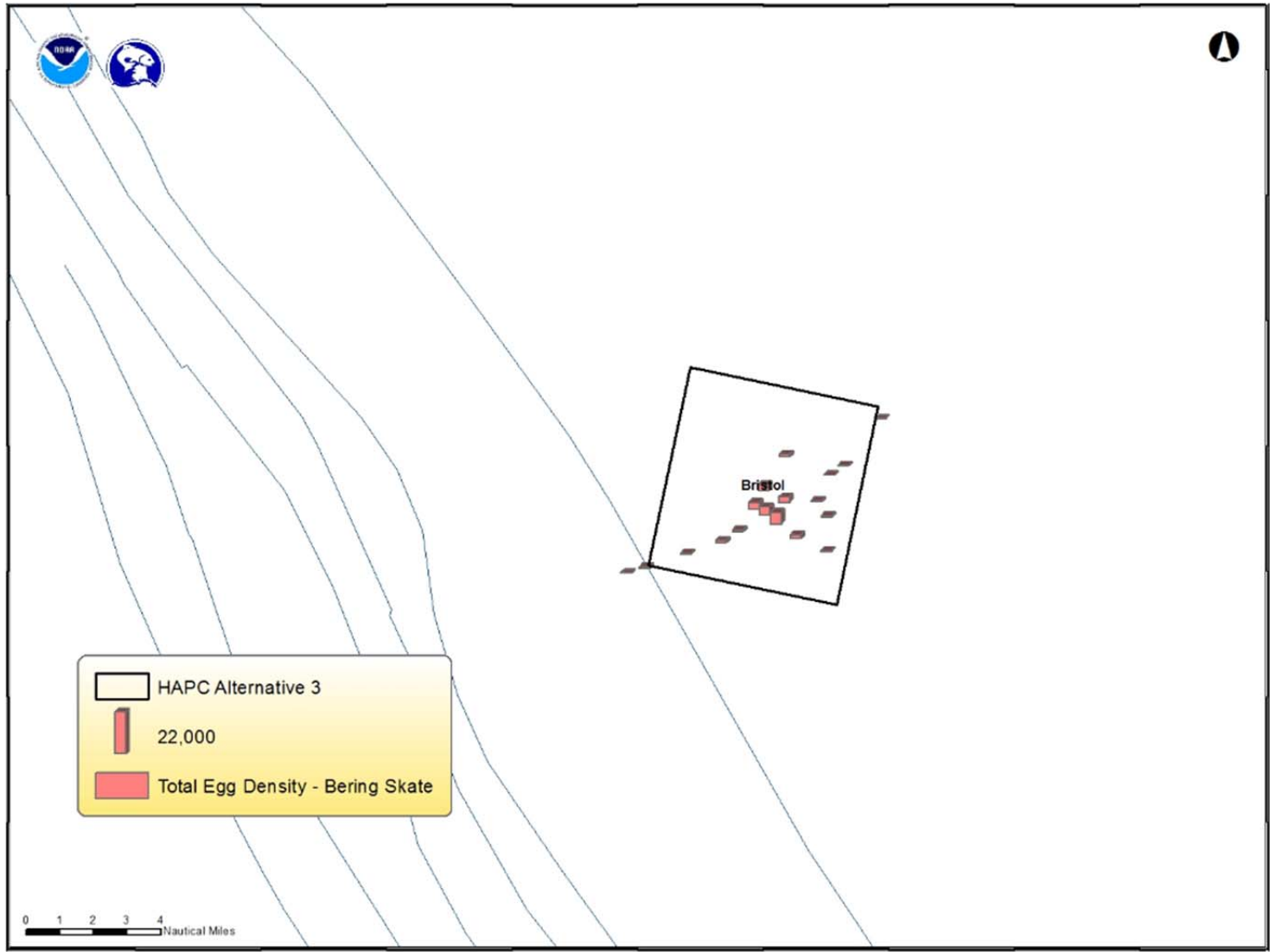
Figure 15 Total Bering skate egg density/km 2 in the Bristol site under Alternative 3. Source: NMFS HCD and AFSC.
