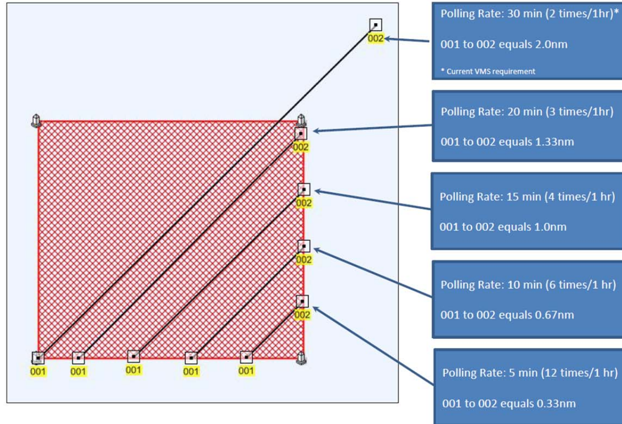
Figure 28 Evaluation of different VMS polling rates relative to skate site boundaries described by Alternative 2 for the Pribilof HAPC. Source: NMFS HCD.
