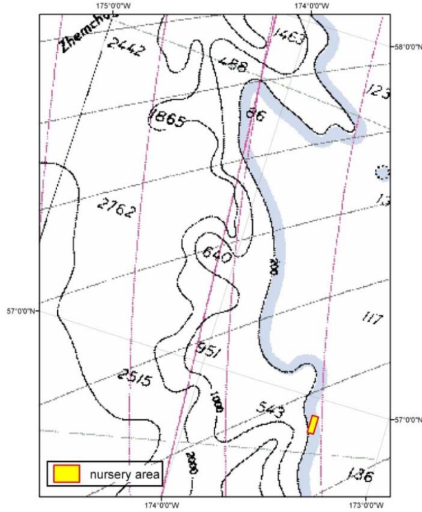
Figure 49 Map detail of the Zhemchug HAPC site south of the Zhemchug Canyon under Alternative 2. Source: AFSC.
