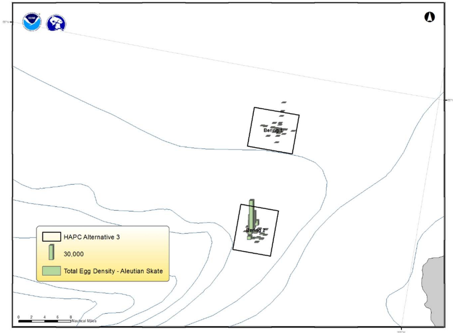
Figure 10 Total Aleutian skate egg density/km 2 in the Bering 1 and 2 sites under Alternative 3. Source: NMFS HCD and AFSC.
