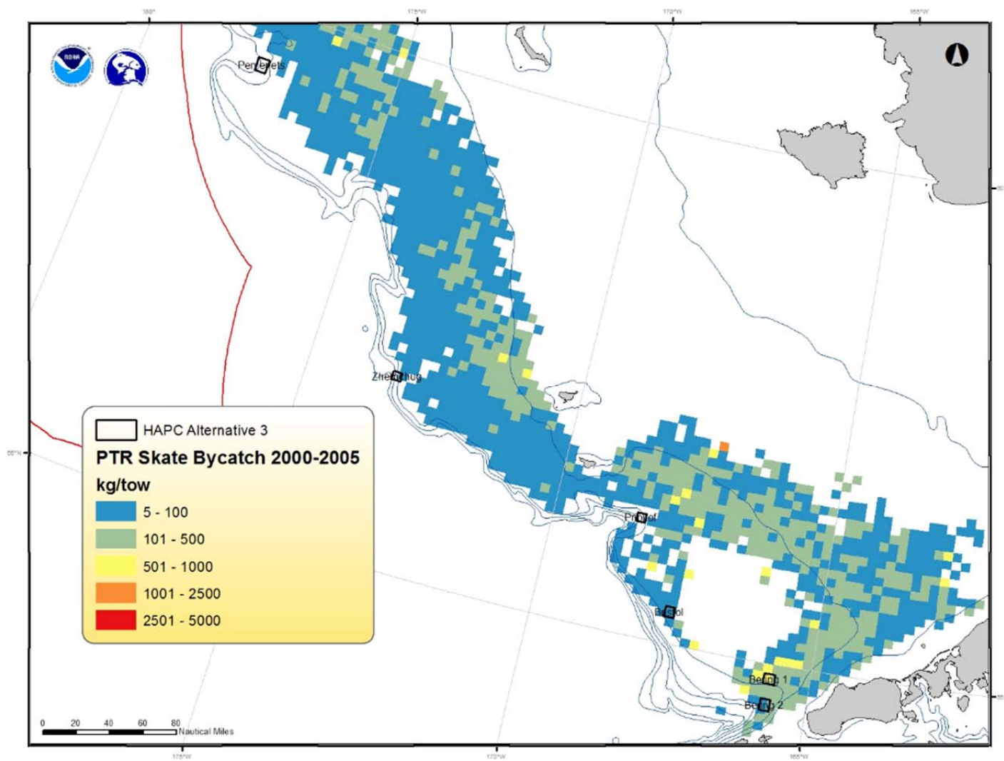
Figure 39 Observed pelagic trawl (PTR) skate bycatch from 2000 to 2005 based on tows with observed skate bycatch only. Source: NMFS HCD.
