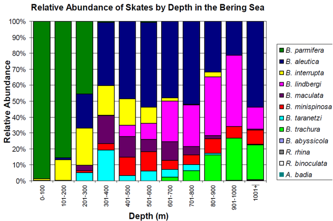
Figure 56 Relative abundance of skate species in the Bering Sea by depth. Source: Stevenson et al. 2006.
