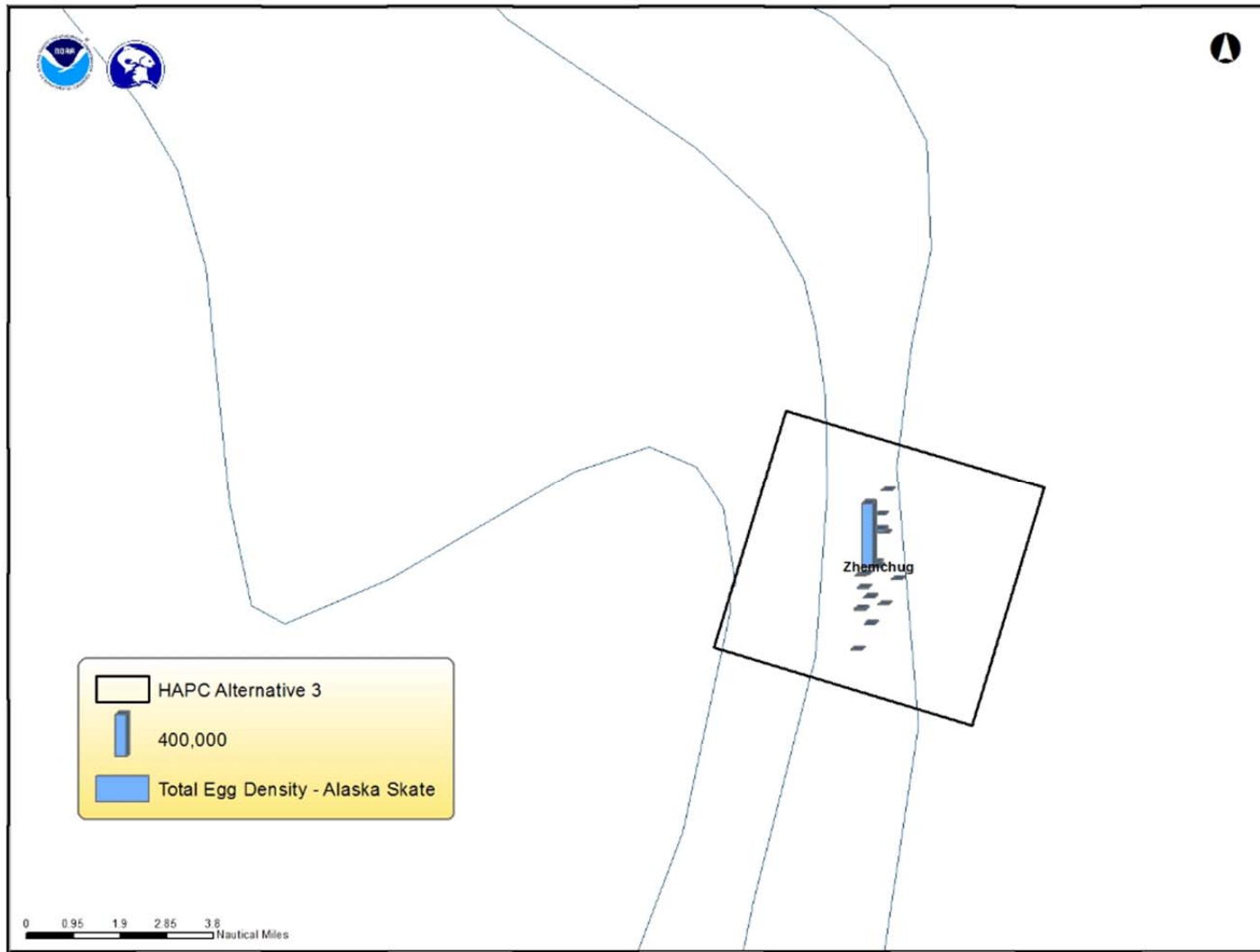
Figure 21 Total Alaska skate egg density/ \text{km}^2 in the Zhemchug site under Alternative 3. Source: NMFS HCD and AFSC.
