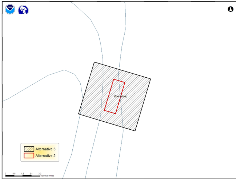
Figure 7 Zhemchug site under Alternative 2 (3.2 nm 2 , red boundary) and Alternative 3 (27.4 nm 2 , black boundary). Source: NMFS HCD.
