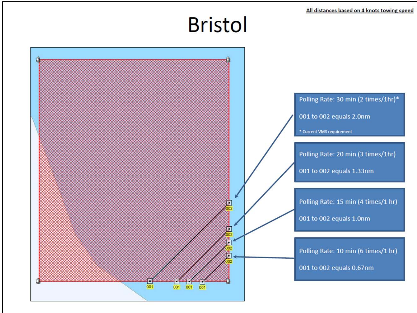
Figure 27 Evaluation of different VMS polling rates relative to skate site boundaries described by Alternative 2 for the Bristol HAPC. Source: NMFS HCD.
