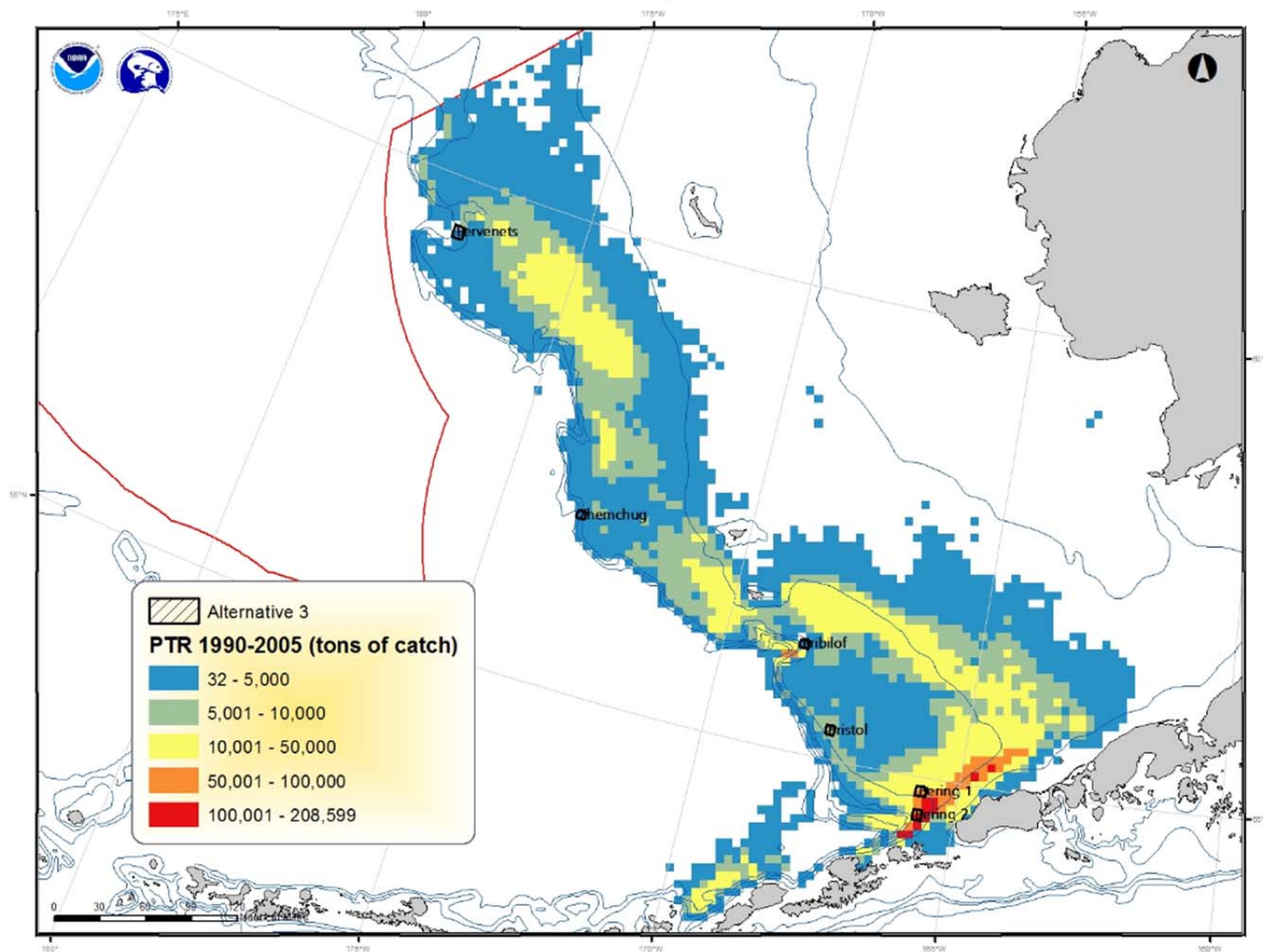
Figure 38 Skate egg concentration areas with observed pelagic trawl (PTR) in tons of catch from 1990 to 2005 under Alternative 3. Source: NMFS HCD.
