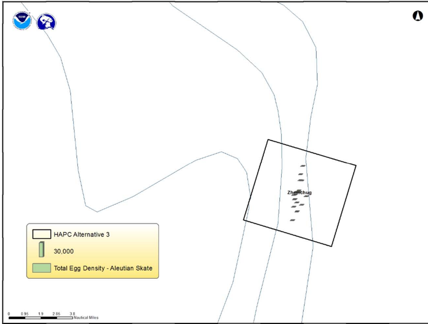
Figure 22 Total Aleutian skate egg density/km 2 in the Zhemchug site under Alternative 3. Source: NMFS HCD and AFSC.
