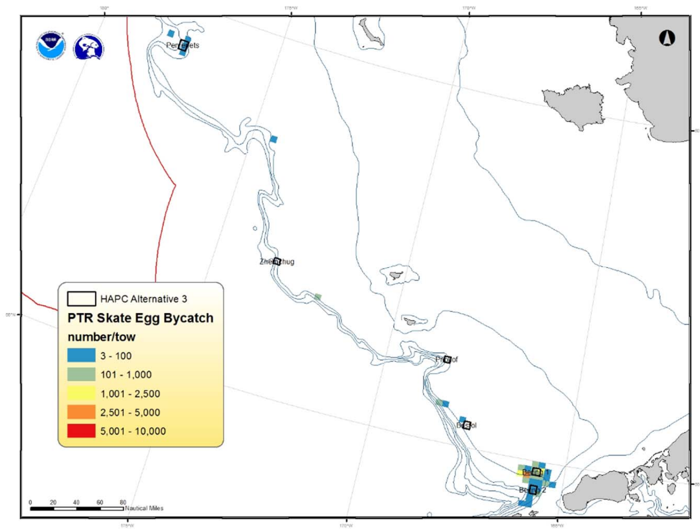
Figure 41 Observed pelagic trawl (PTR) skate egg bycatch from 1998 to 2011 based on tows with observed skate egg bycatch only. Source: NMFS HCD.
