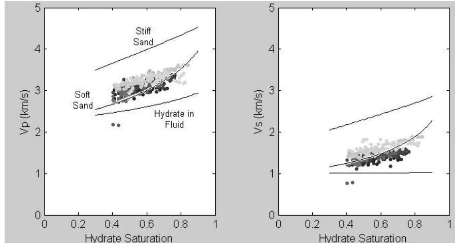
Figure 5.2. P - and S -wave velocity versus methane hydrate saturation in a quartz-sand-brine-hydrate system. The upper curves are from the stiff-sand model. The lower curves are from the hydrate-in-fluid model. The middle curves are from the soft-sand model. The symbols are log data from a methane hydrate well Mallik-2L-38. The data are color-coded by depth where light is for deep and dark is for shallow. The model curves are calculated with parameters relevant to the shallow-depth portion of the well.
