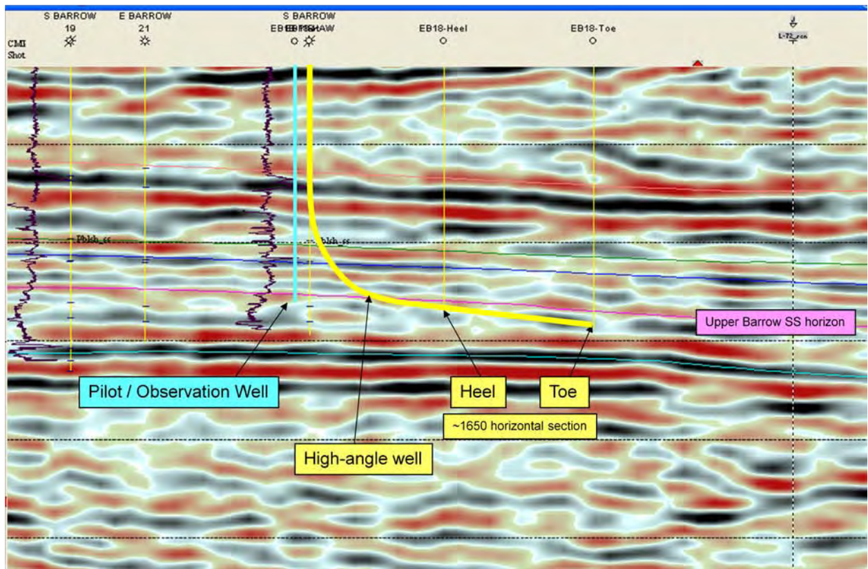
Figure 9: Observation Well and Horizontal Well on Seismic Cross Section
